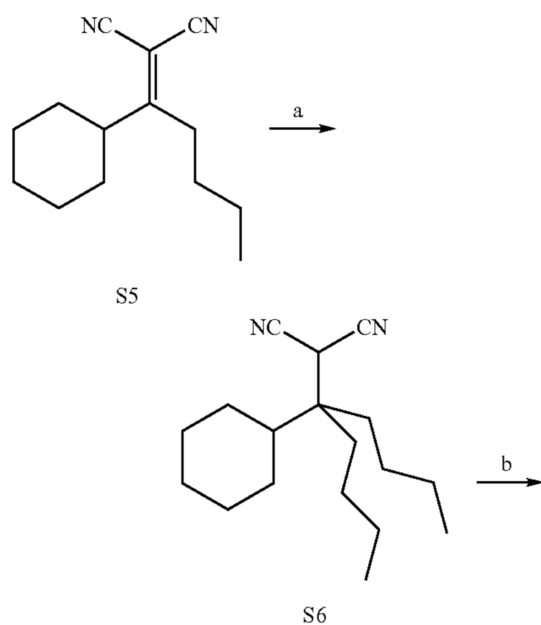
Scheme 2. Synthesis of TPA-2-S
