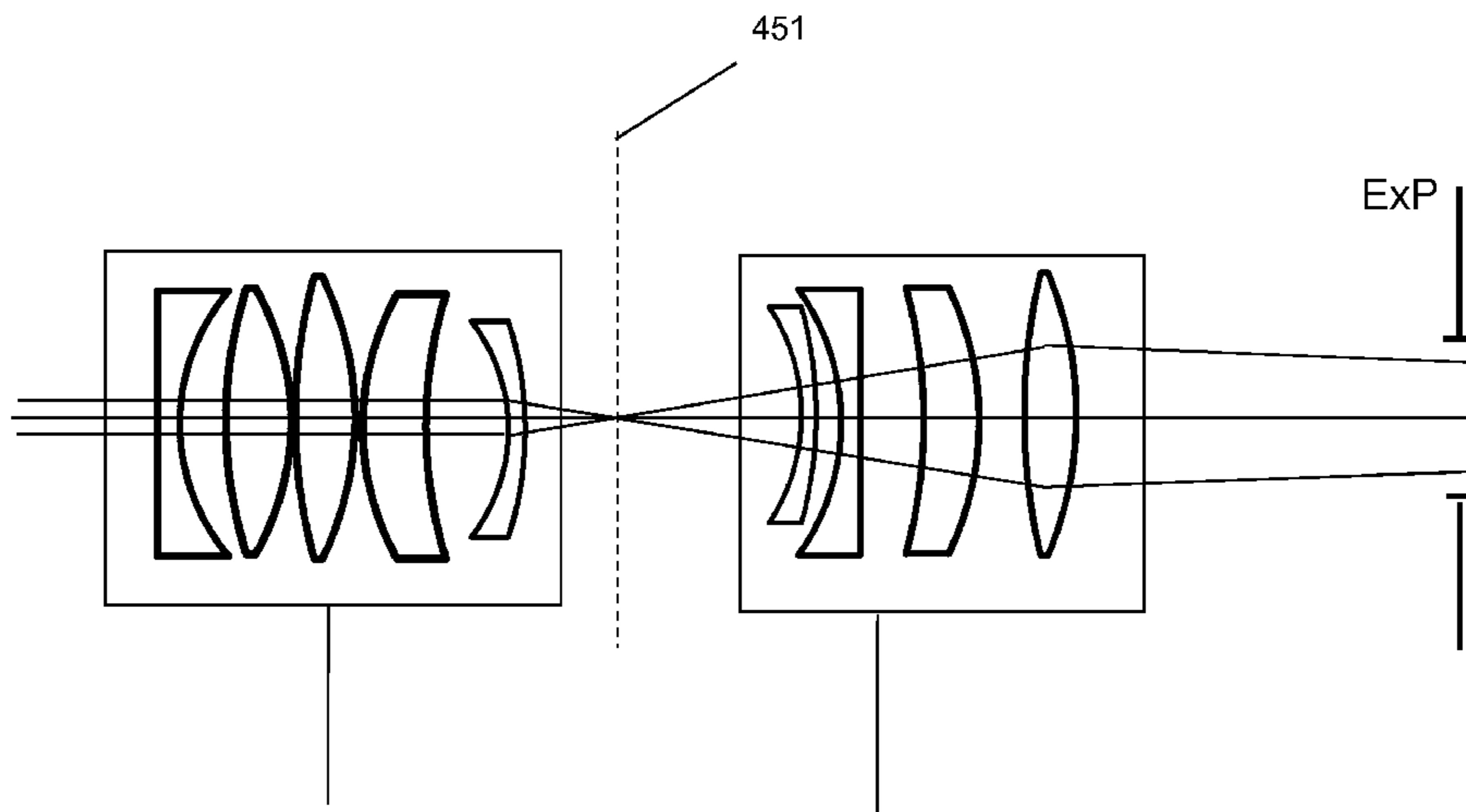
First Beam Expander block 400 Movable Beam Expander block 500
