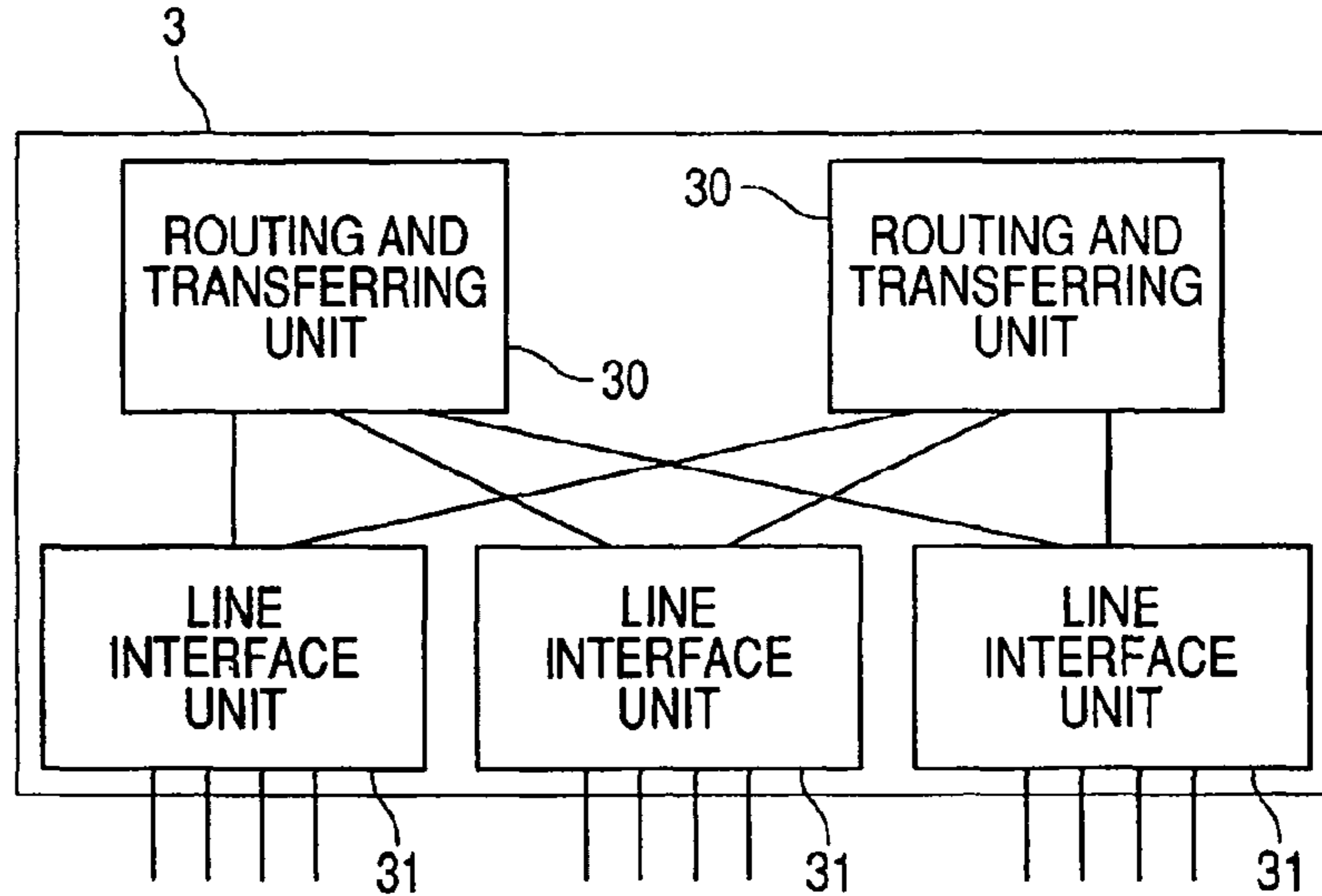
FIG. 5 "DISTRIBUTED" INTEGRATED NETWORK NODE
