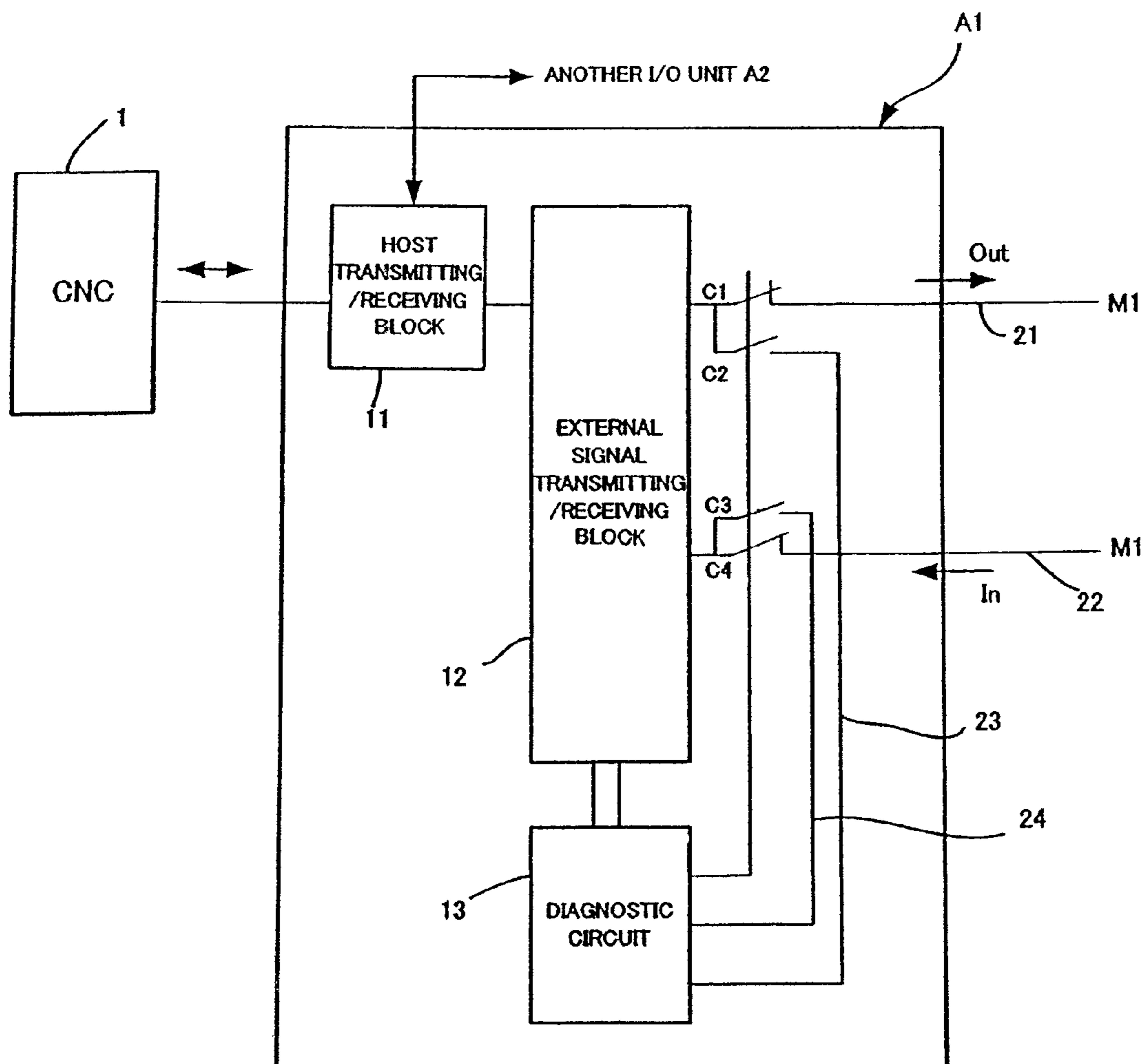
FIG. 2 PRIOR ART
