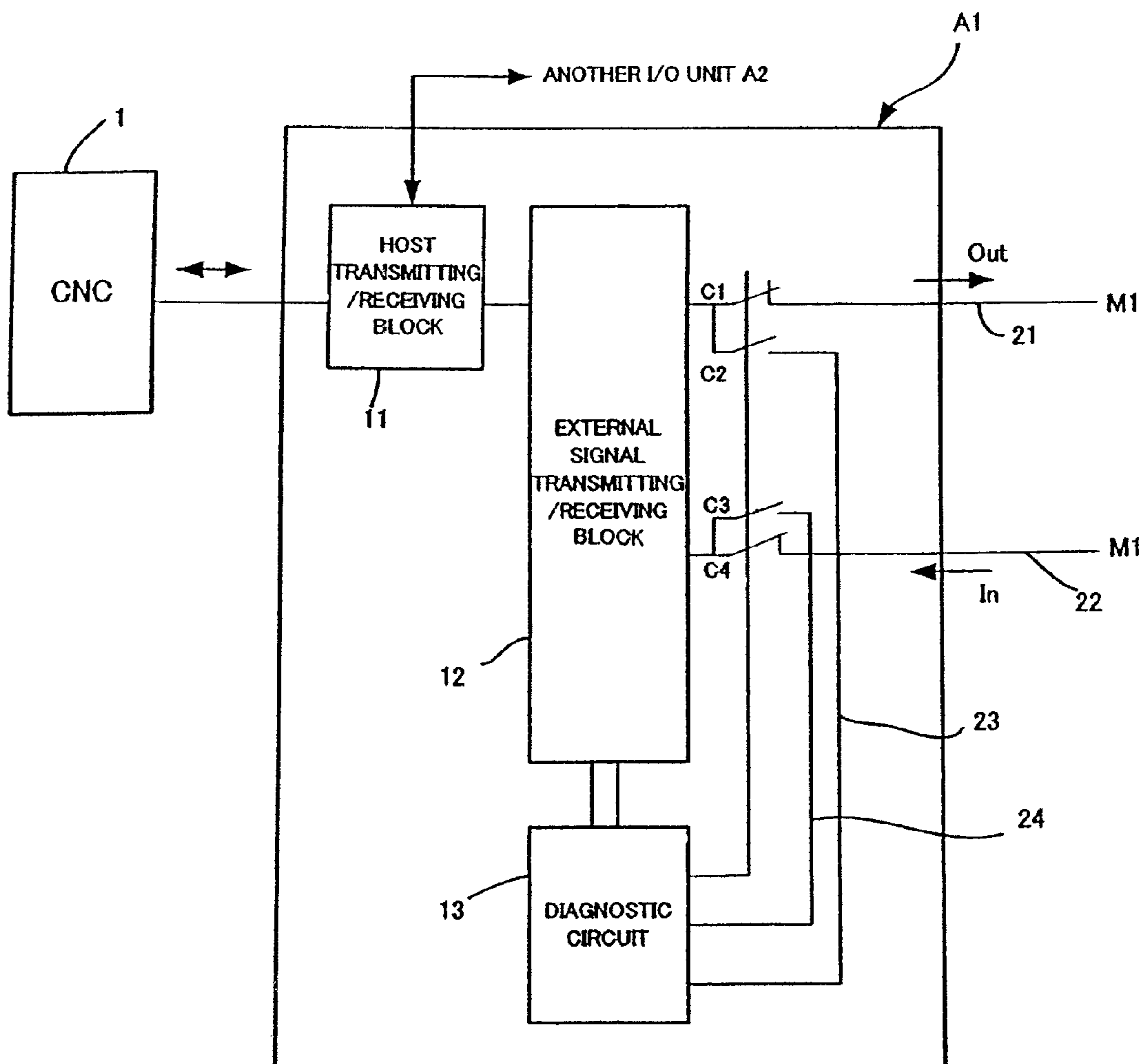
FIG. 2 PRIOR ART
