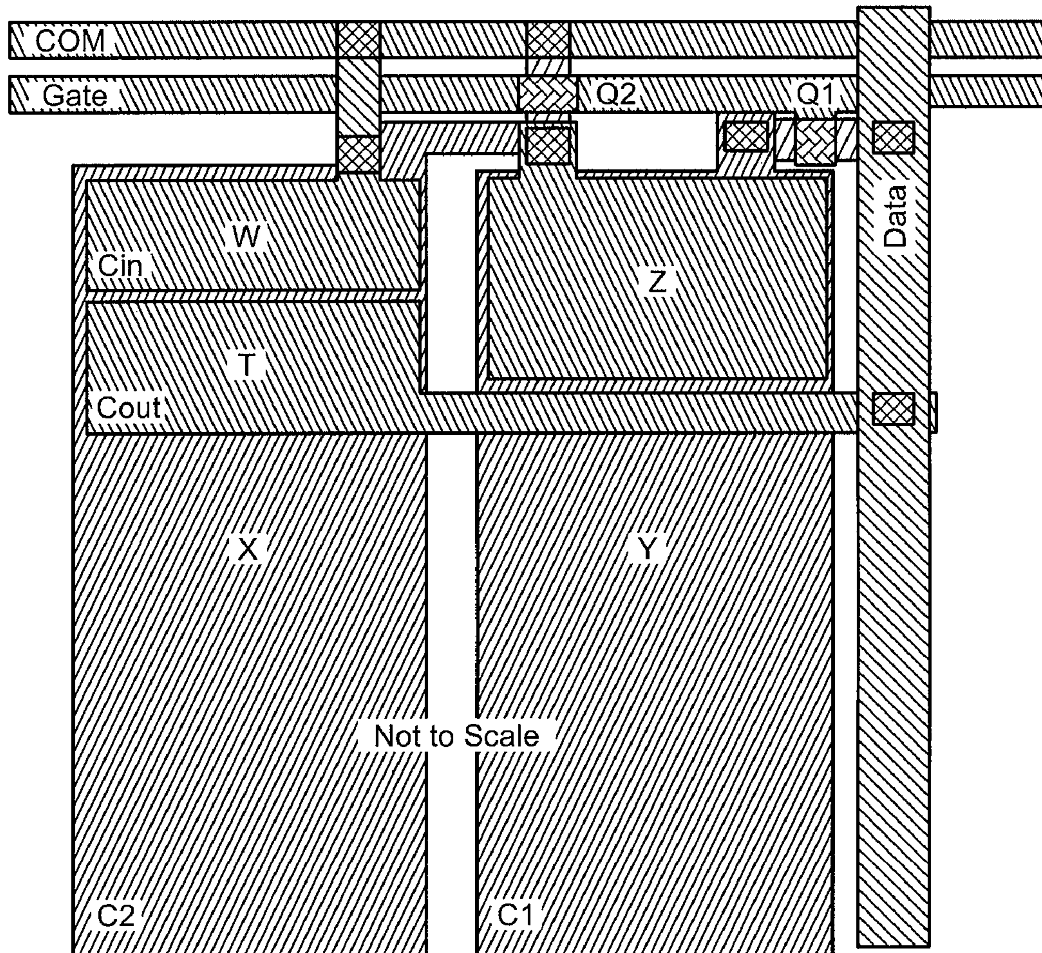
Subpixel Layout
