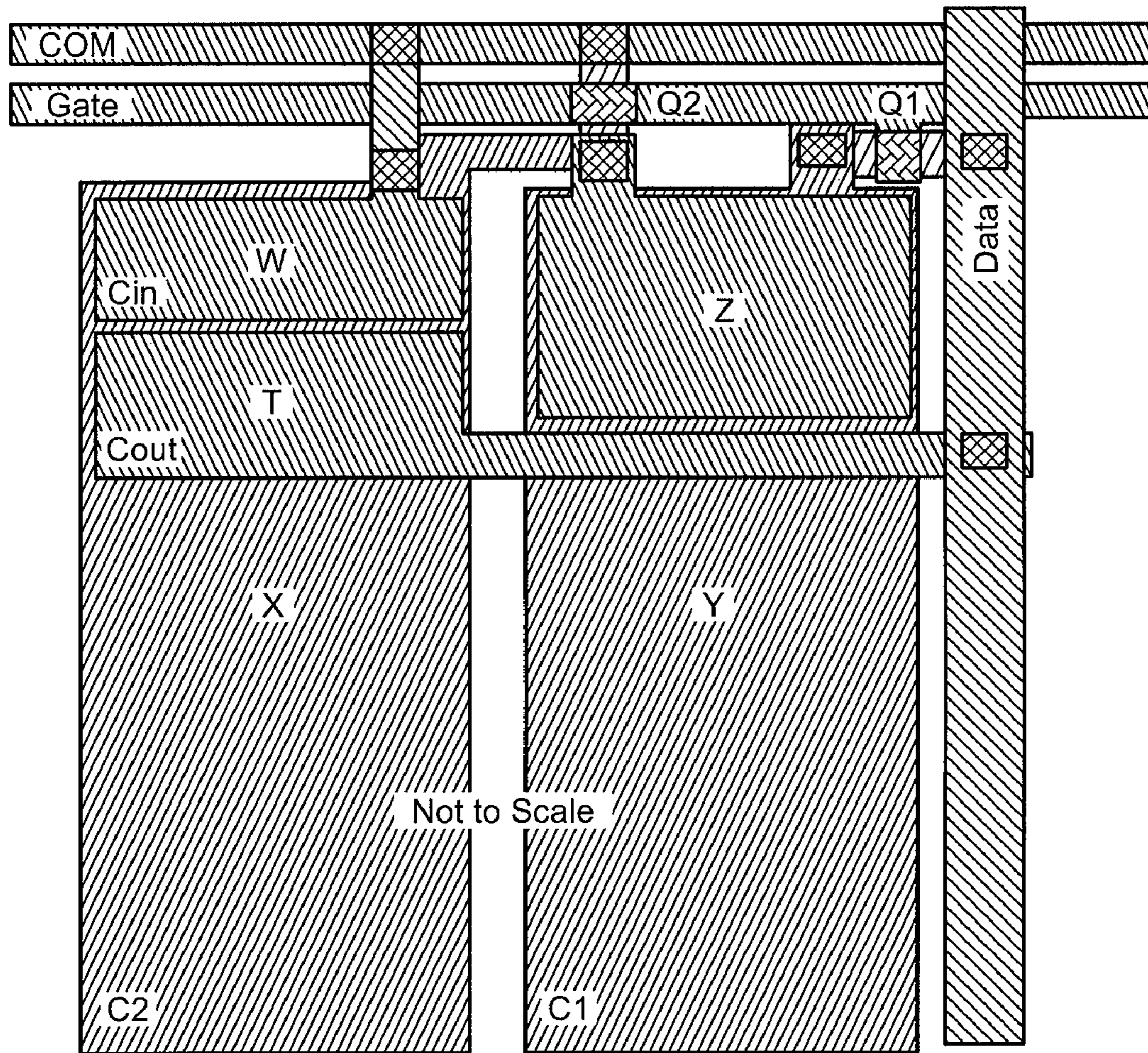
Subpixel Layout
