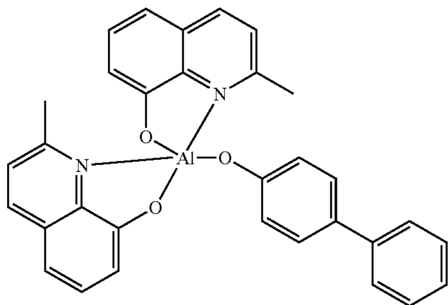
Bis-(2-methyl-8-quinolinolato)-4-(phenyl-phenolato)-aluminium-(III)
