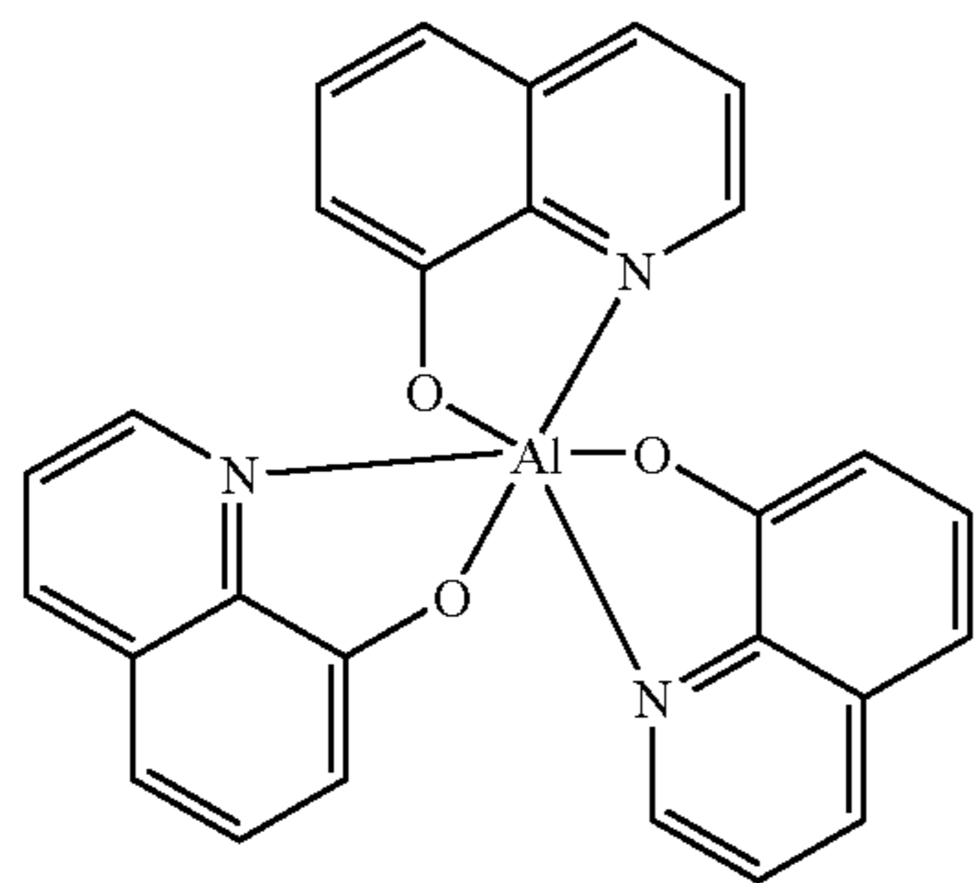
tris (8-hydroxy-quinolinato)-aluminium
