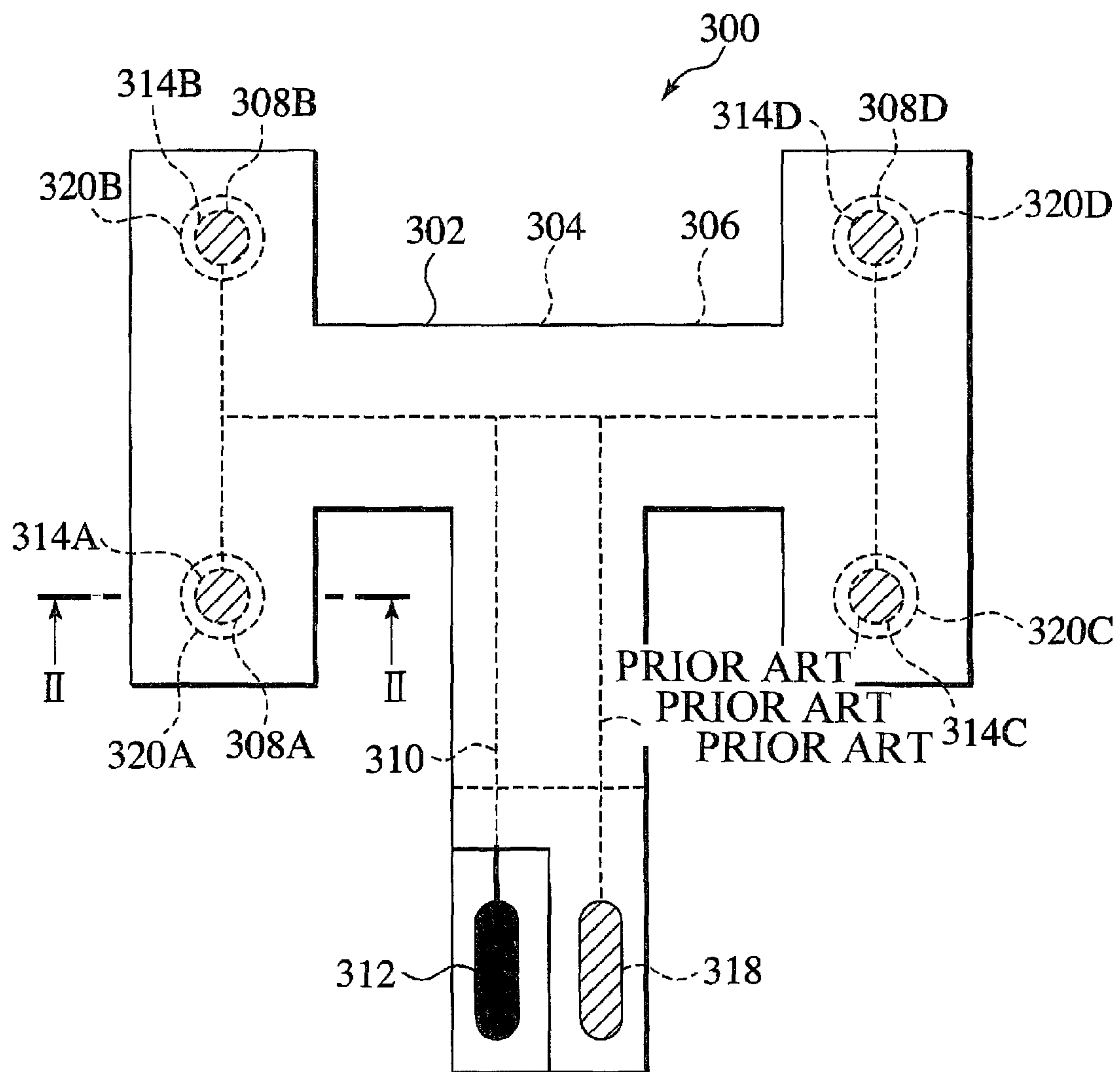
FIG. 1 PRIOR ART
