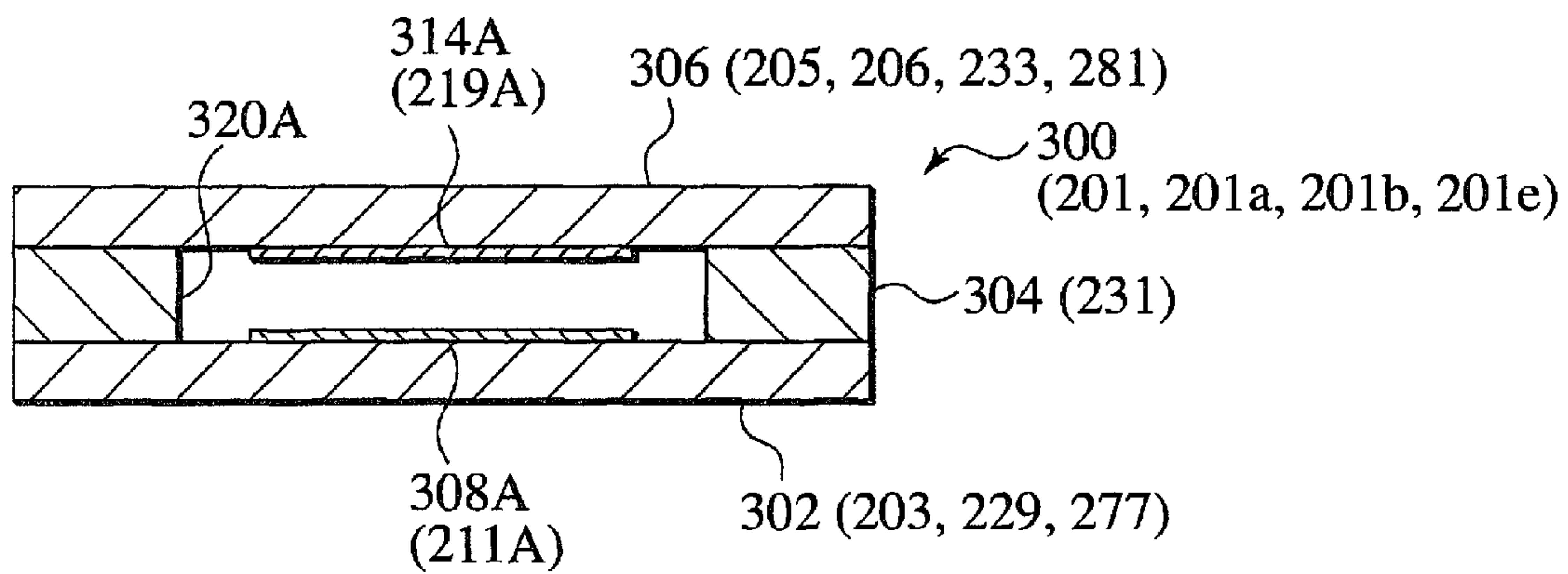
FIG.2 PRIOR ART
