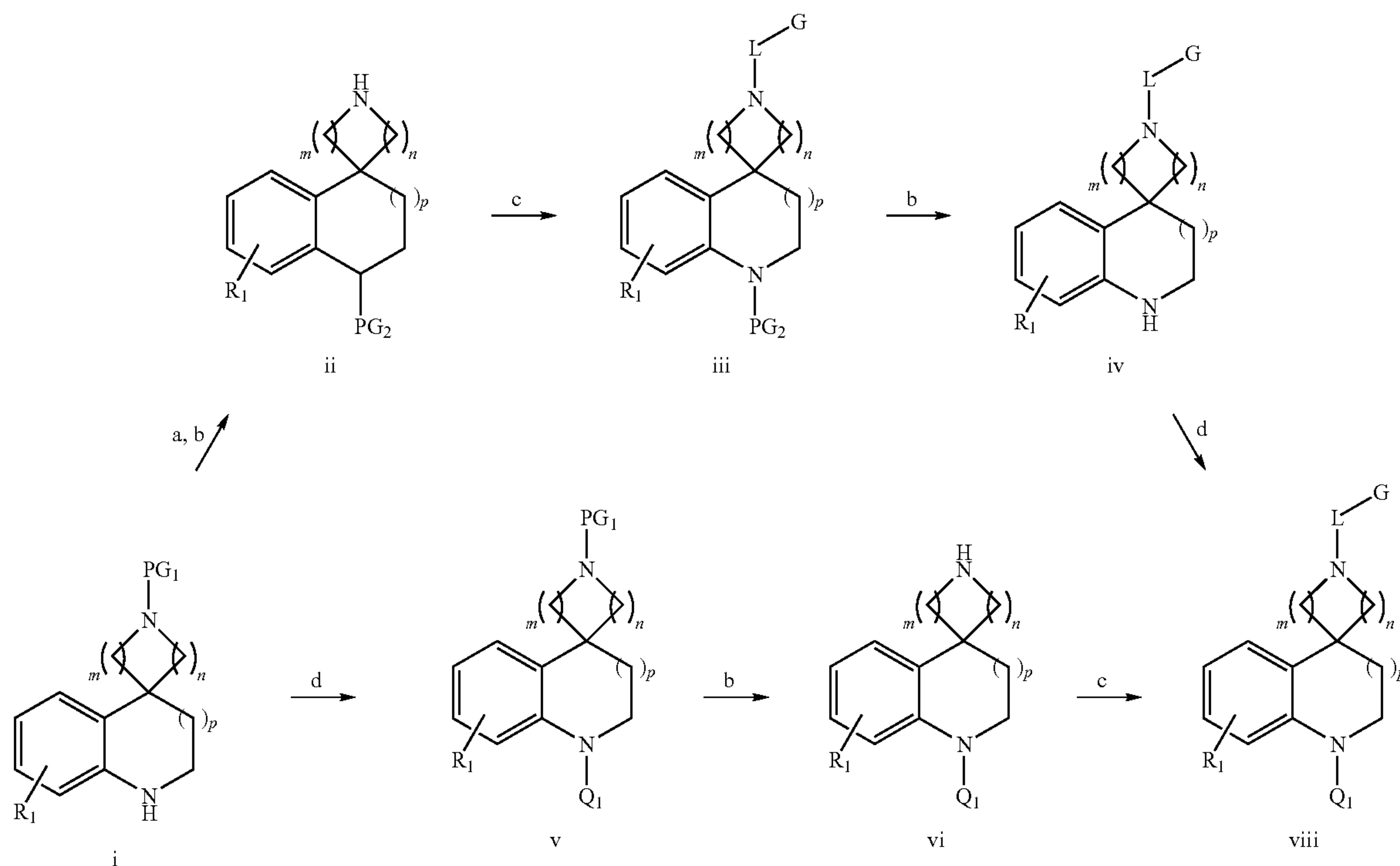
Scheme 4:
