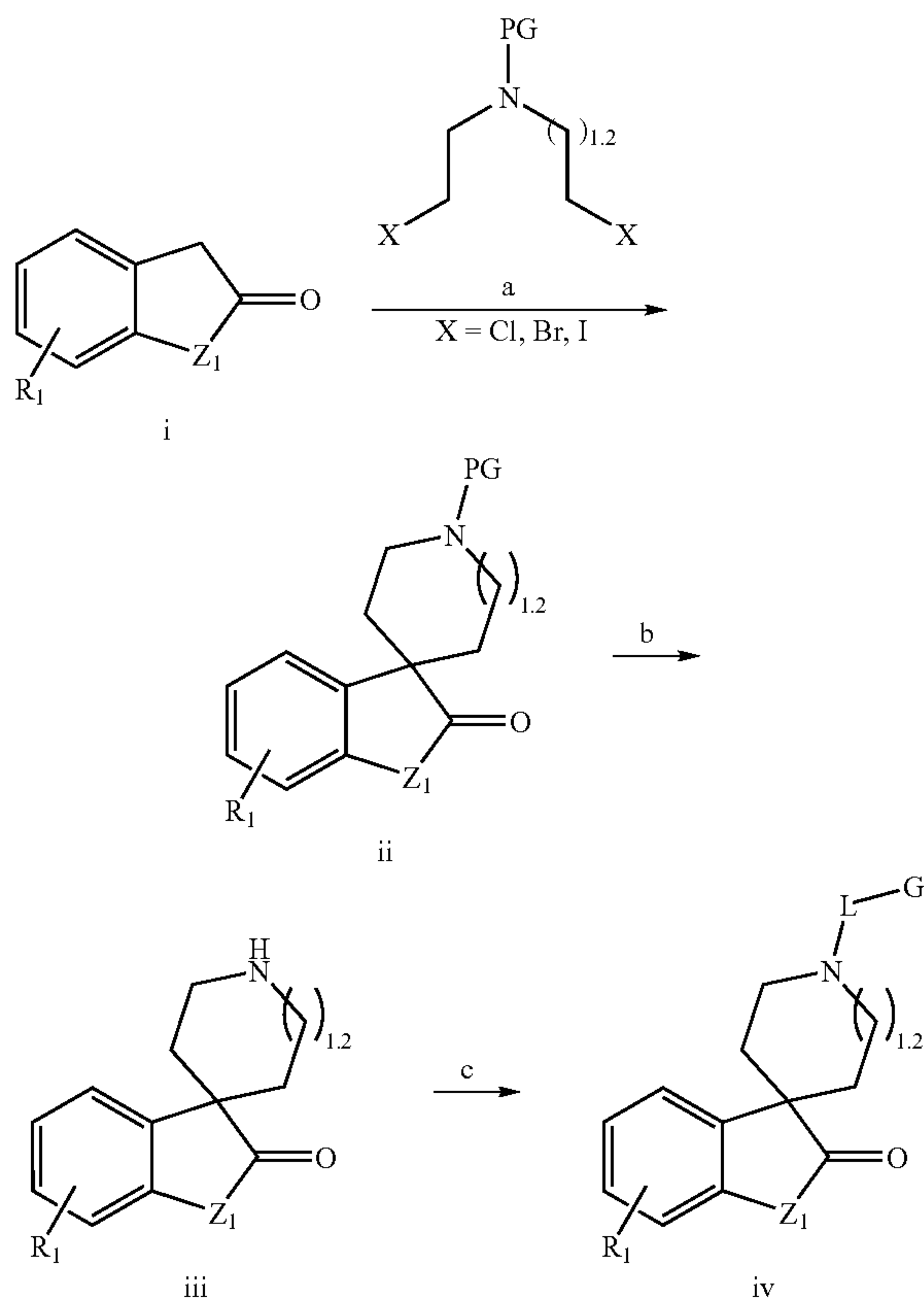
Scheme 9:
