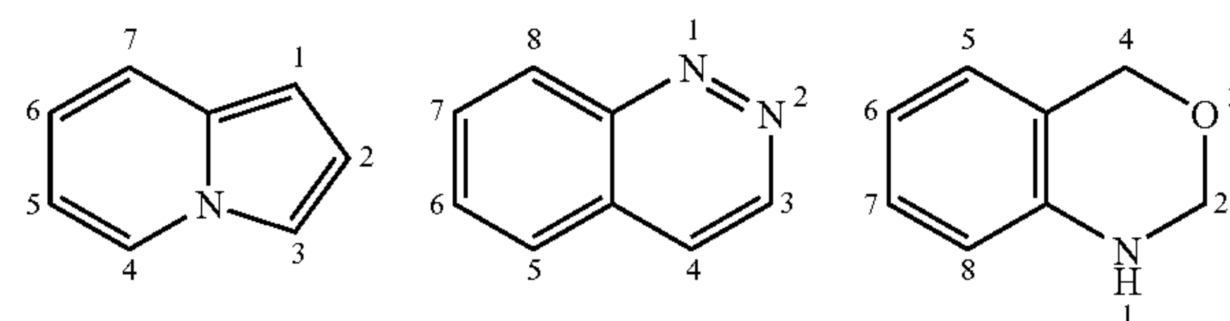
Indolizine
