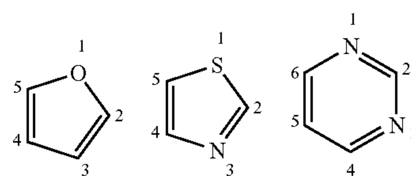
Furan
