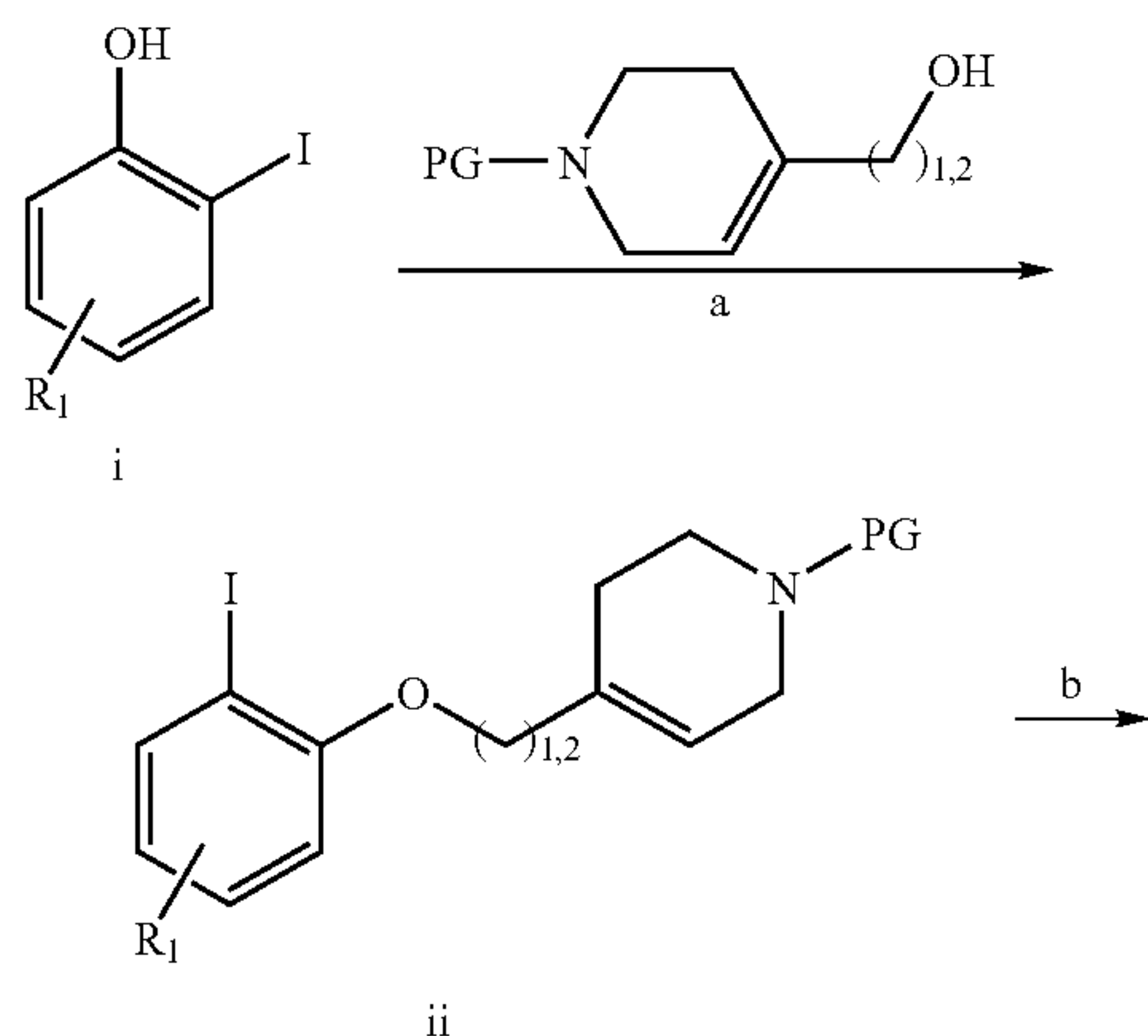
Scheme 3:
