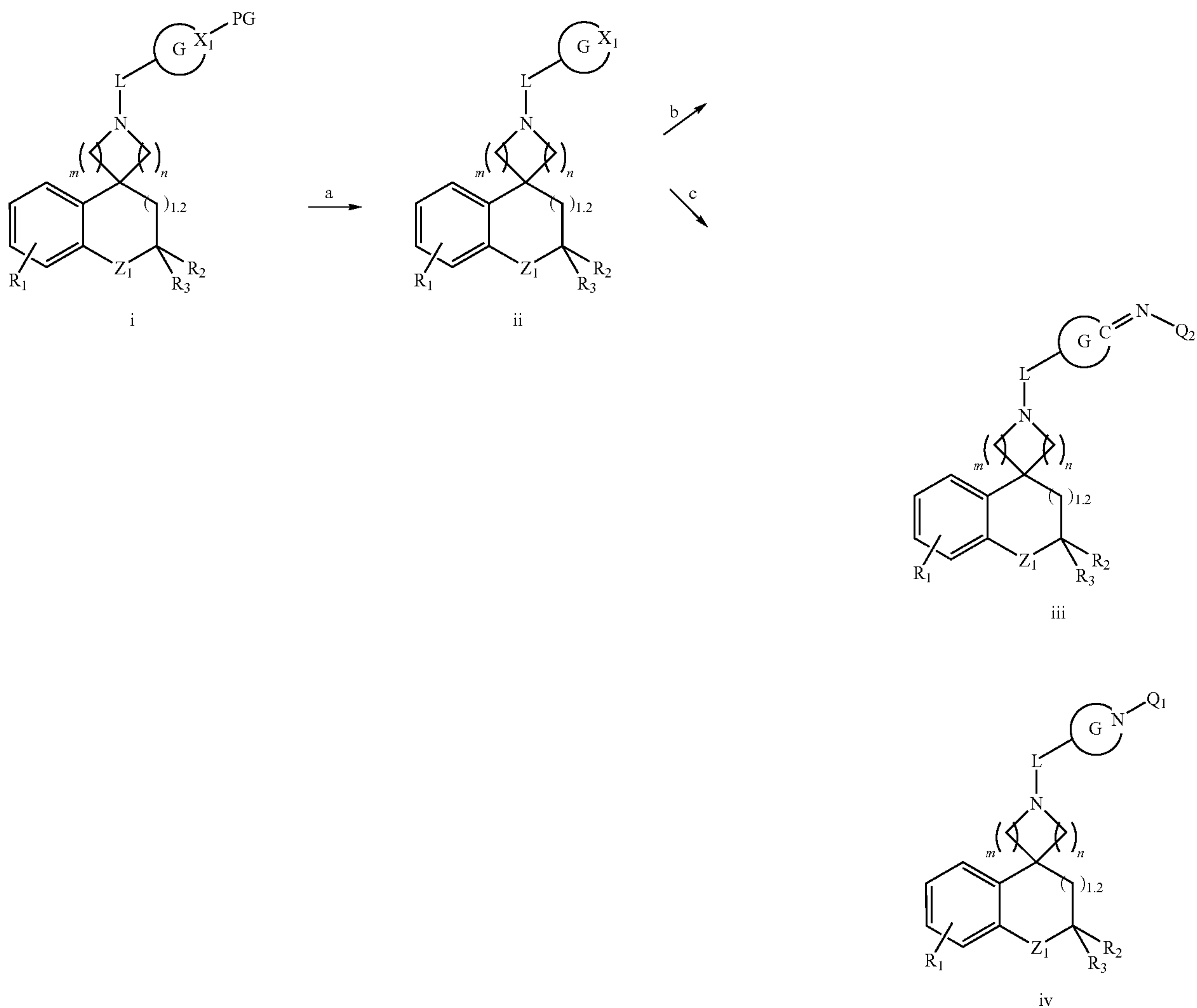
Scheme 8:
