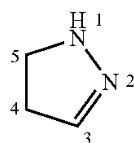
2-Pyrazoline
