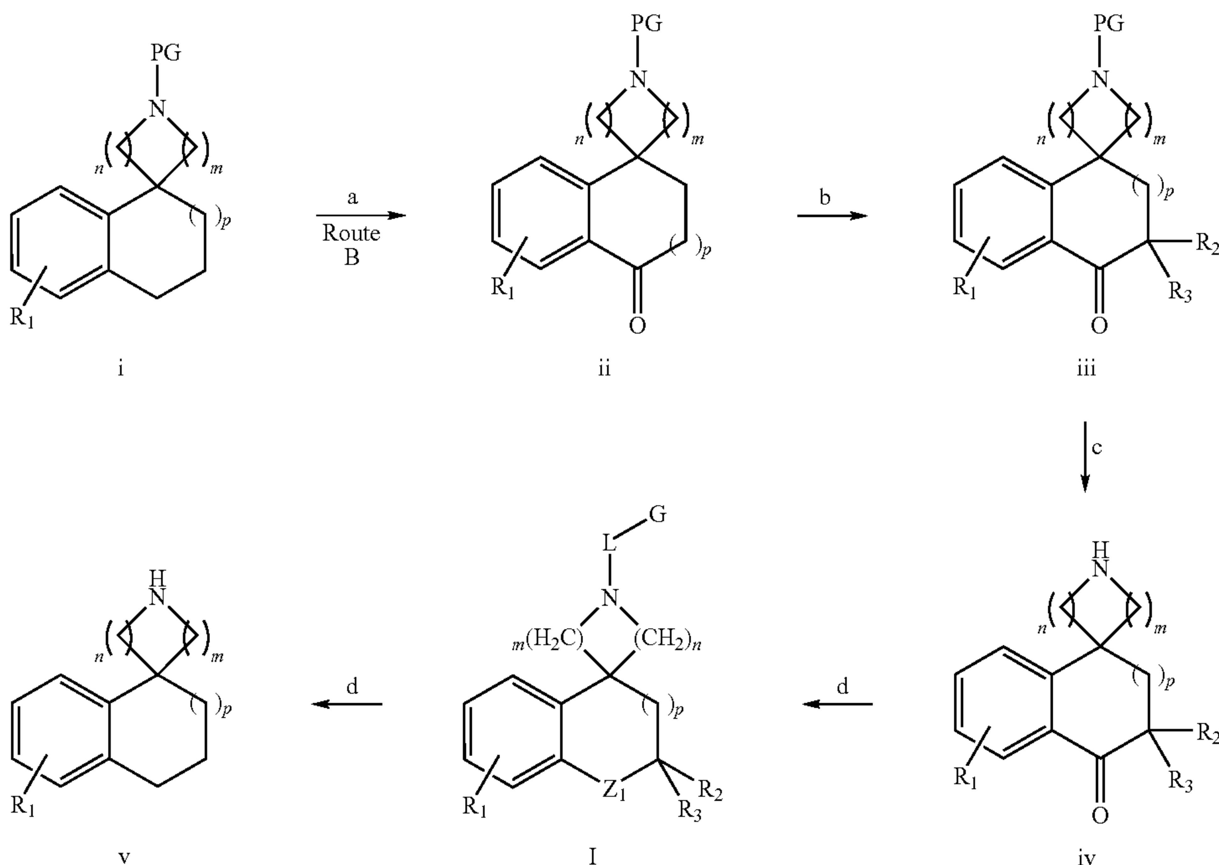
Scheme 2:
