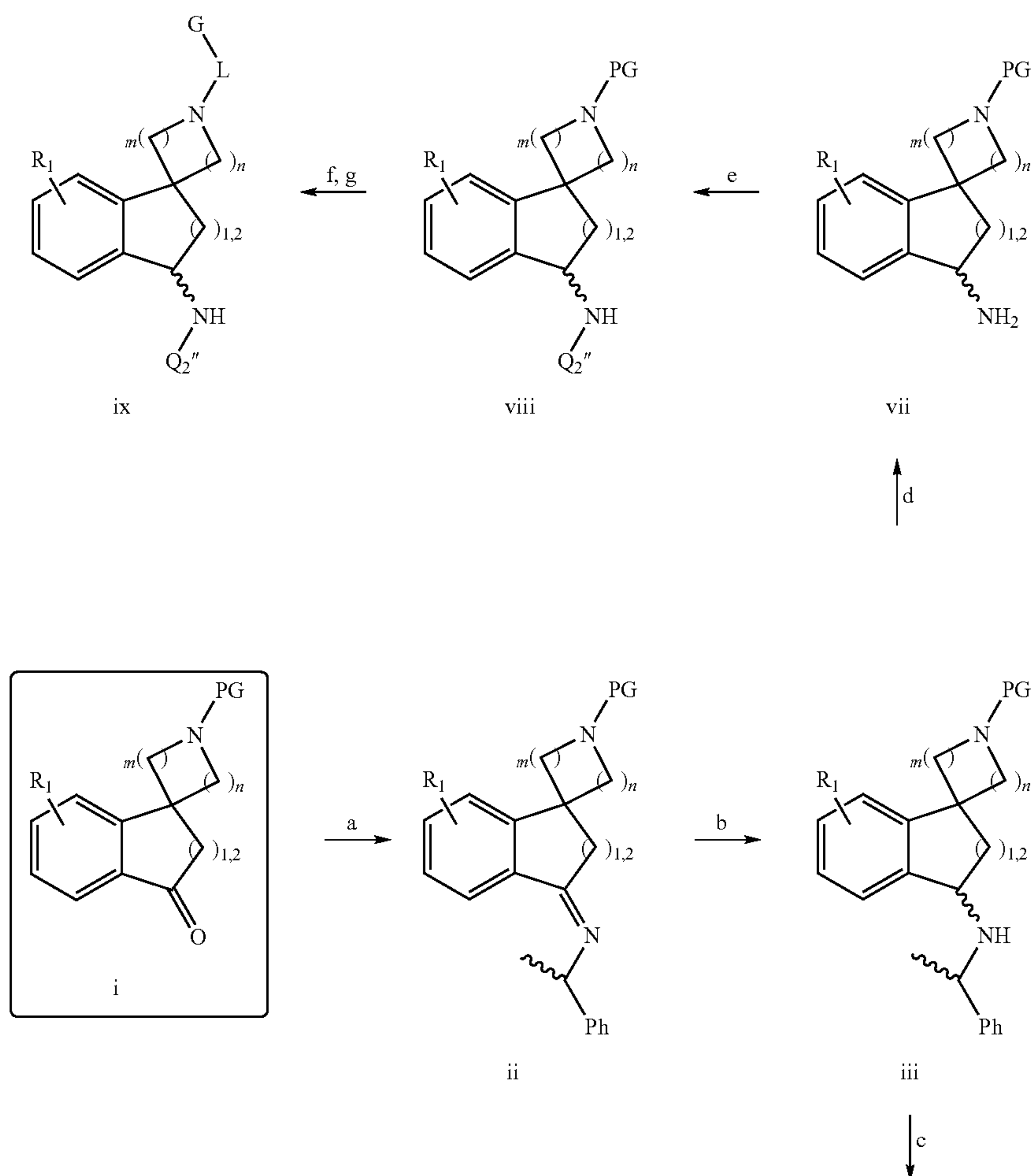
Scheme 7:
