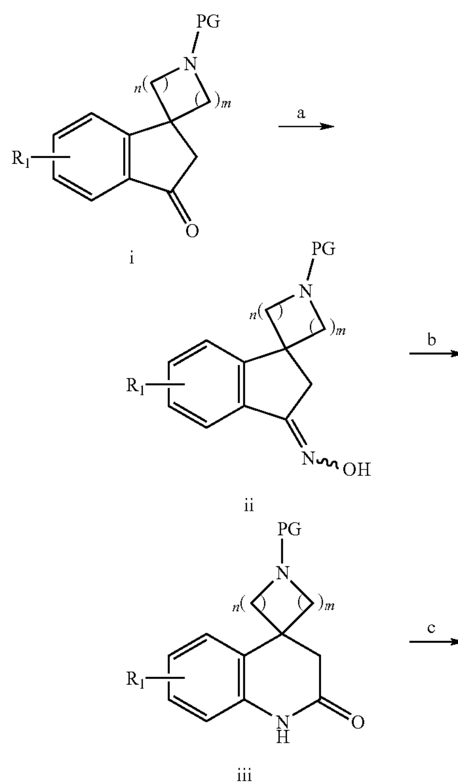
Scheme 6:
