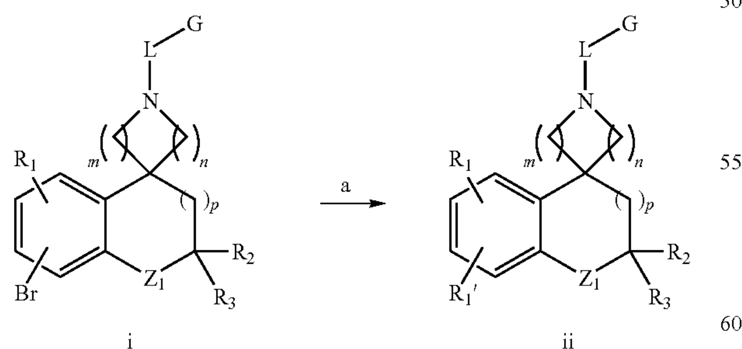
Scheme 5:
