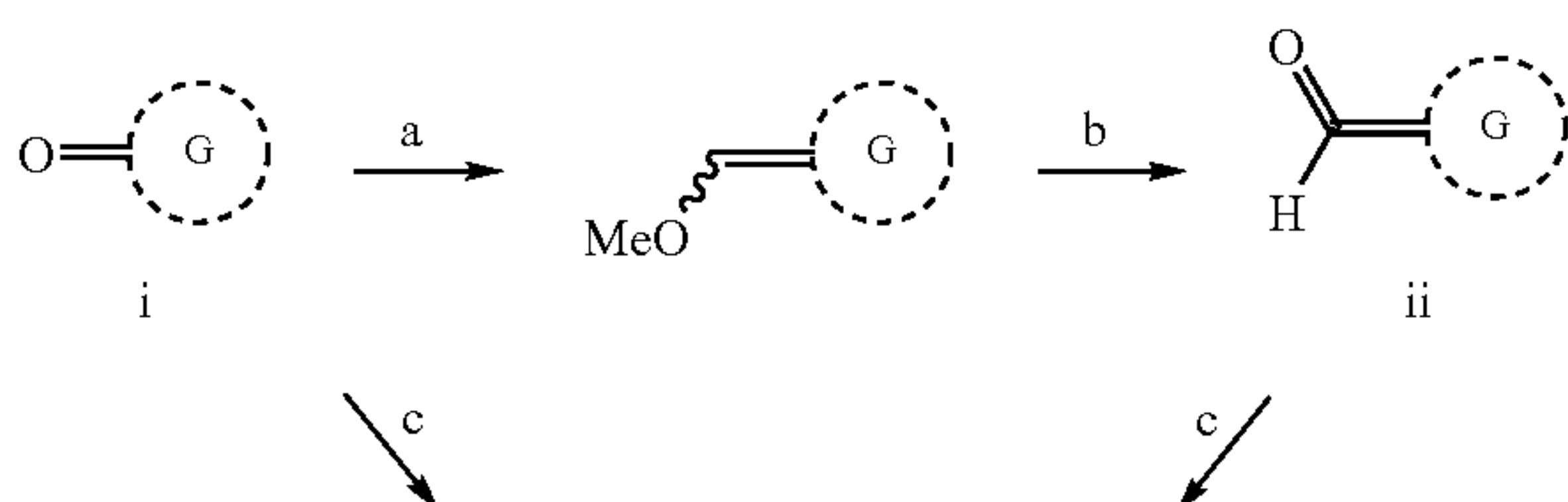
Scheme 10:
