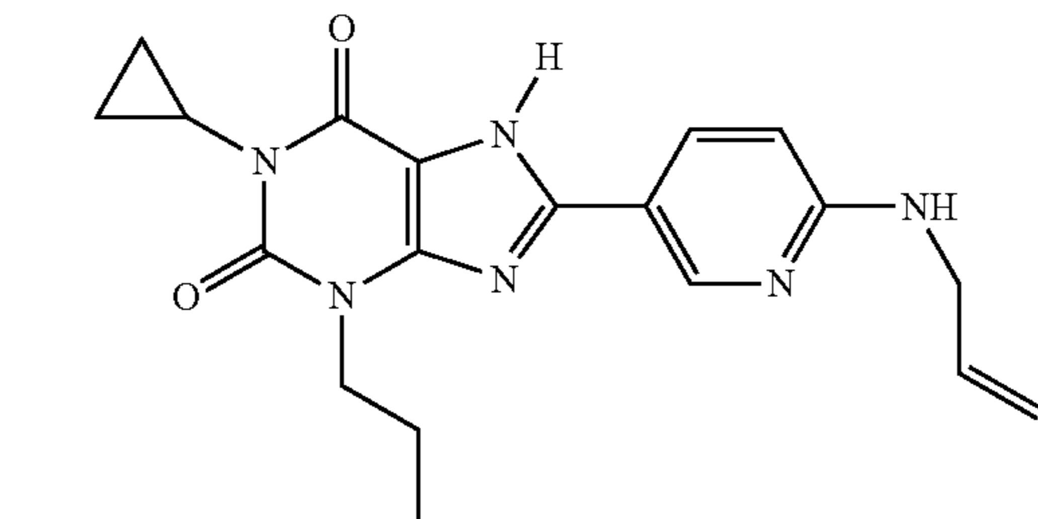
1B: 1-Cyclopropyl-3-propyl-8-[6-methylamino-3-pyridyl]xanthine
