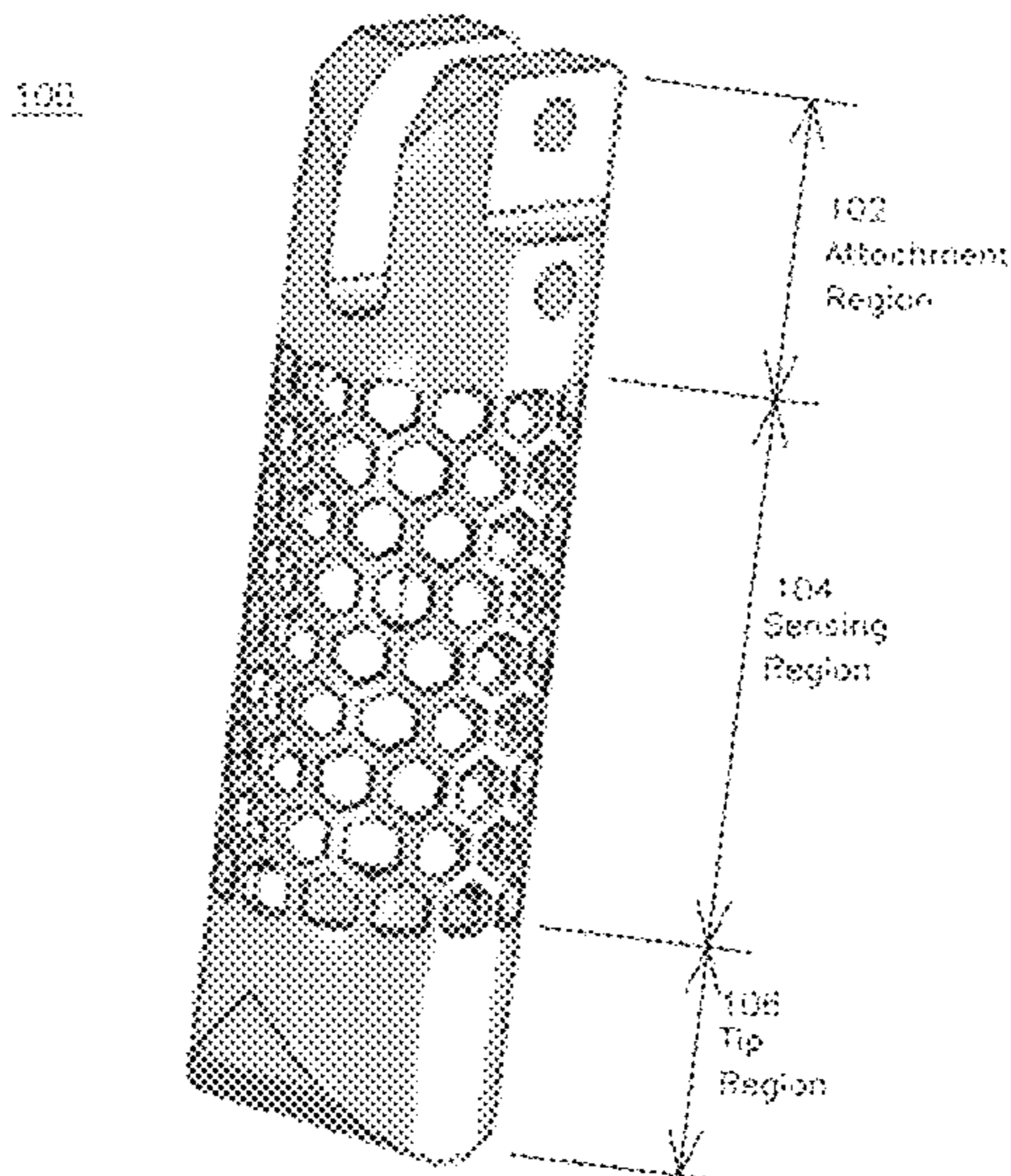
Sensor with elastomeric shell
