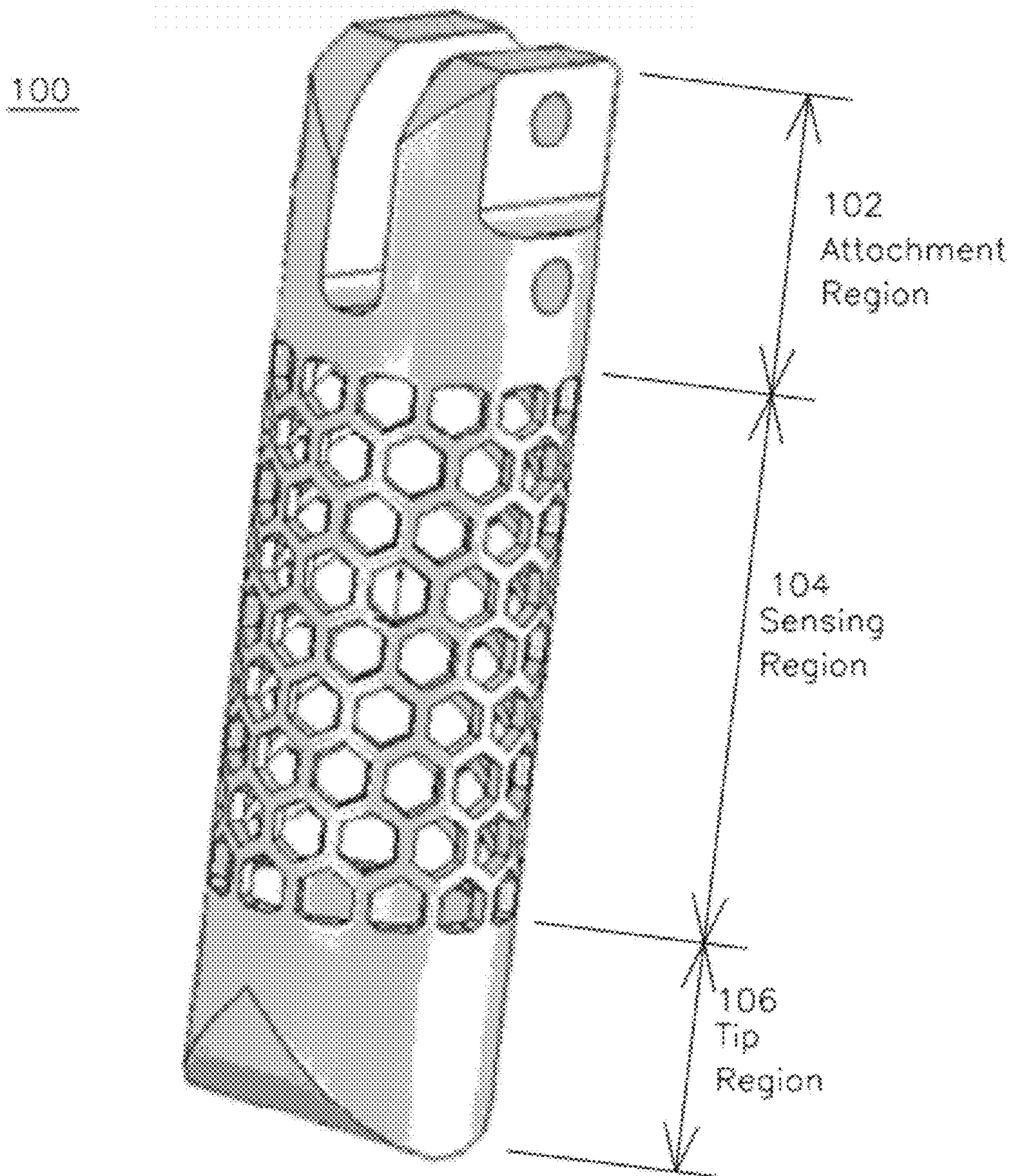
Figure 1 Sensor with elastomeric shell
