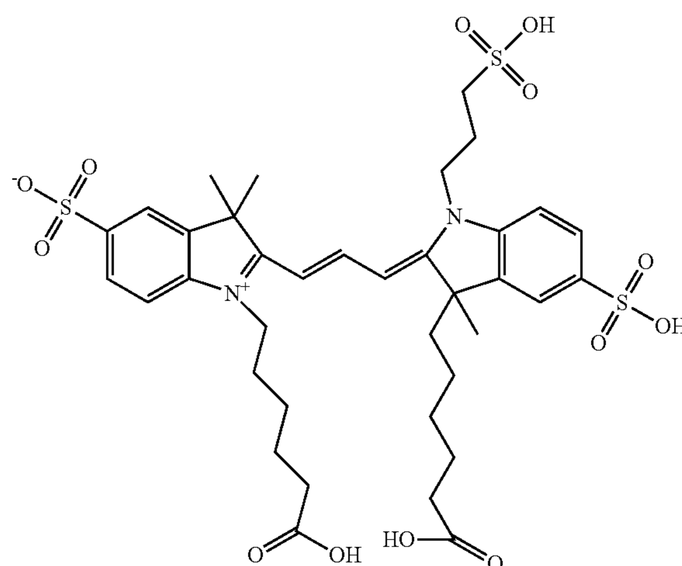
Compound 18
