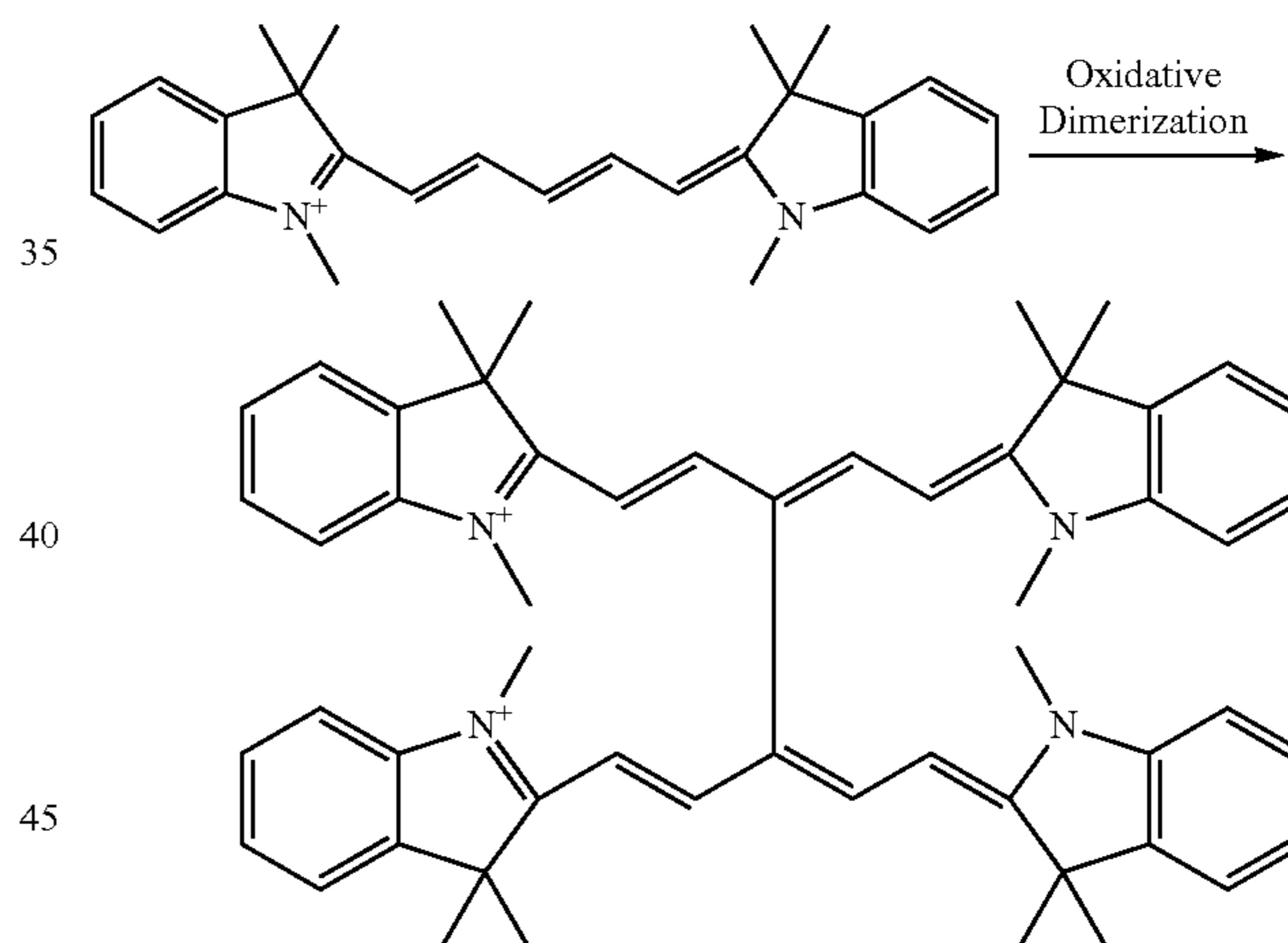
Scheme 2. Oxidative dimerization of carbocyanines
