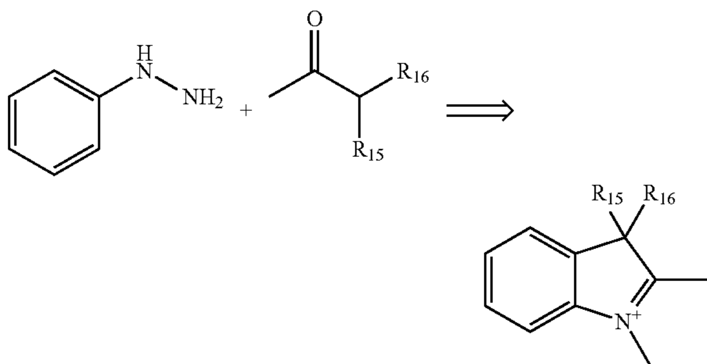
Scheme 3. Typical synthesis of indolium intermediate
