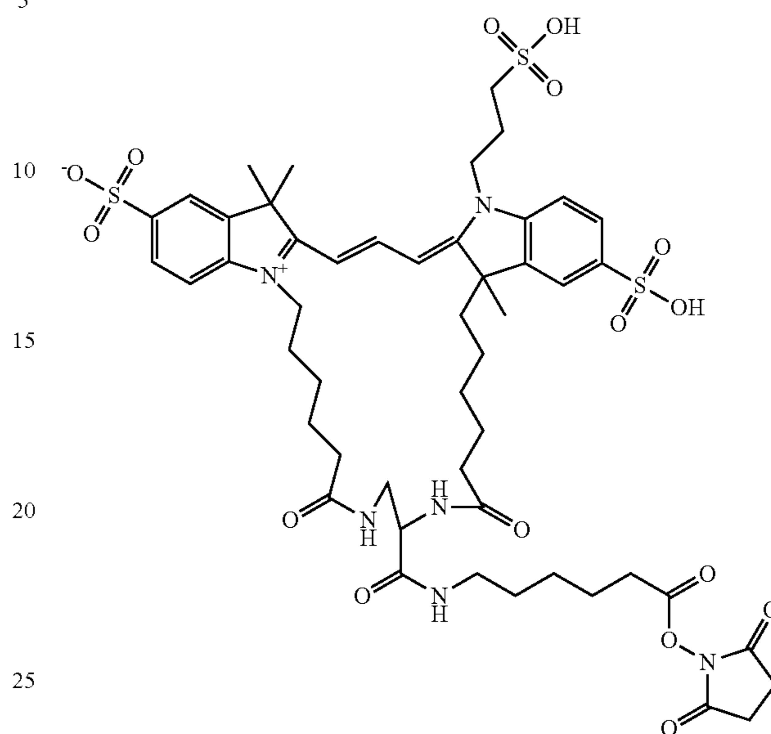
Compound 20
