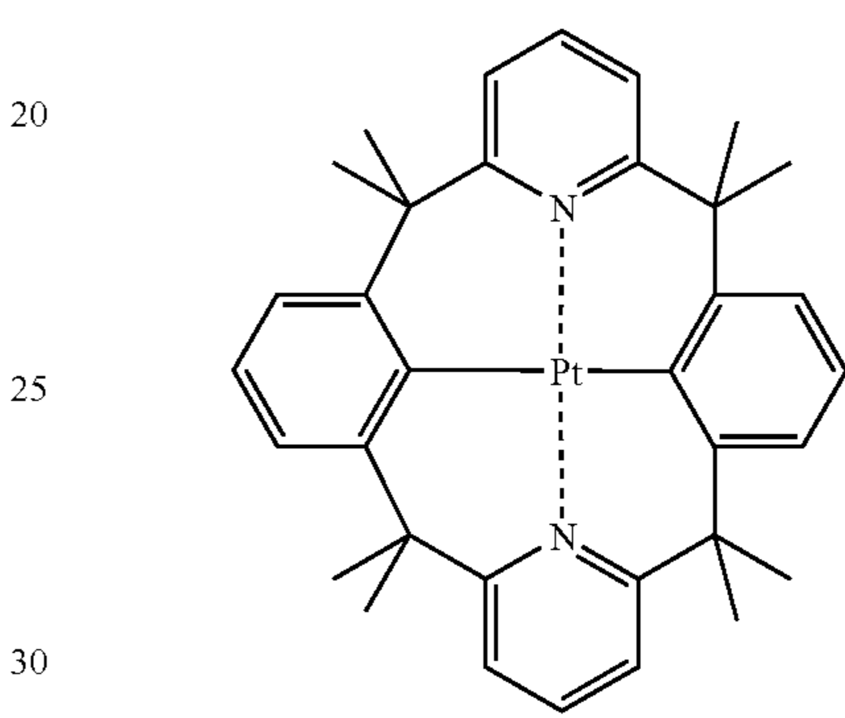
Compound (121)
