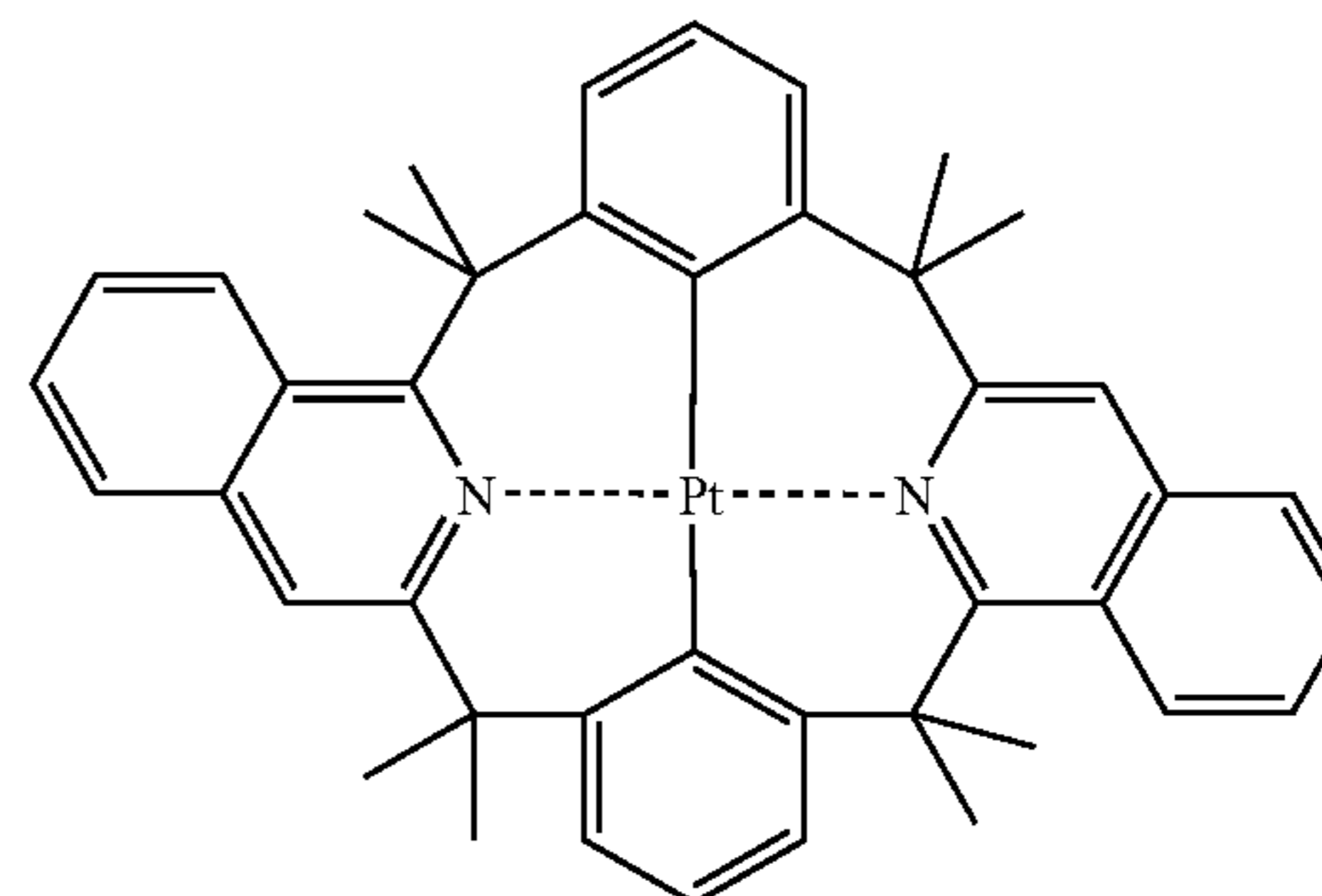
Compound (148)
