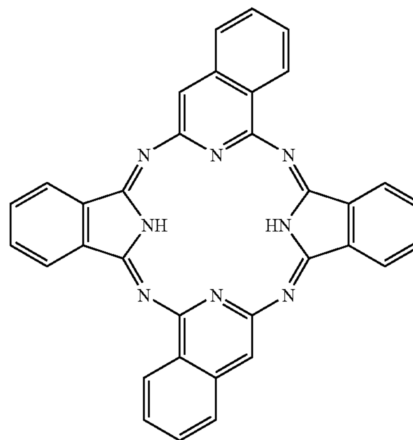
Compound (35)
