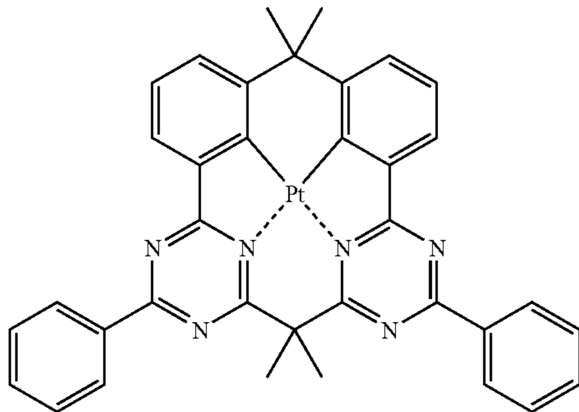
Compound (110)
