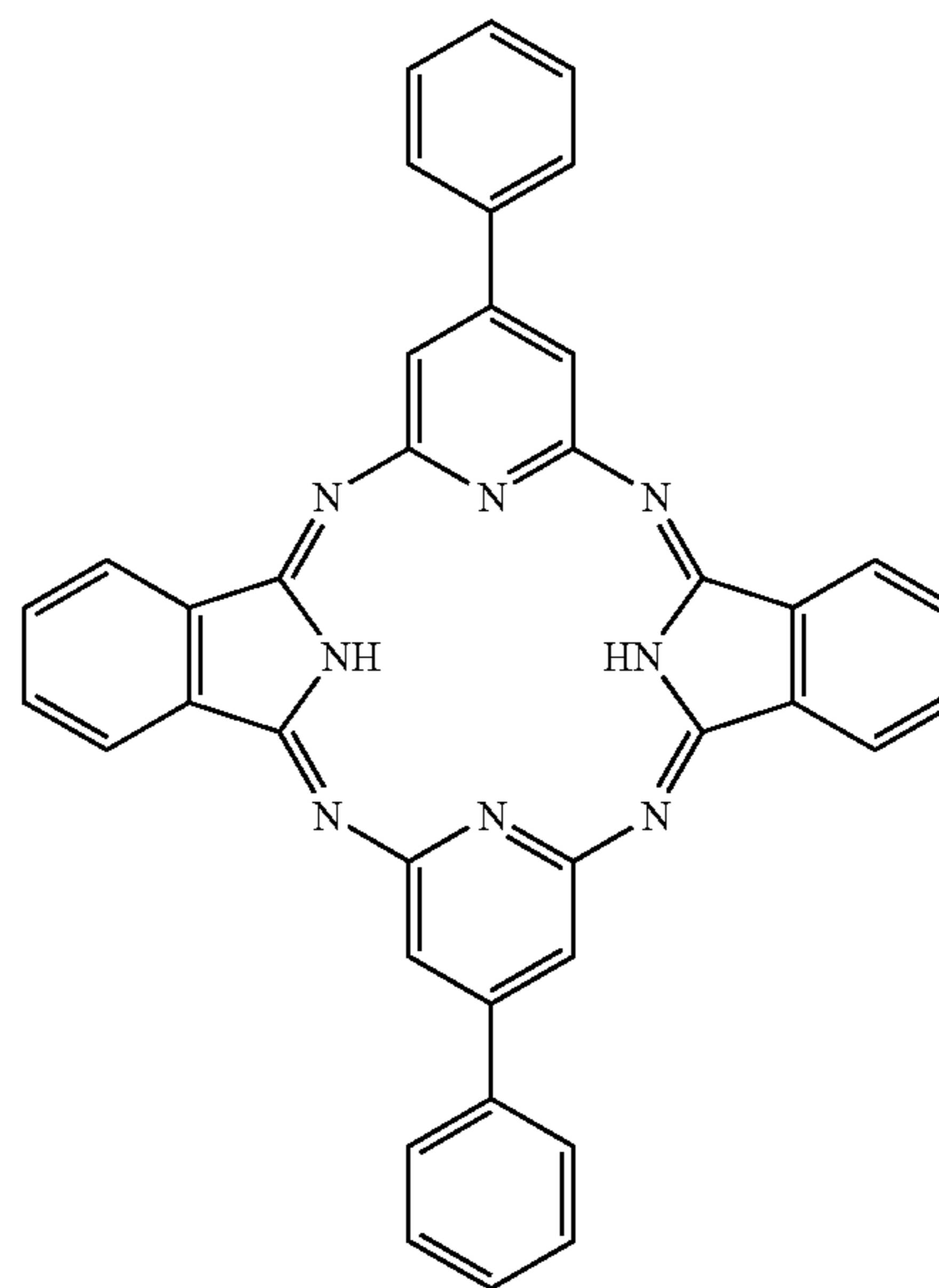
Compound (34)
