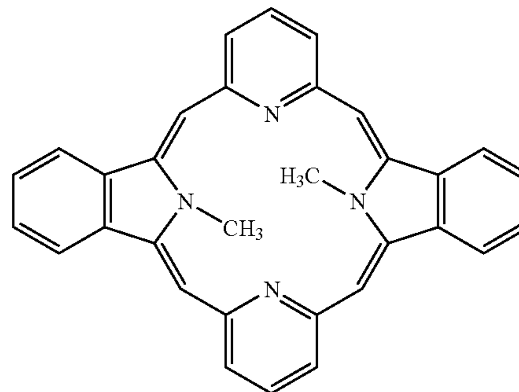
Compound (57)
