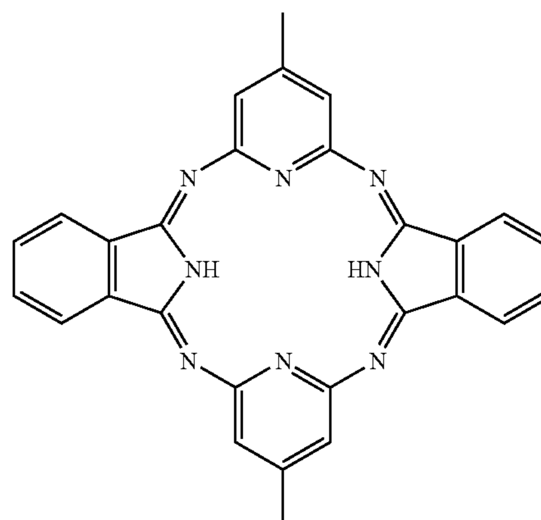
Compound (33)
