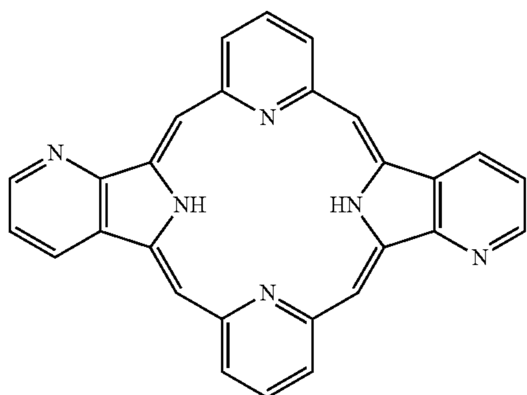
Compound (23)
