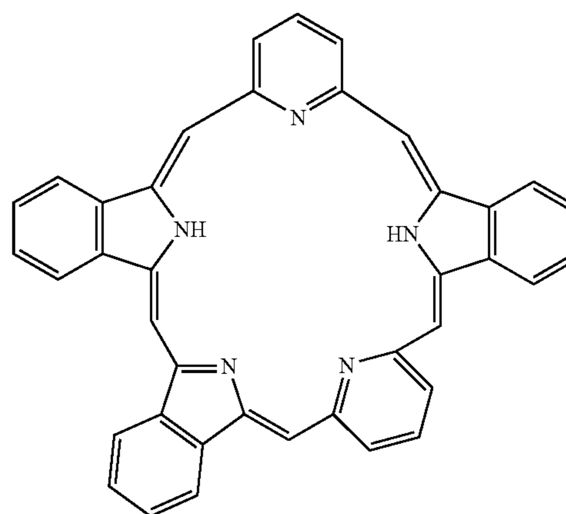
Compound (40)
