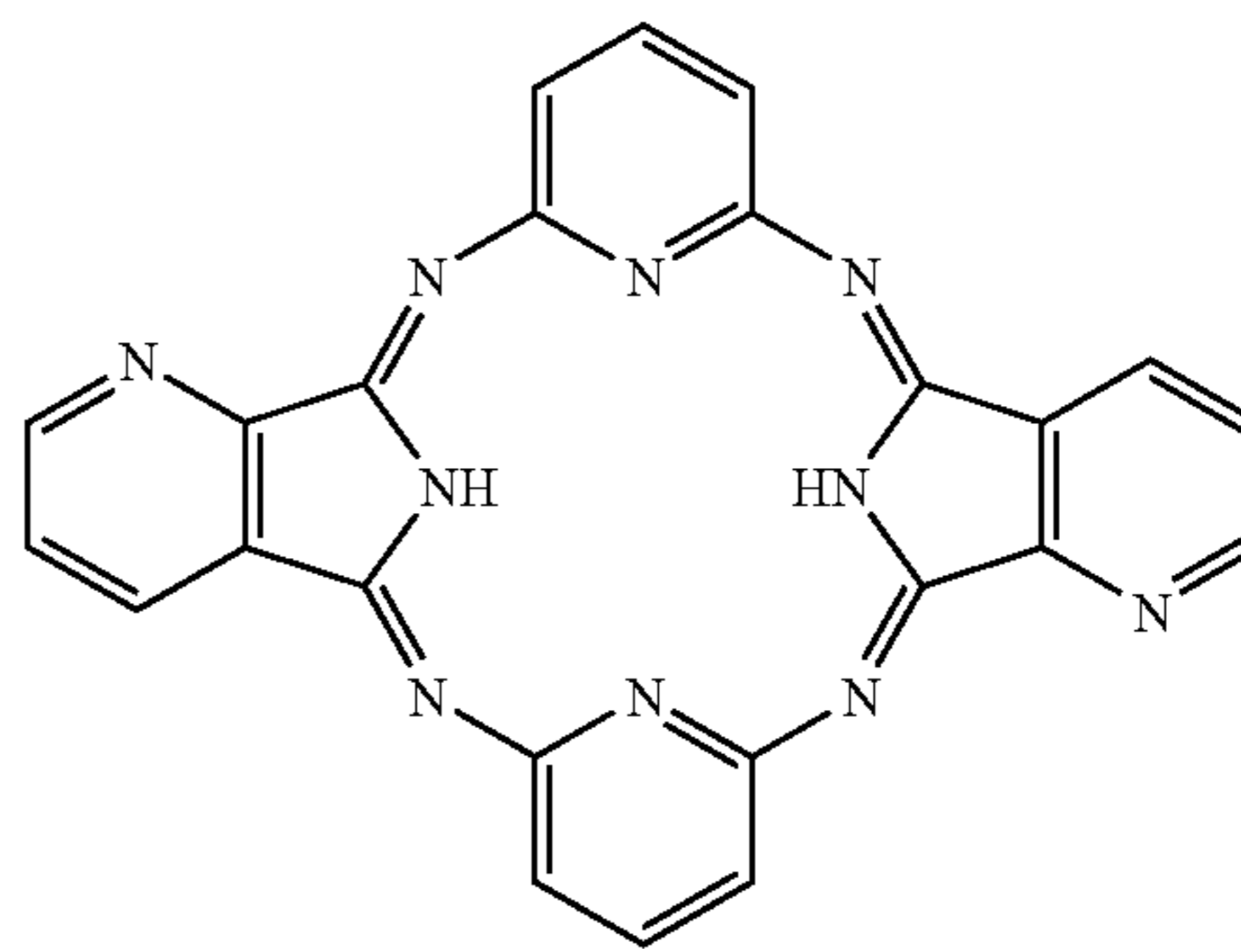
Compound (12)
