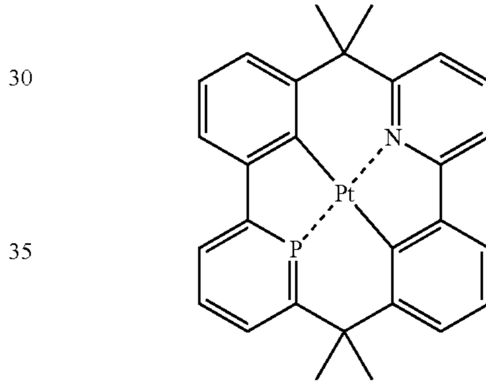
Compound (111)
