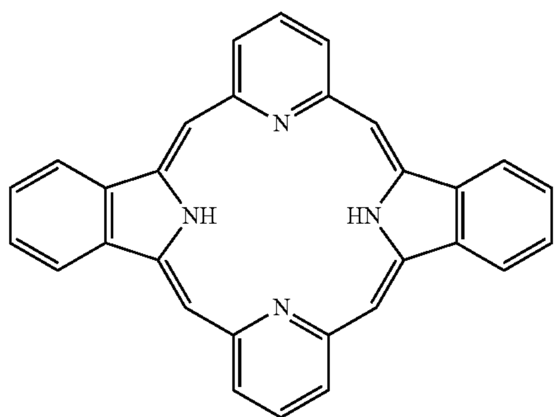
Compound (21)
