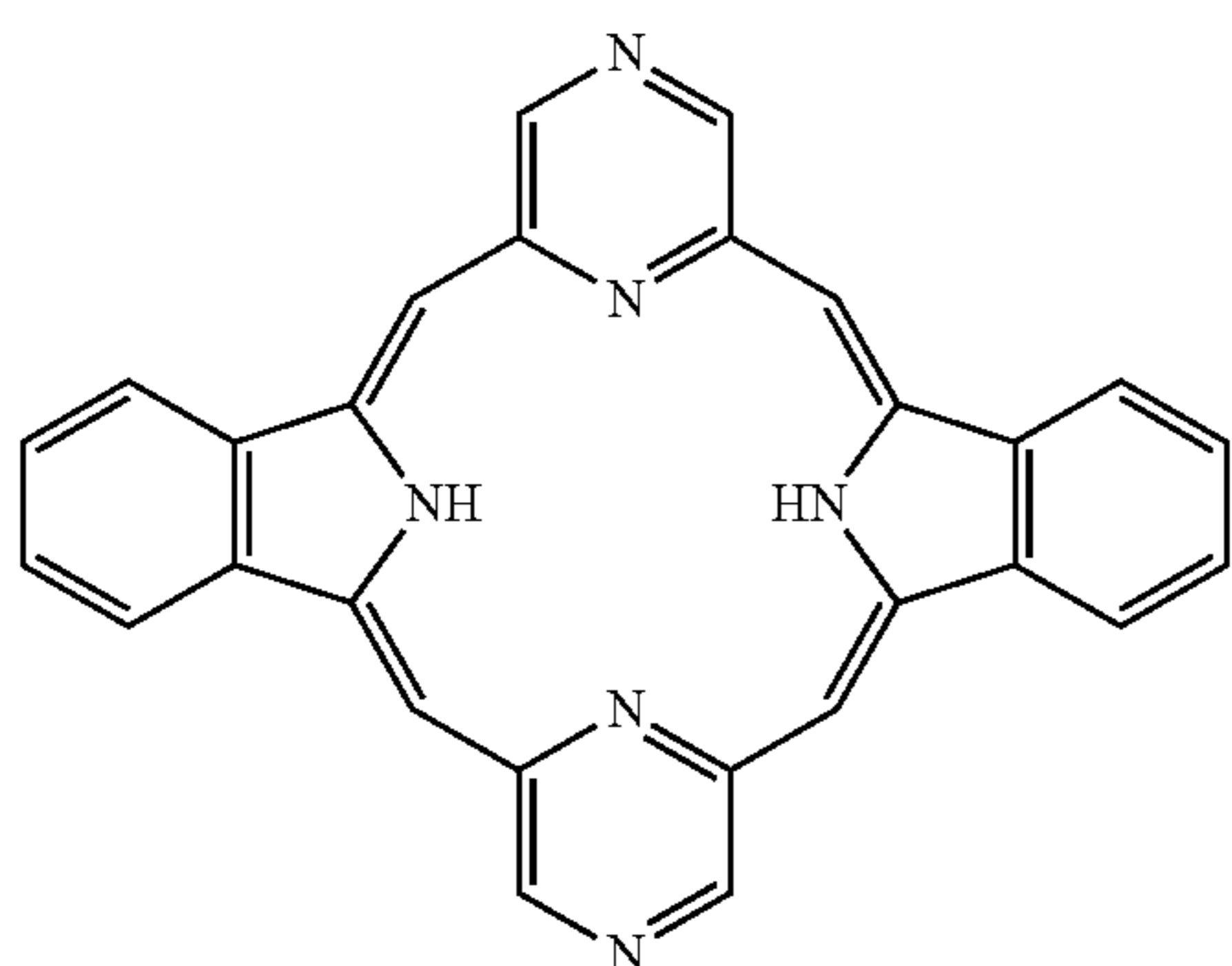
Compound (23)
