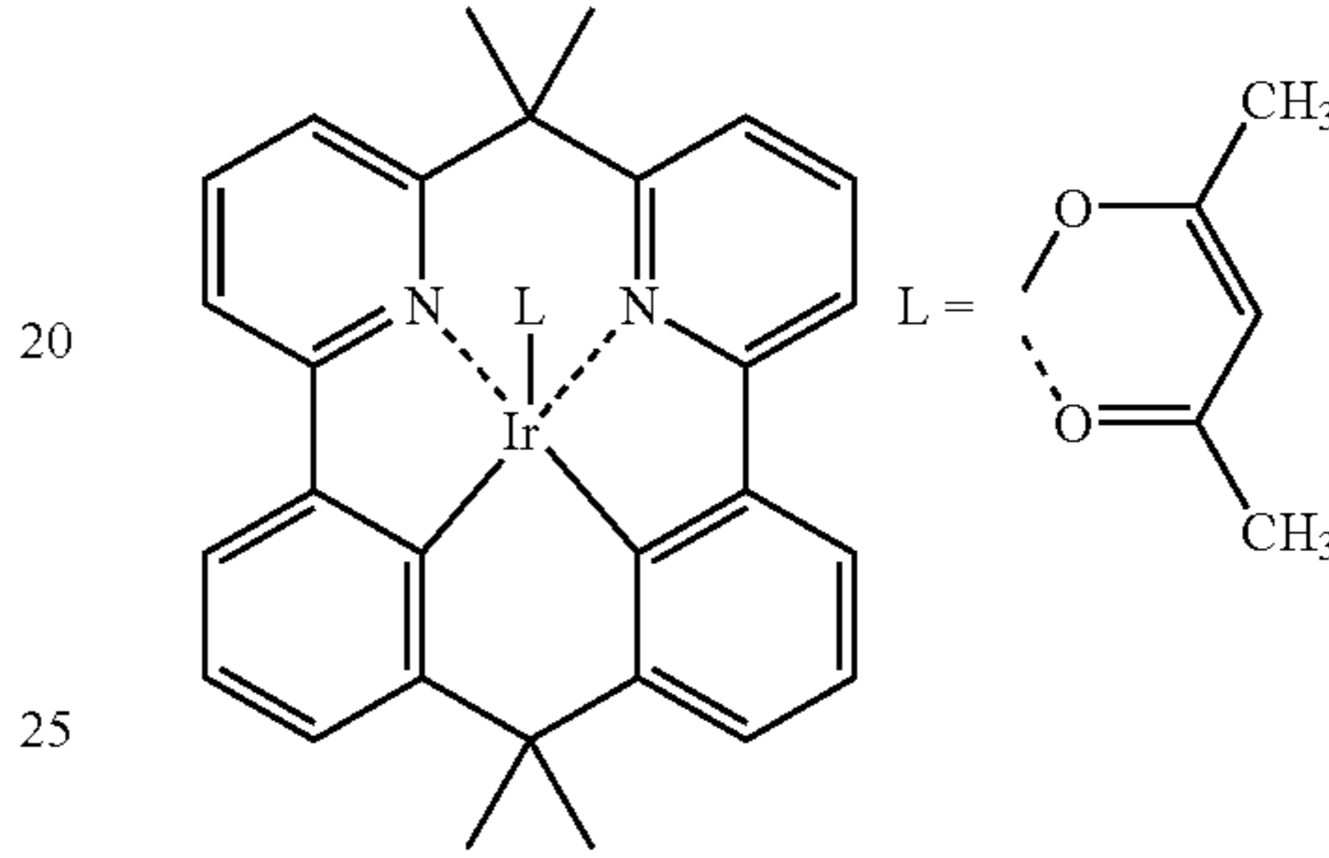
Compound (110)
