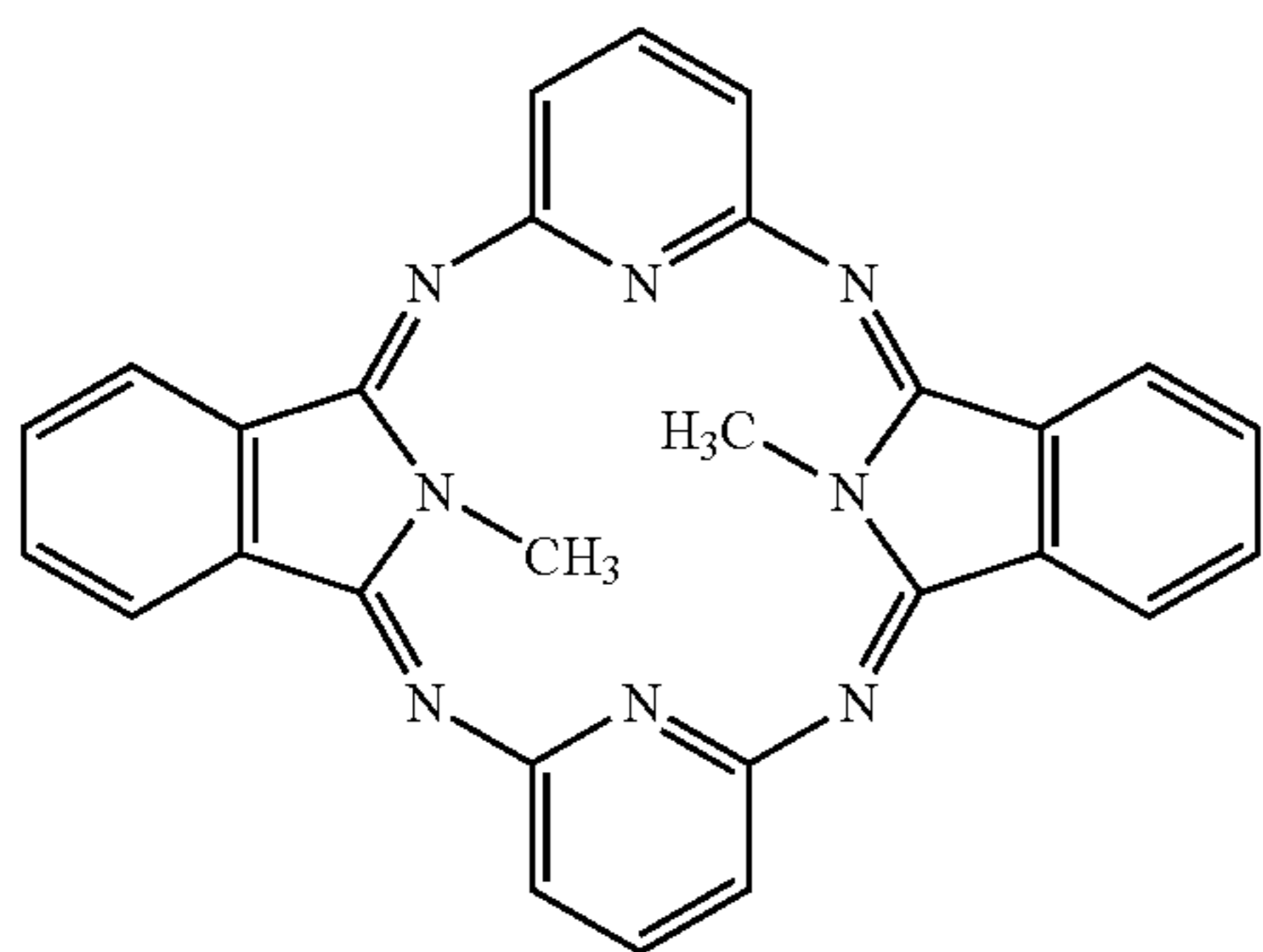
Compound (55)
