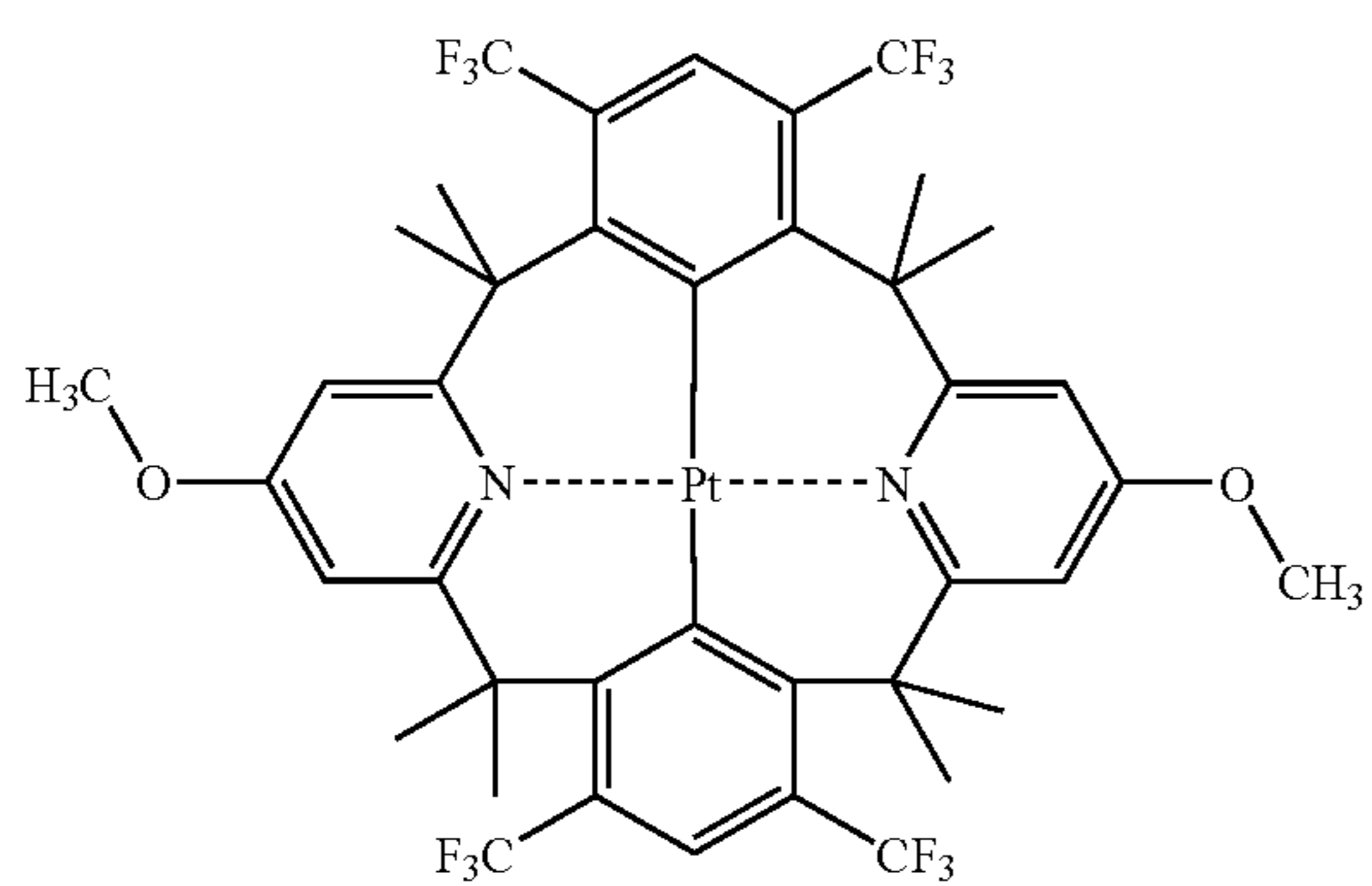
Compound (146)
