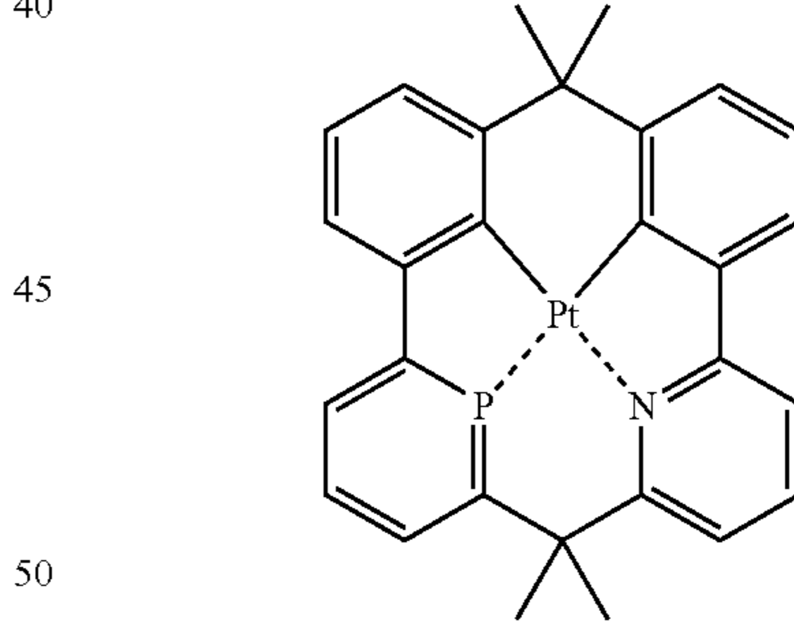
Compound (112)
