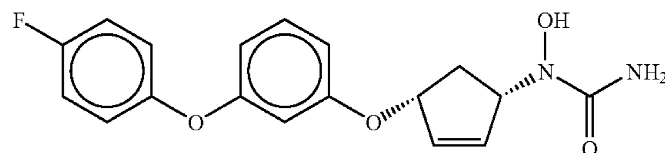
Compound 7
