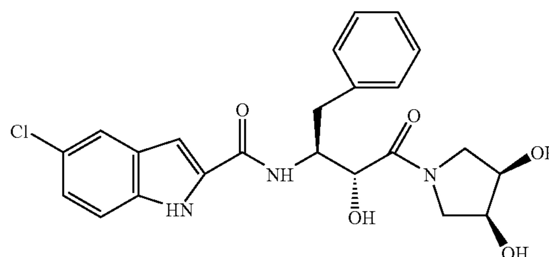
Compound 9
