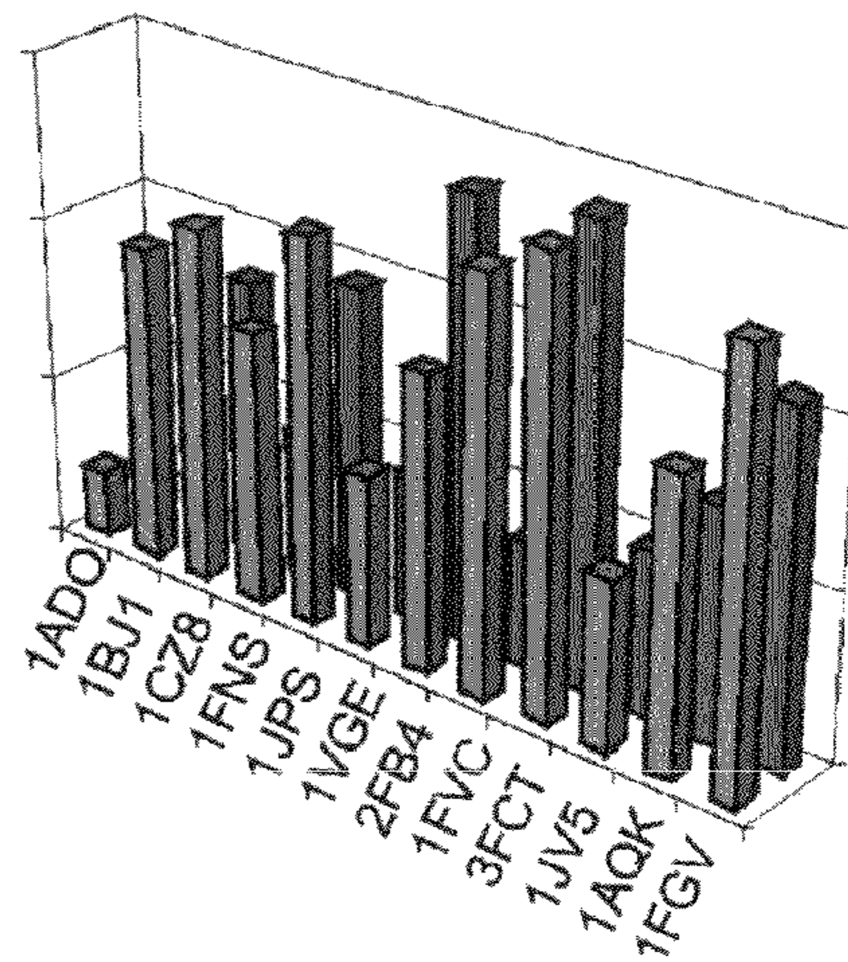
Homology with MNAC13
