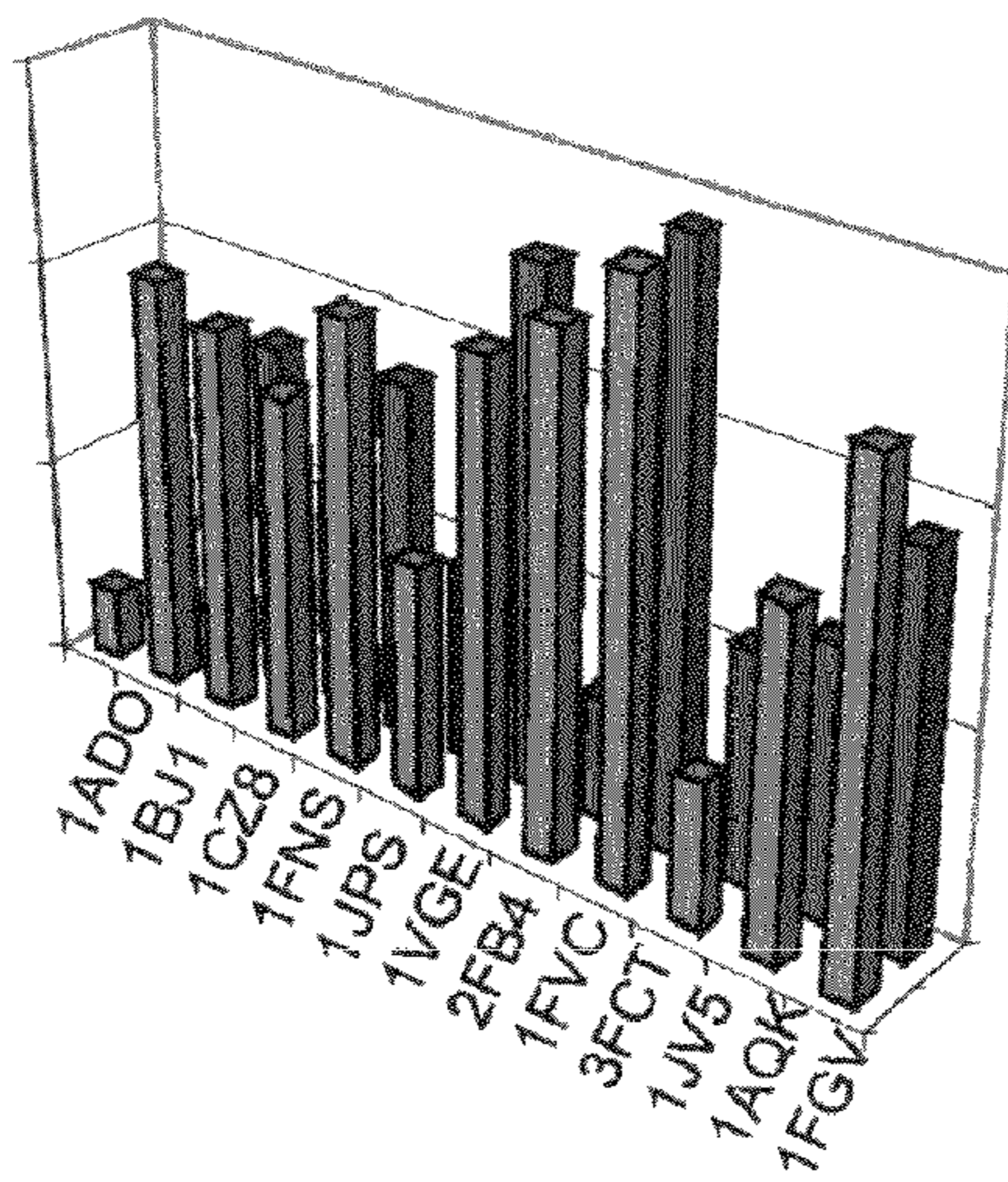
Identity with MNAC13
