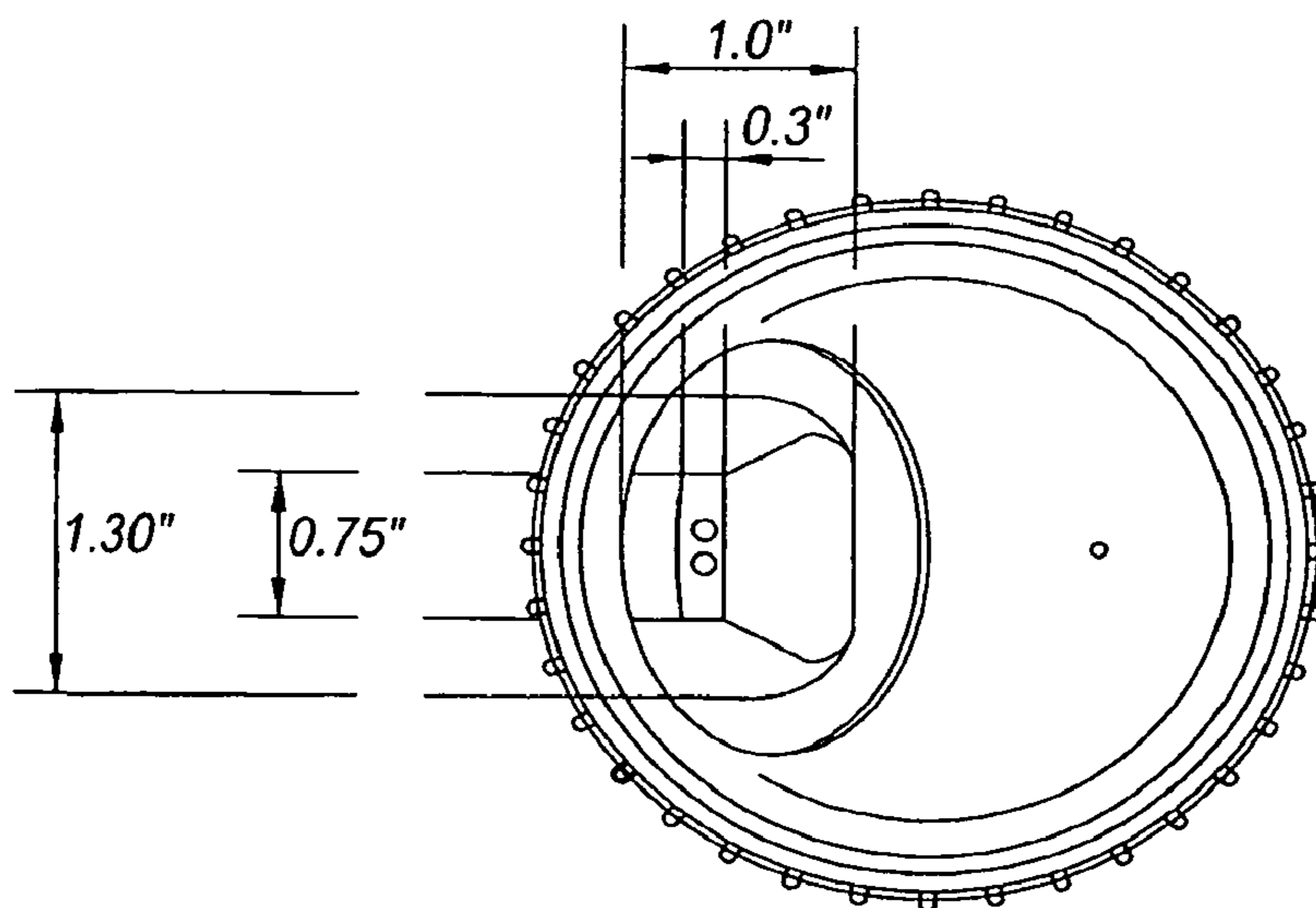
Fig. 17 (Prior Art)
