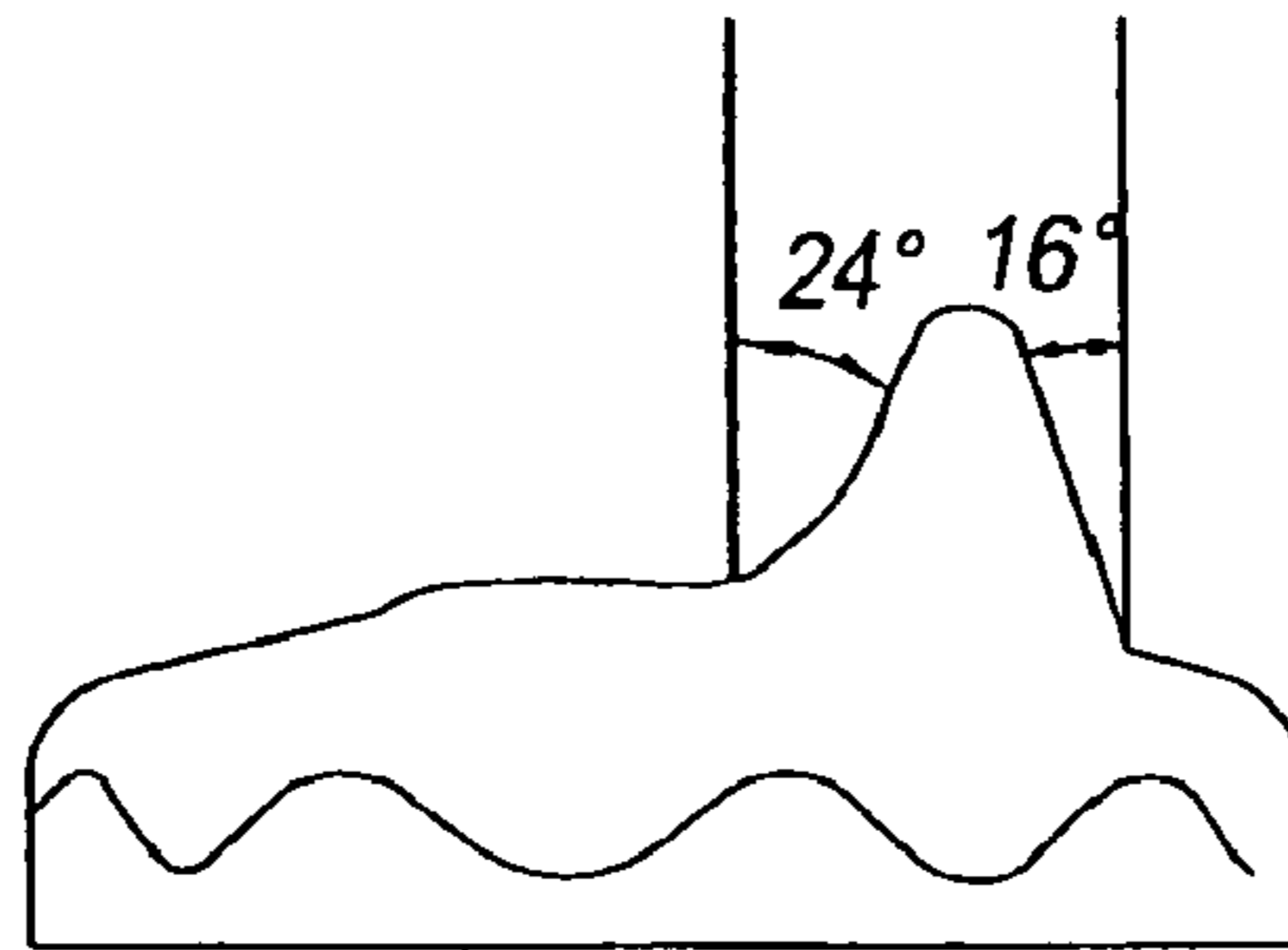
Fig. 19 (Prior Art)
