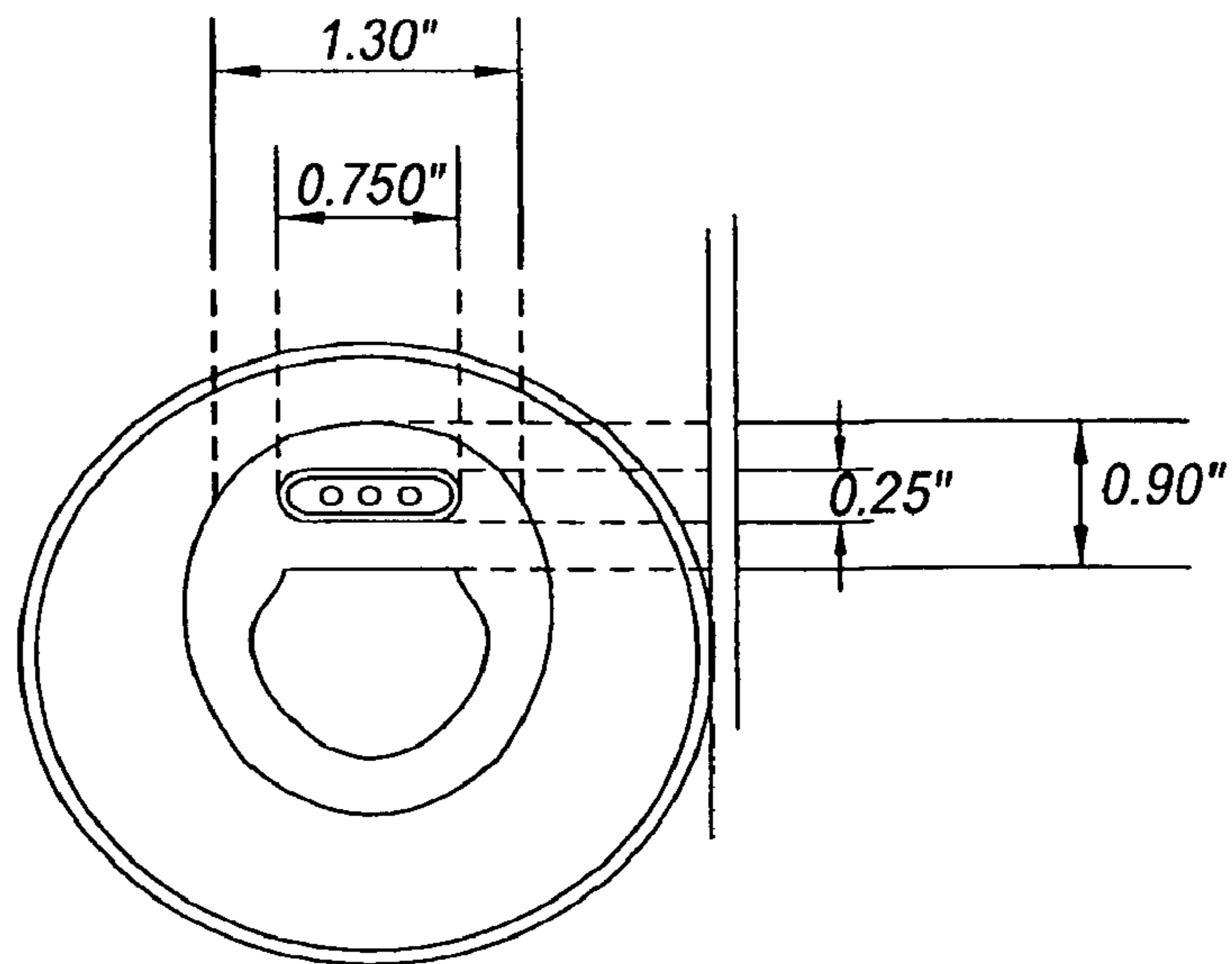
Fig. 20 (Prior Art)
