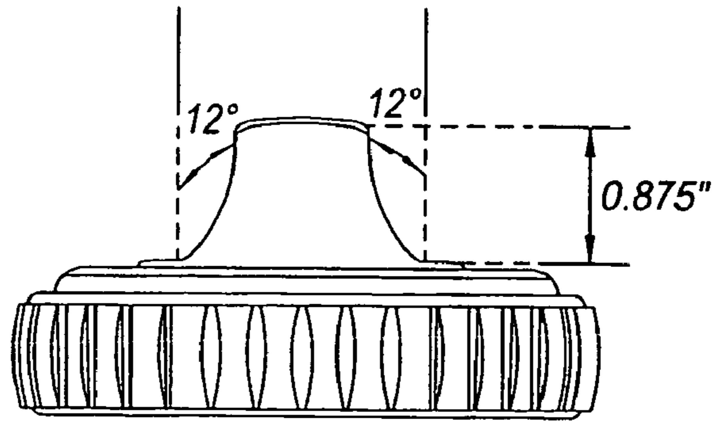
Fig. 15 (Prior Art)
