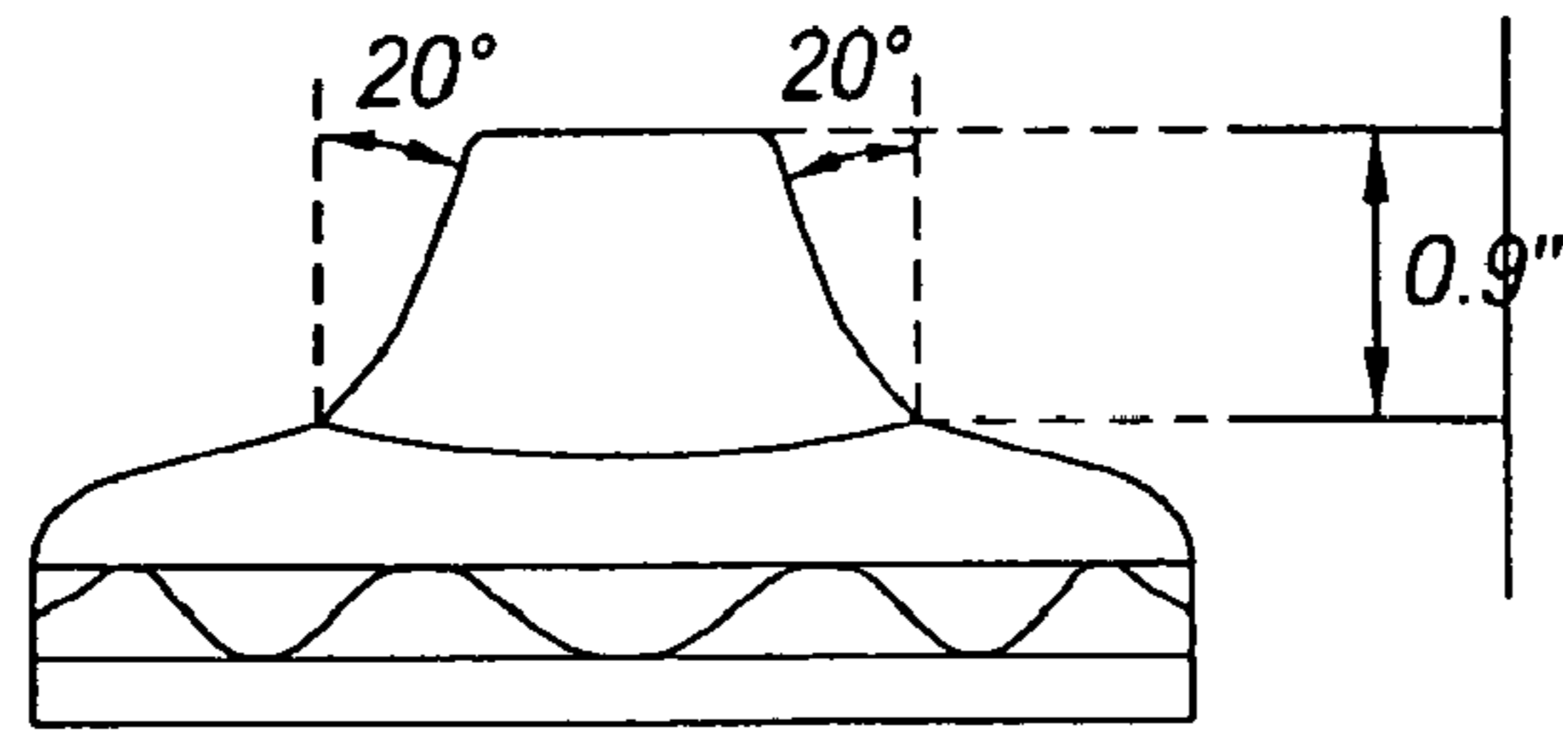
Fig. 18 (Prior Art)
