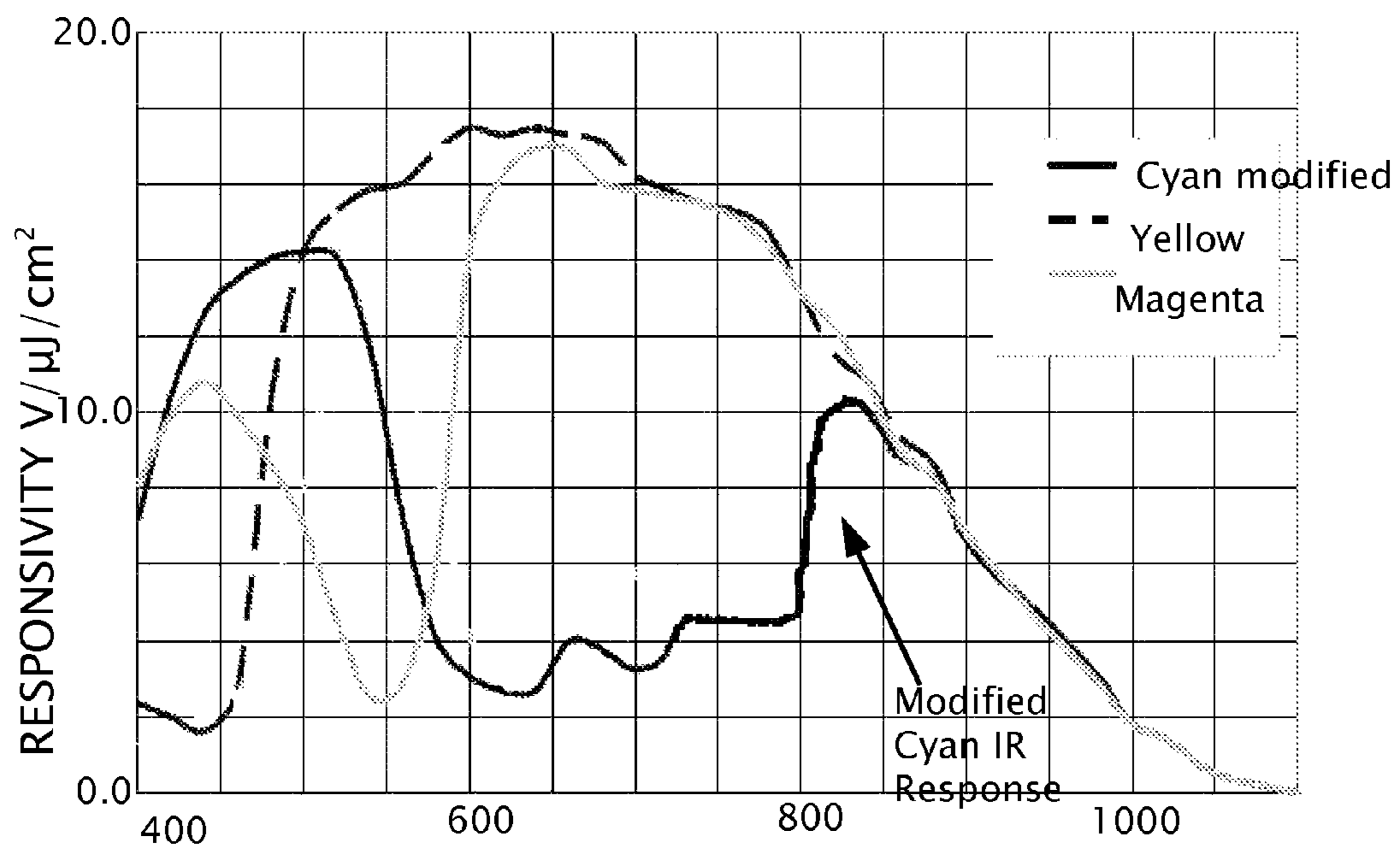
WAVELENGTH (nm) Fig. 3b
