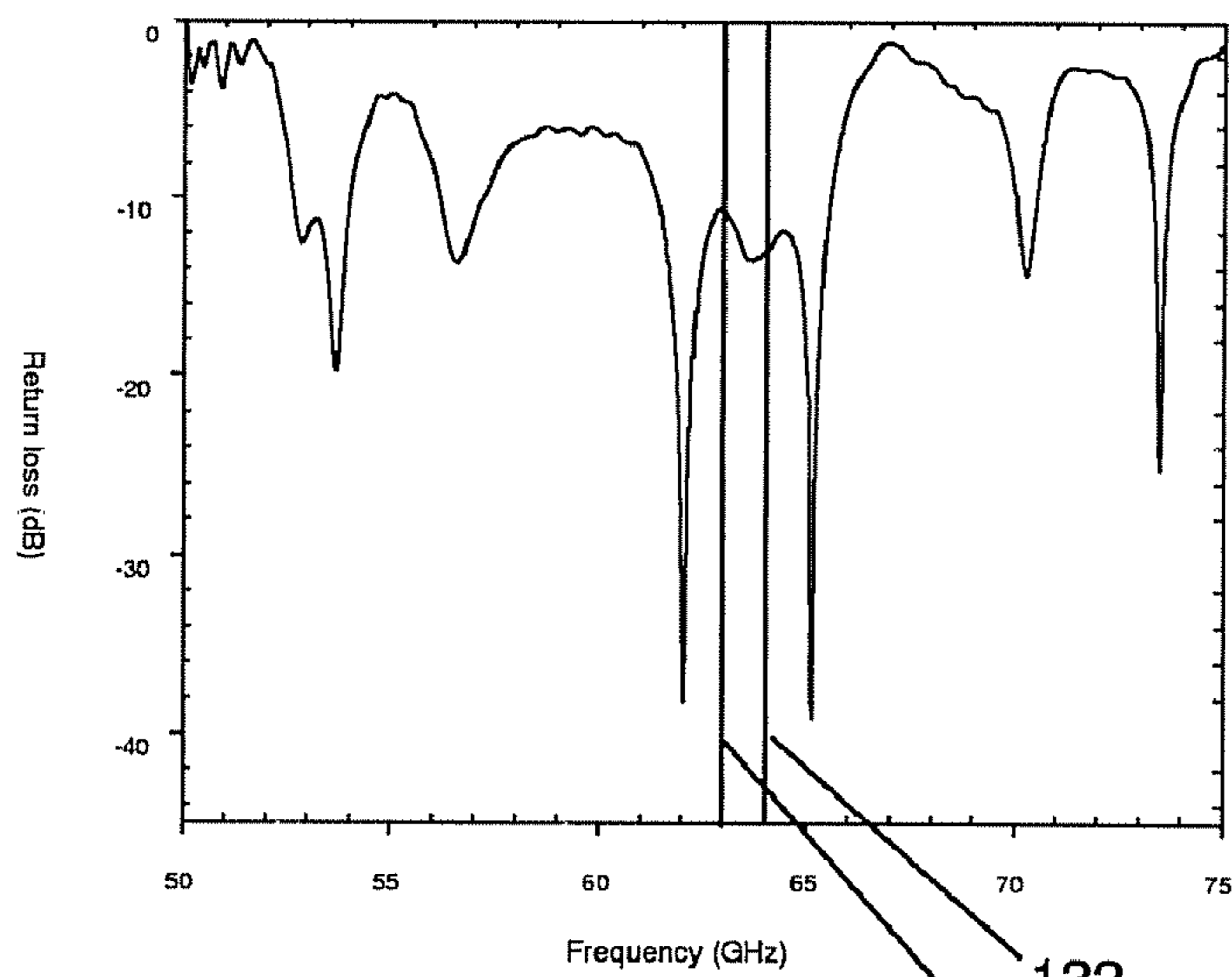
Slot with bent transition
