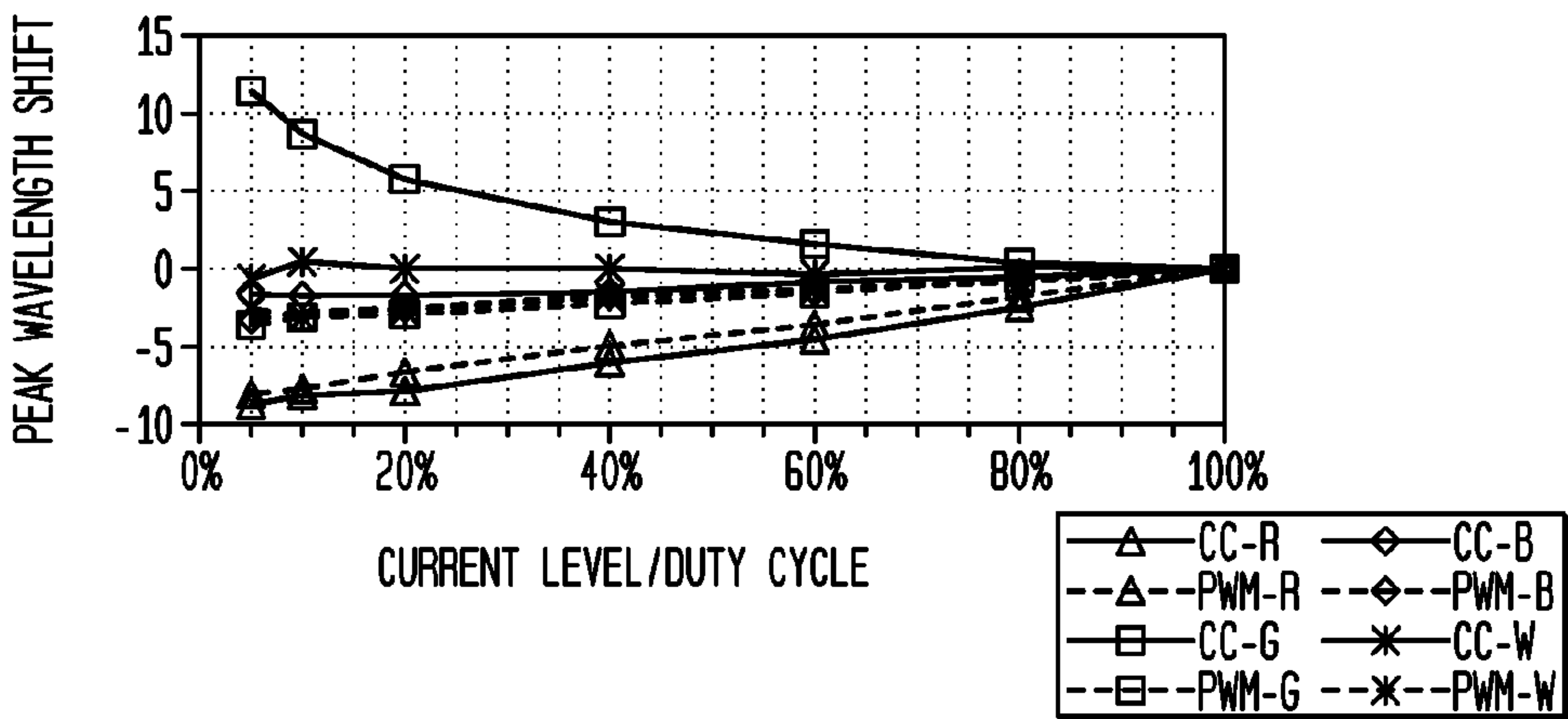
FIG. 2C (PRIOR ART)
