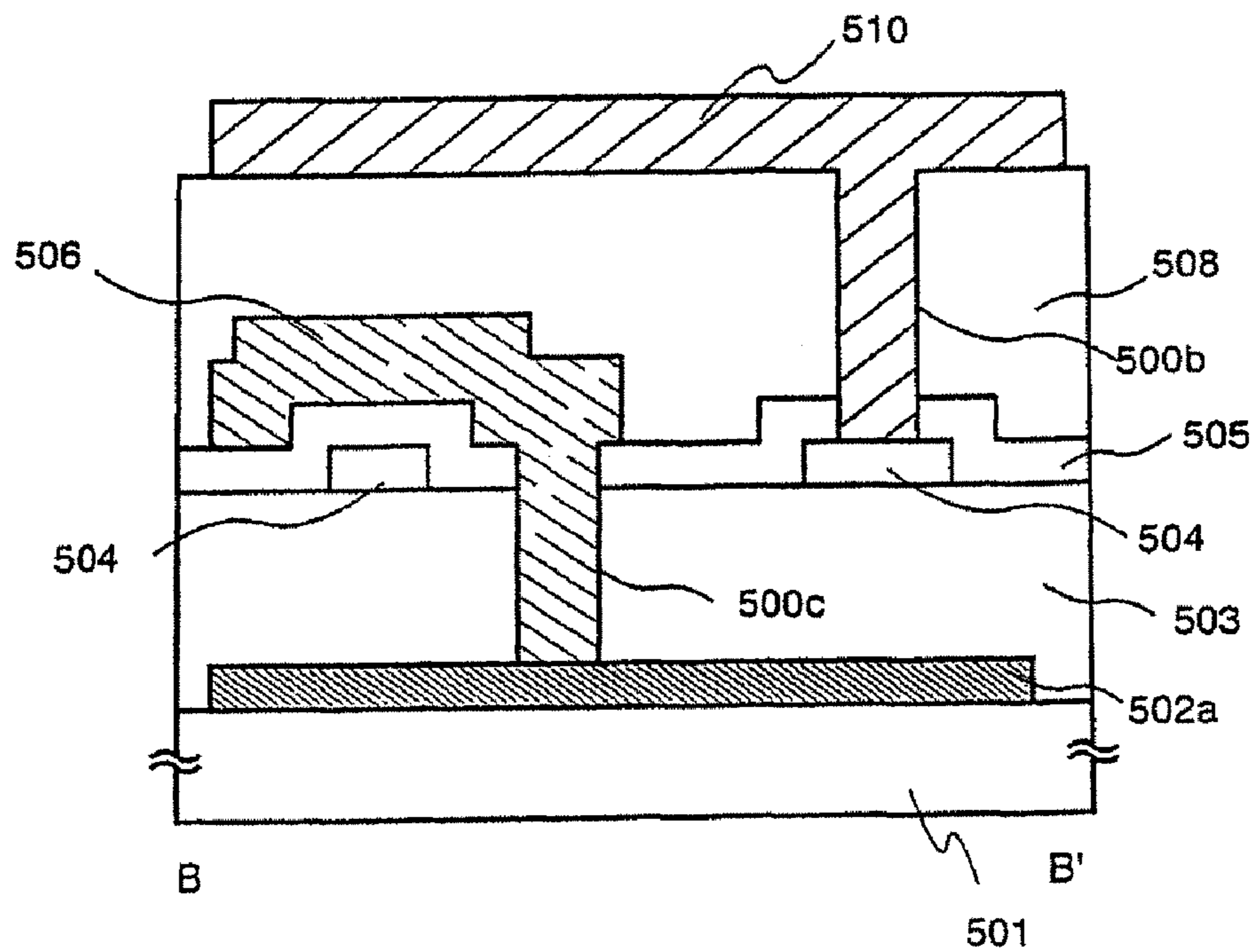
Fig. 15B B-B' Cross sectional view
