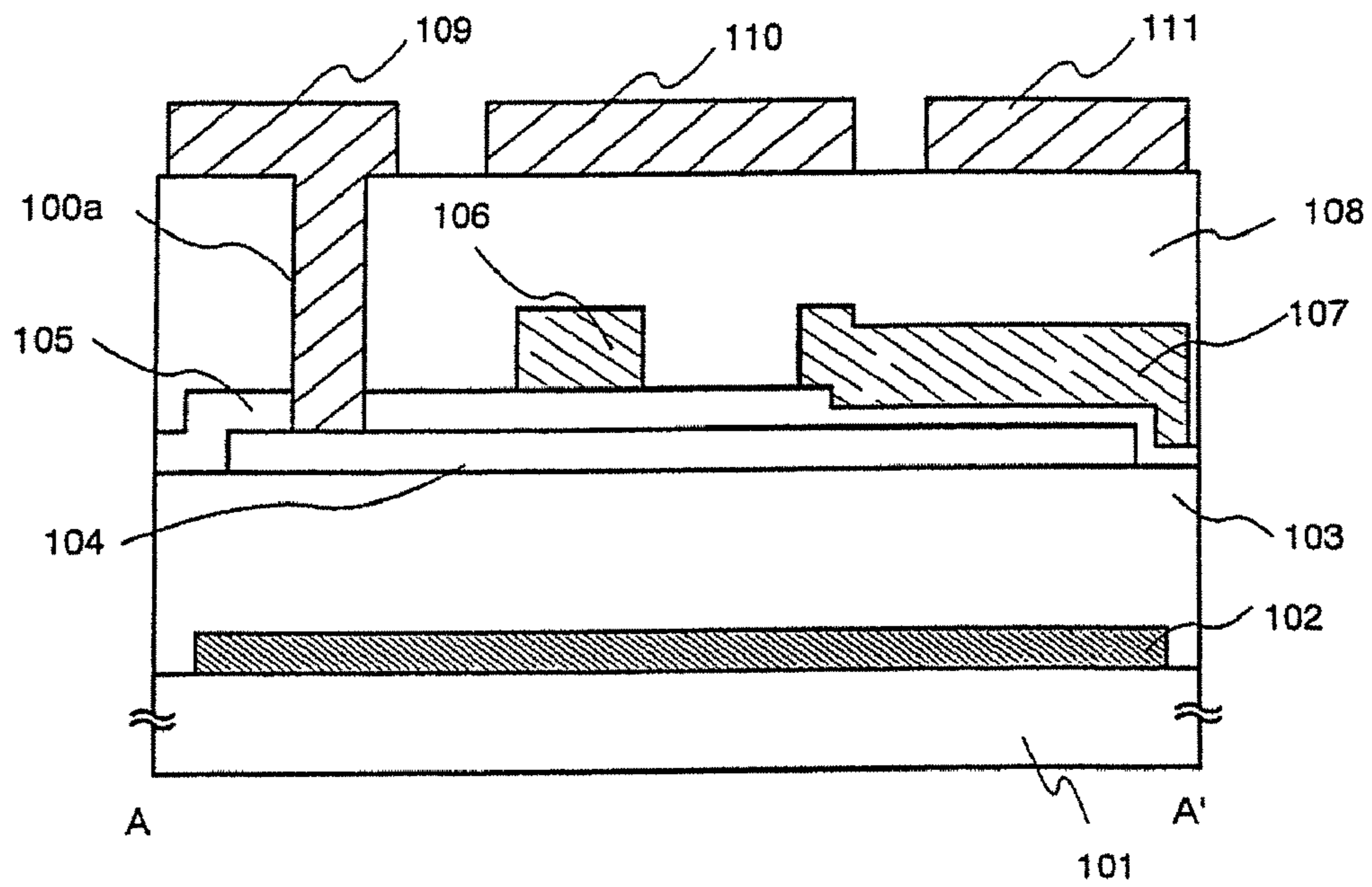
Fig. 3A A-A' cross sectional view
