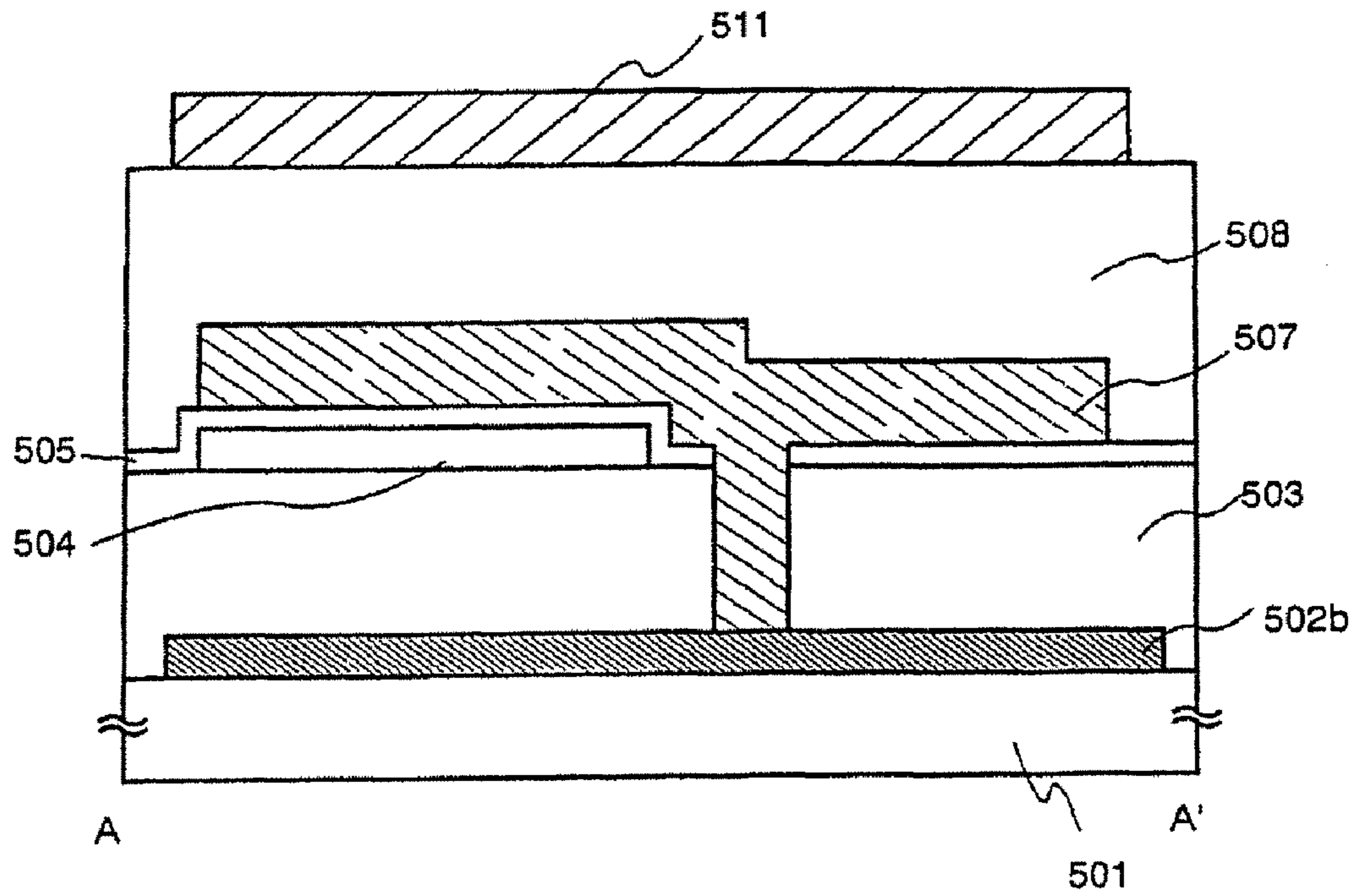
Fig. 15A A-A' Cross sectional view
