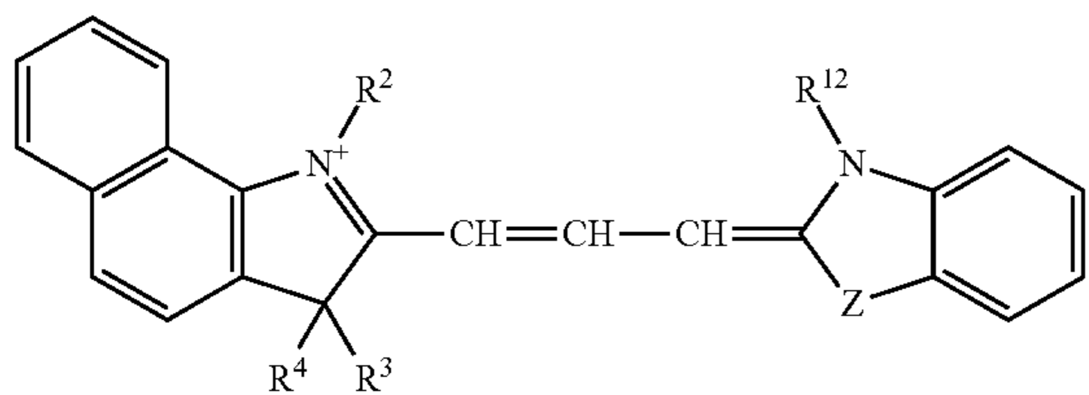
Formula XV
