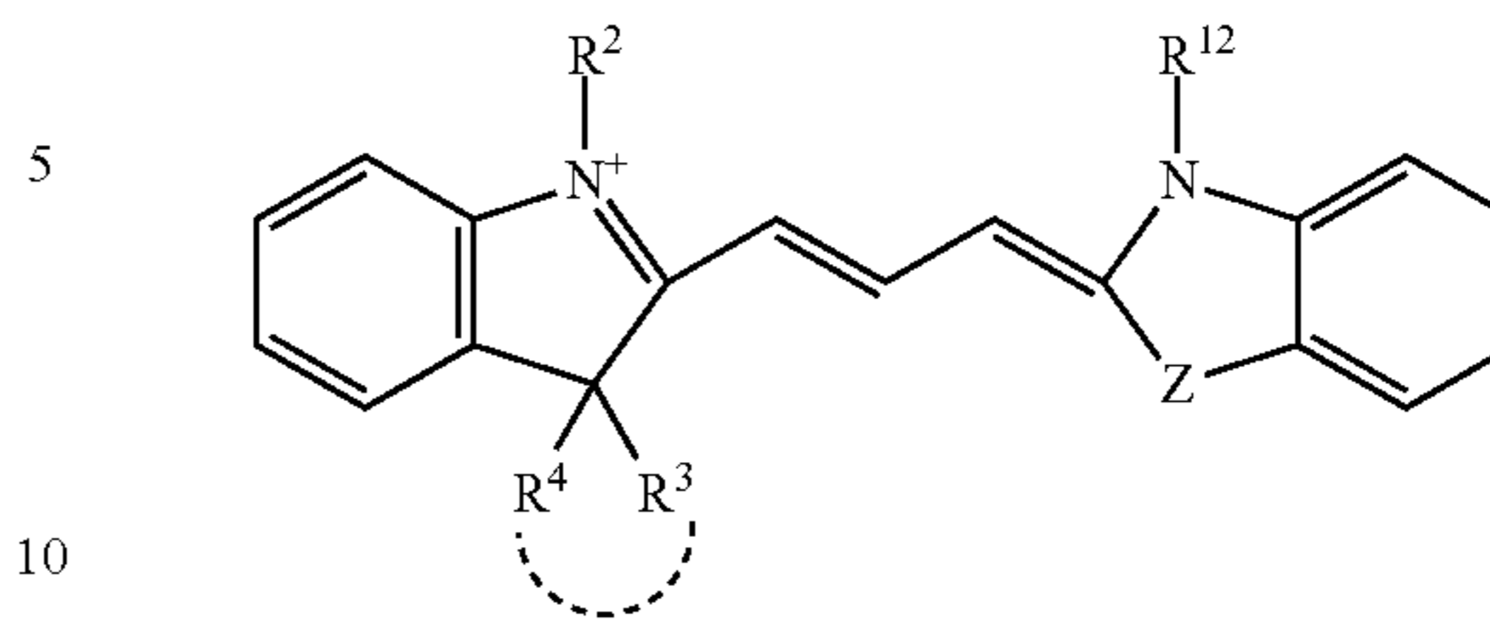
Formula XII
