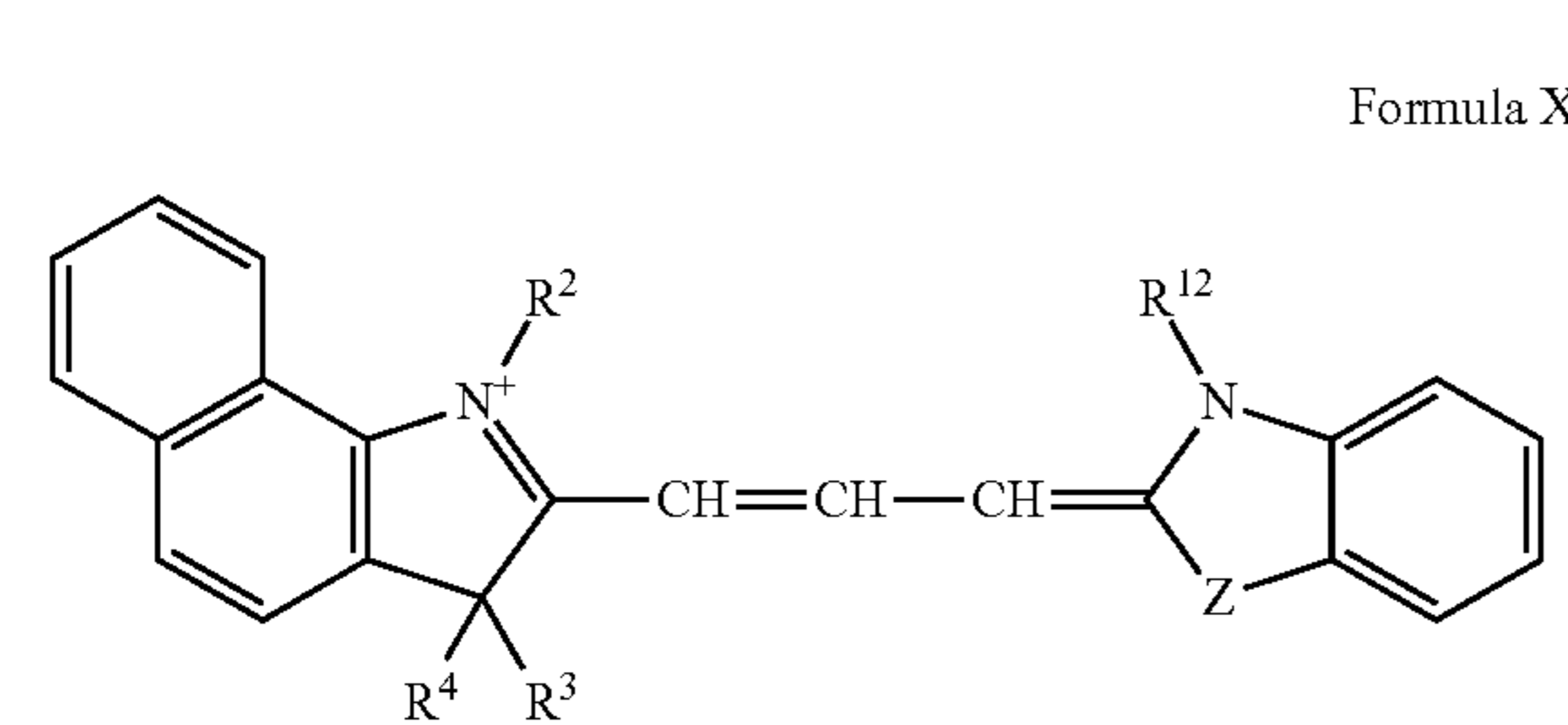
Formula XVI
