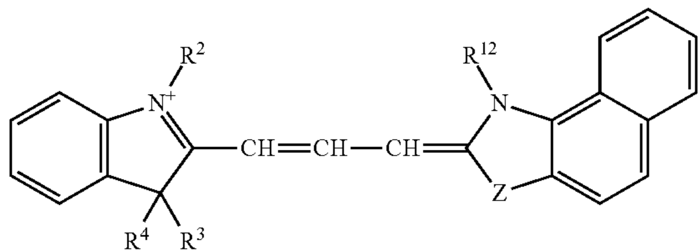
Formula XVII
