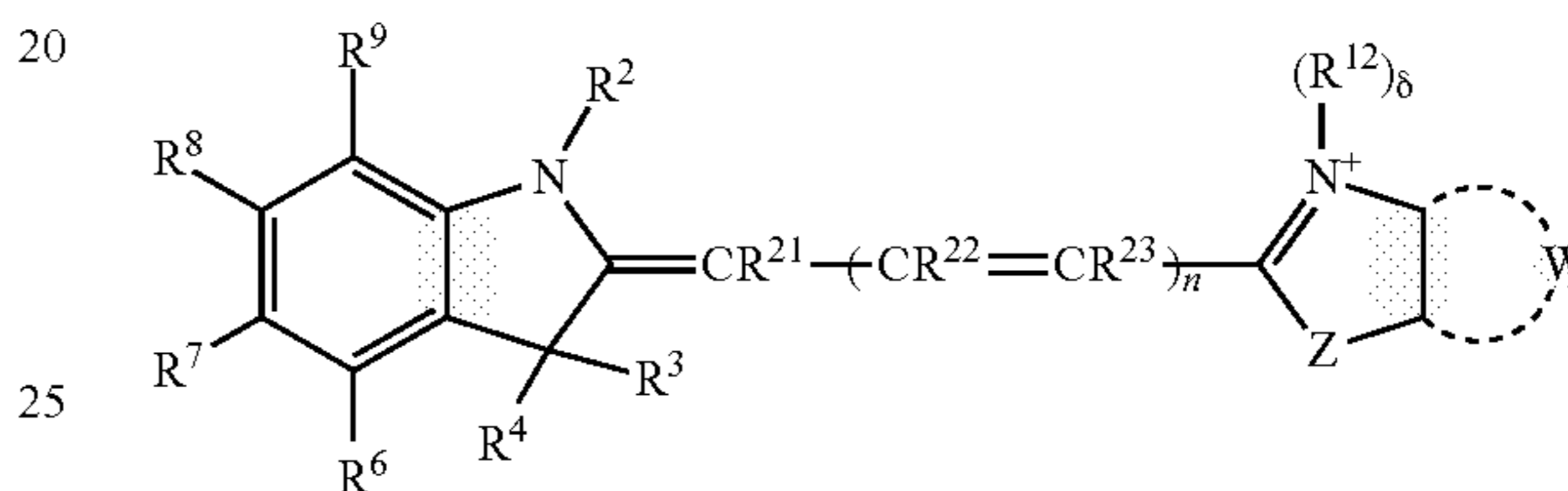
Formula XI
