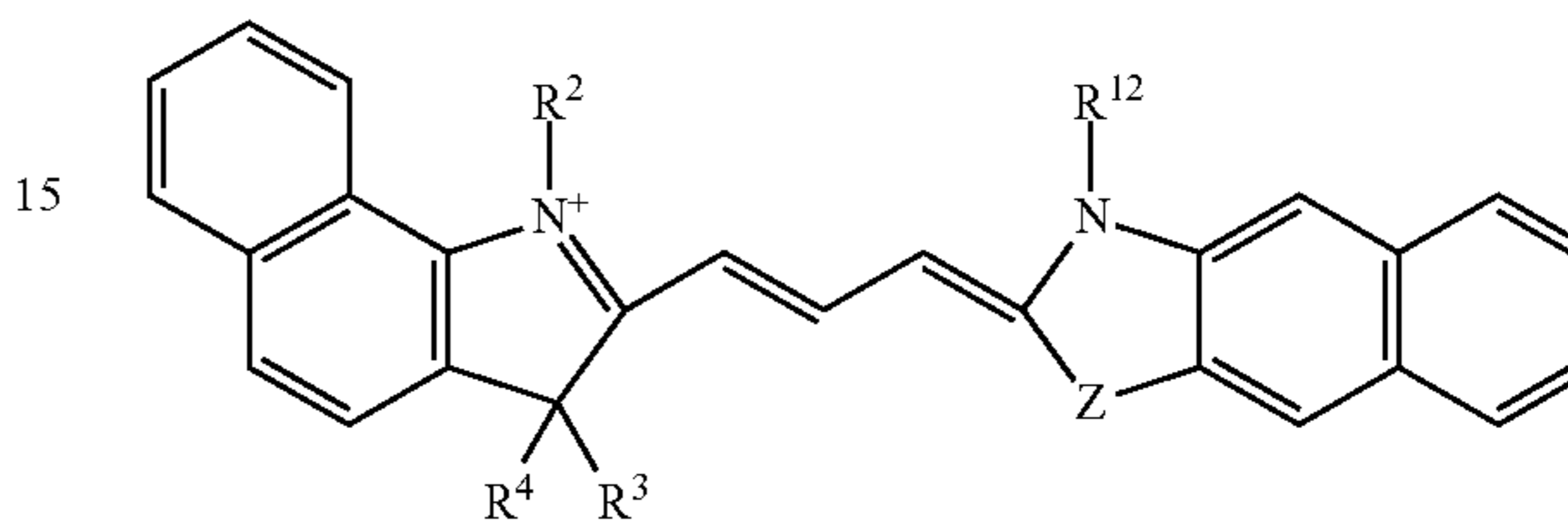
Formula XIII
