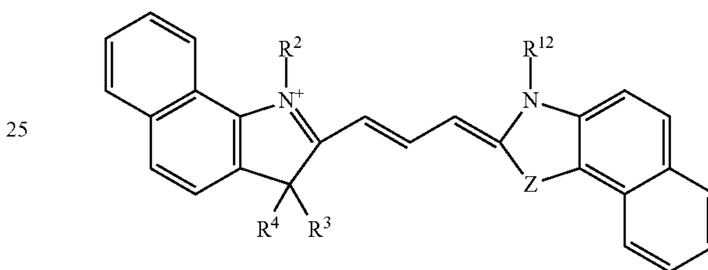
Formula XIV
