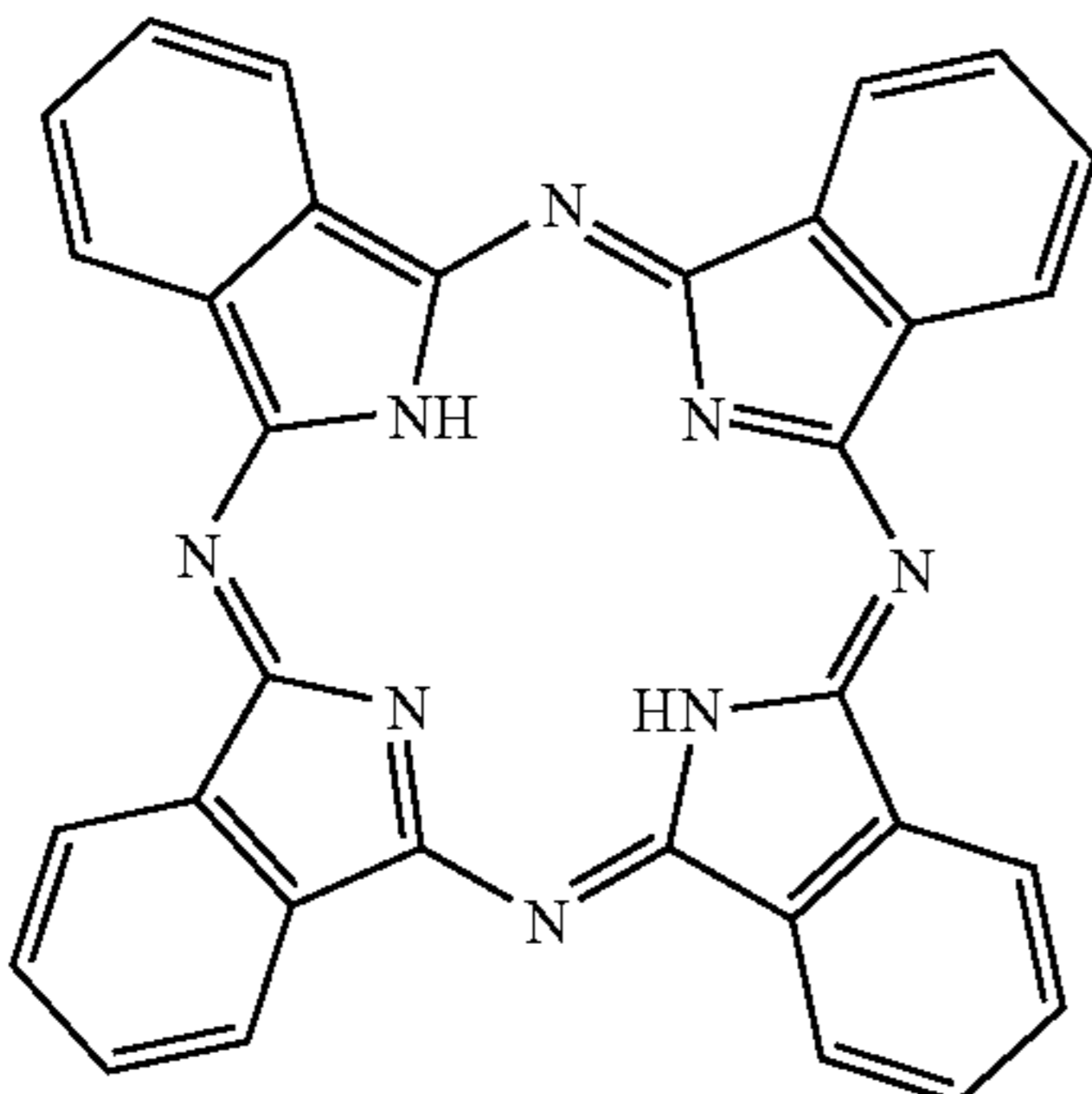
Phthalocyanine
