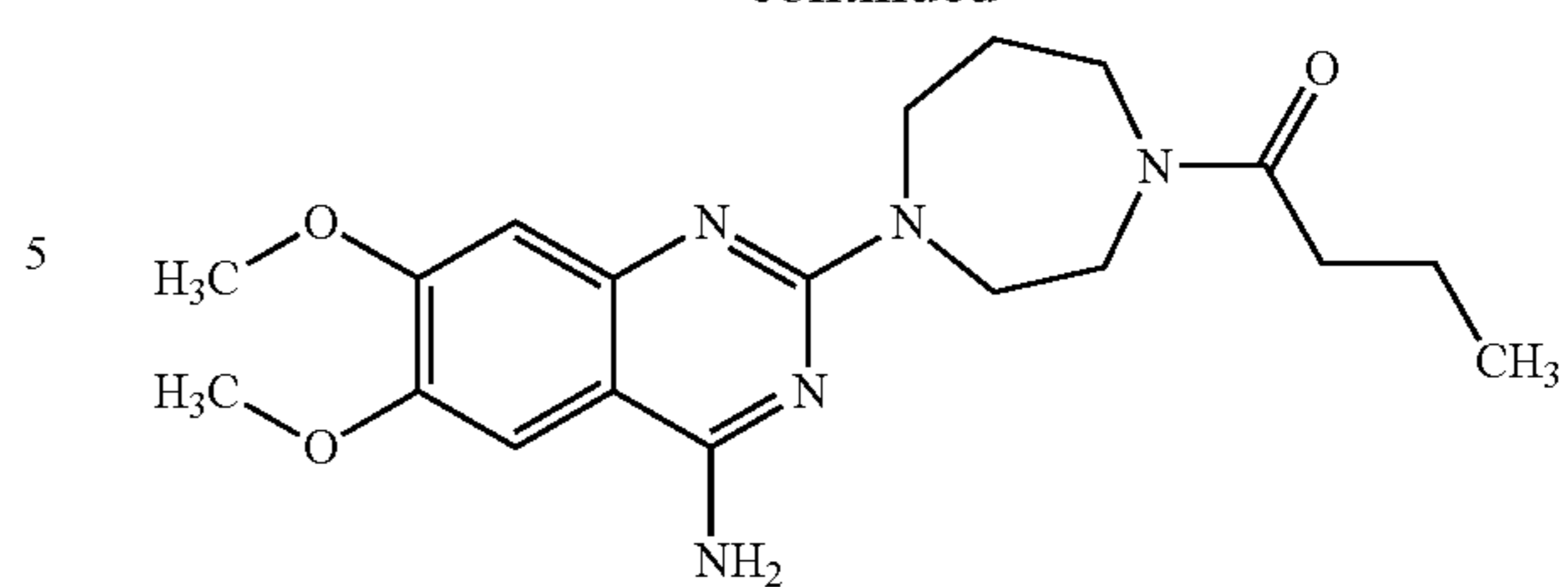
Bunazosin: U.S. Pat. No. 3,920,636
