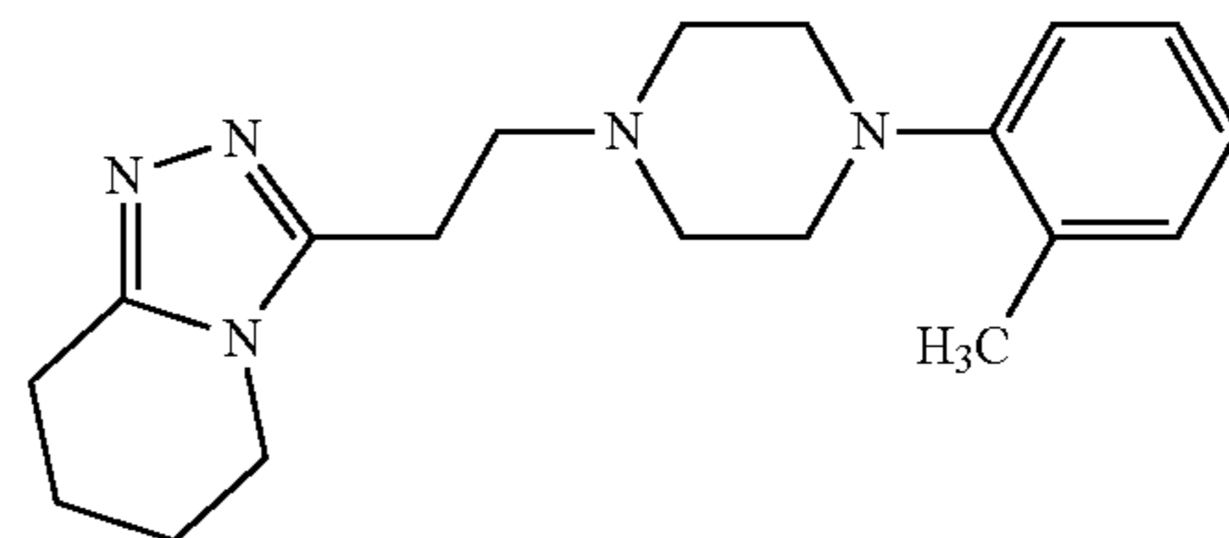
Dapiprazole: U.S. Pat. No. 4,252,721
