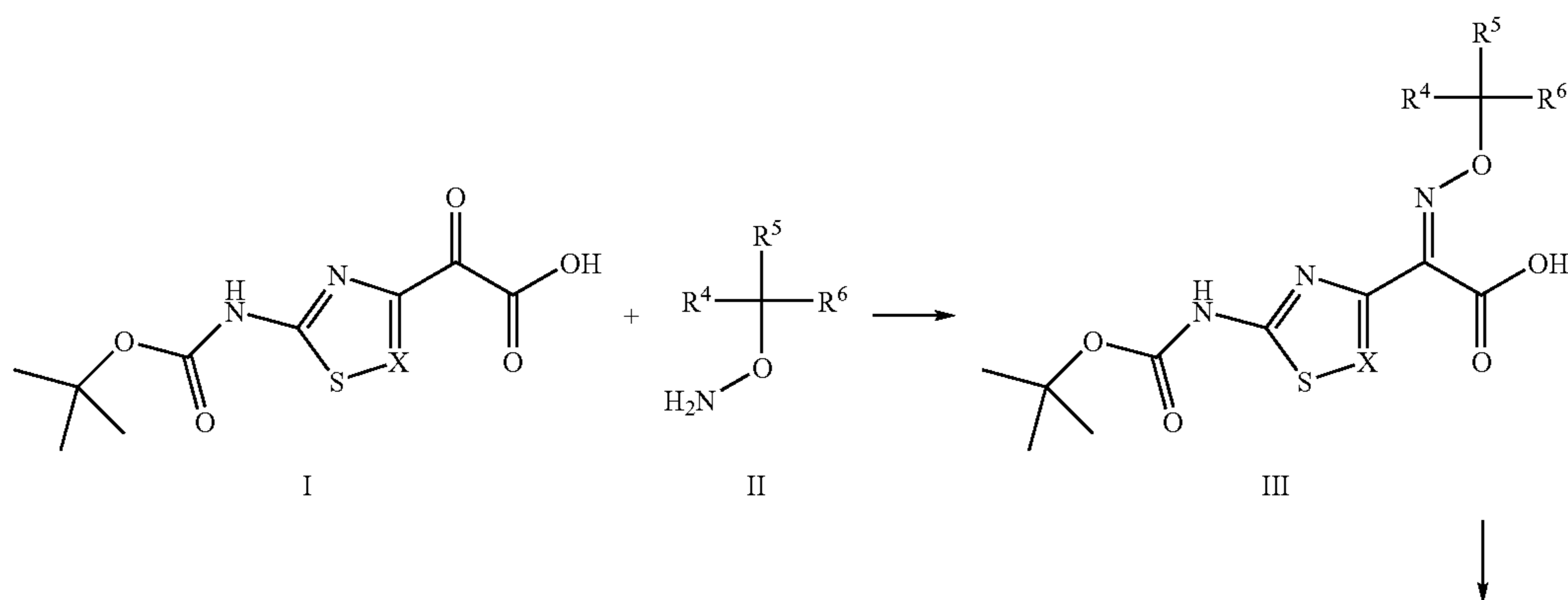
Scheme A
