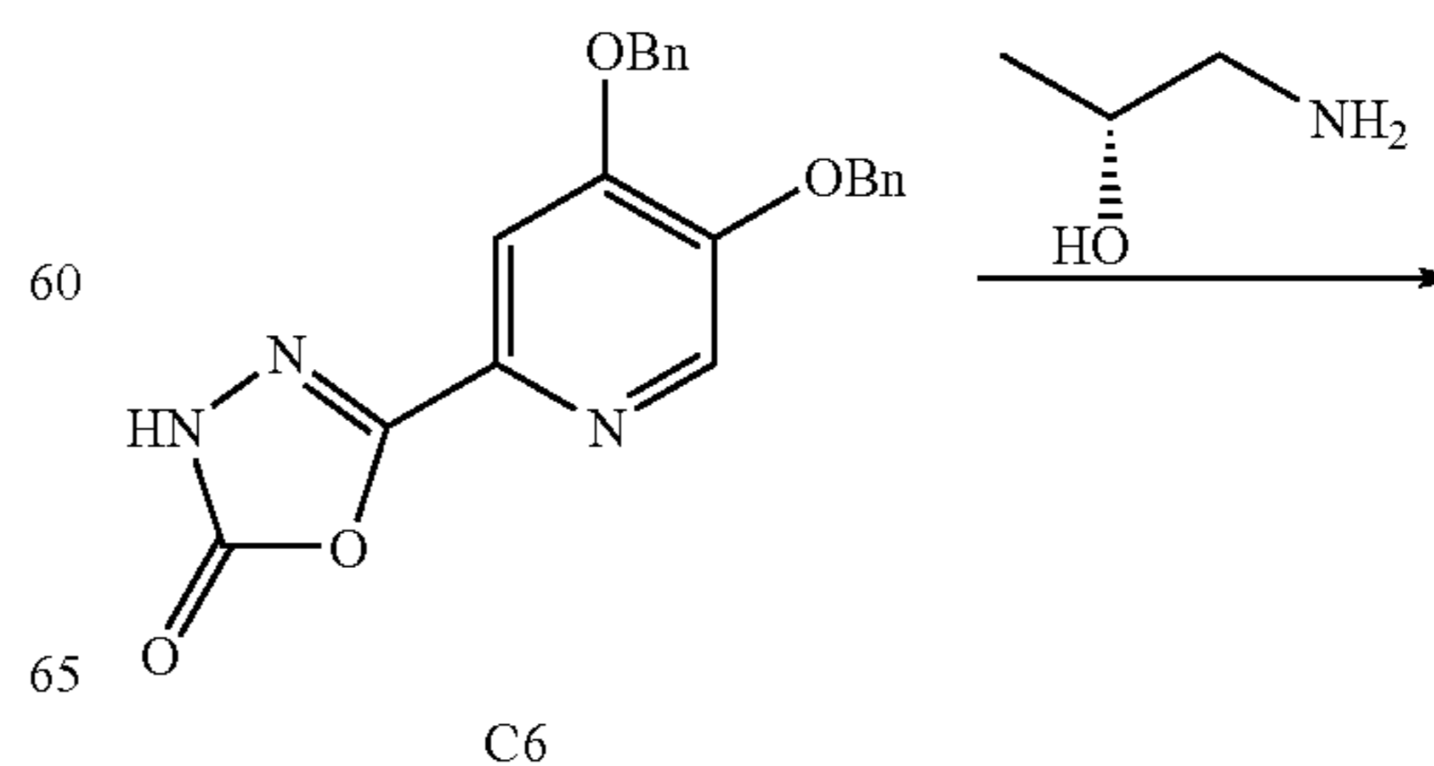
Scheme 17
