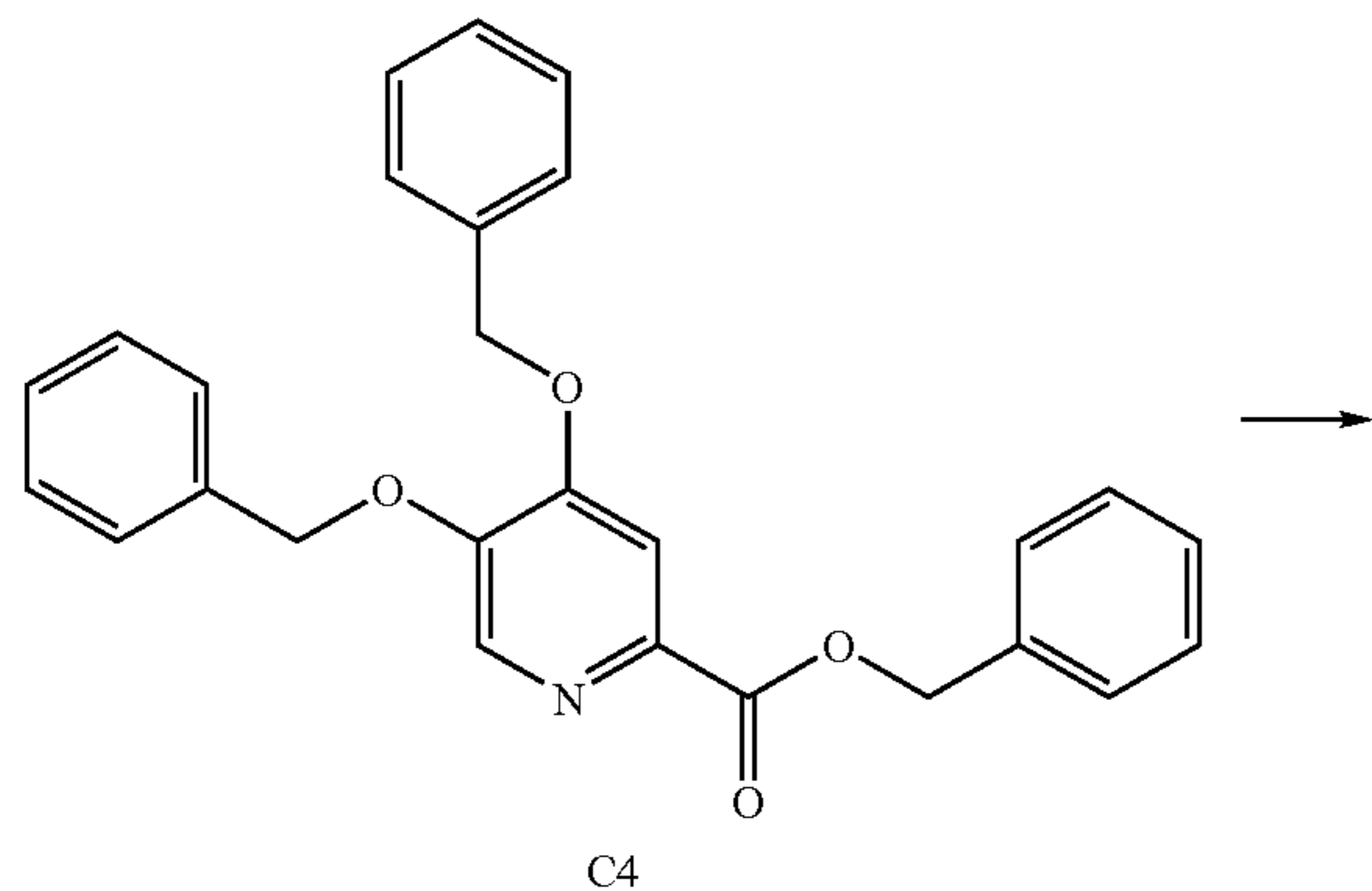
Scheme 2
