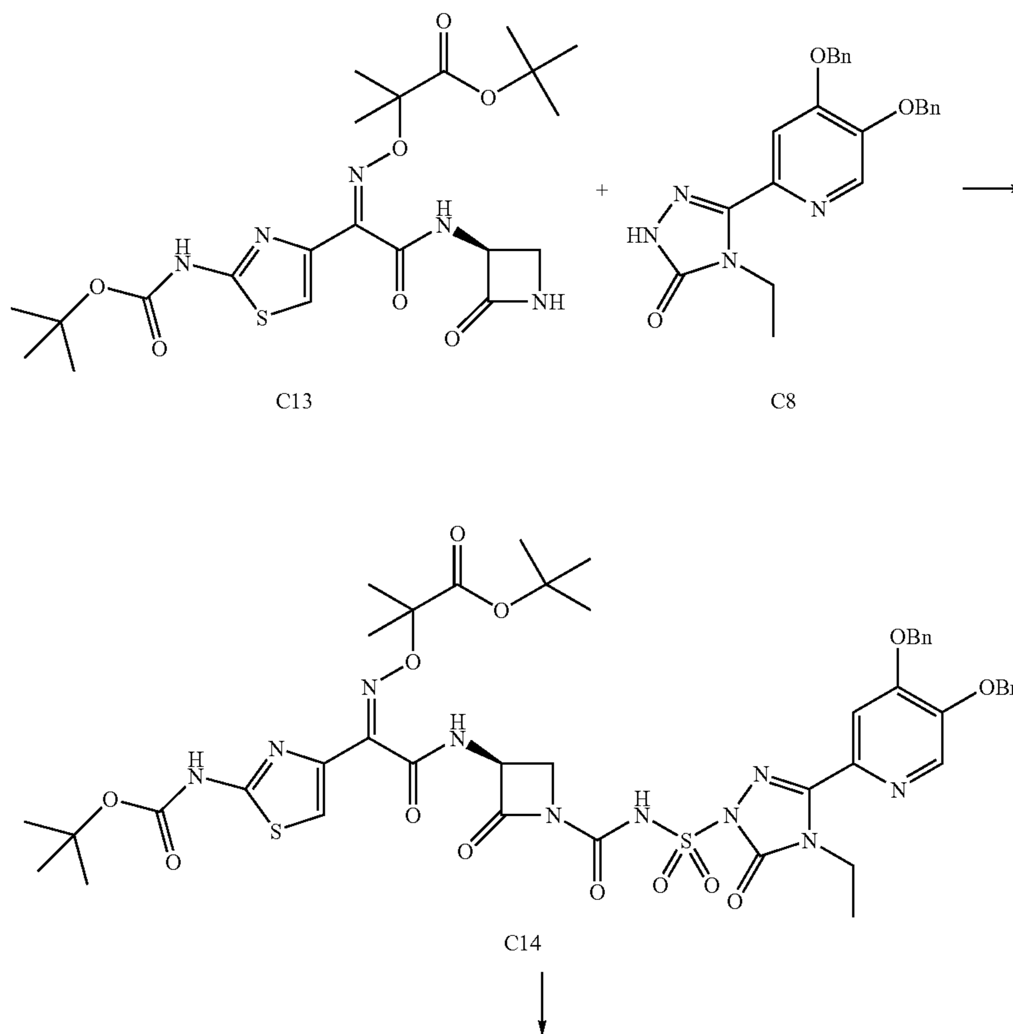
Scheme 6
