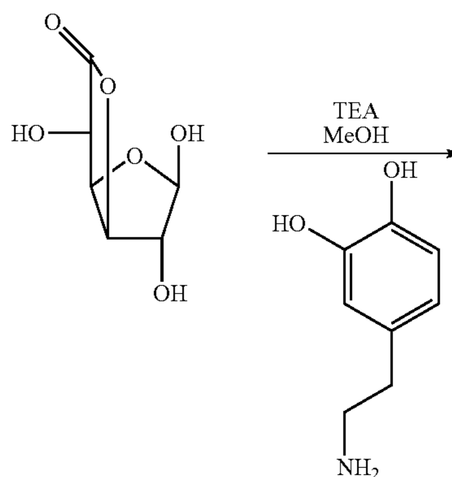
Scheme 1
