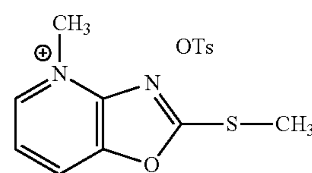
(4-methyl-2-methylthioxazolo[4,5-b]pyridinium tosylate)
