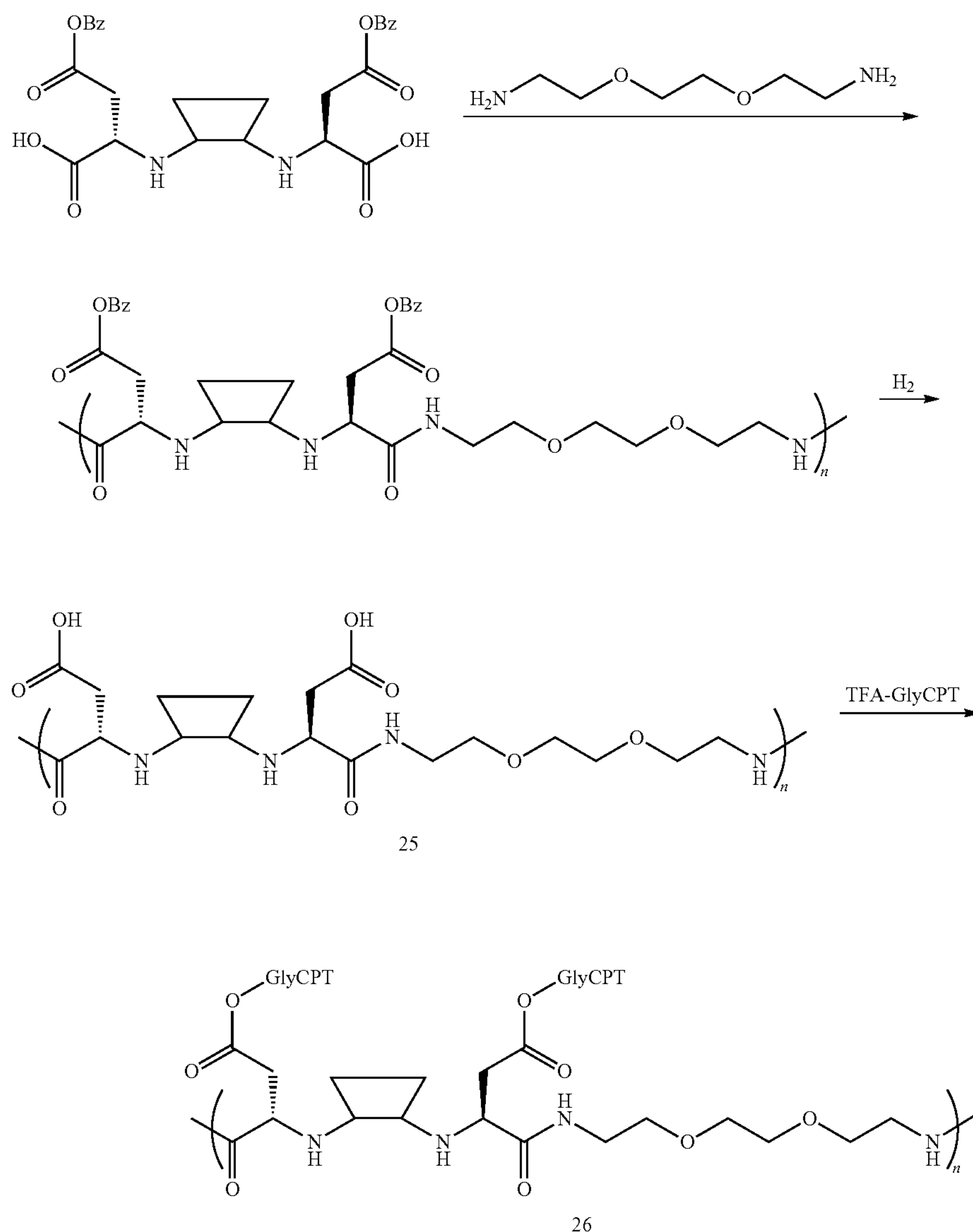
Scheme XXXI
