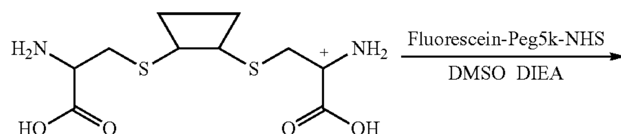
Scheme XXXX
