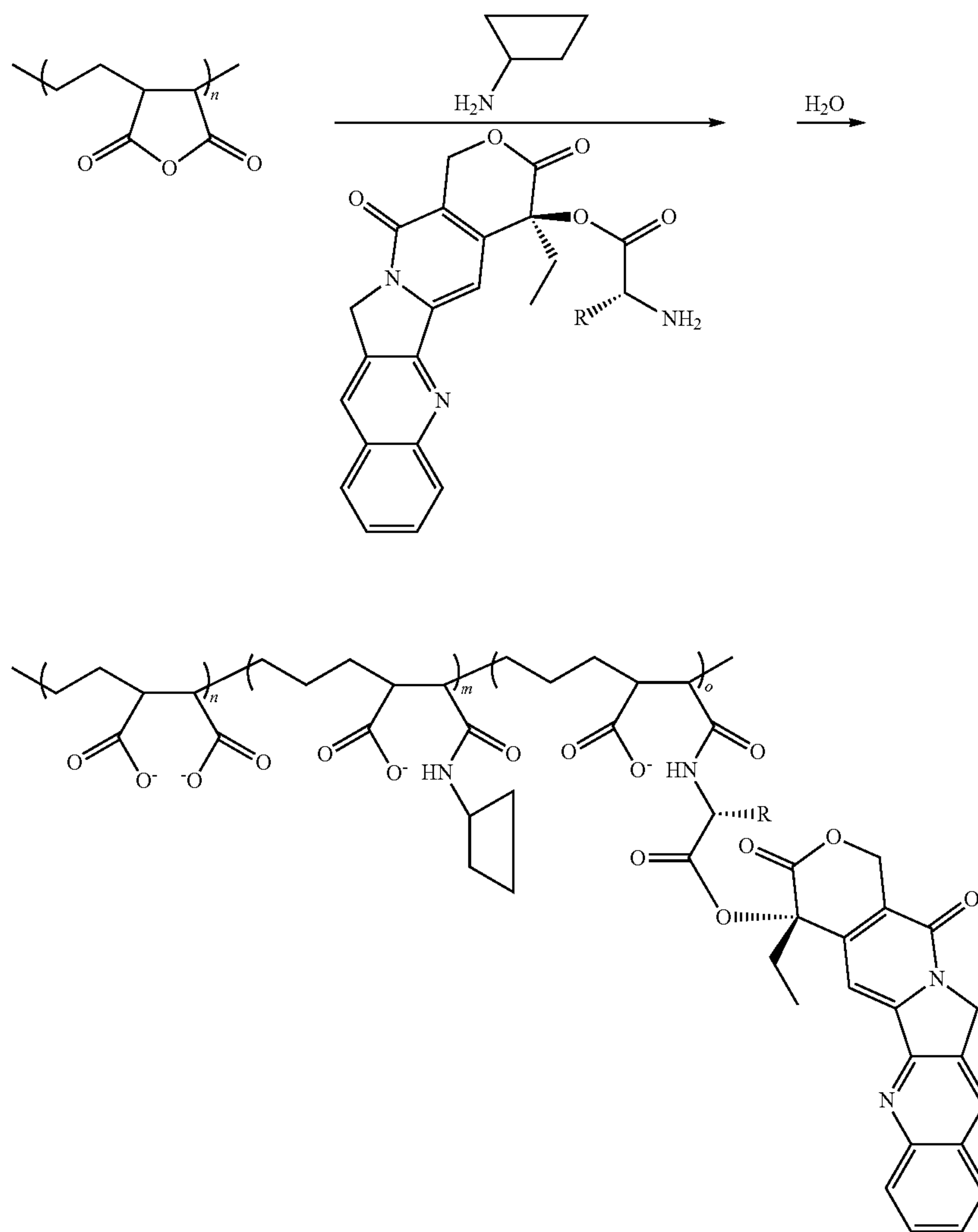
Scheme XI
