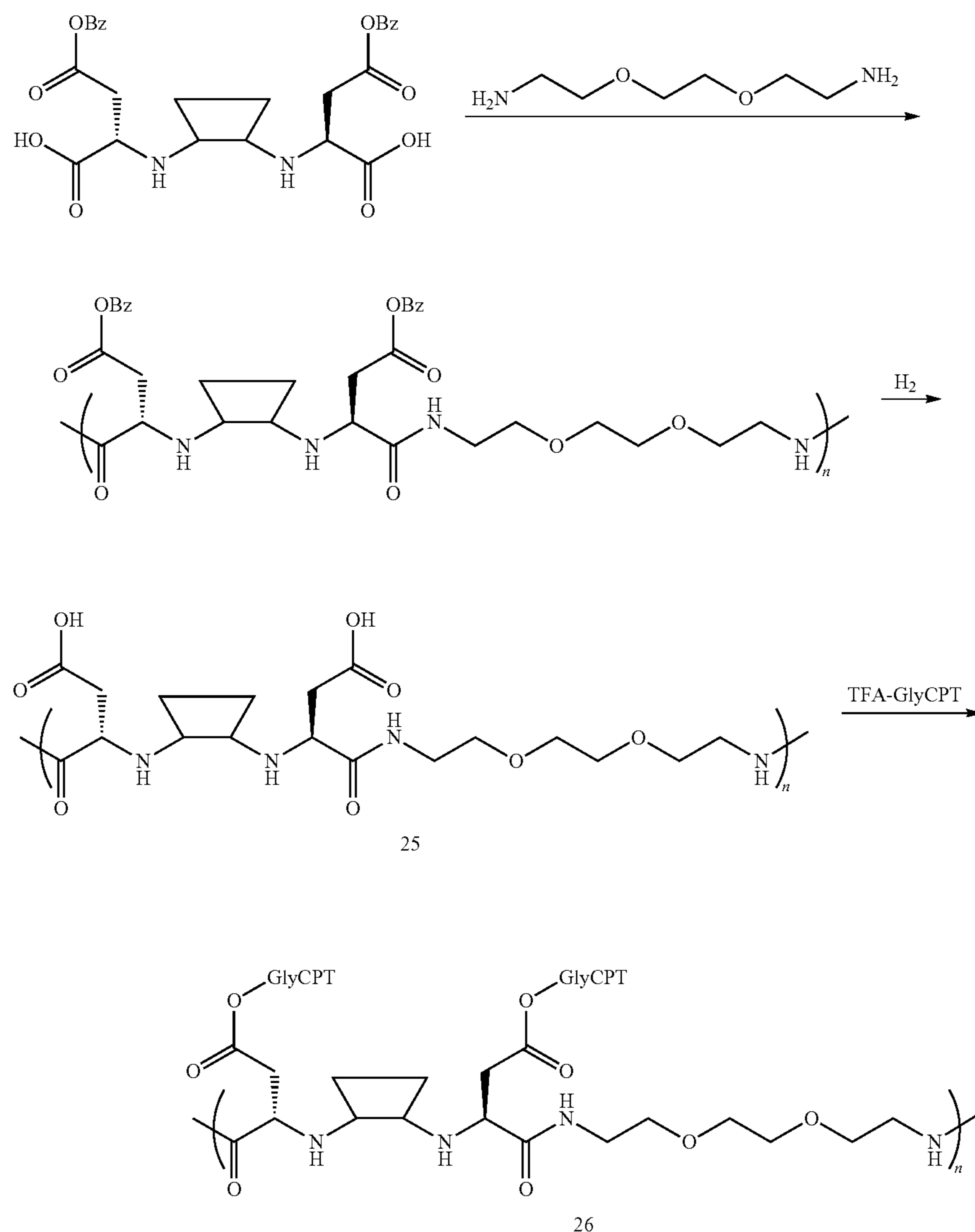
Scheme XXXI
