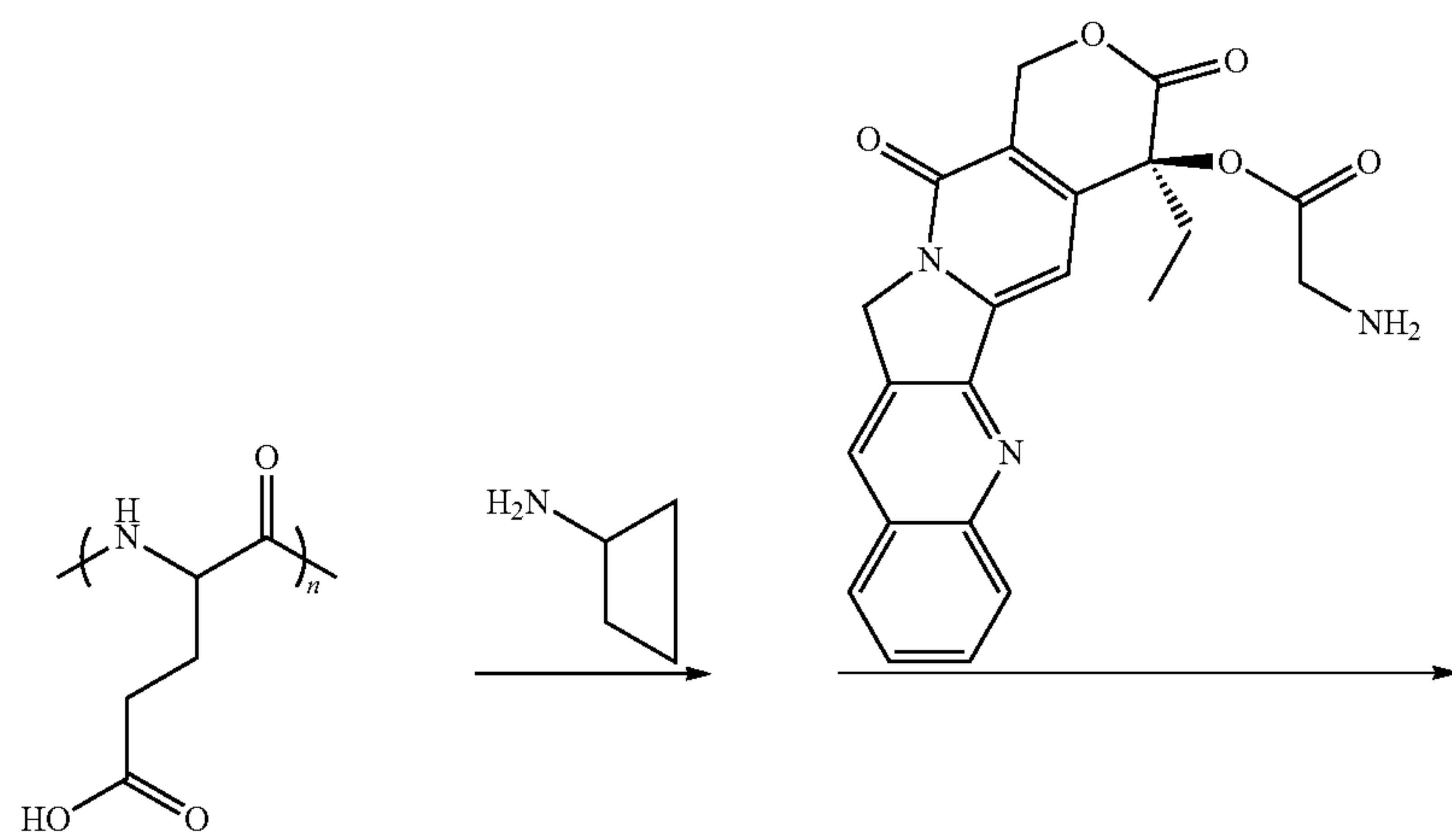
Scheme XII
