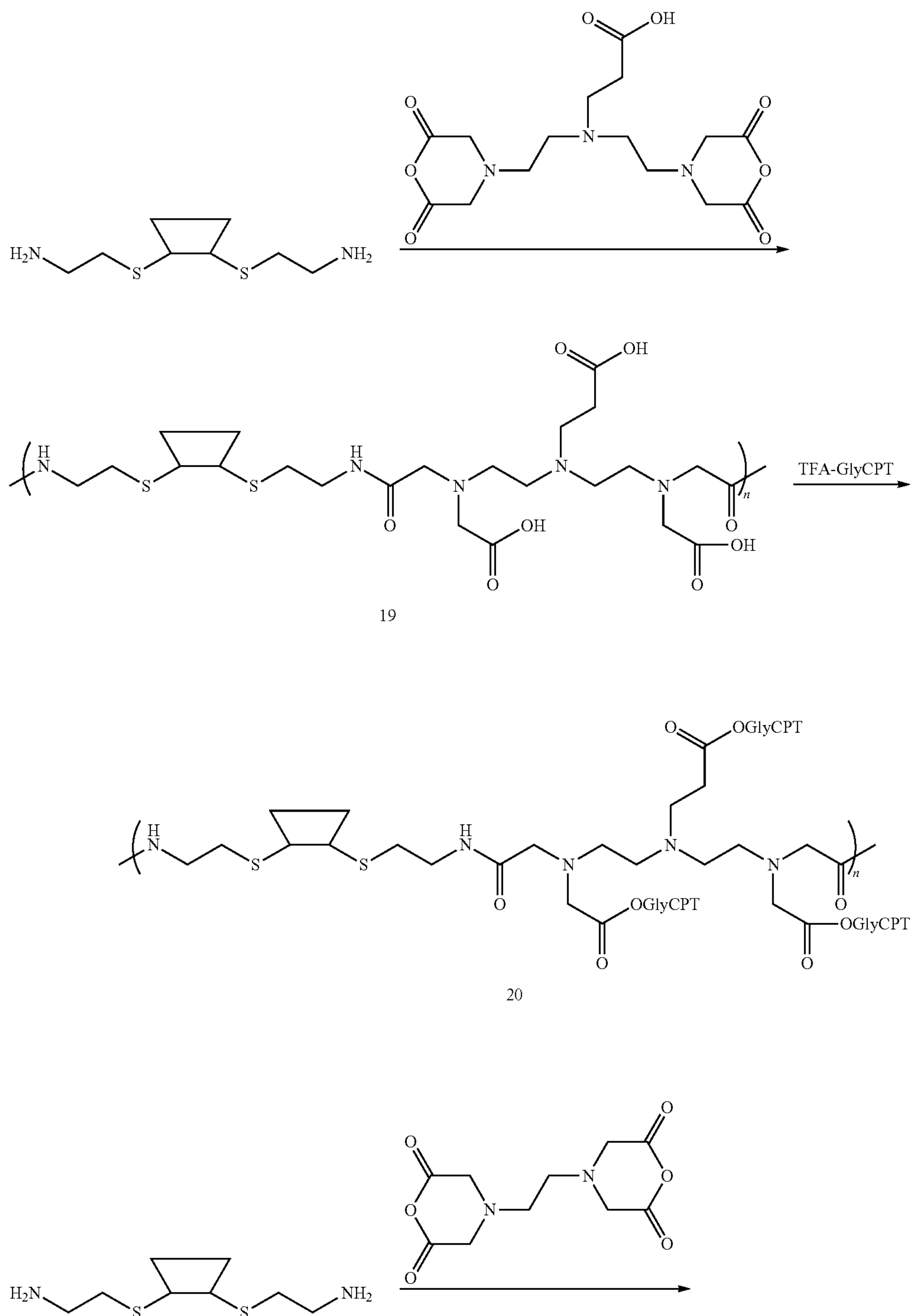
Scheme XXIX
