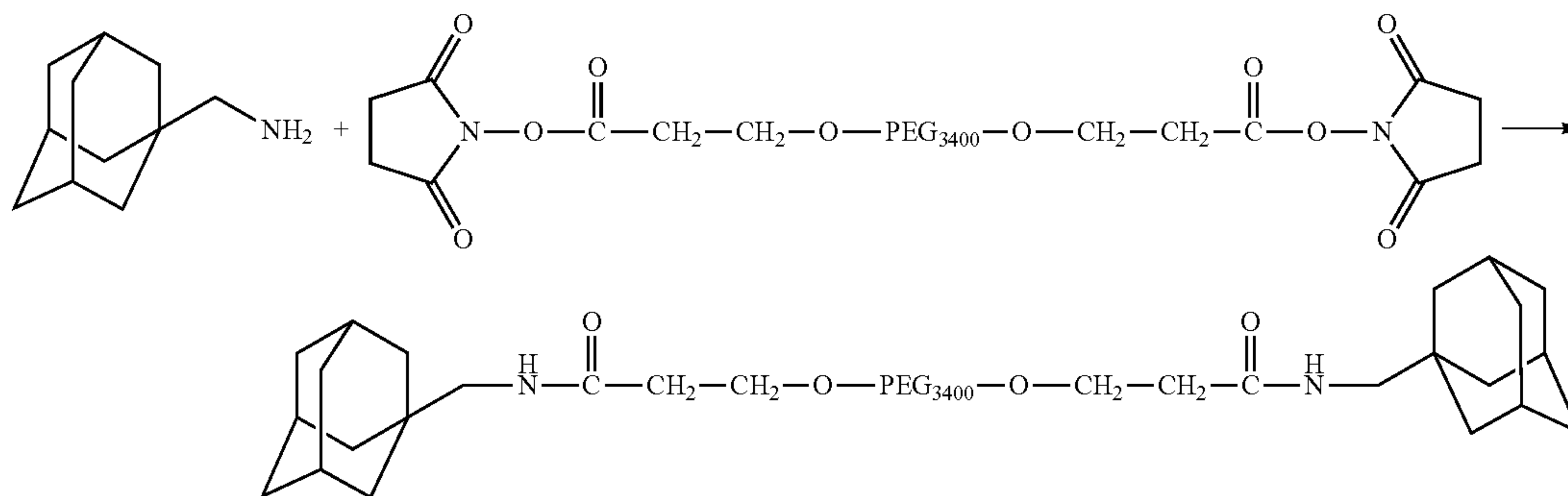
Scheme XXXXVI
