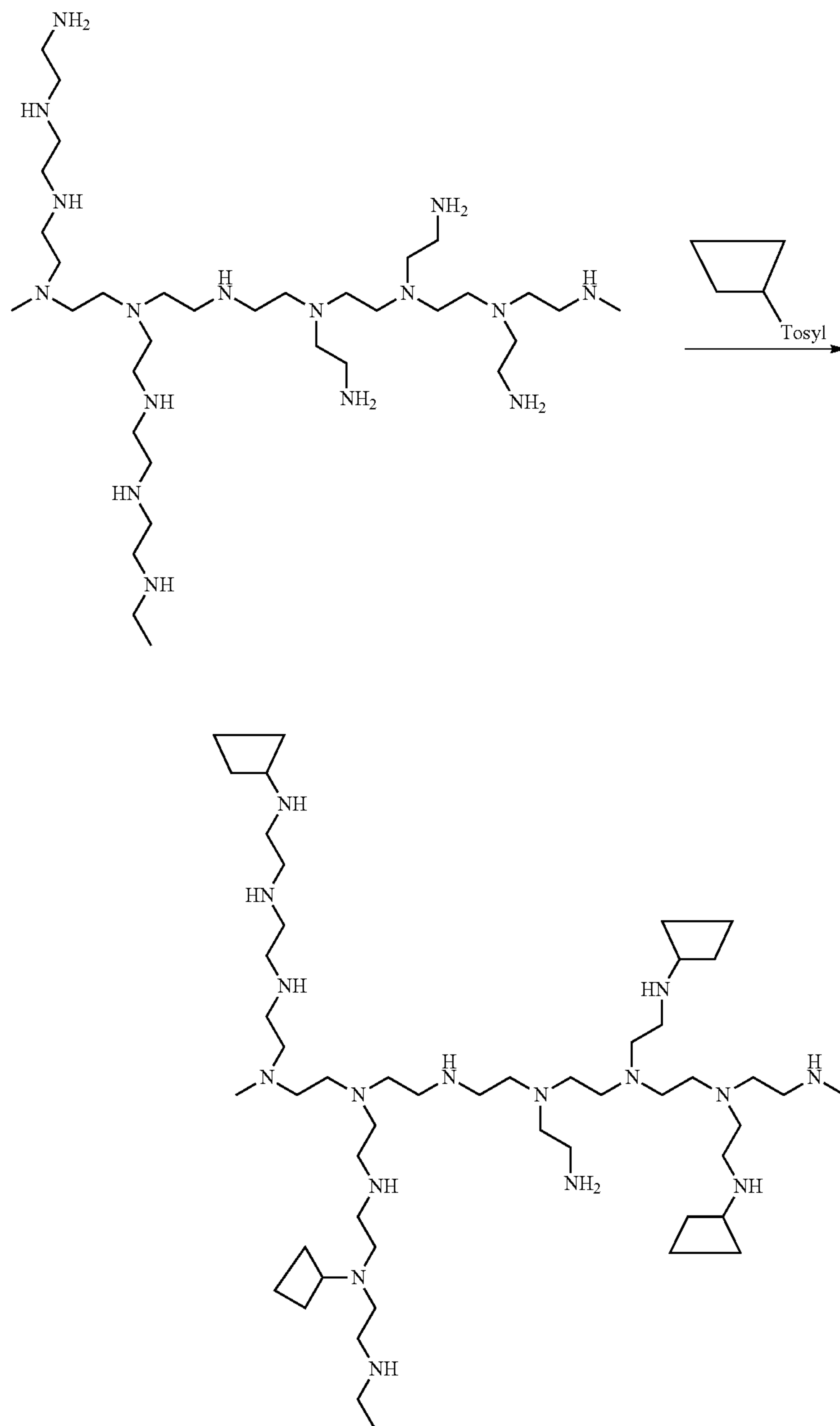
Scheme XXXXIV
