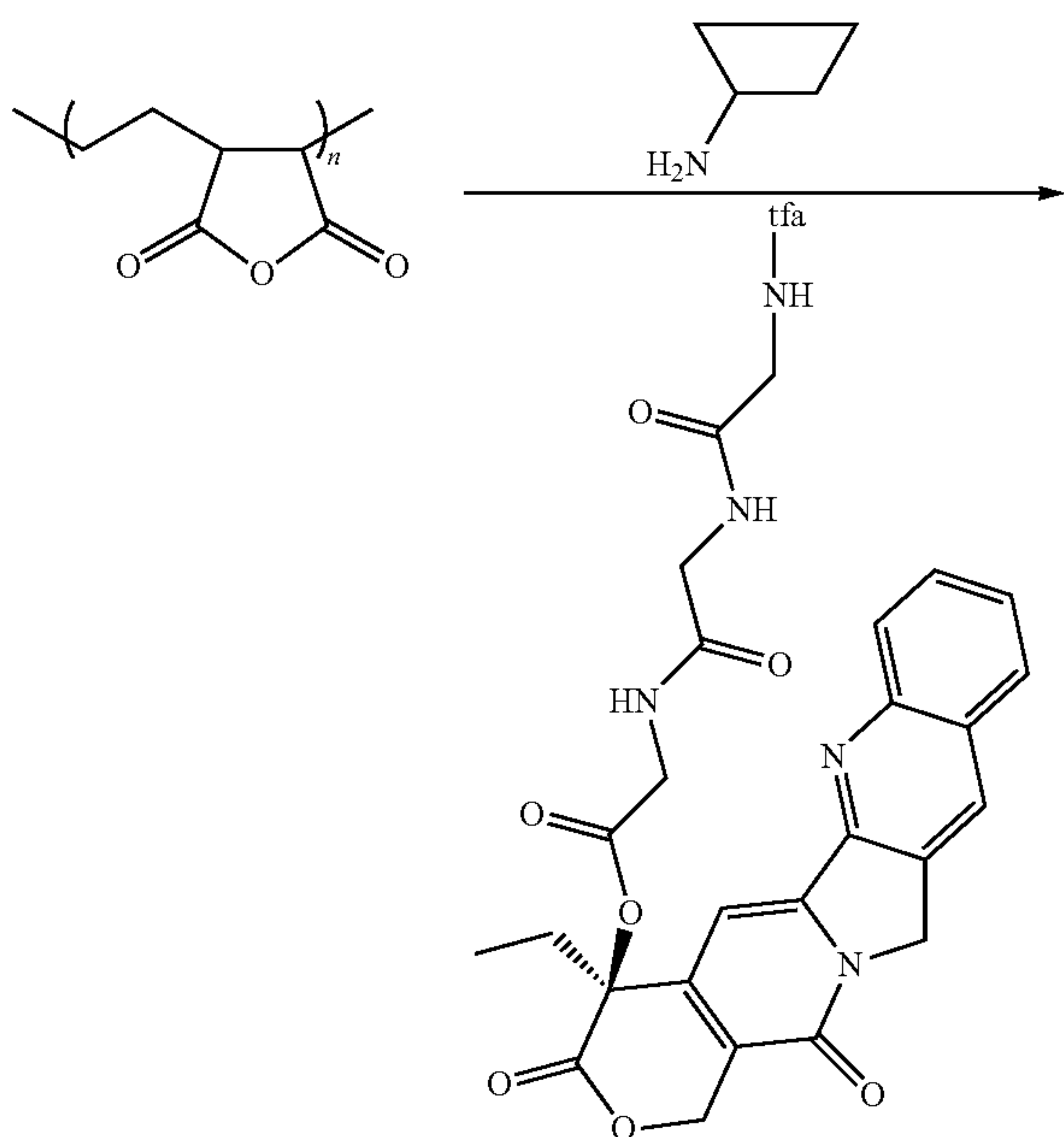
Scheme XXXVI
