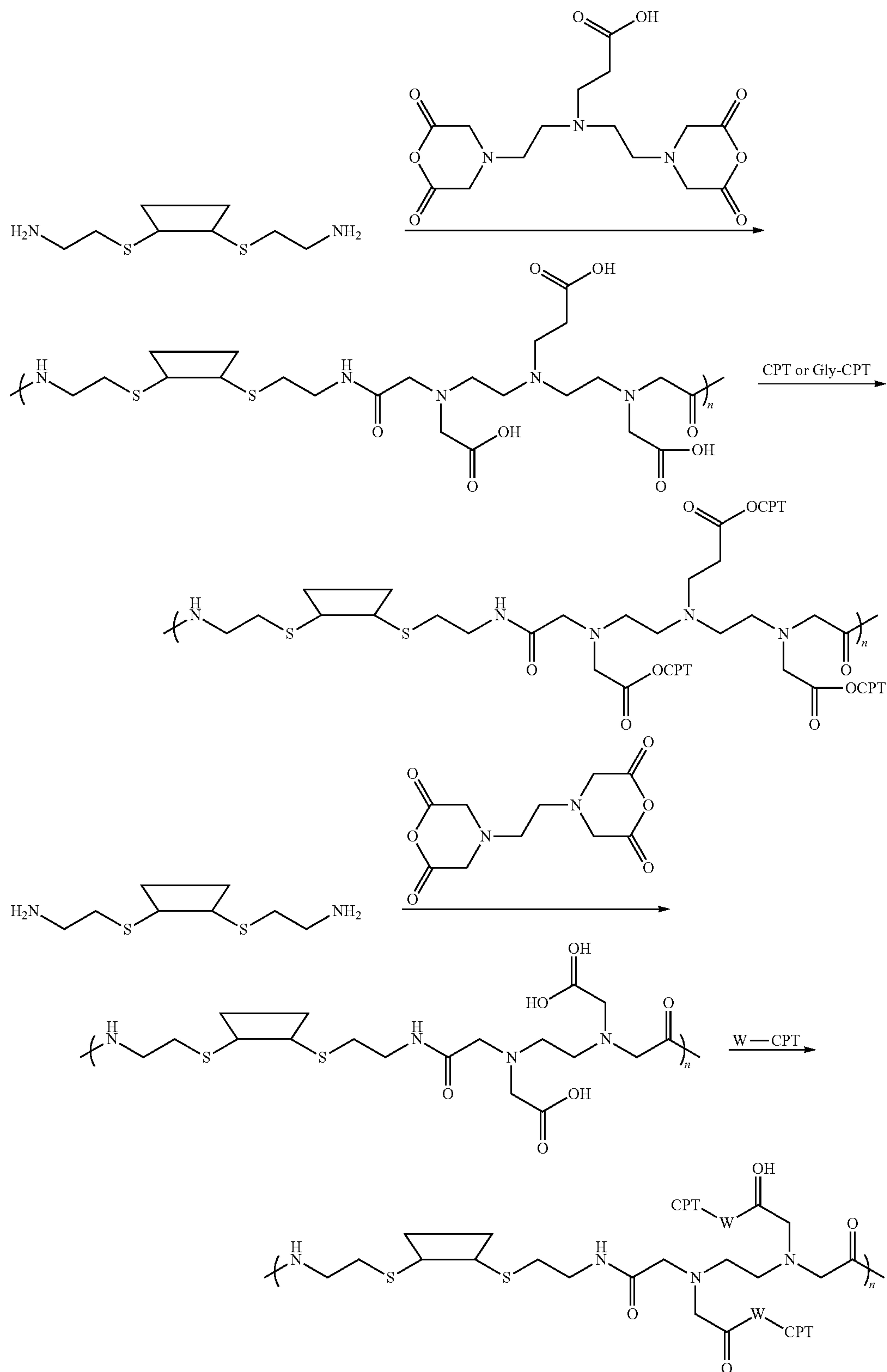
Scheme V
