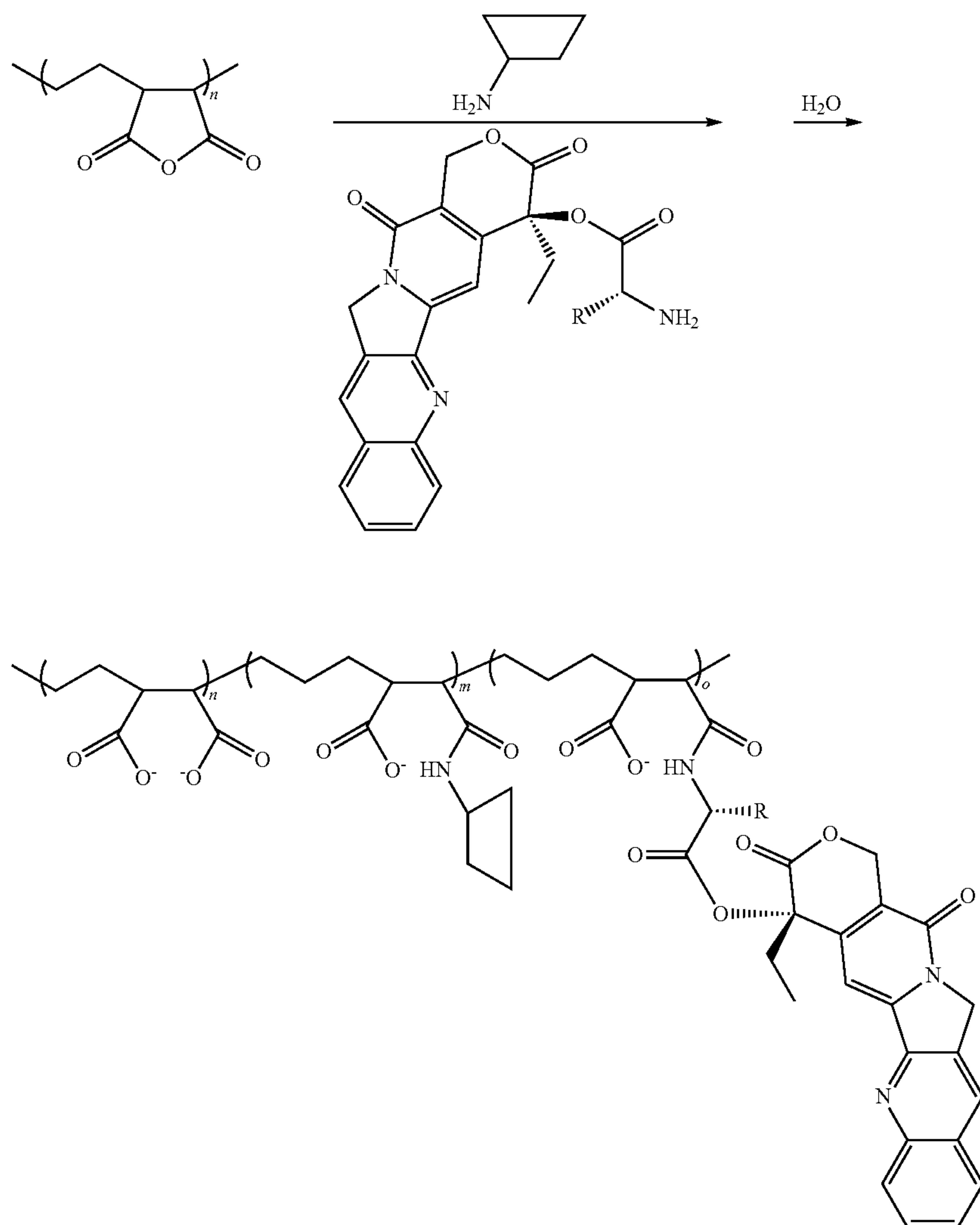
Scheme XI
