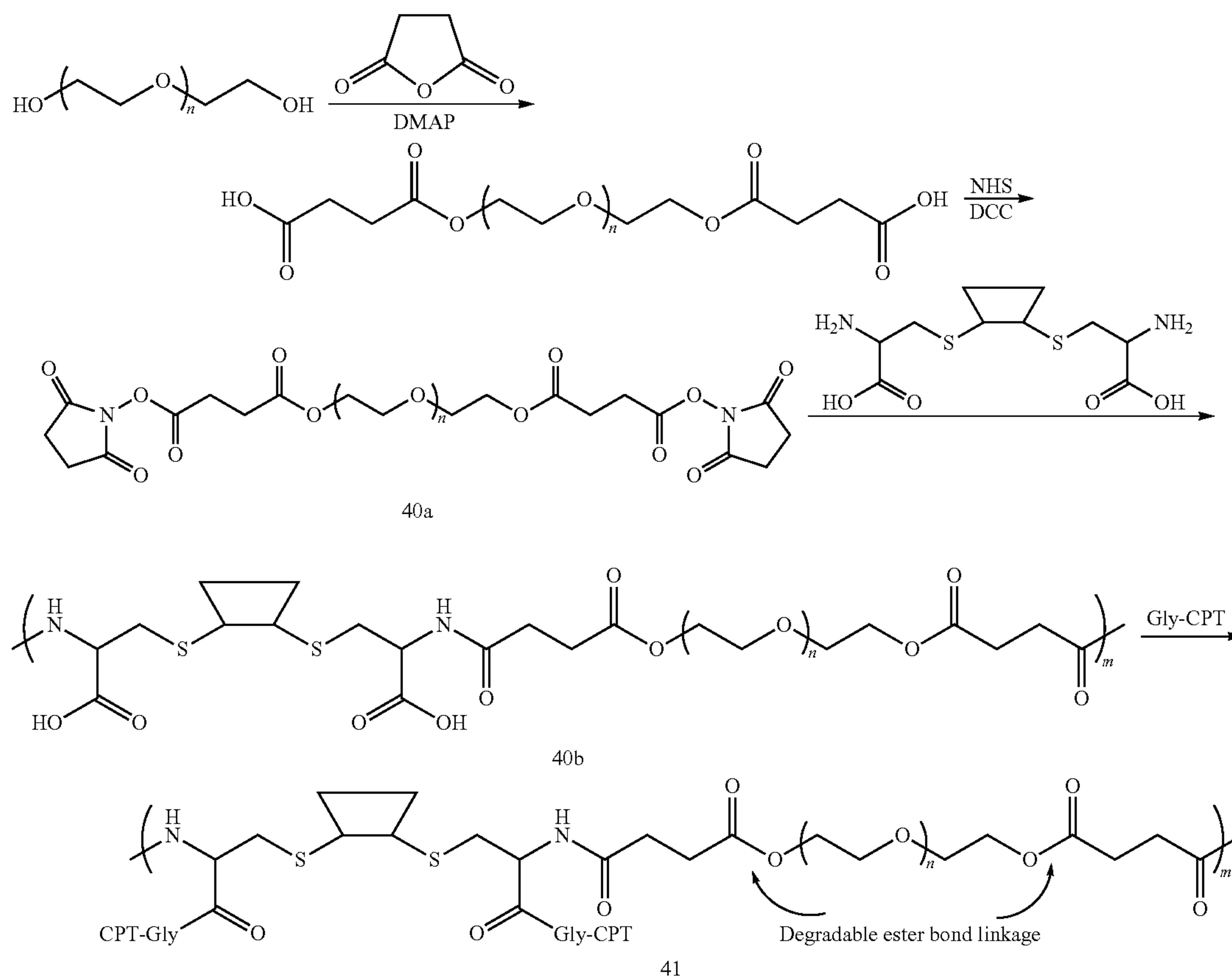
Scheme XXXXI
