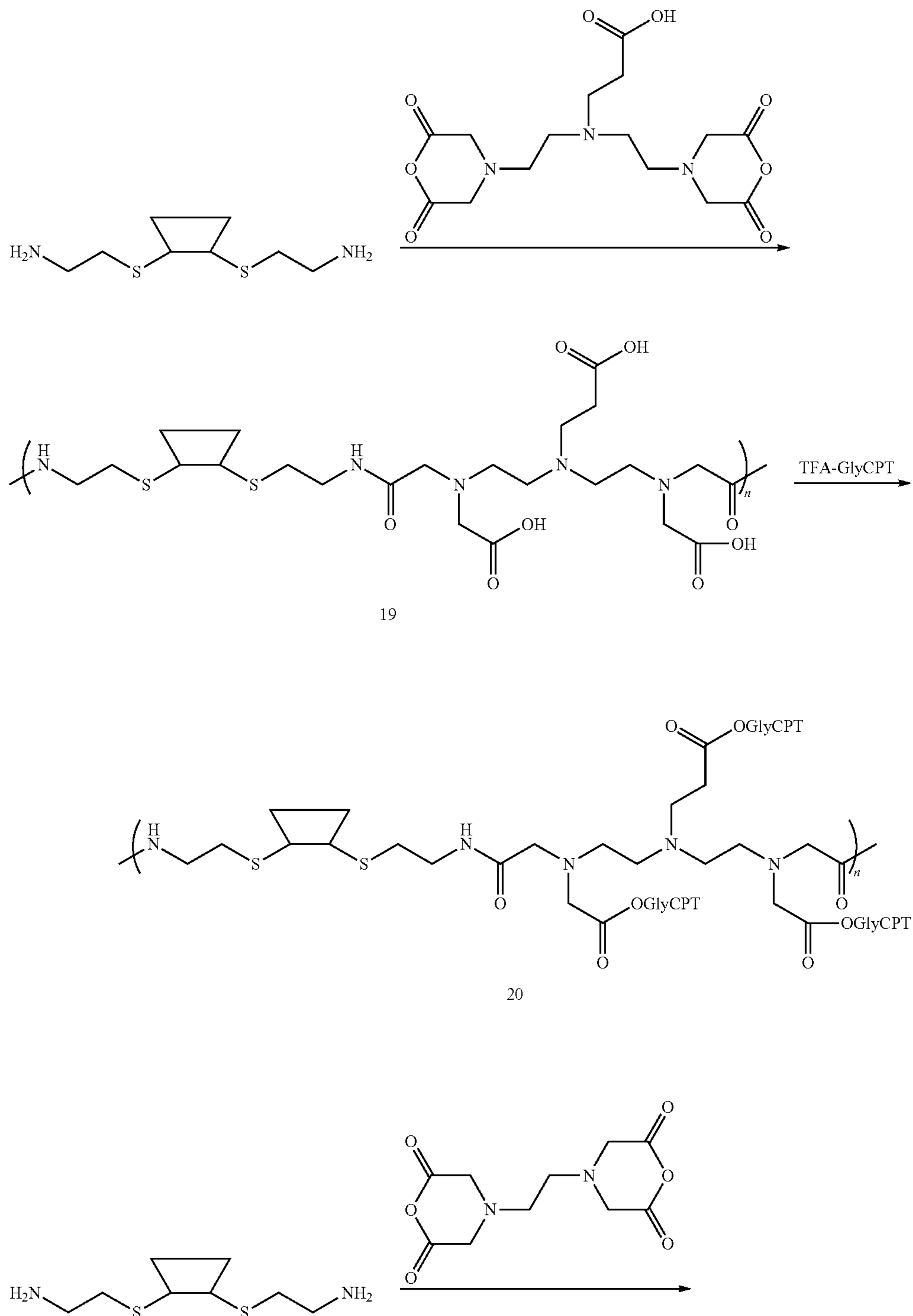
Scheme XXIX
