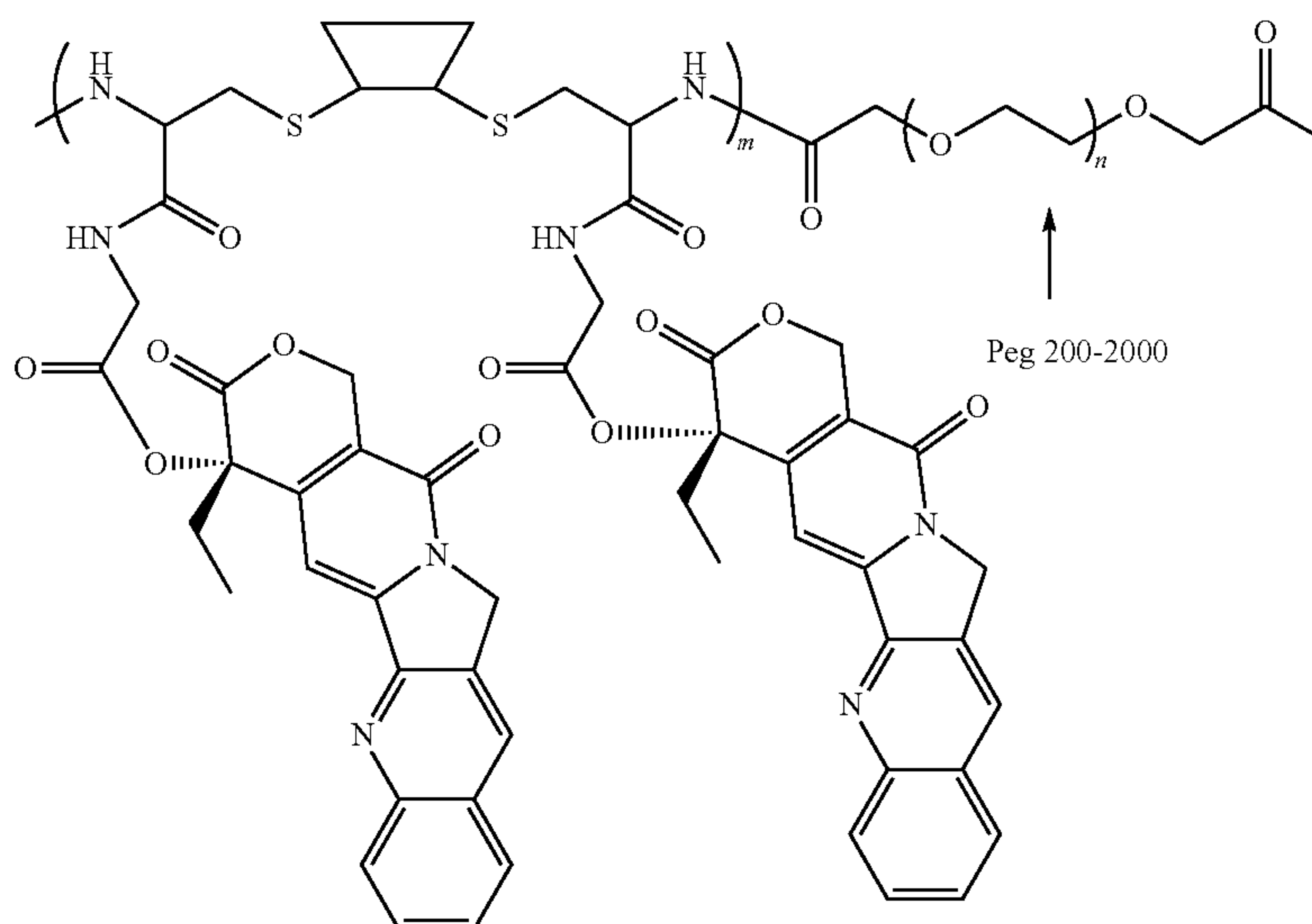
Scheme XXXXII
