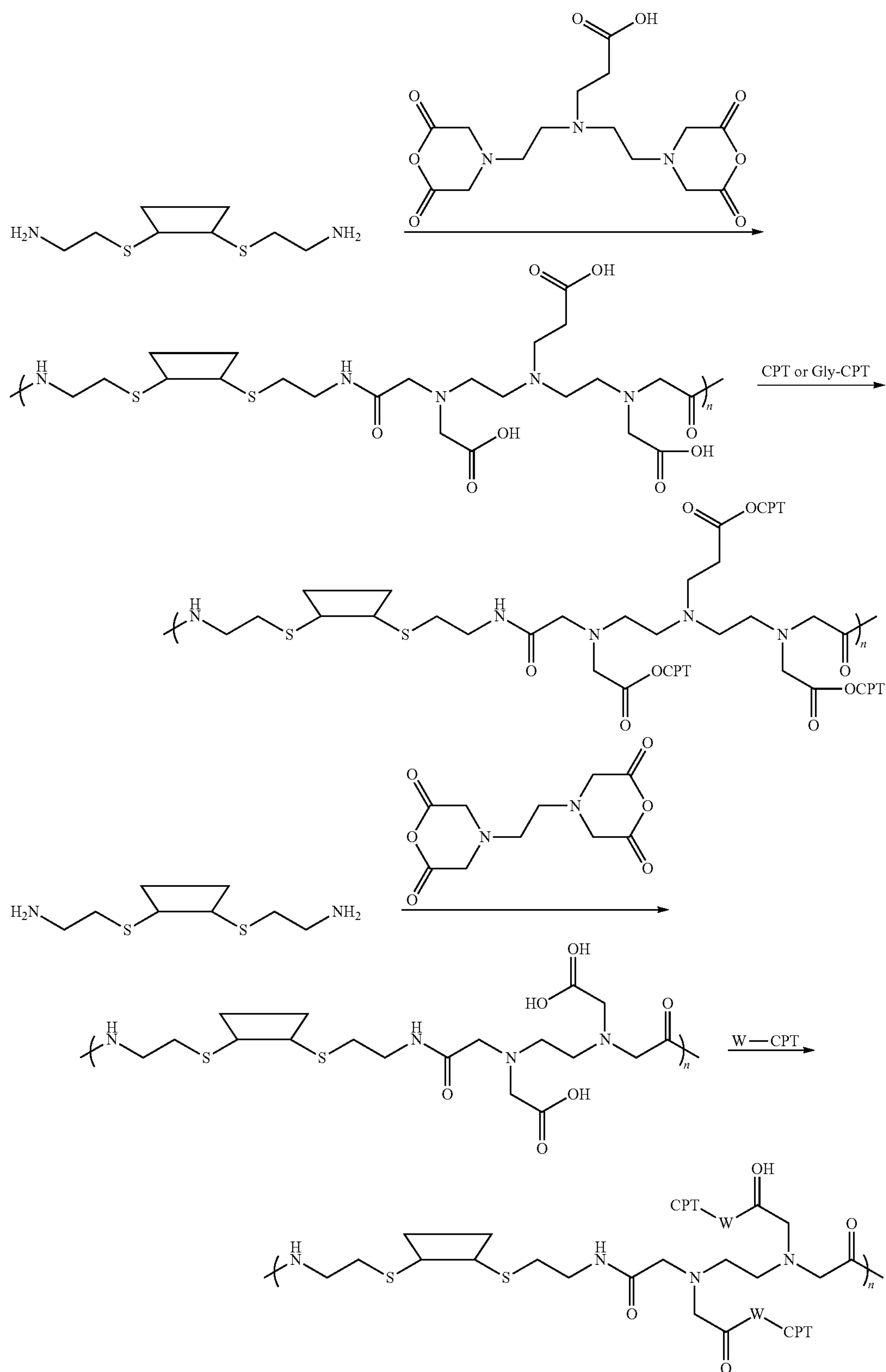
Scheme V
