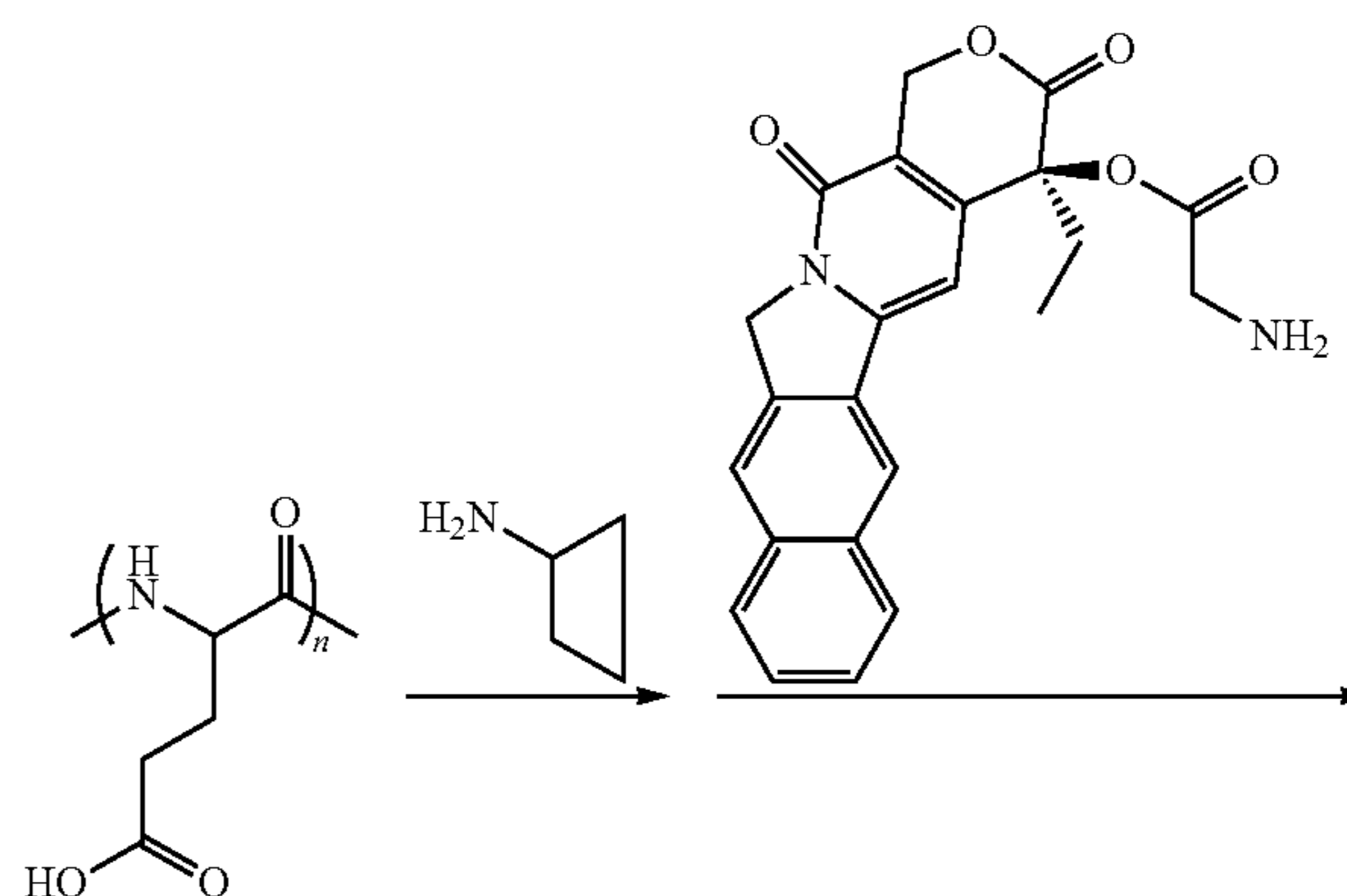
Scheme XXXVII
