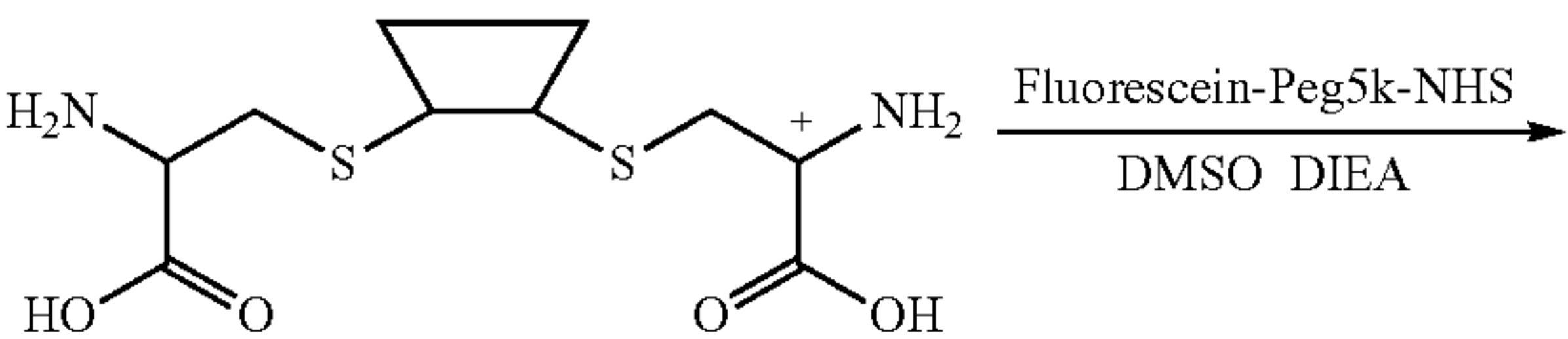
Scheme XXXX
