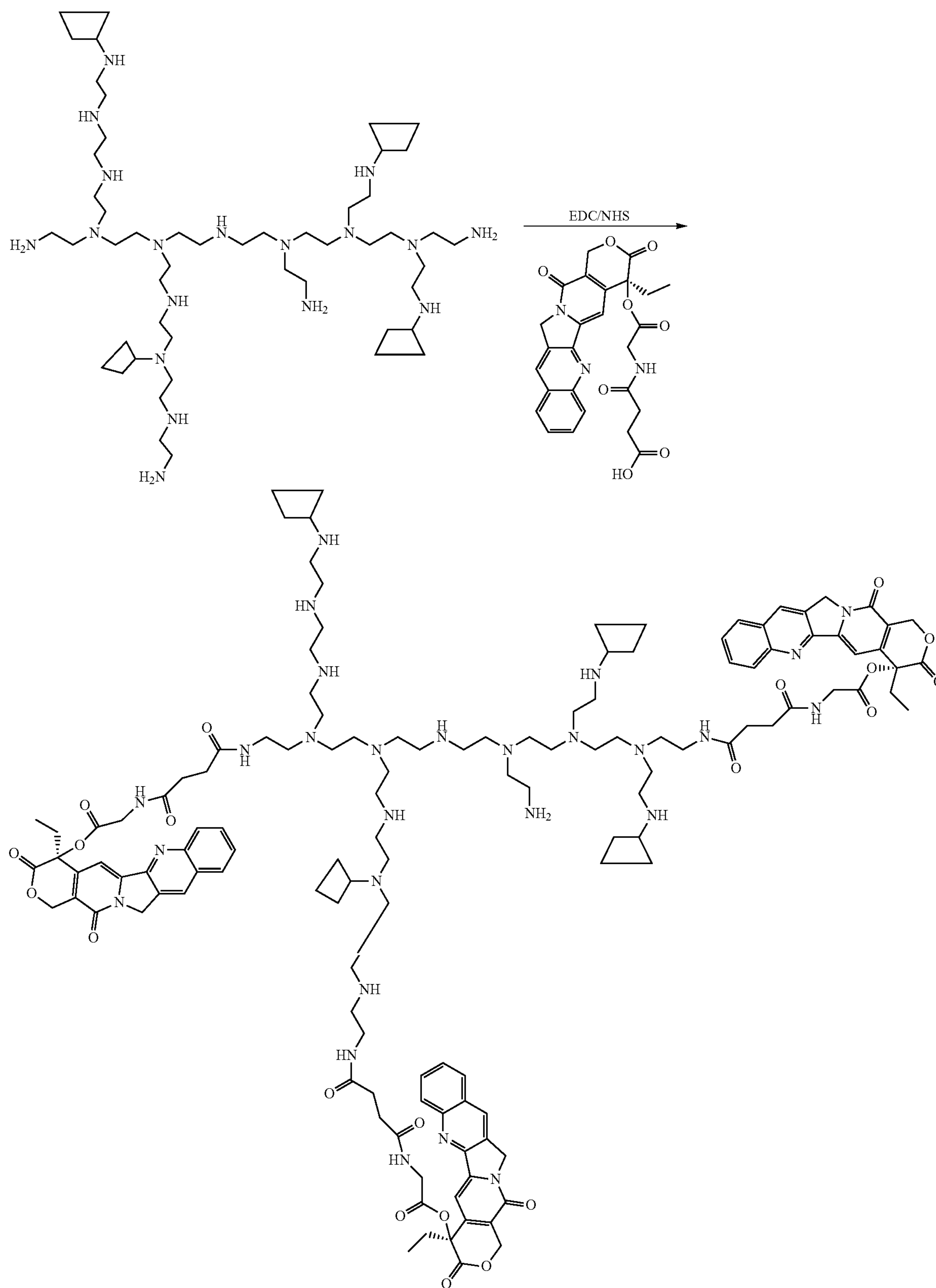
Scheme XXXXV
