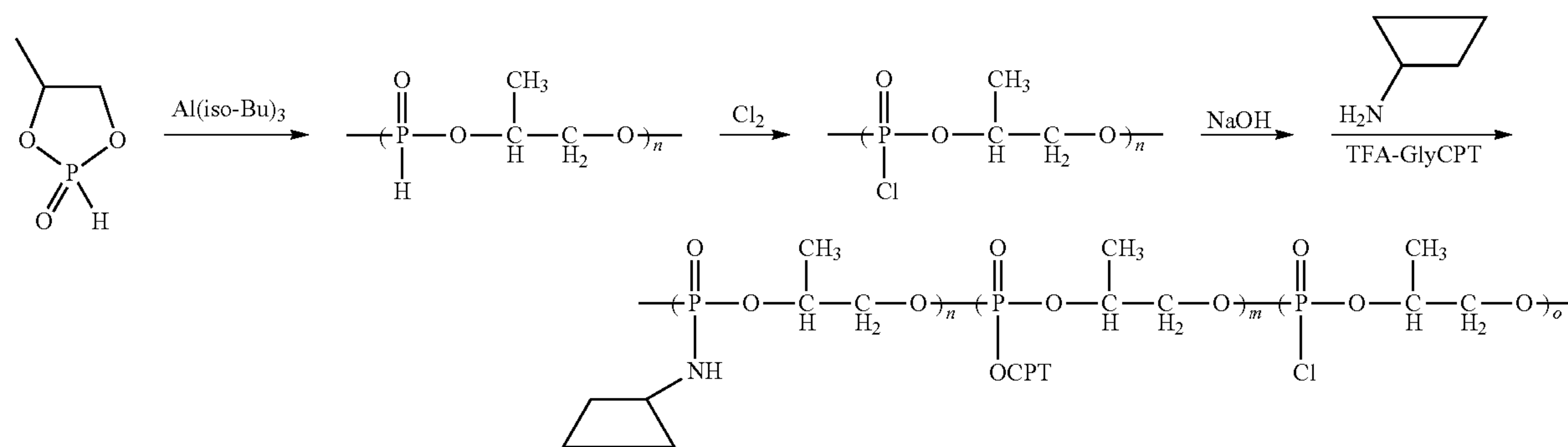
Scheme XXXIV
