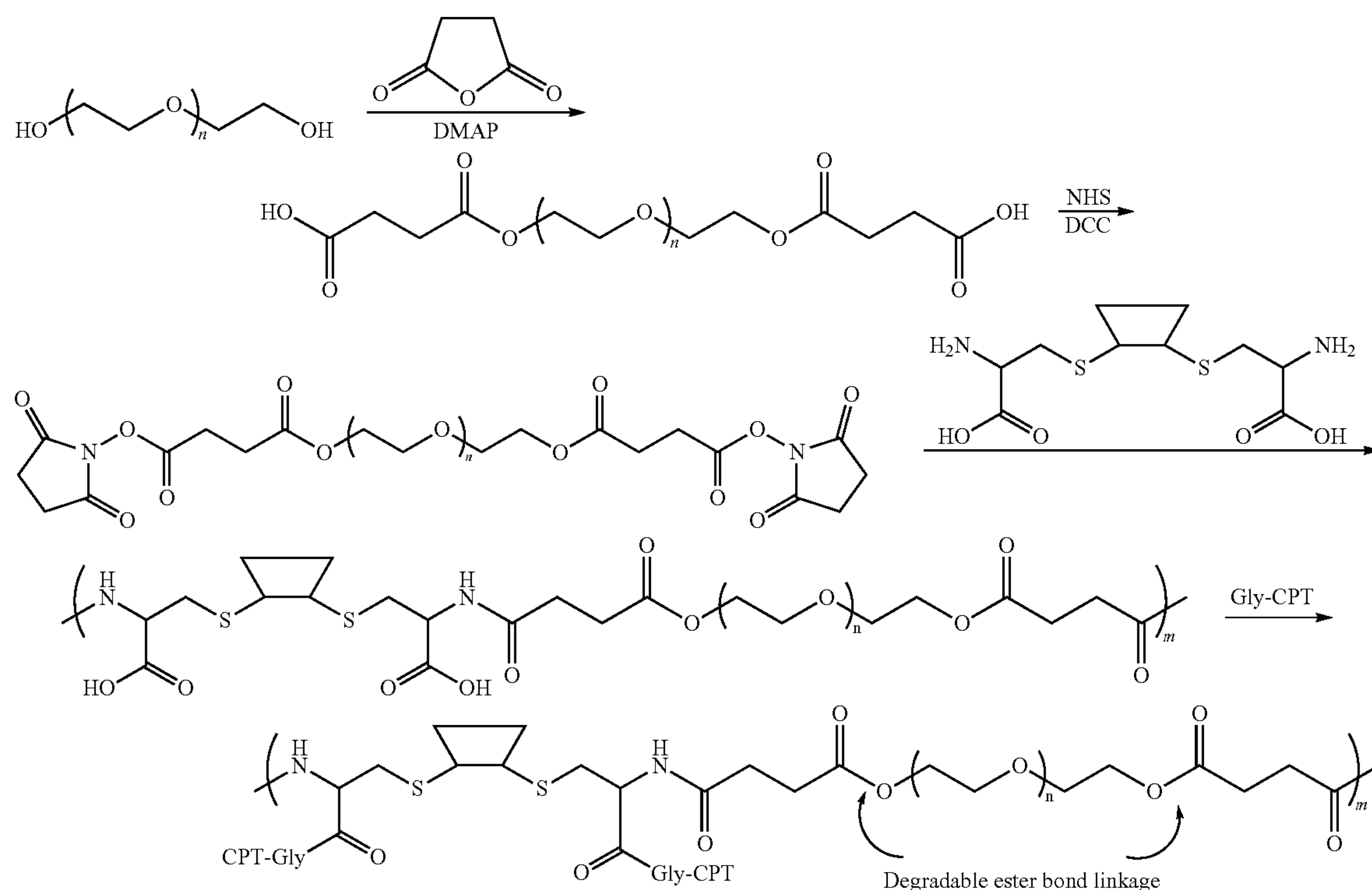
Scheme XIV
