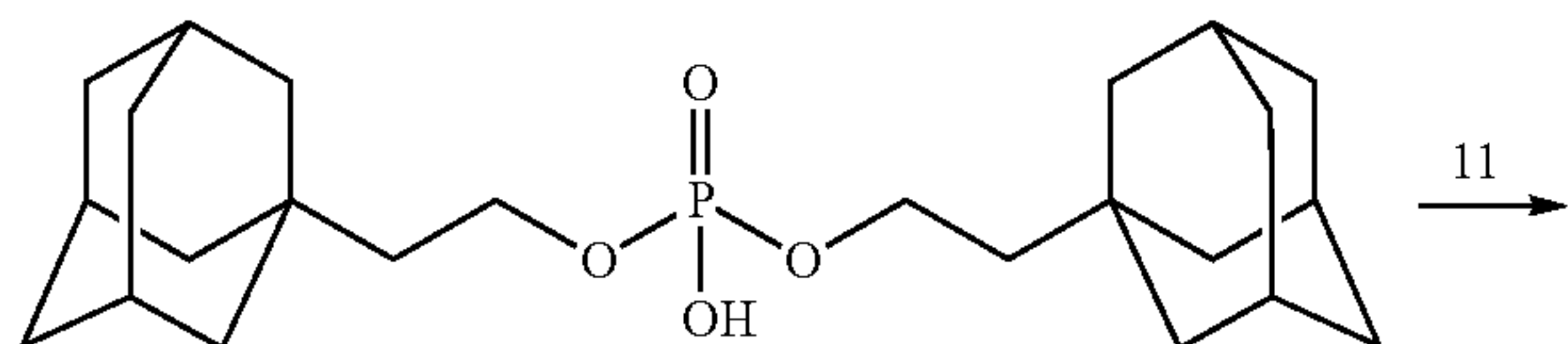
Scheme XXXXVIII
