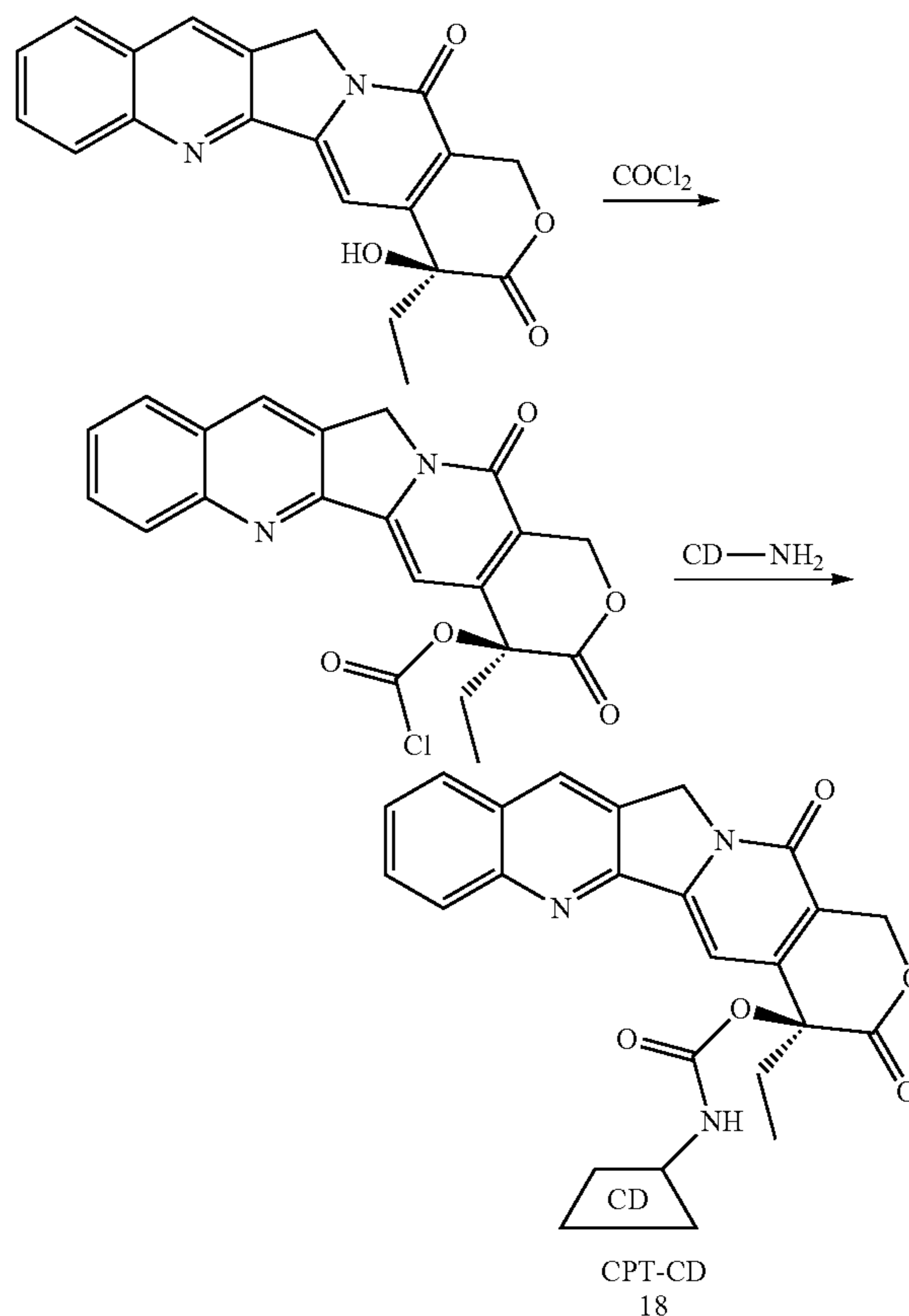
Scheme XXVIII
