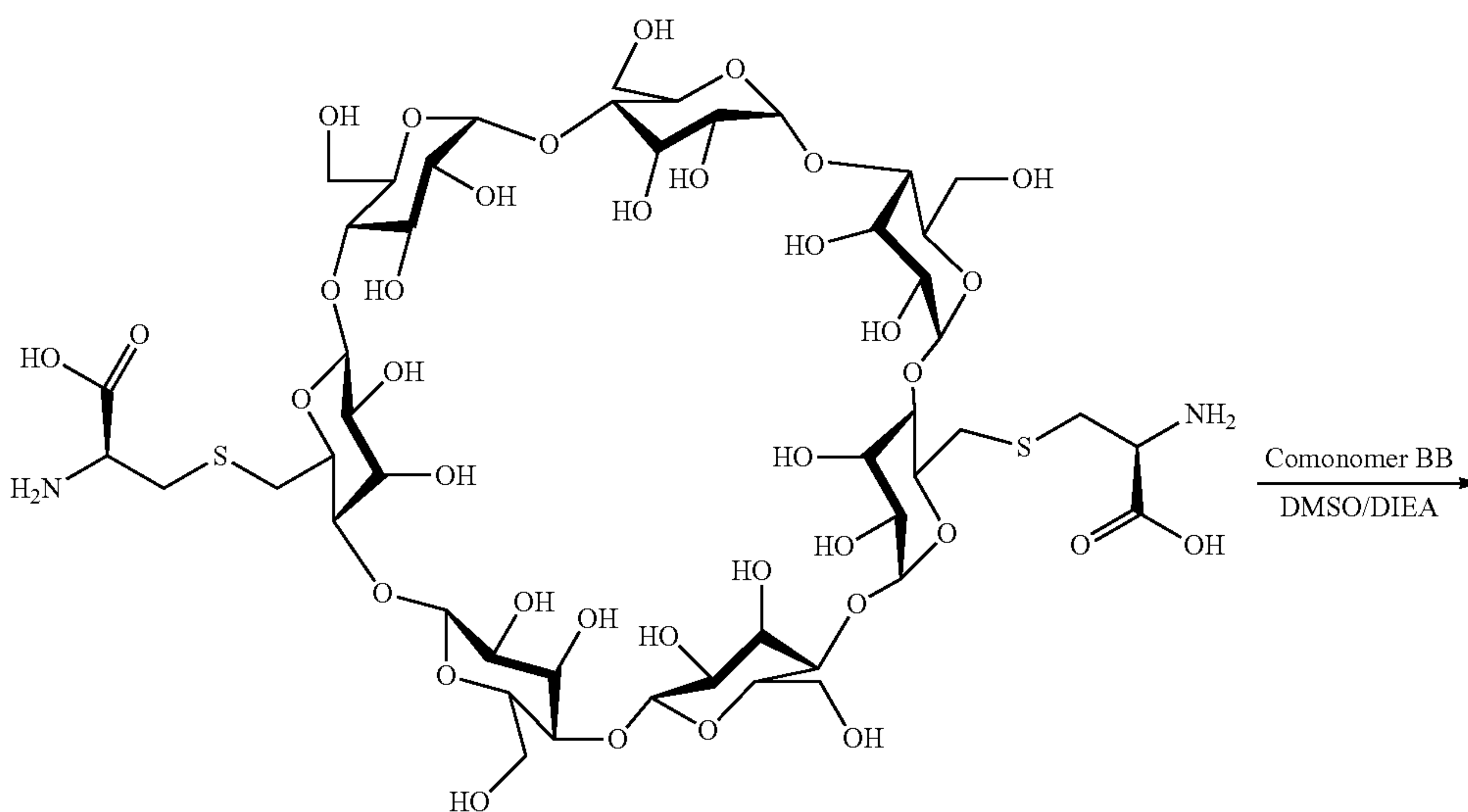
Scheme XXXVIIIb
