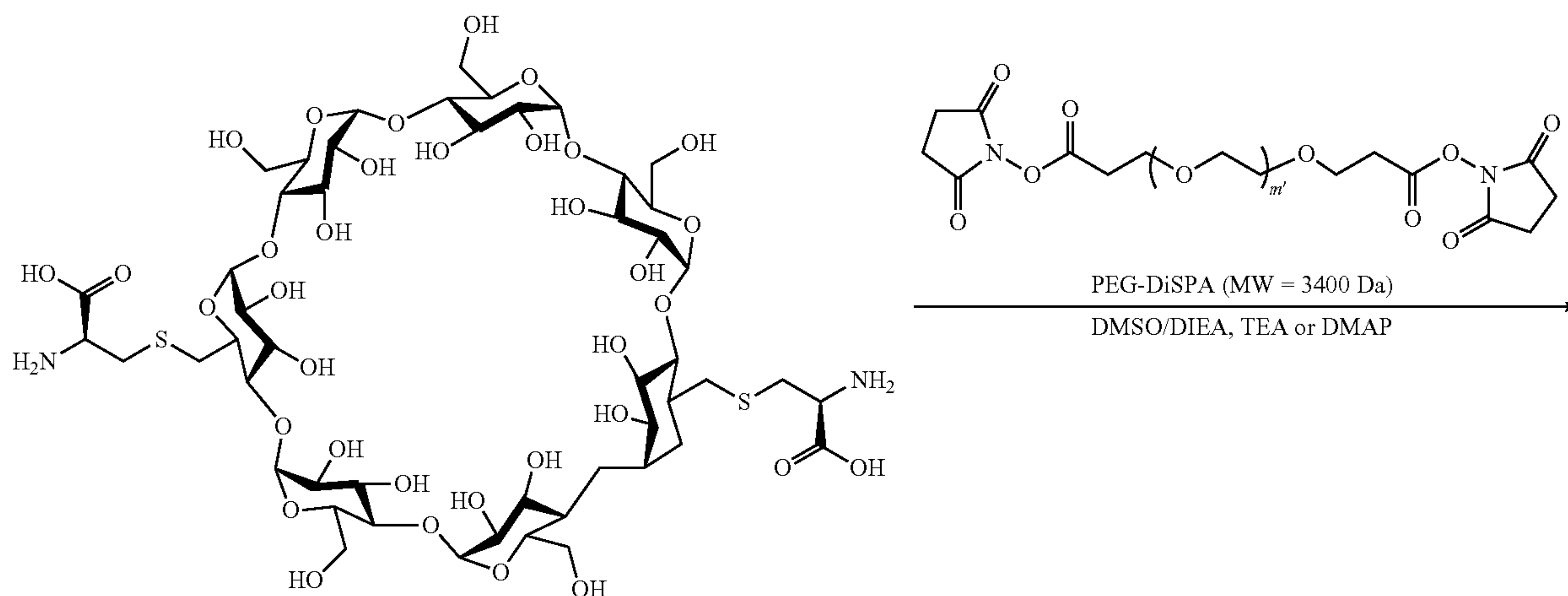
Scheme XXXVIIIa
