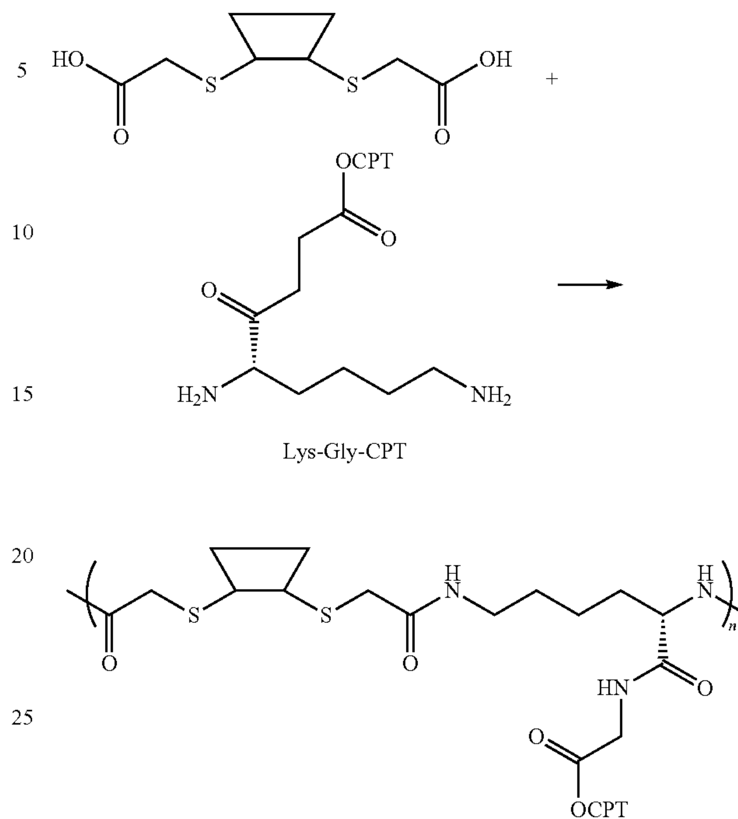
Scheme VIII
