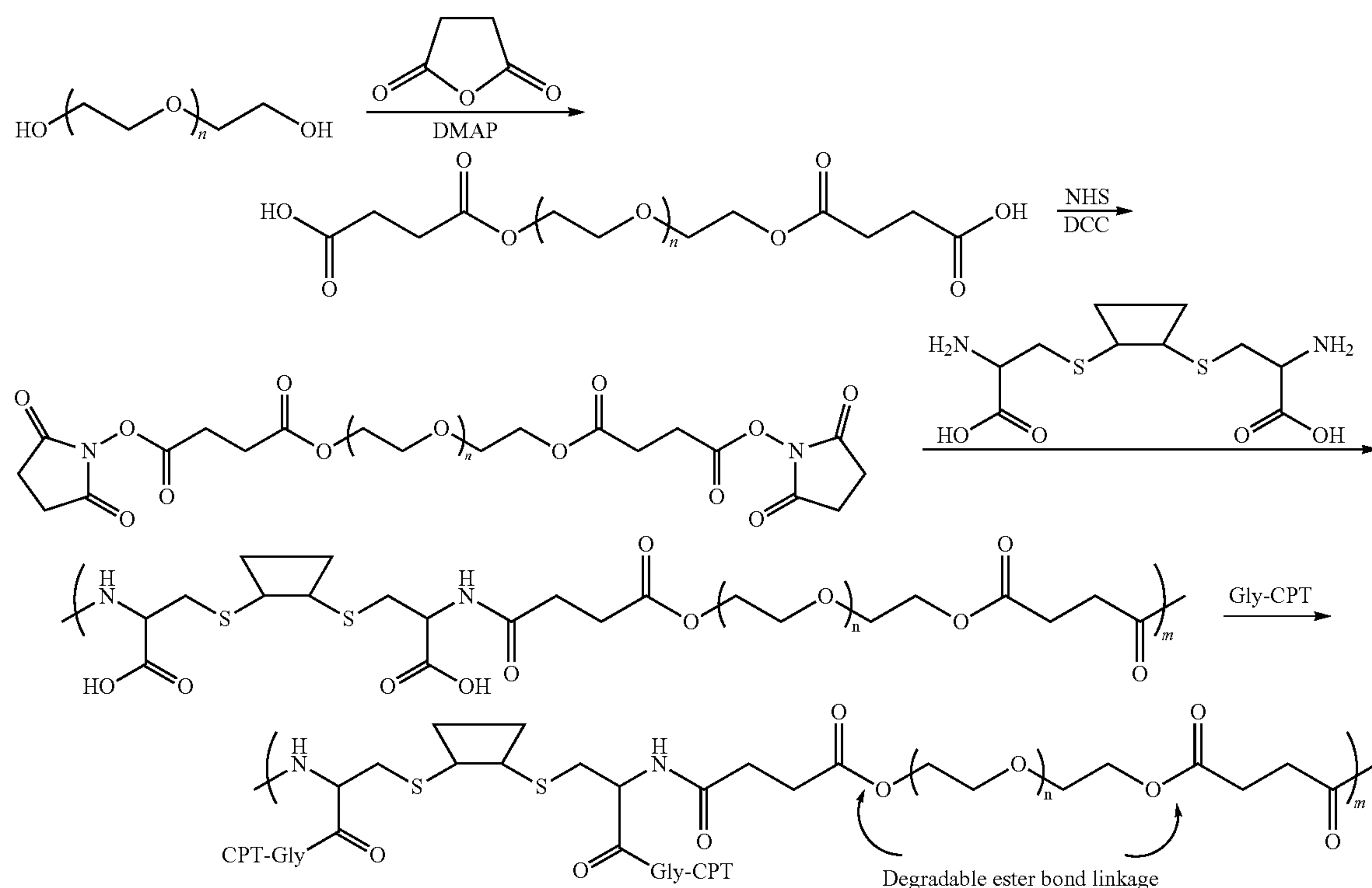
Scheme XIV
