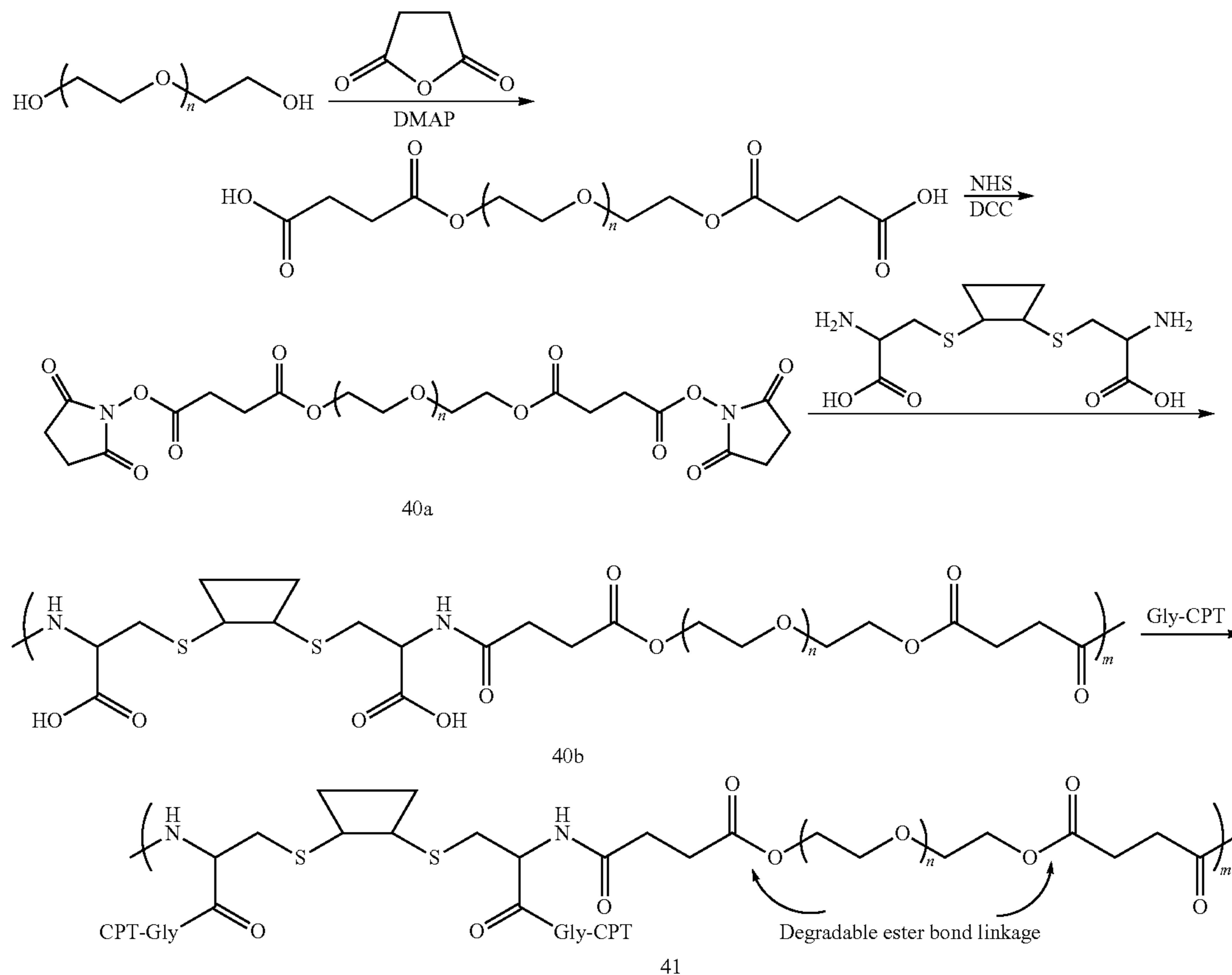
Scheme XXXXI
