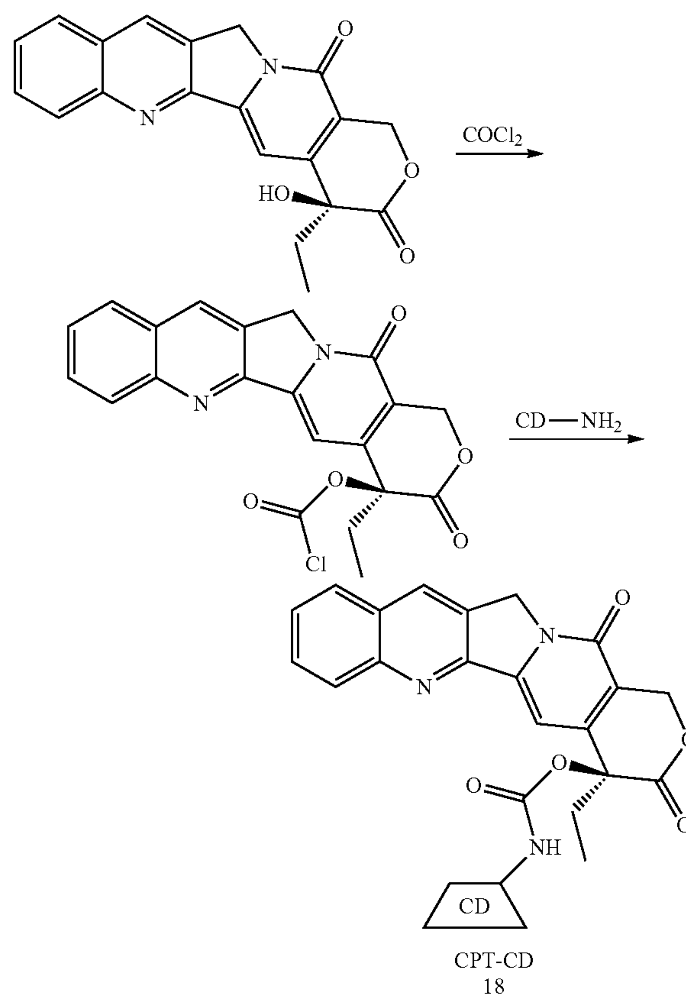
Scheme XXVIII
