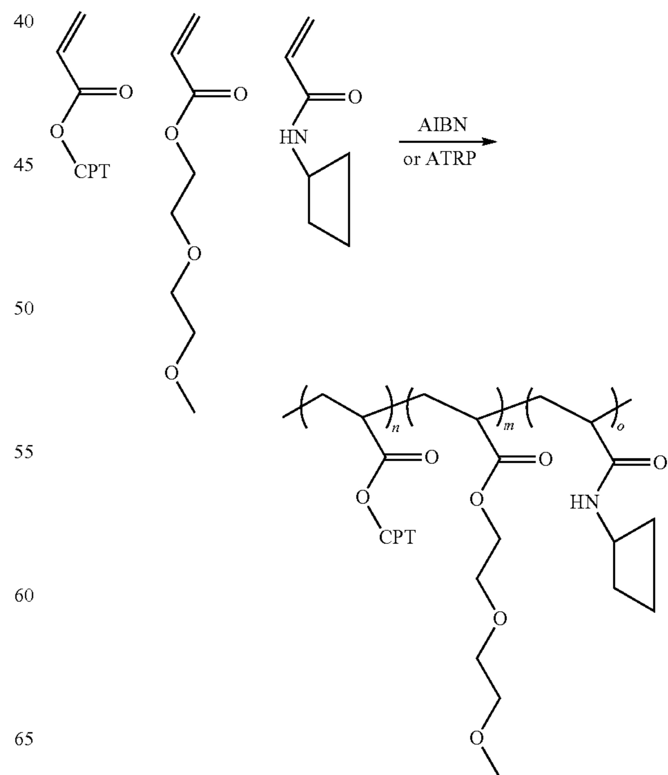
Scheme X
