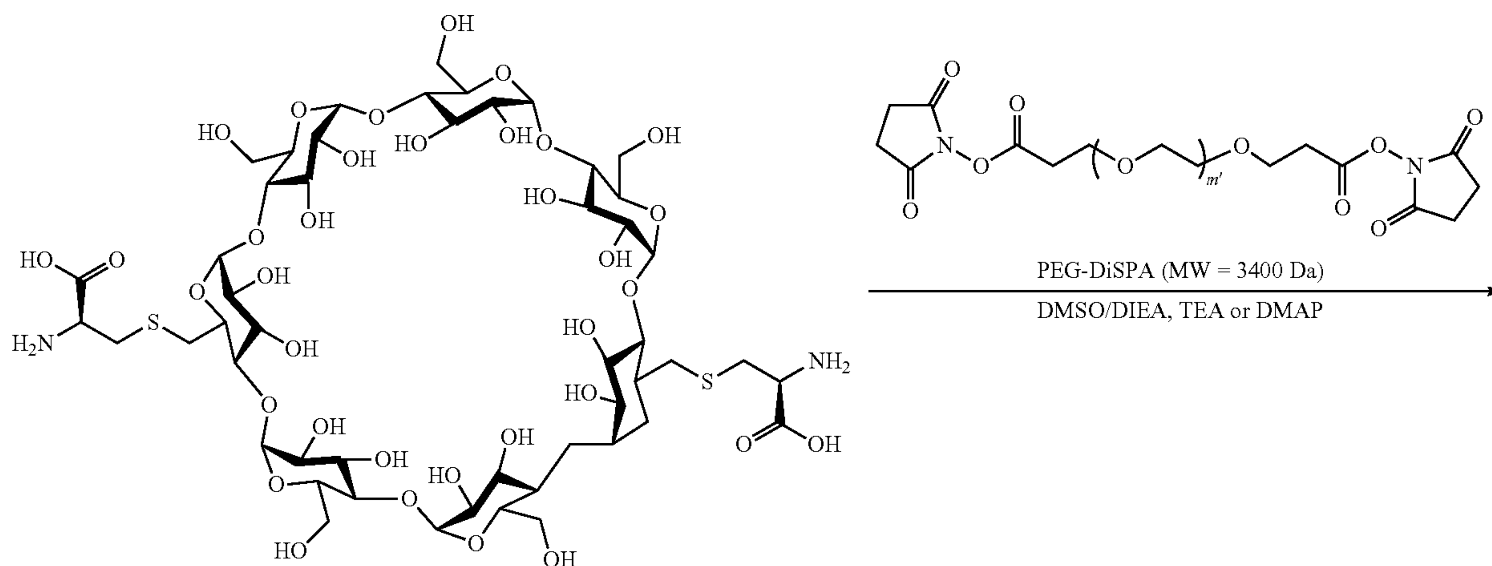
Scheme XXXVIIIa
