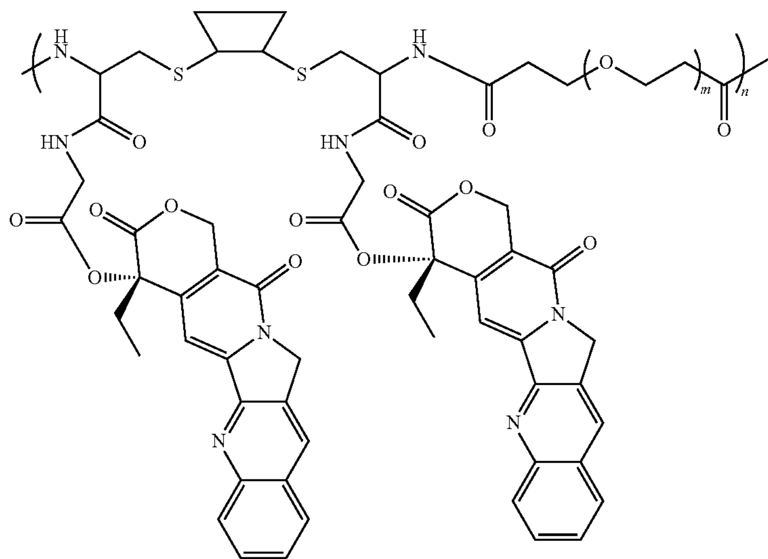
Scheme XXXXIII
