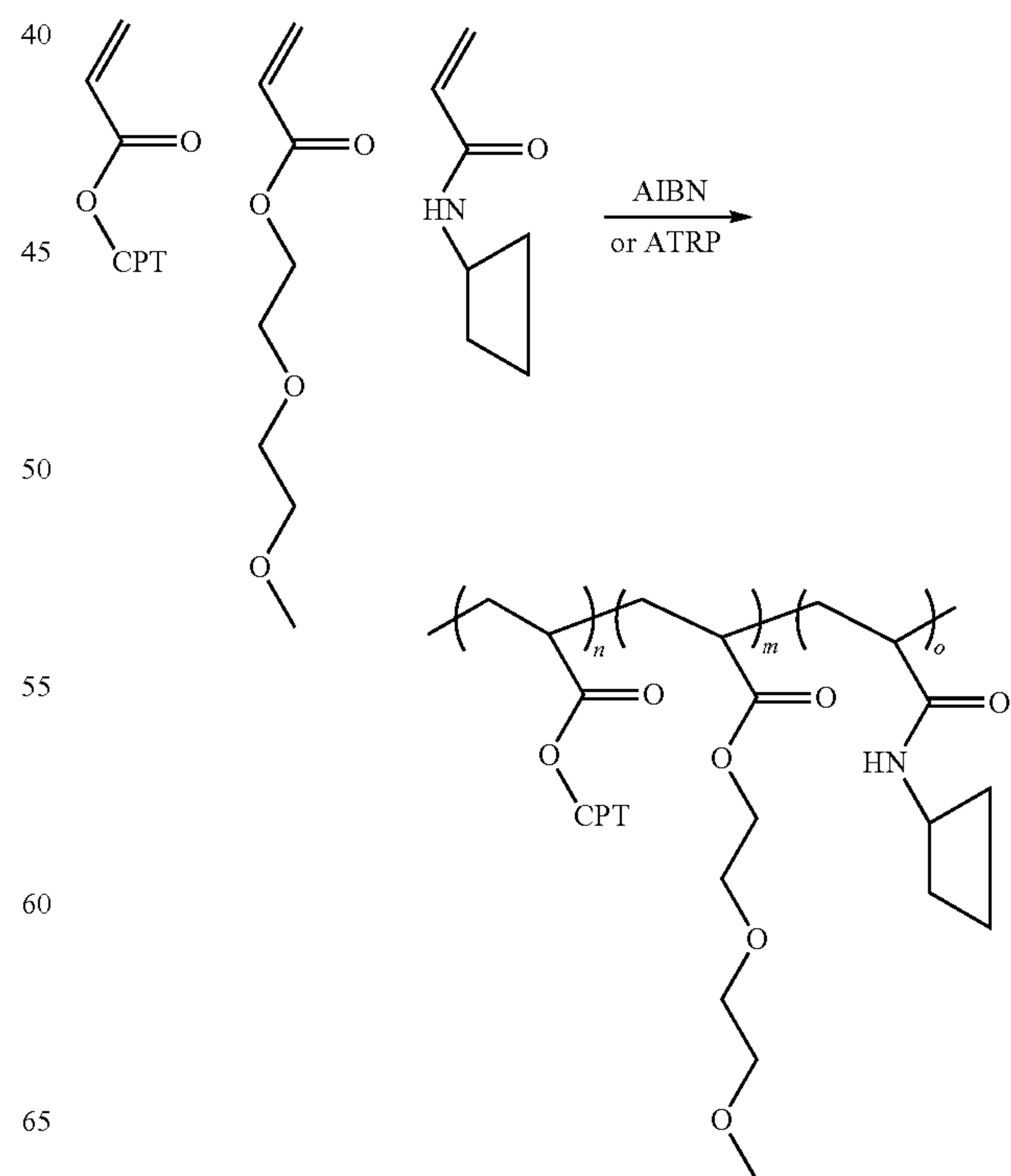
Scheme X
