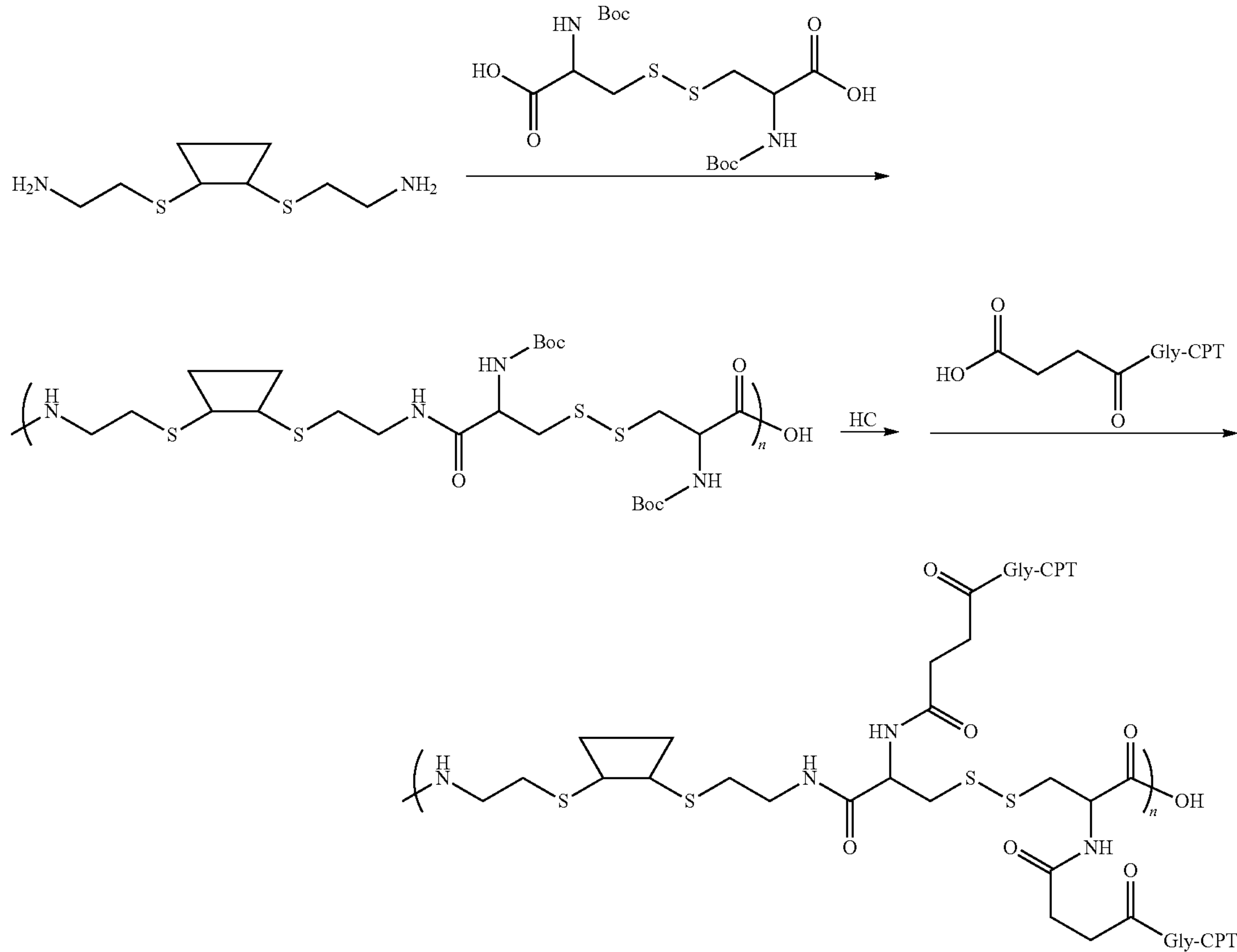
Scheme VII
