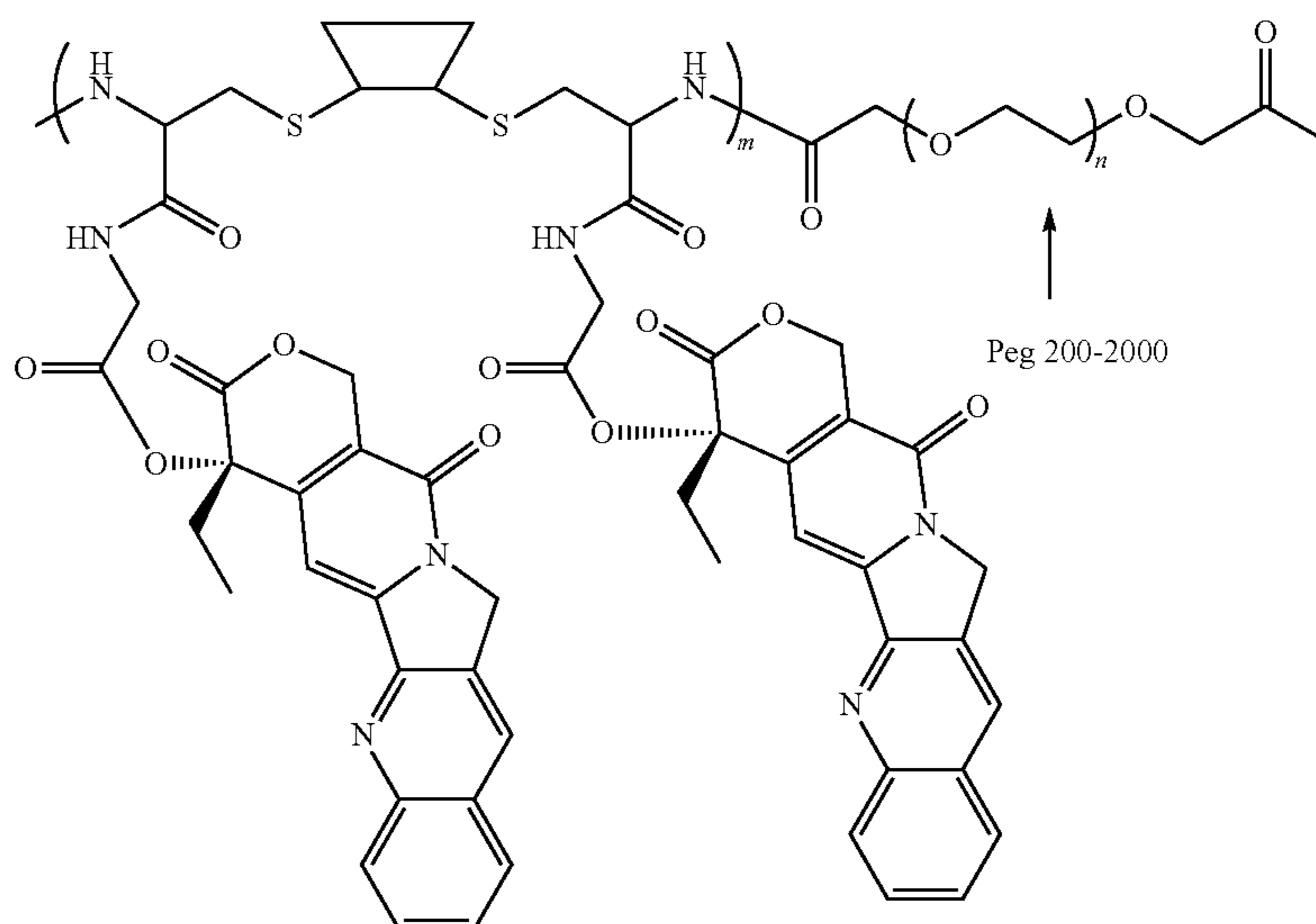
Scheme XXXXII
