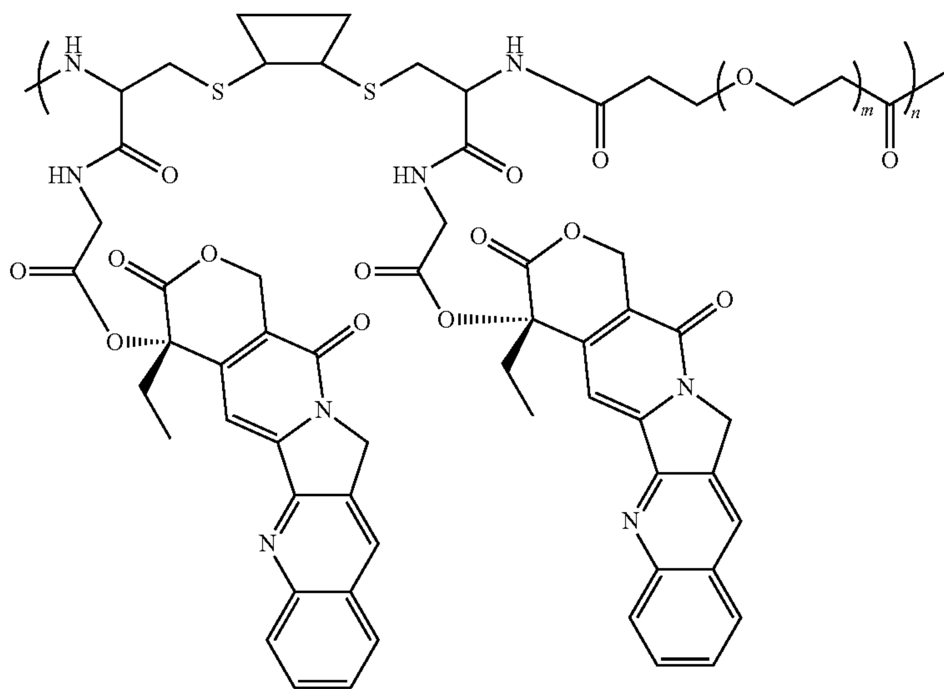
Scheme XXXXIII
