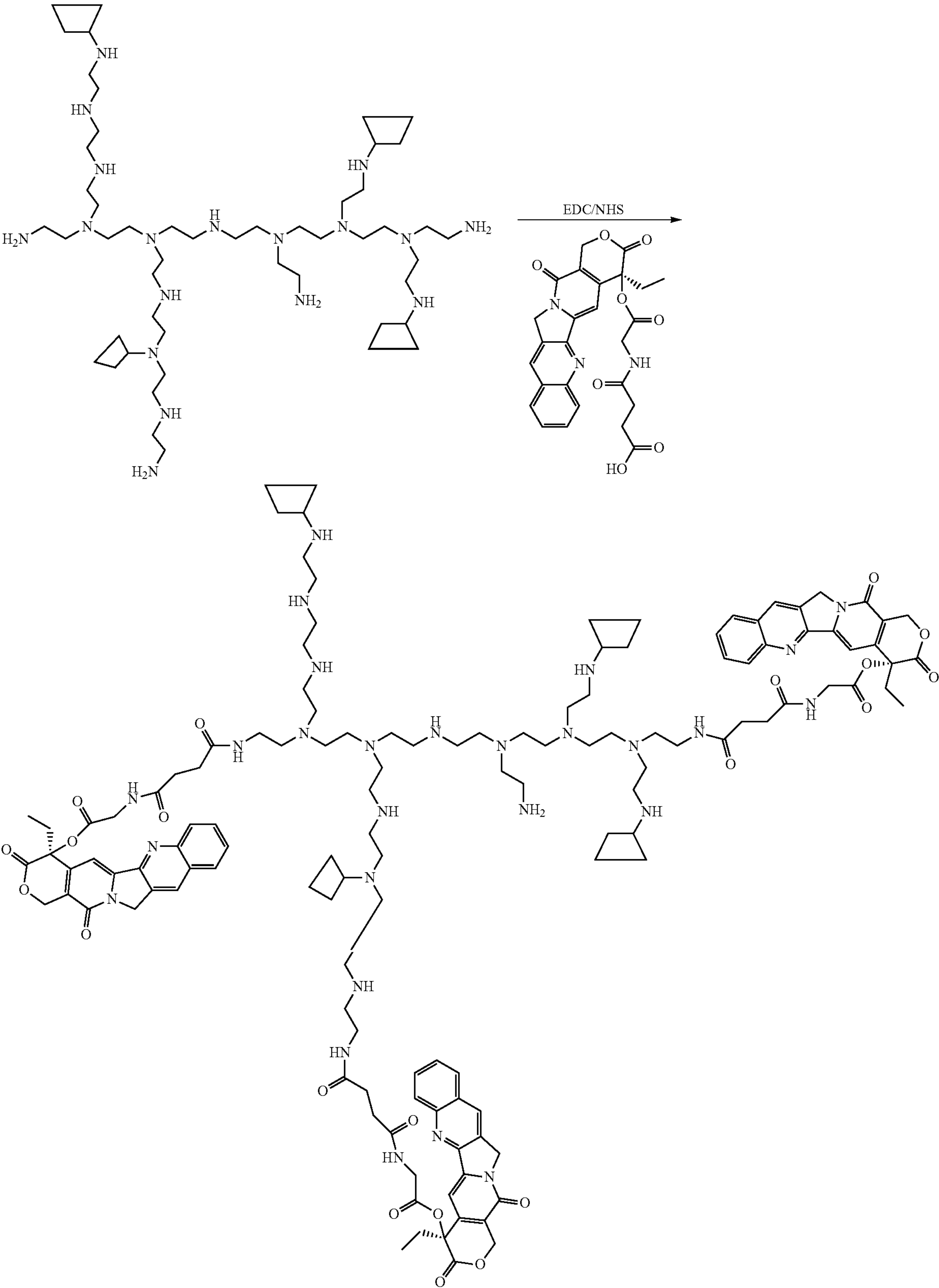
Scheme XXXXV
