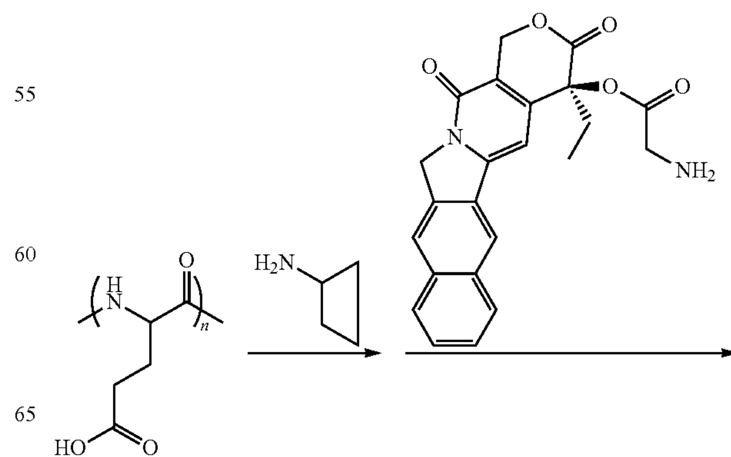
Scheme XXXVII
