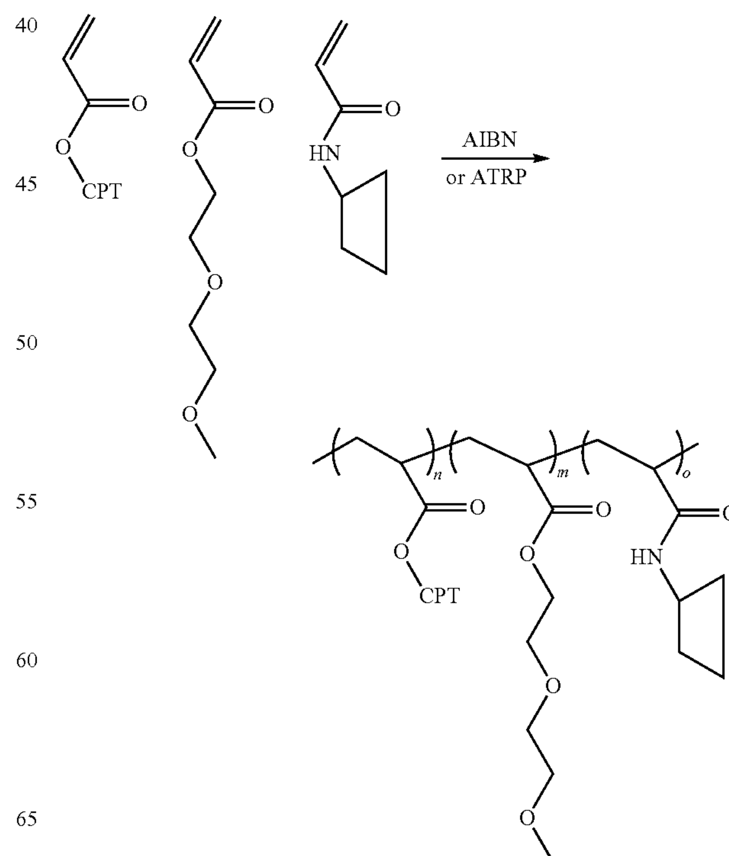
Scheme X
