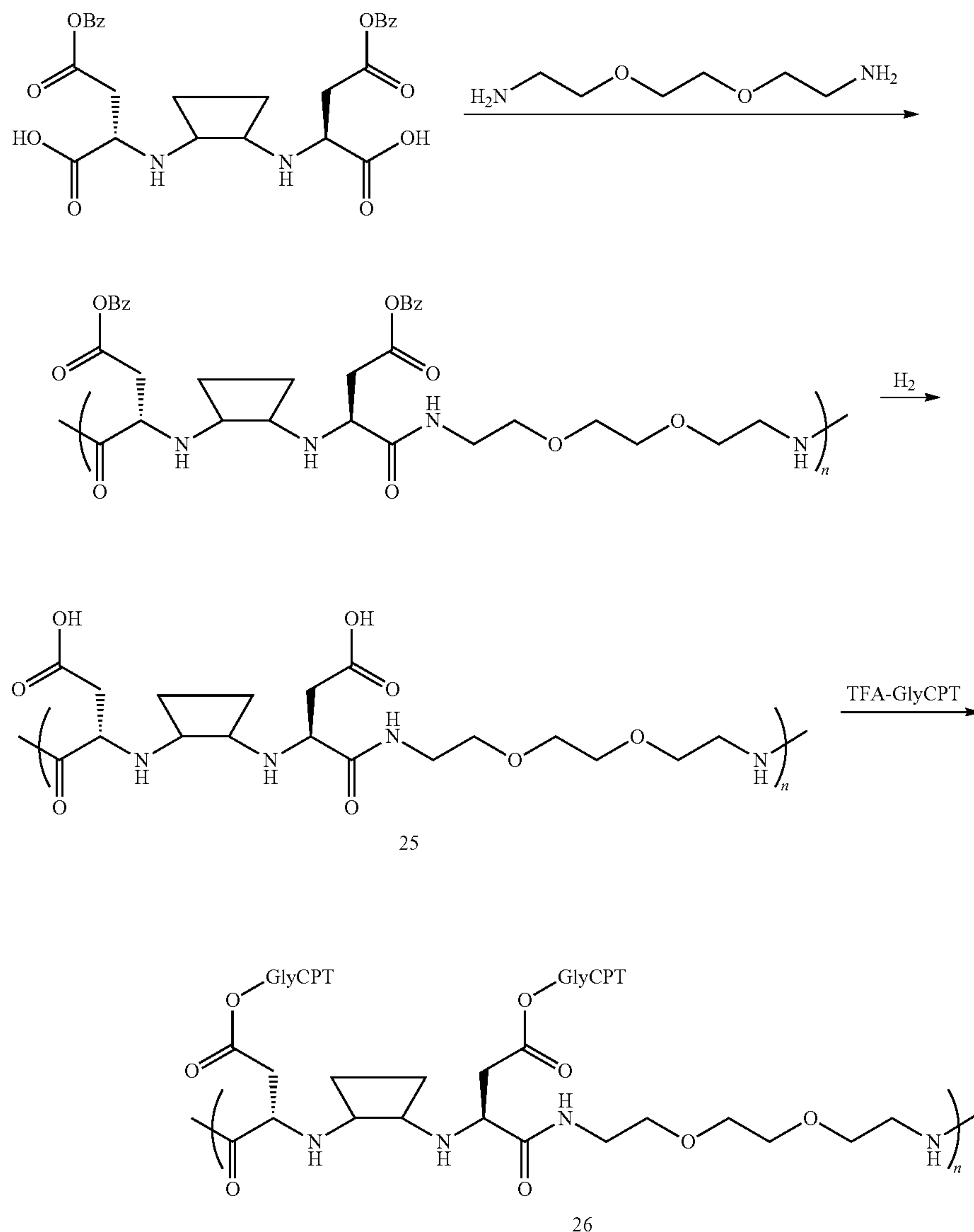
Scheme XXXI
