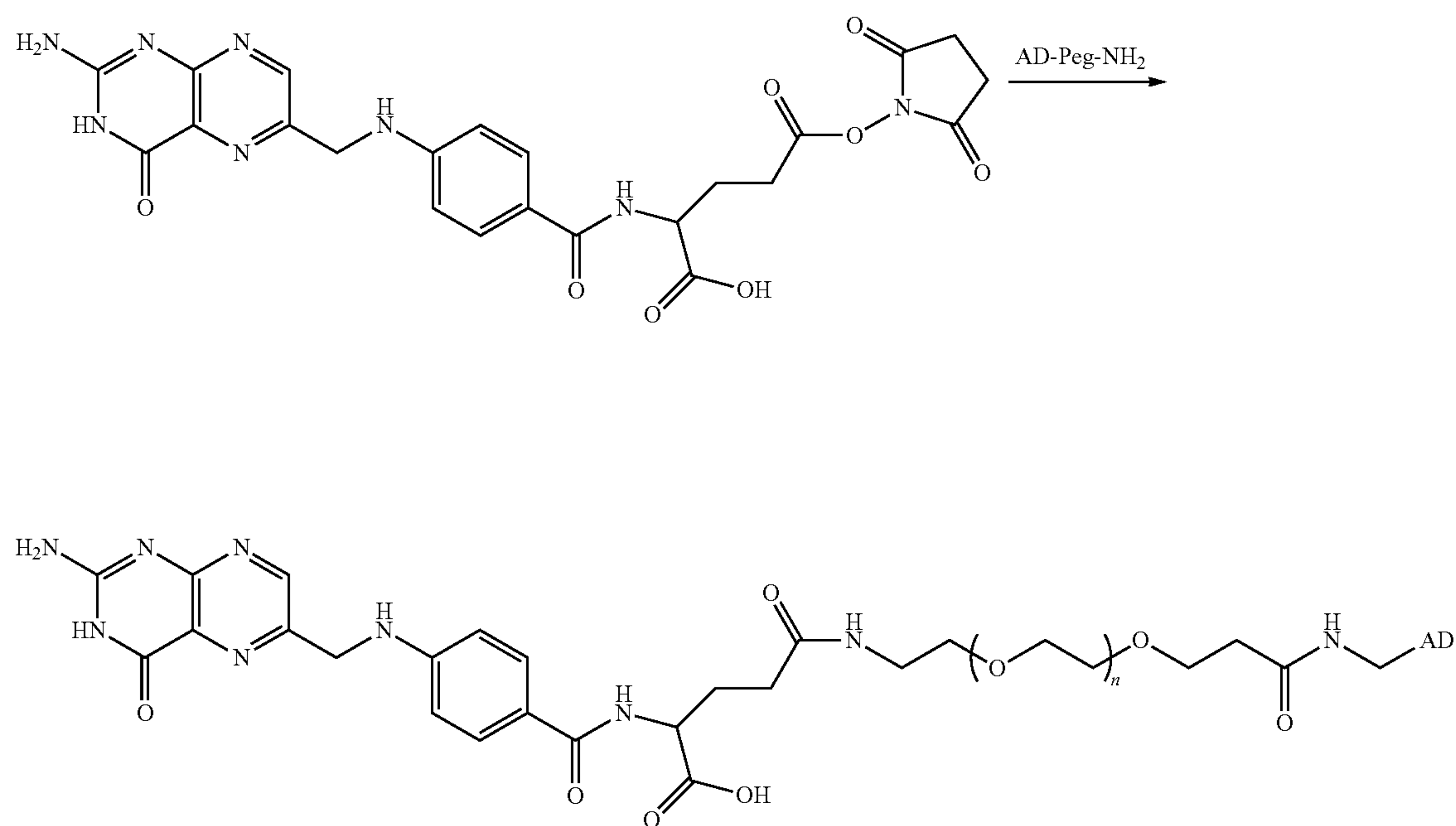
Scheme L
