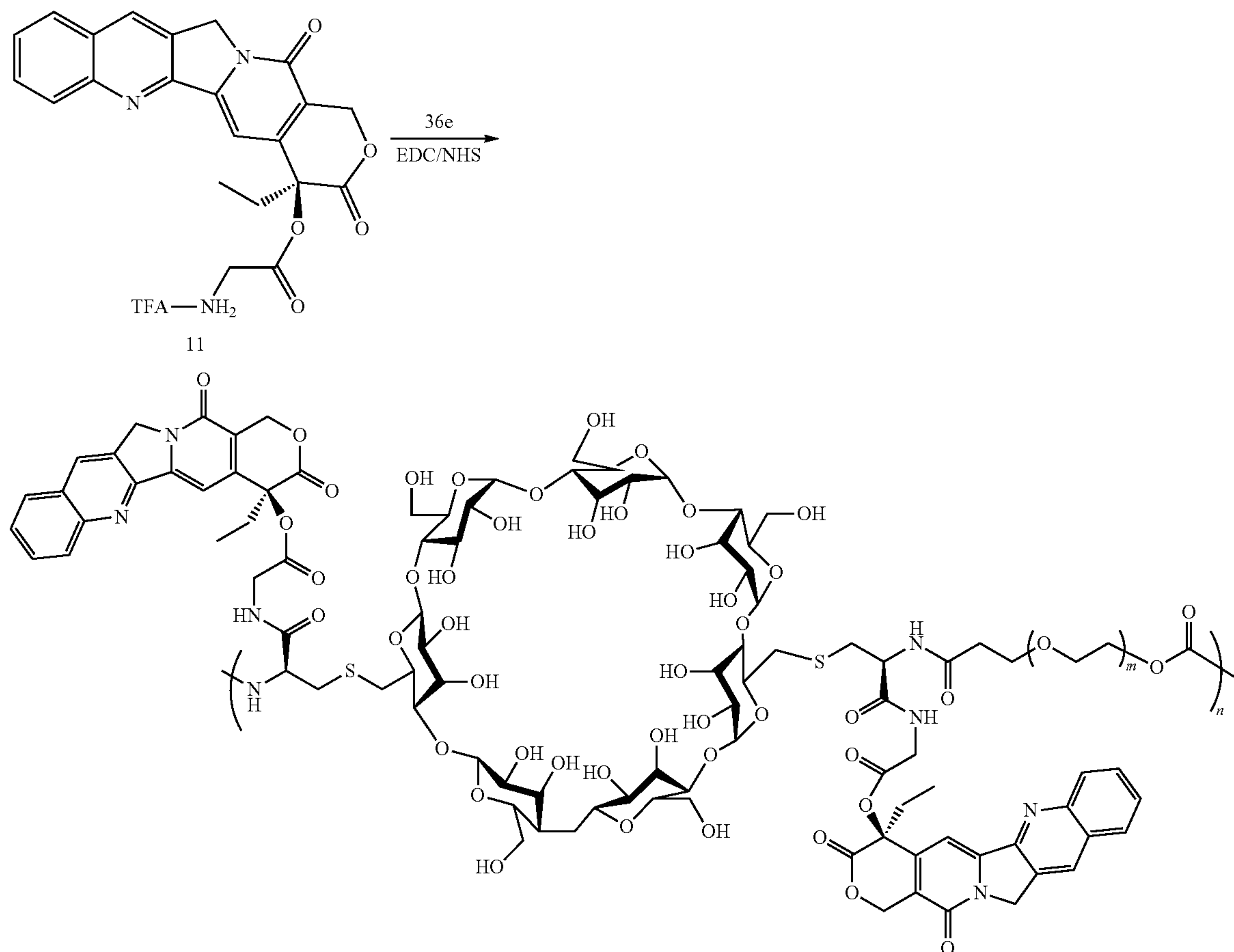
Scheme XXXIX
