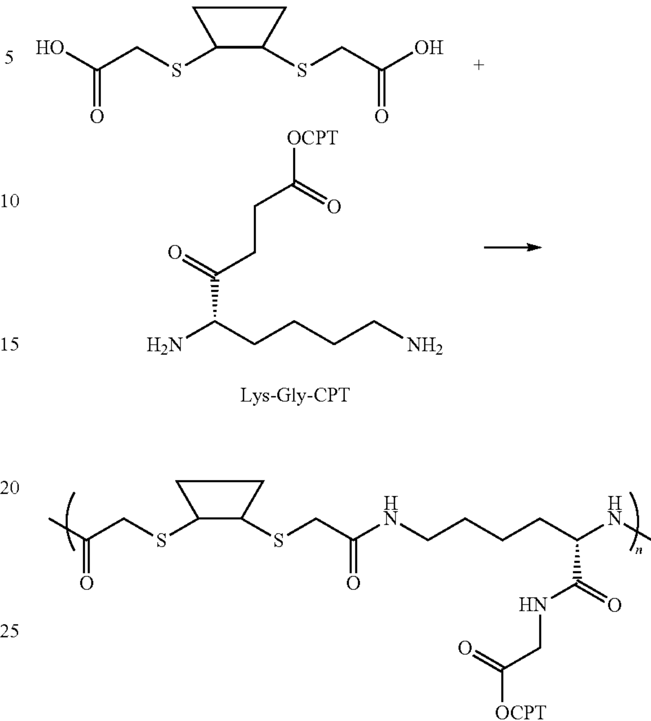
Scheme VIII
