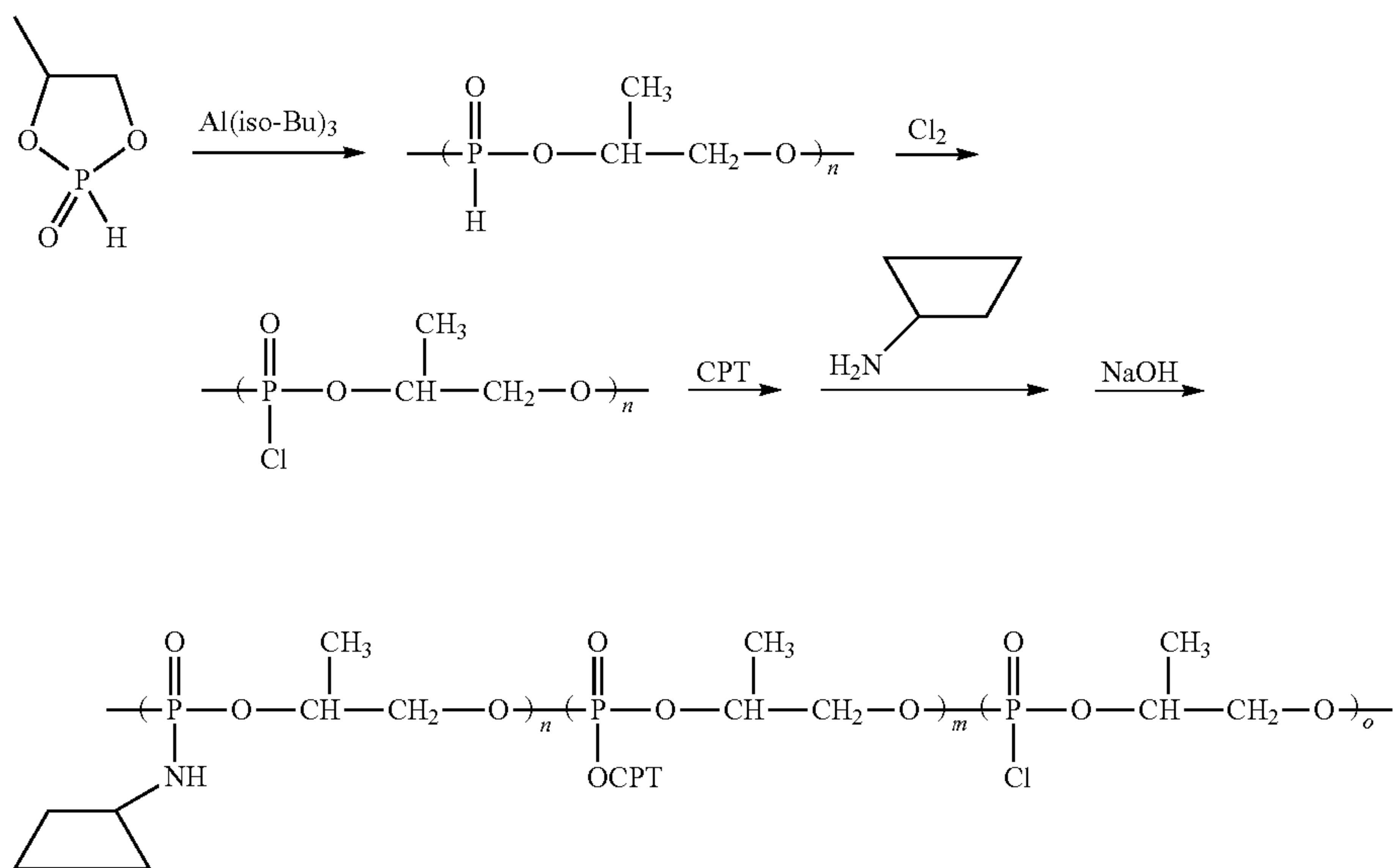
Scheme IX
