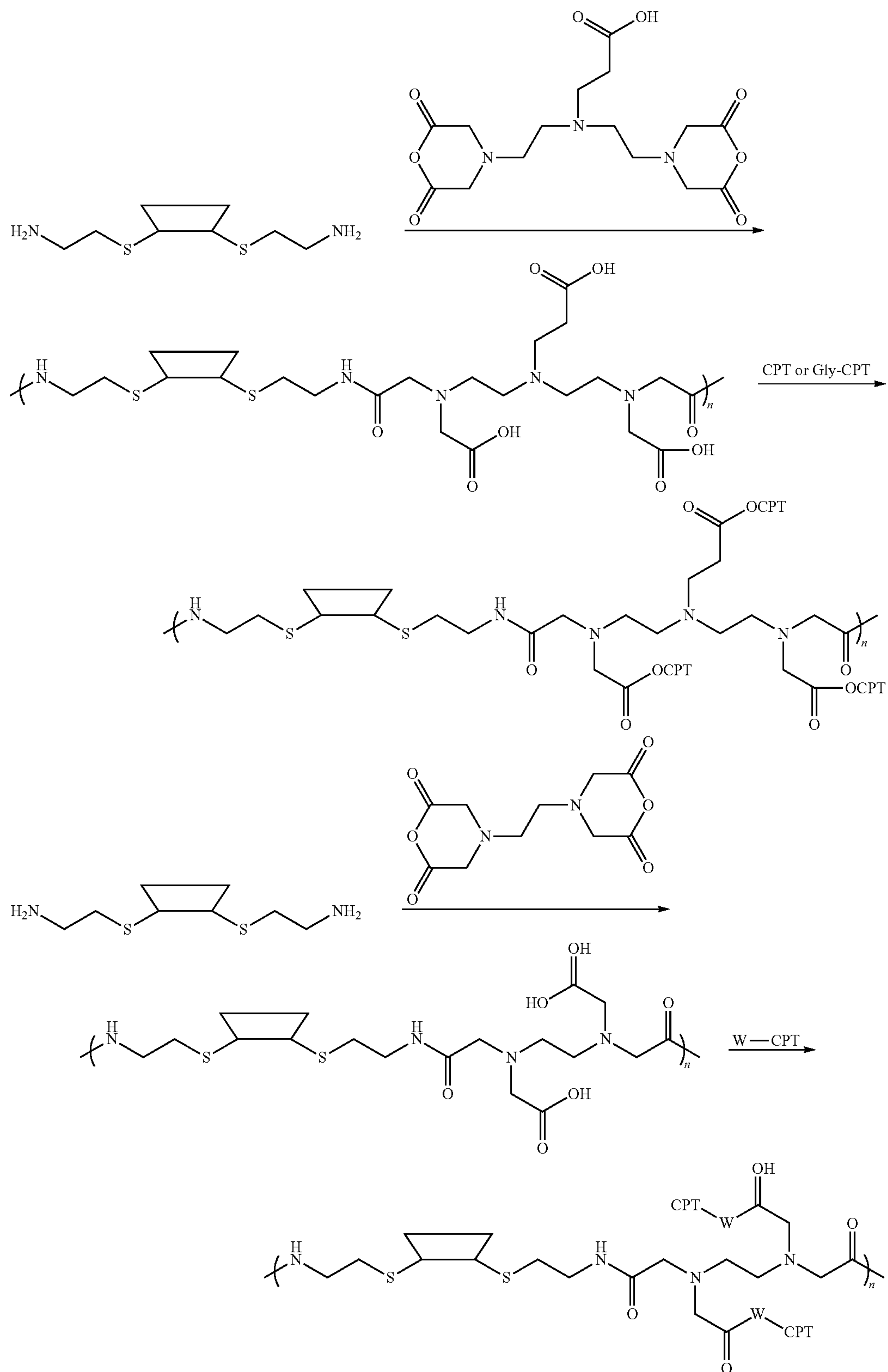
Scheme V
