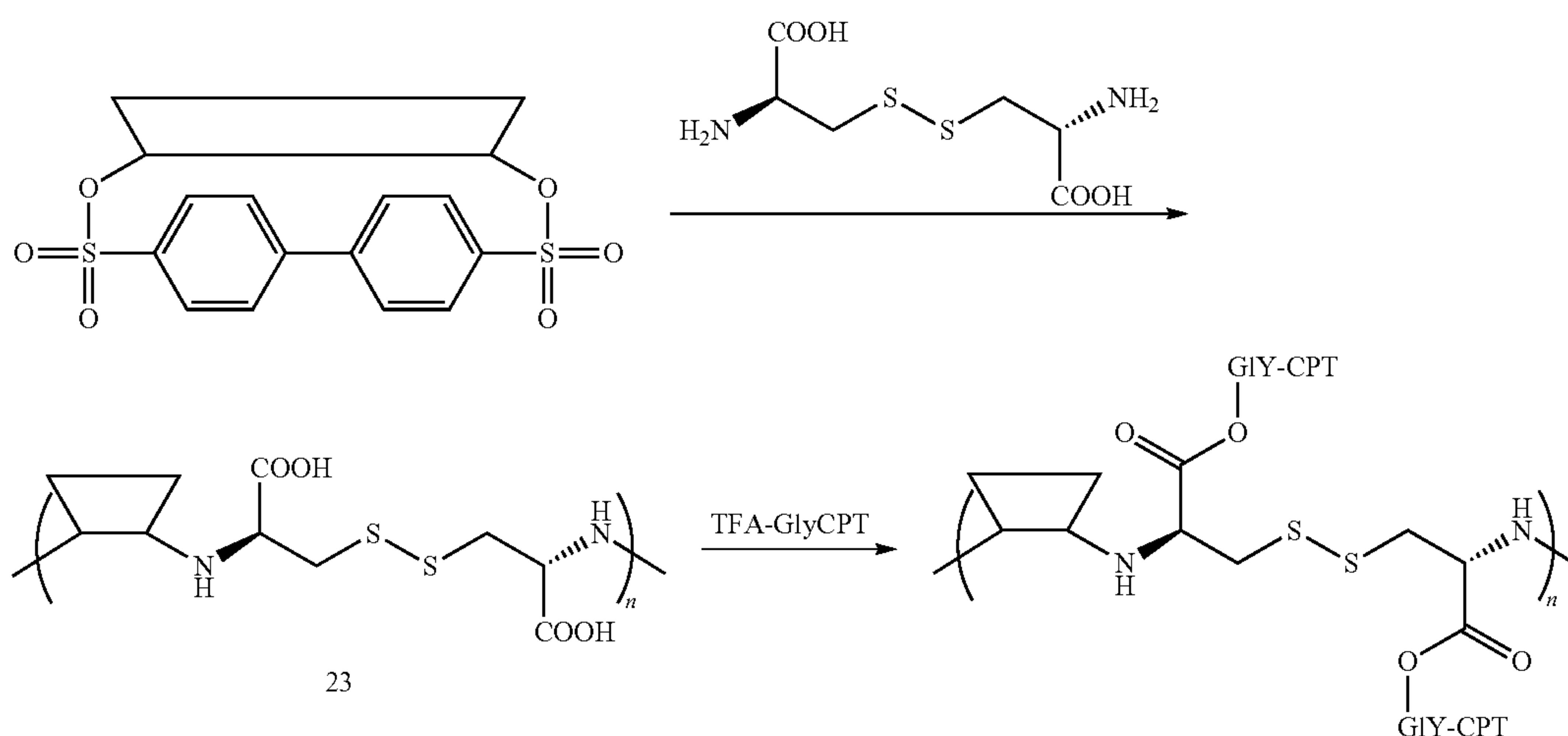
Scheme XXX
