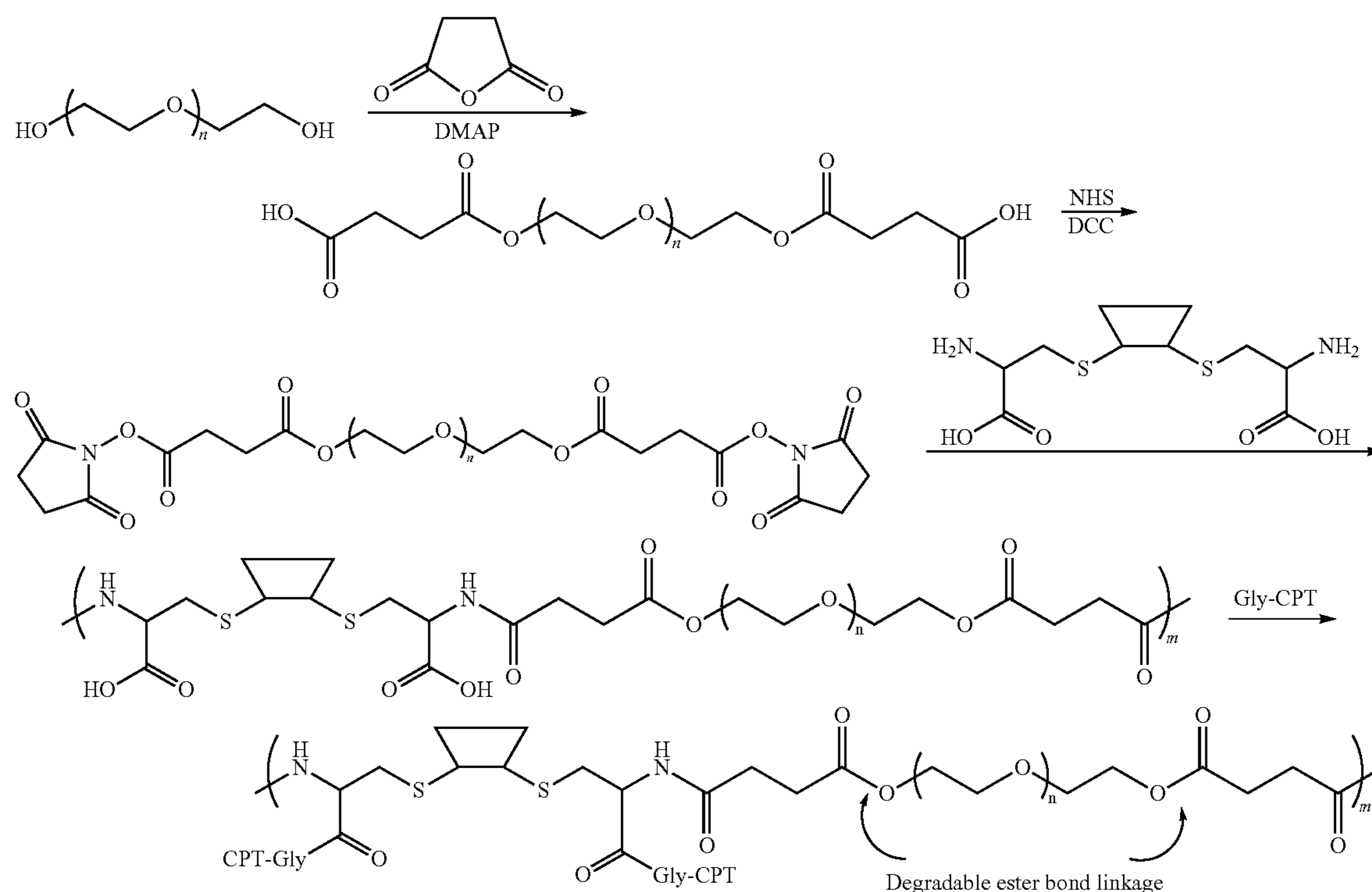
Scheme XIV
