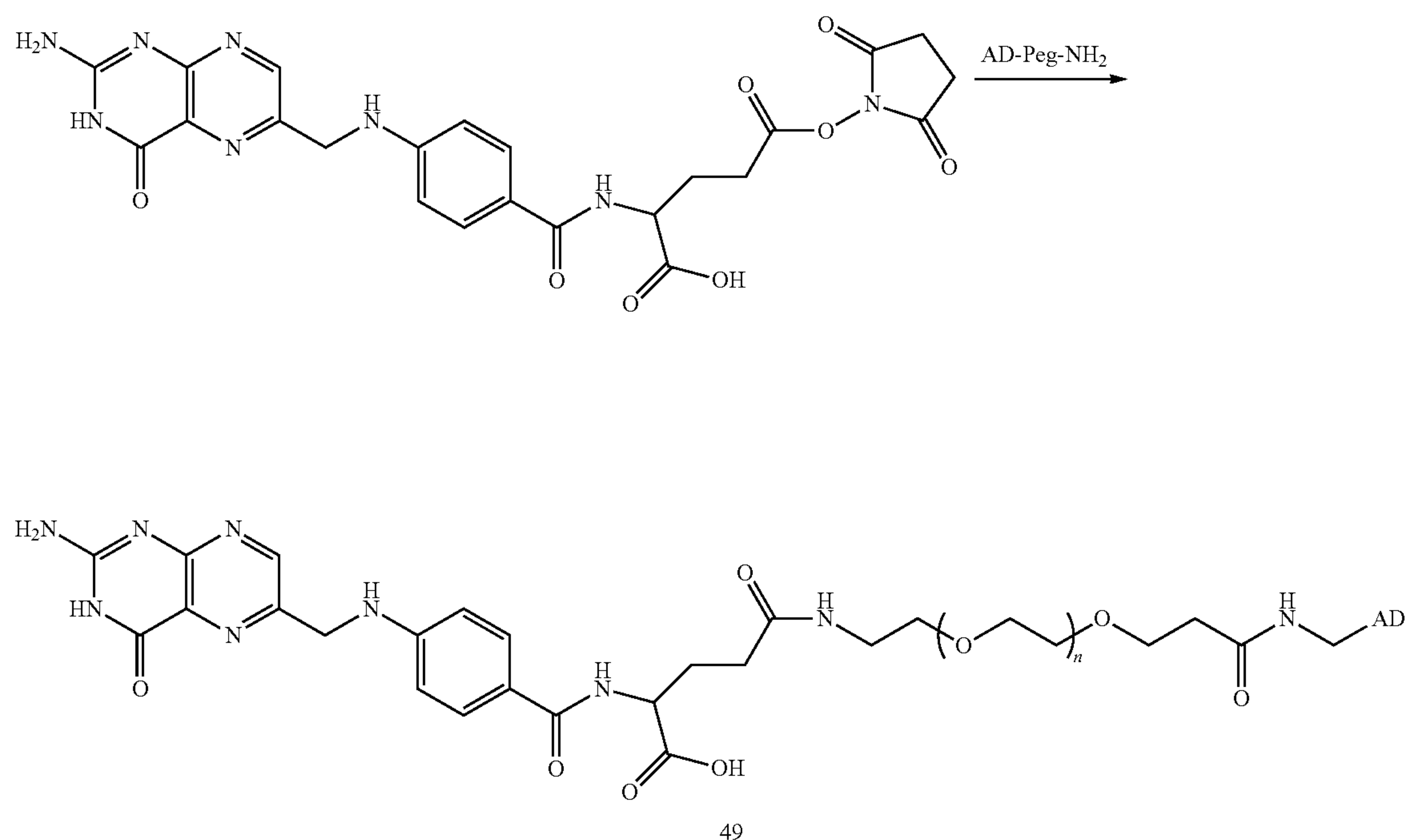
Scheme L
