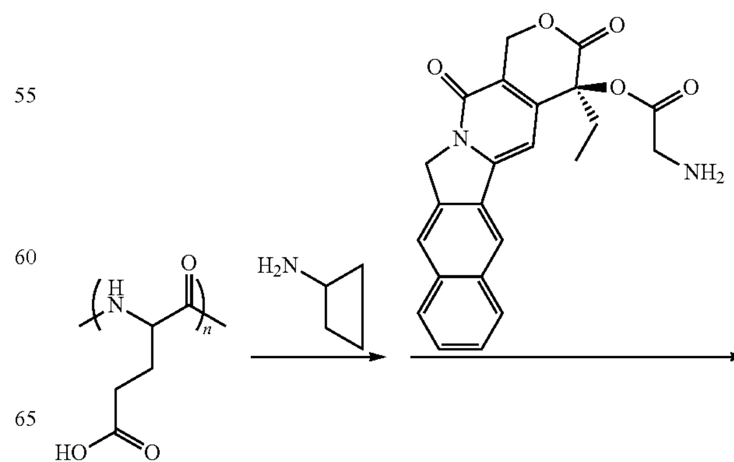
Scheme XXXVII
