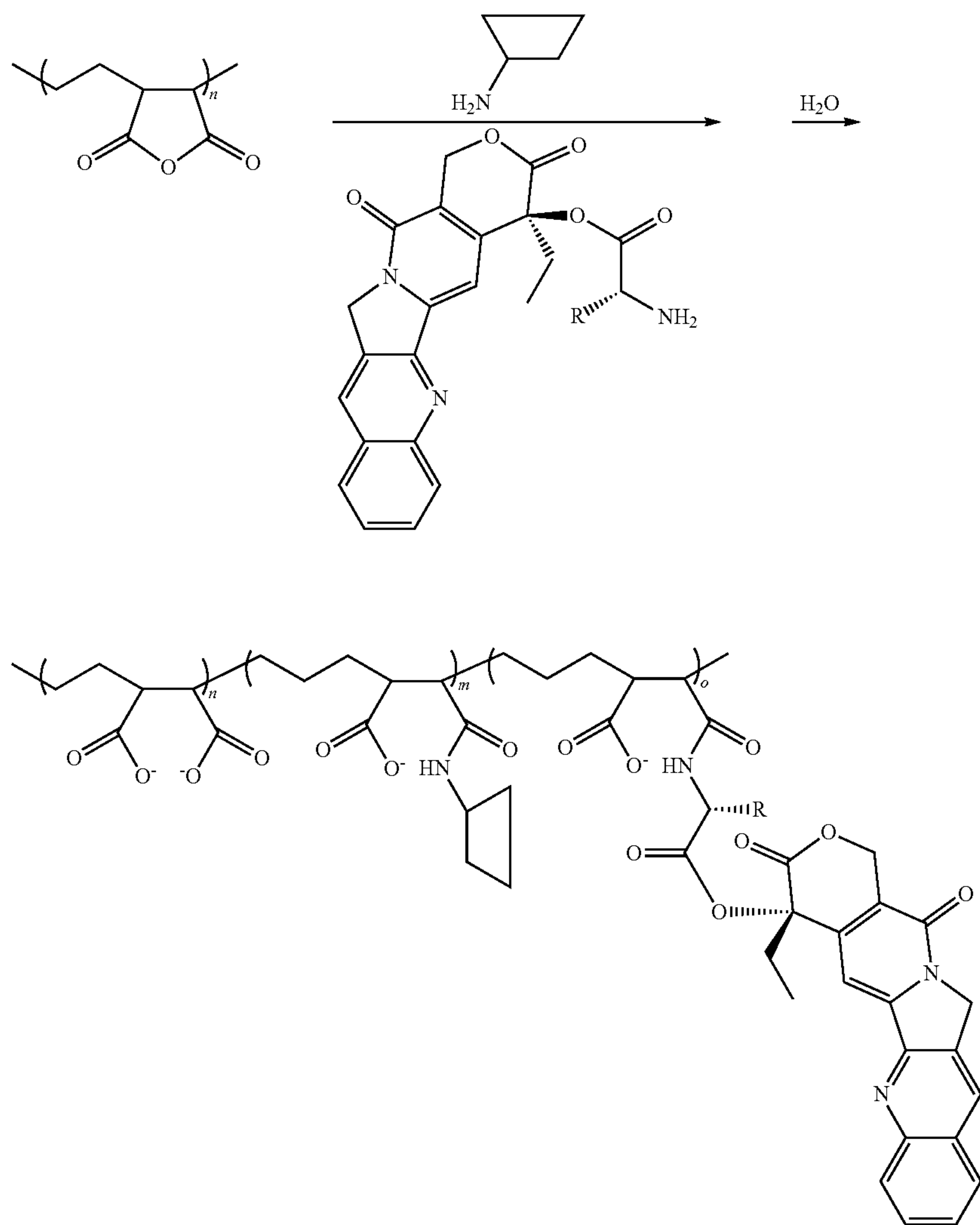
Scheme XI
