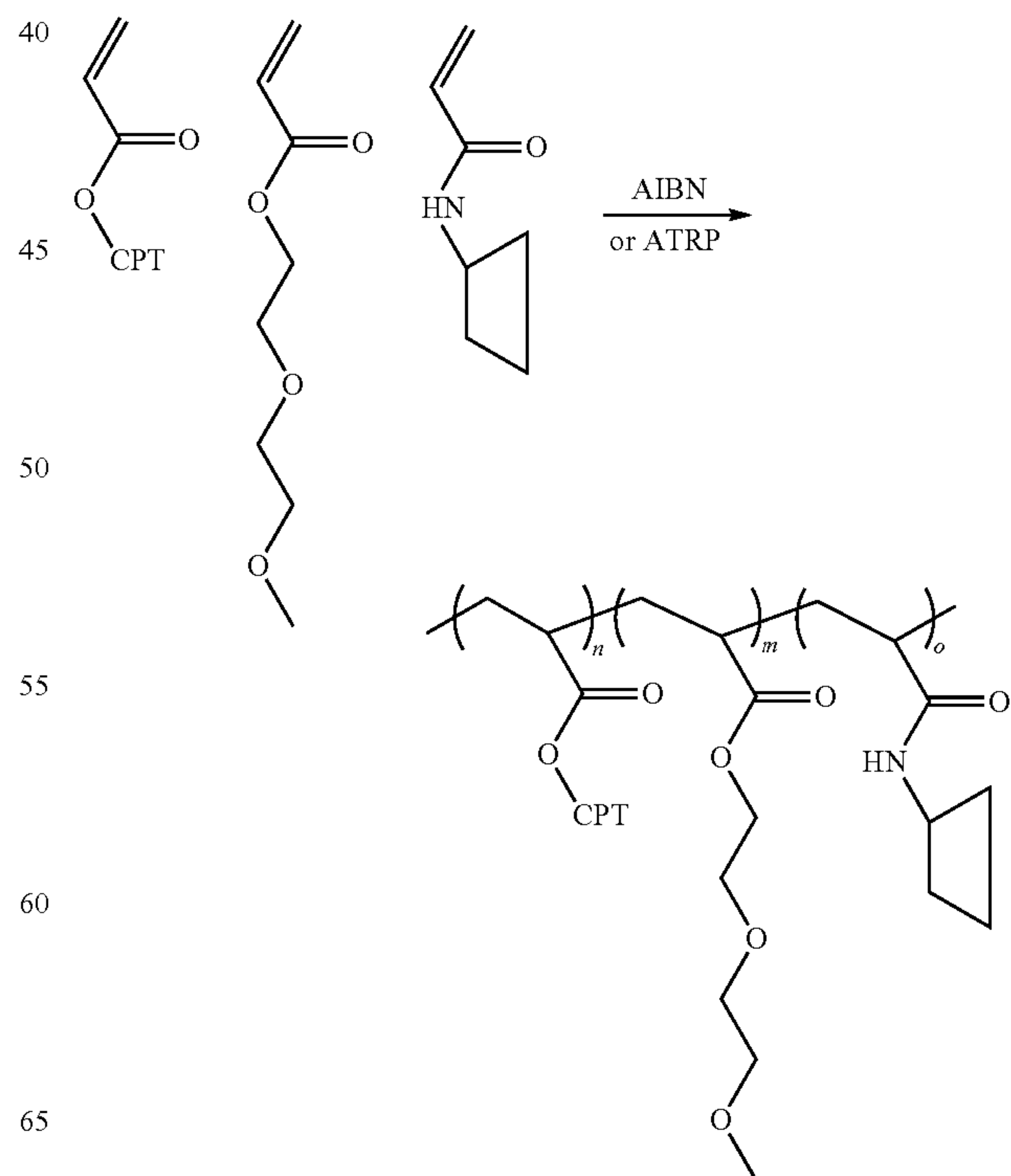
Scheme X
