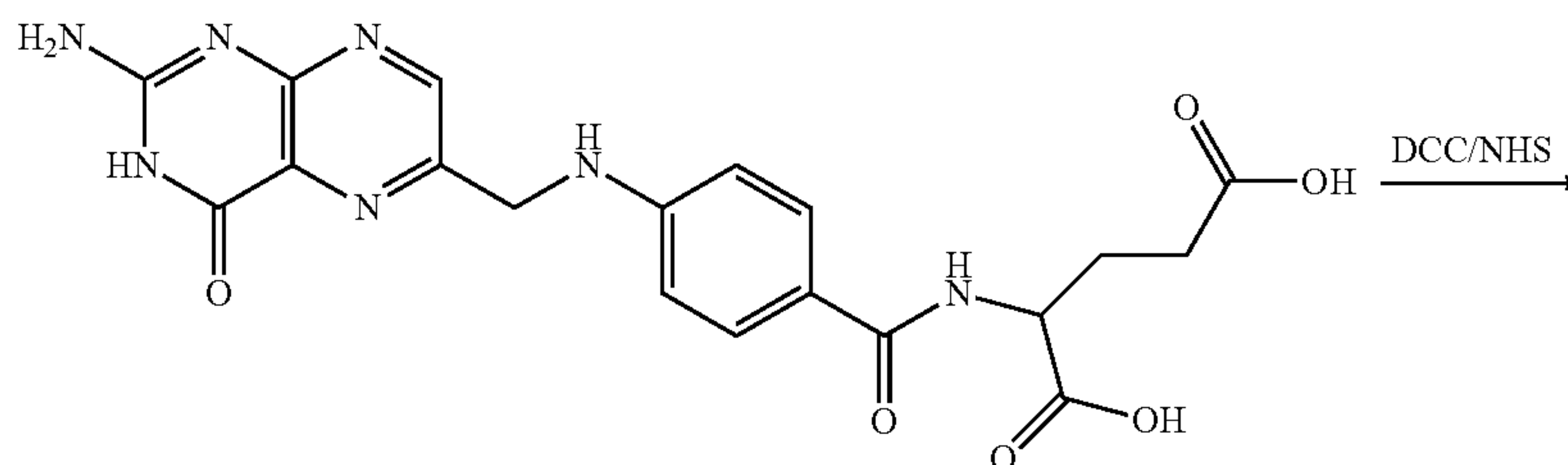
Scheme XXXXIX
