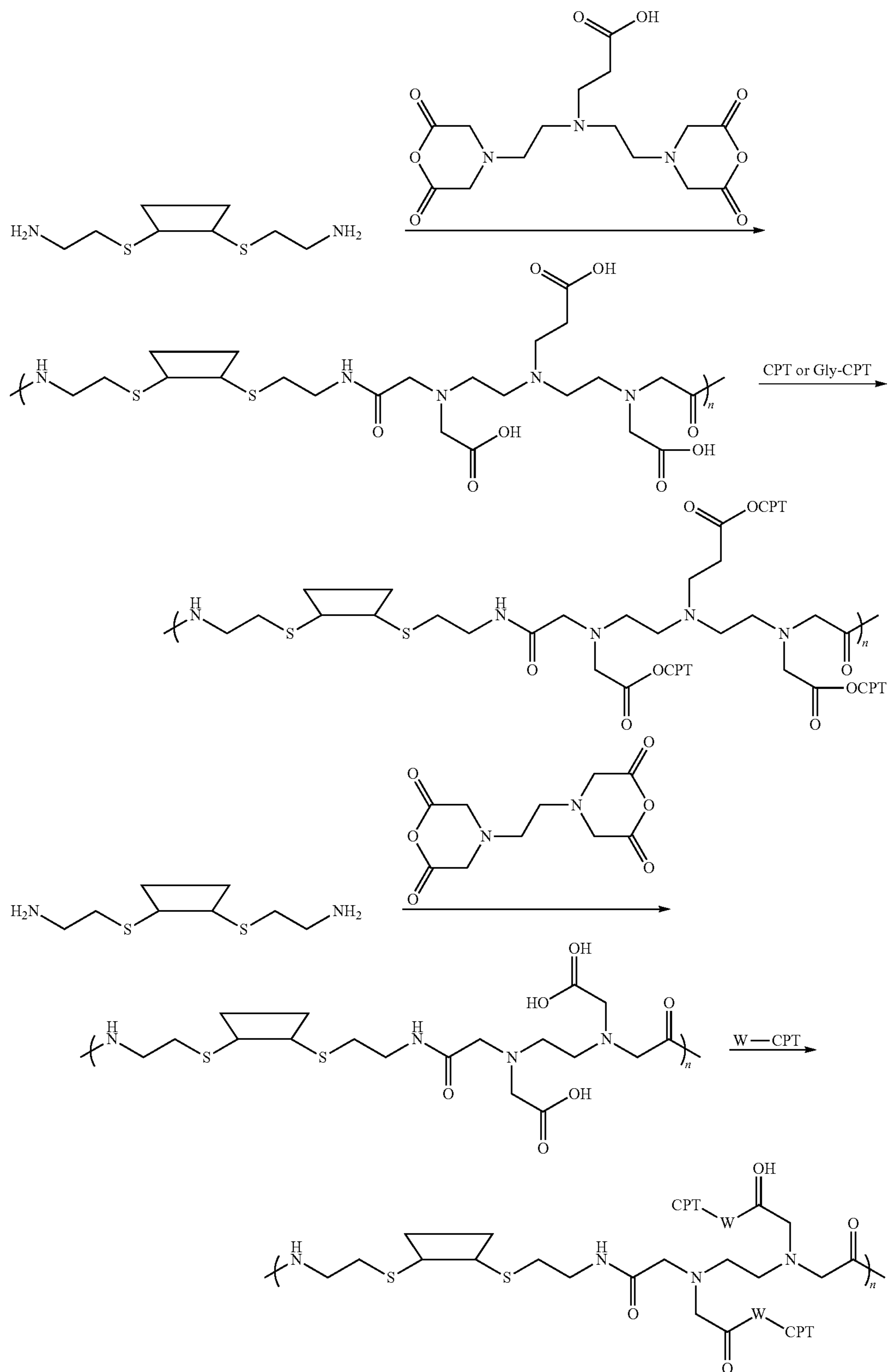
Scheme V
