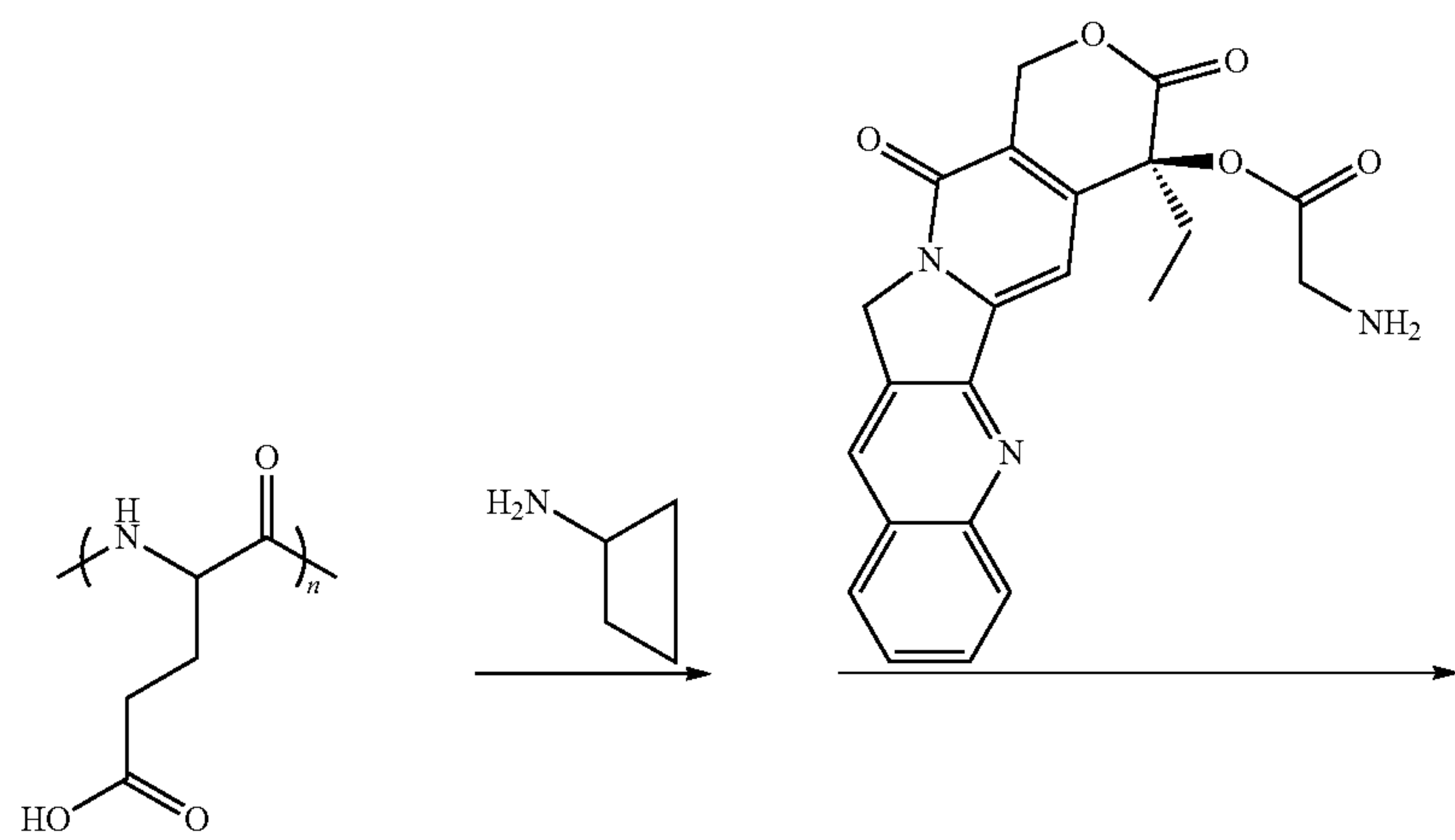
Scheme XII
