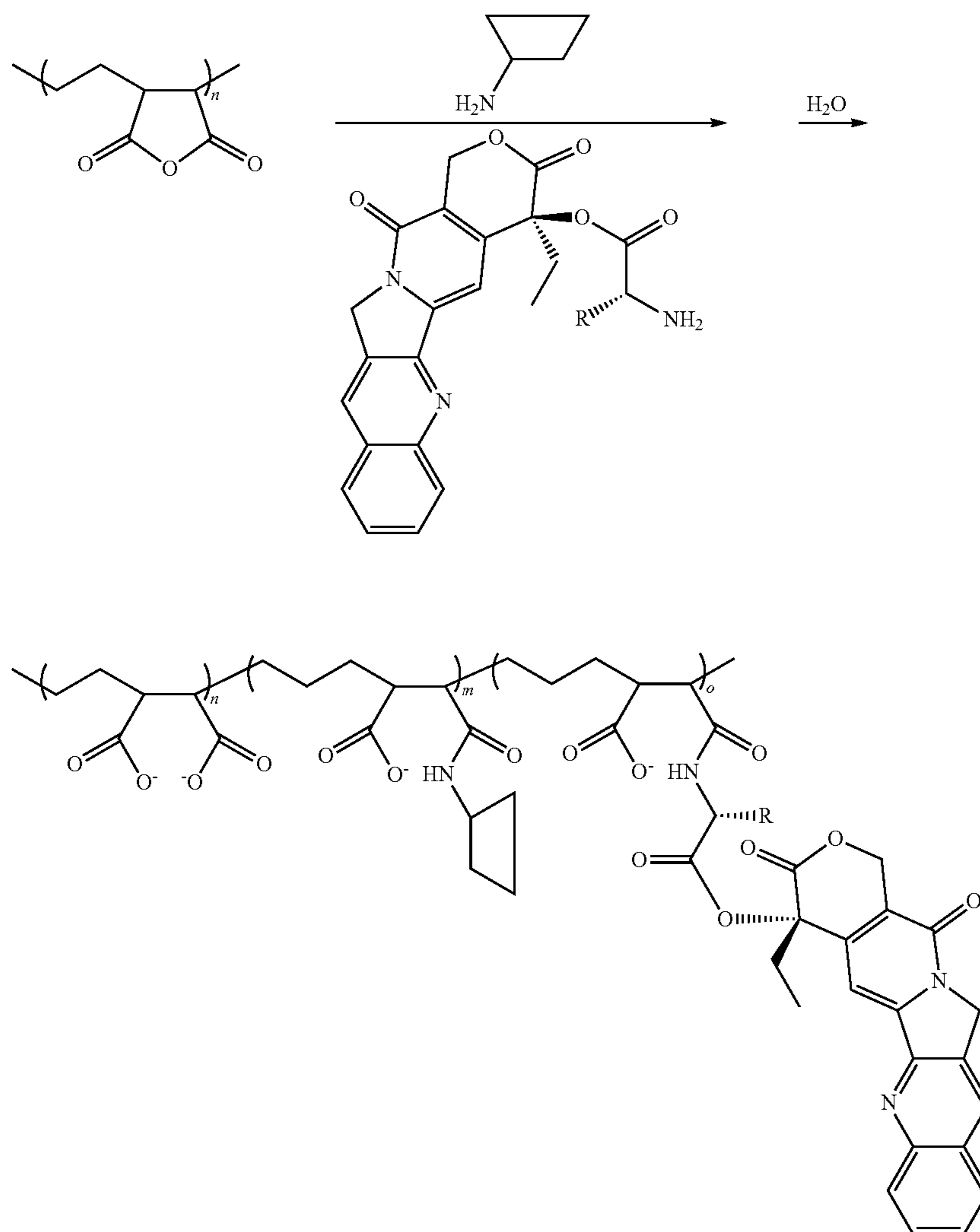
Scheme XI
