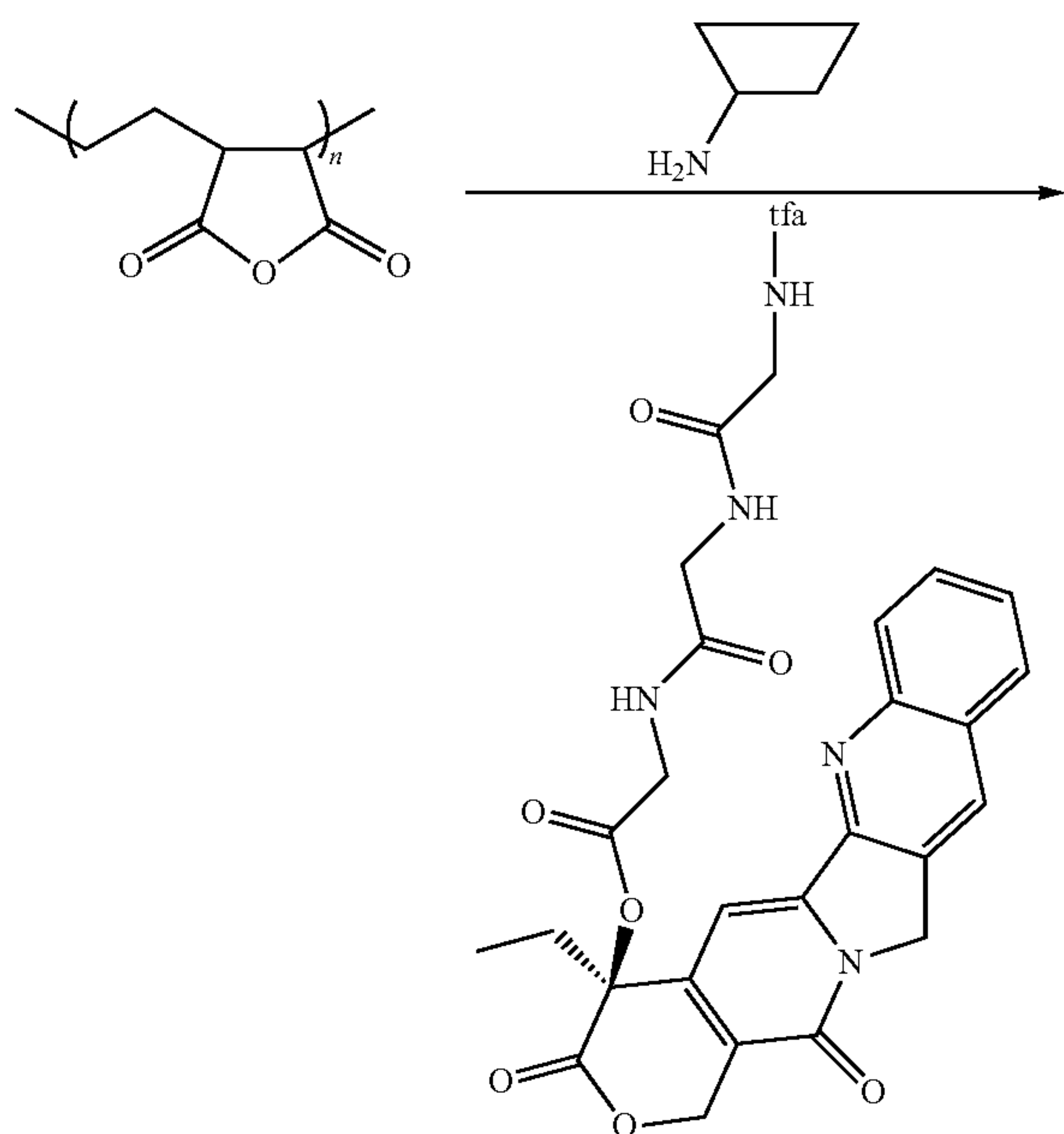
Scheme XXXVI
