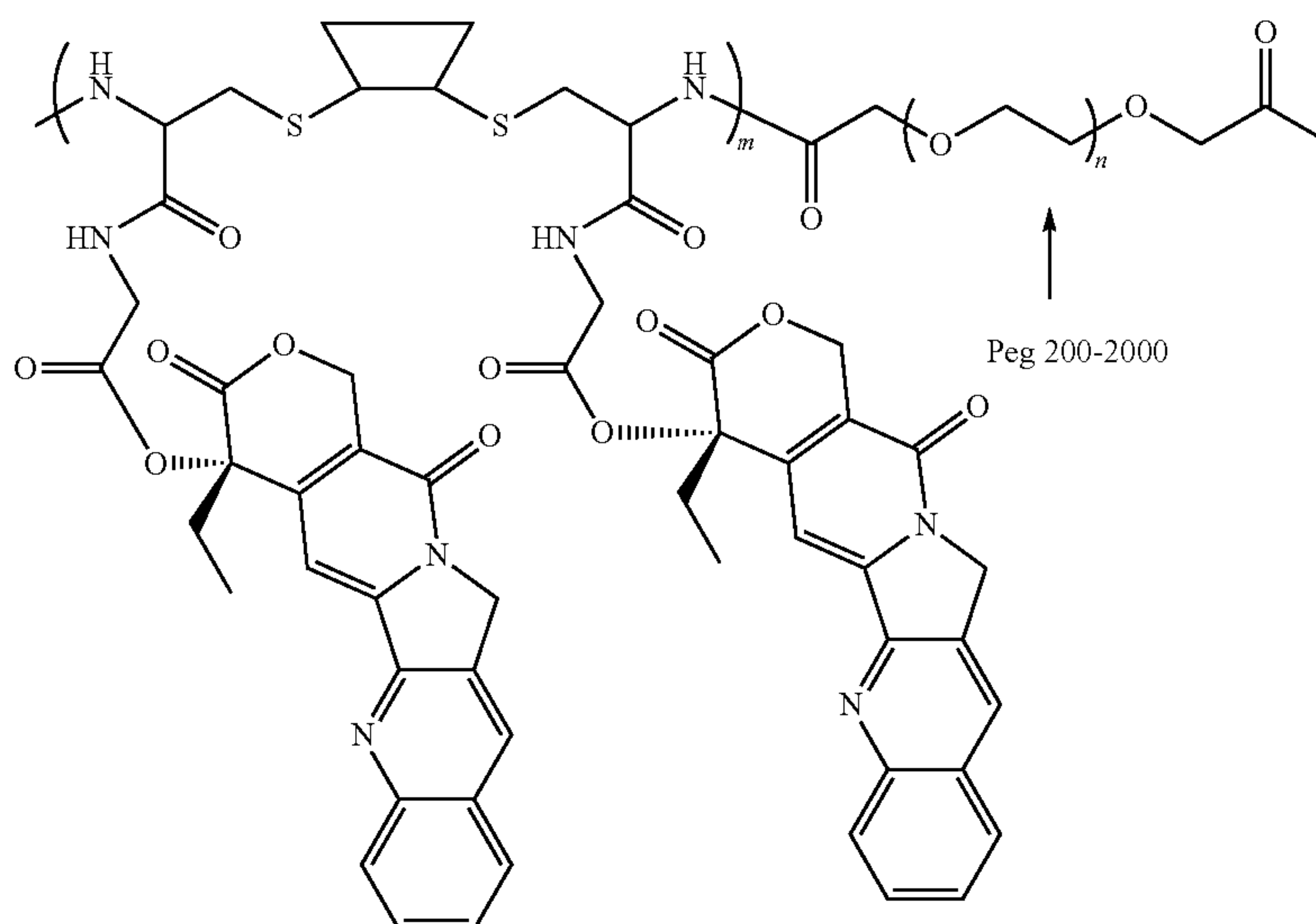
Scheme XXXXII
