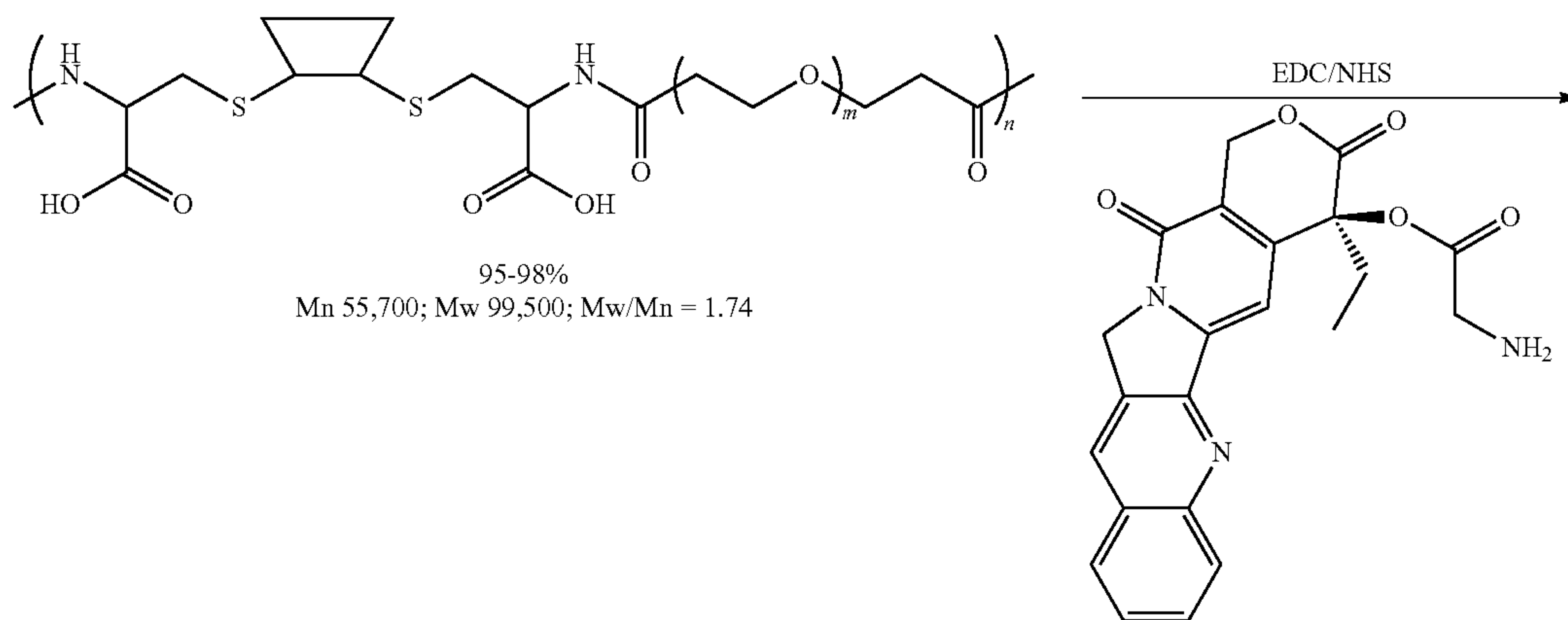
Gly-CPT
