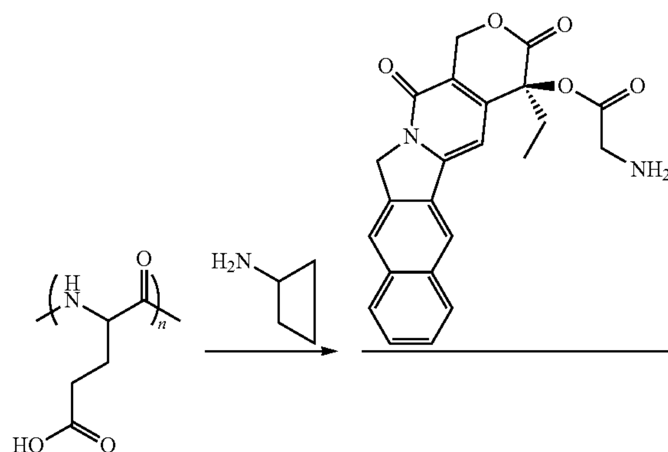
Scheme XXXVII
