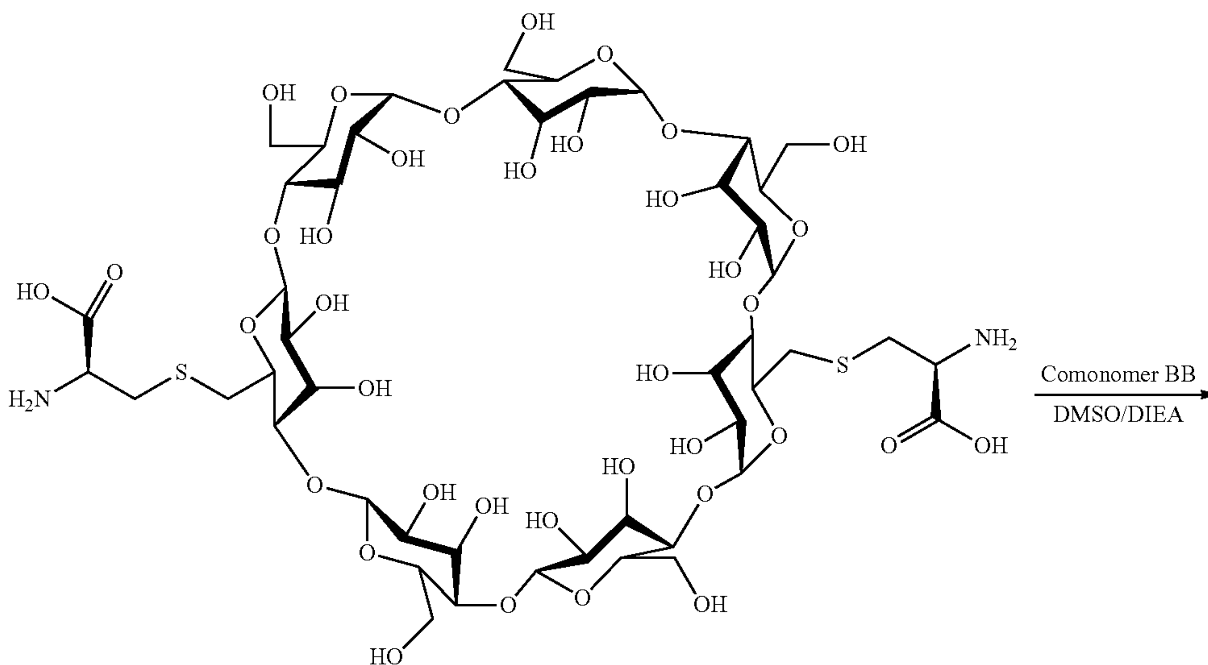
Scheme XXXVIIIb
