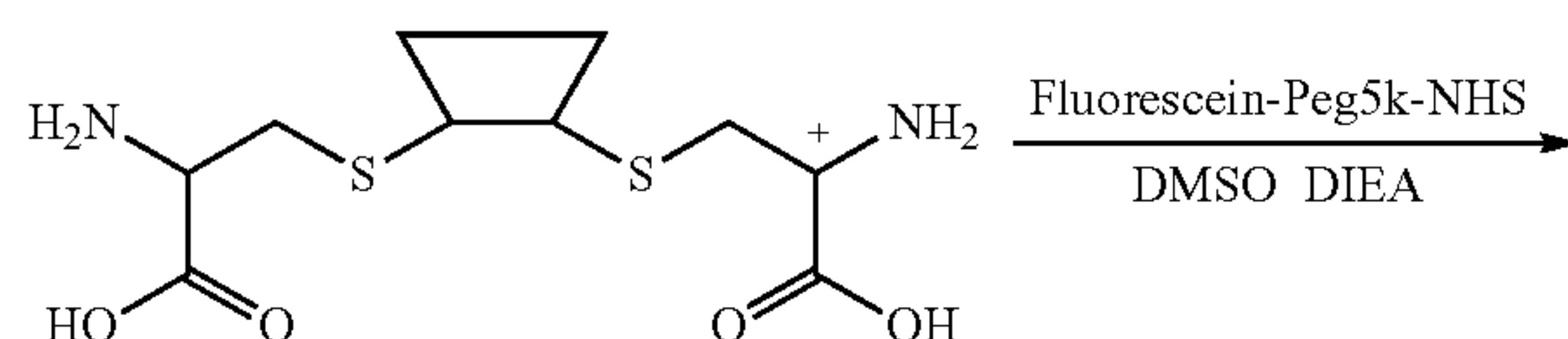
Scheme XXXX
