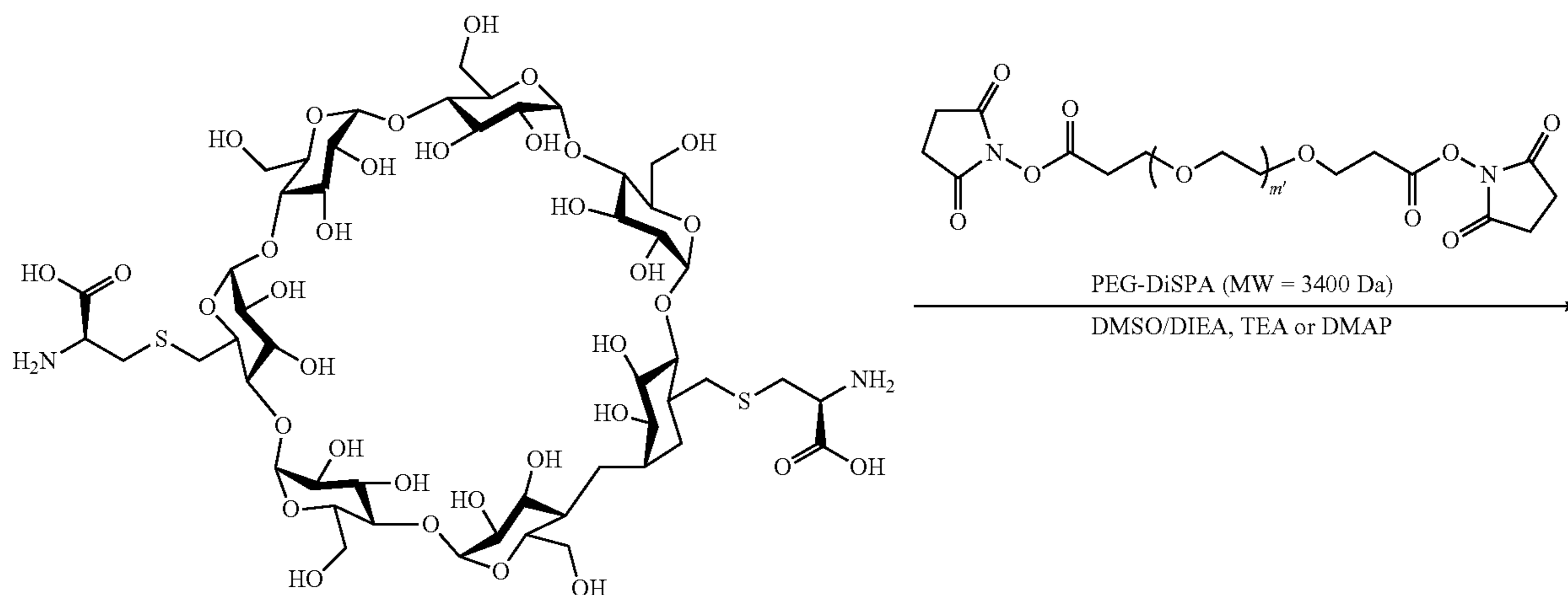
Scheme XXXVIIIa
