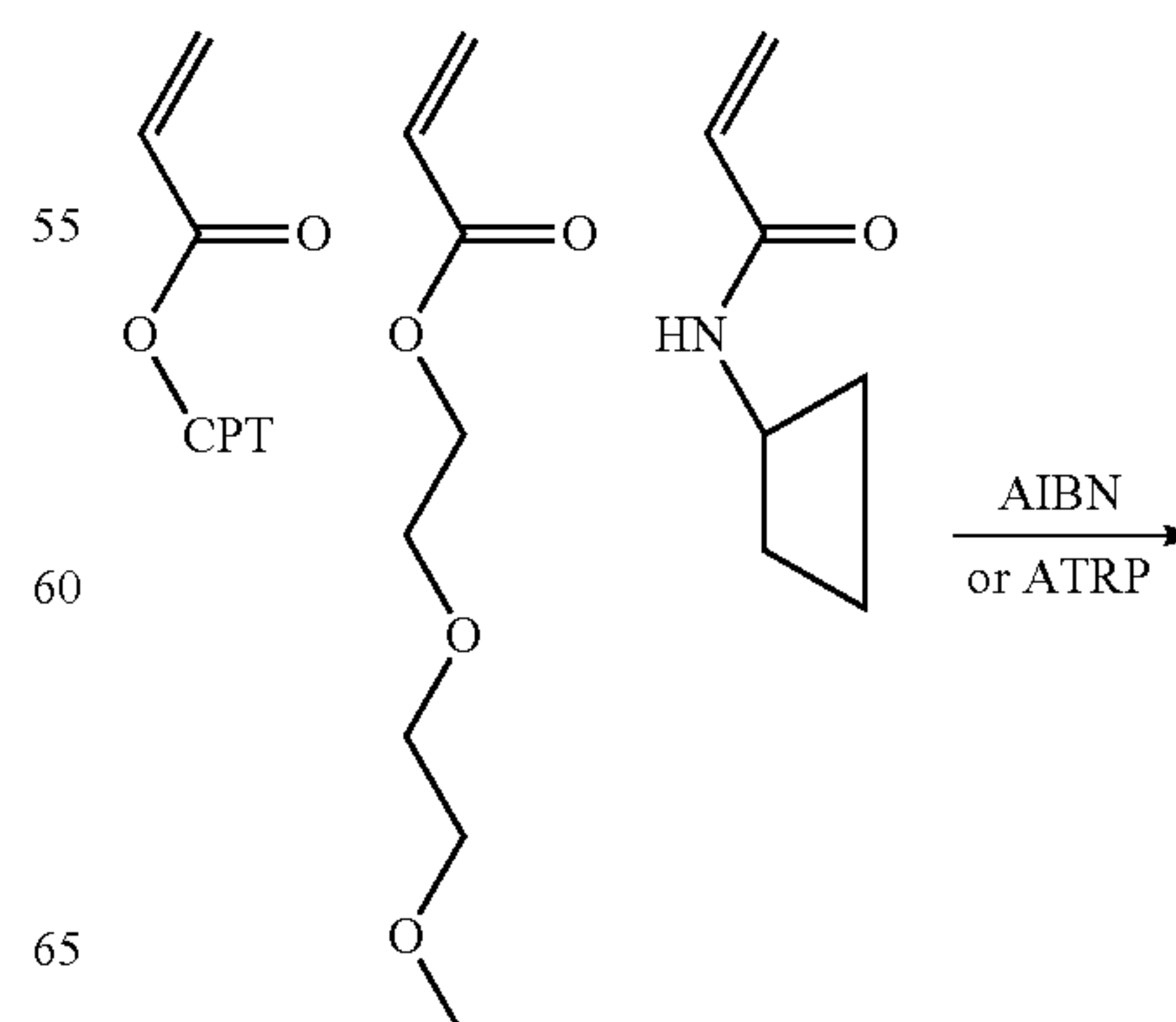
Scheme XXXV
