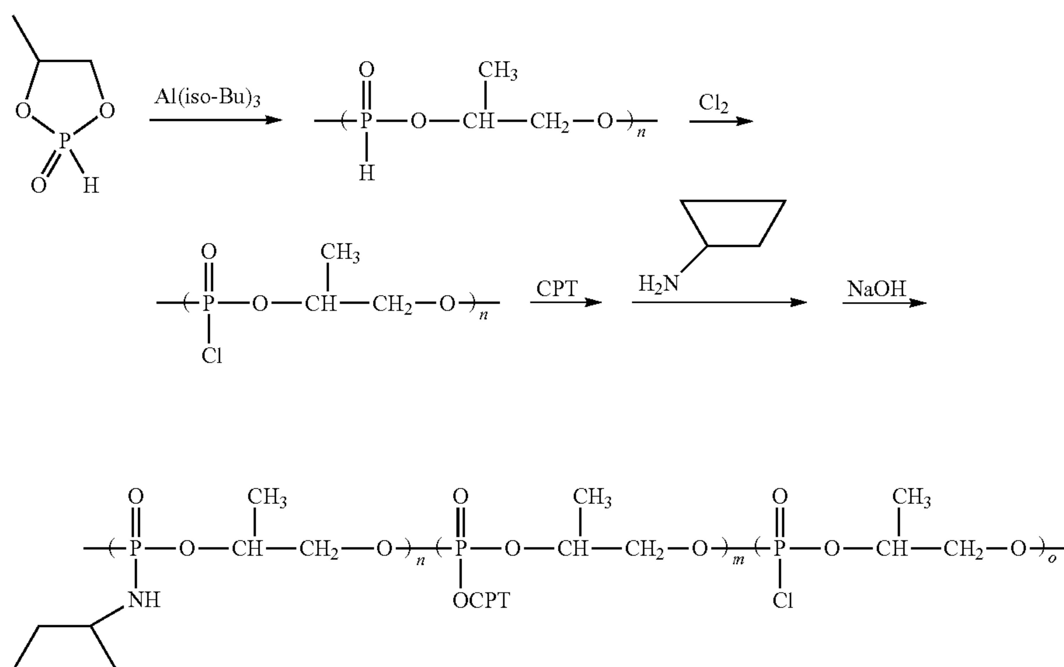
Scheme IX
