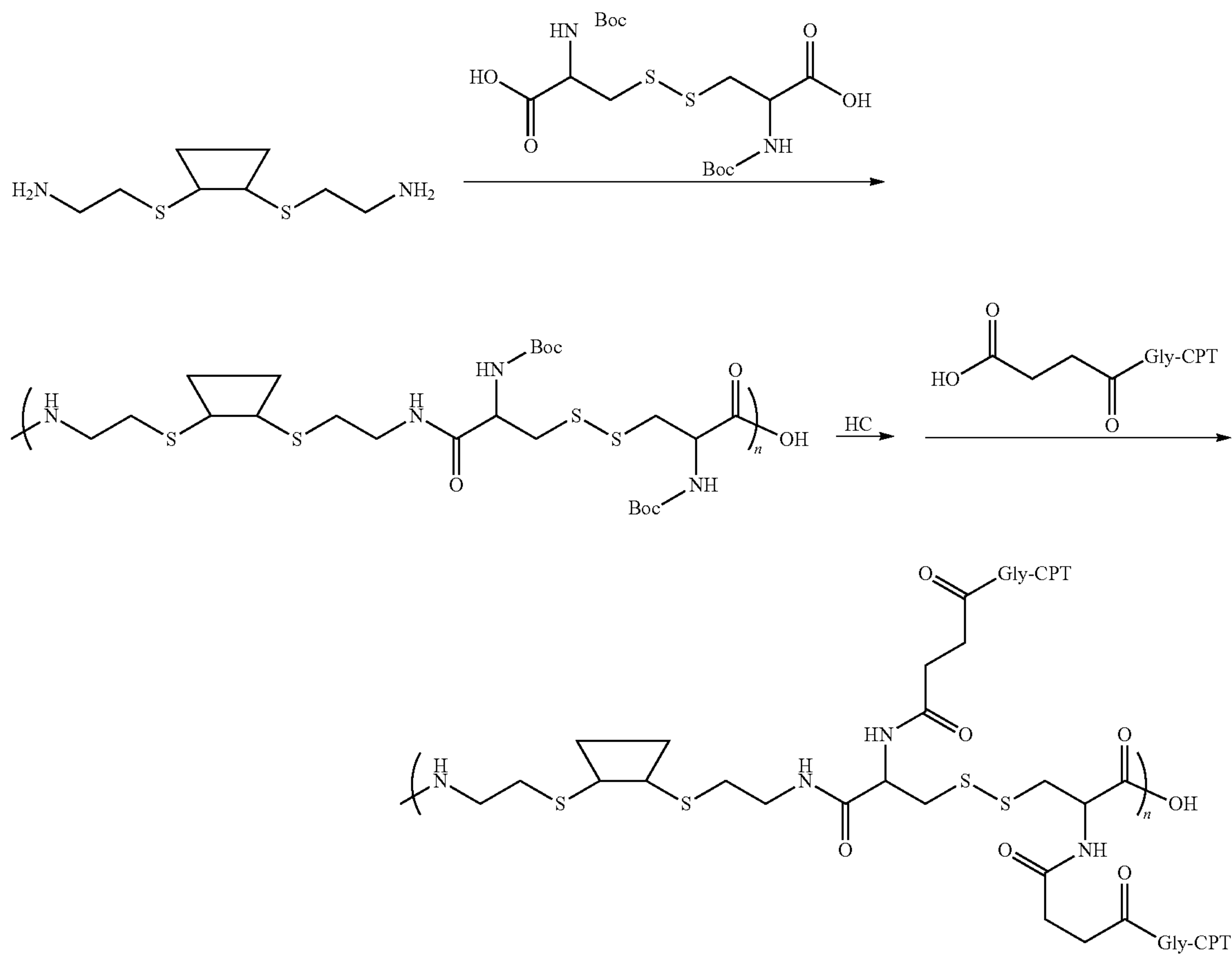
Scheme VII
