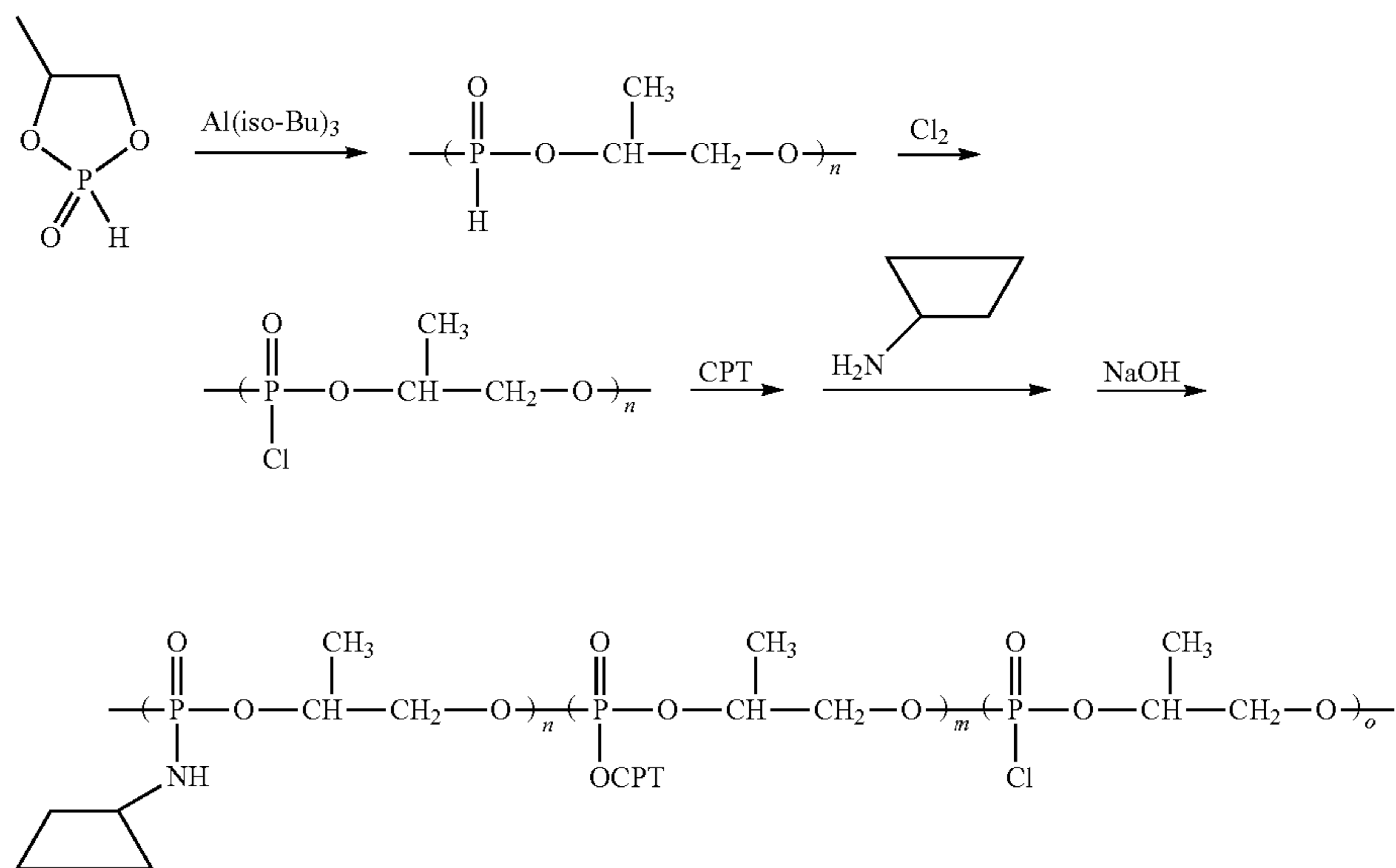
Scheme IX
