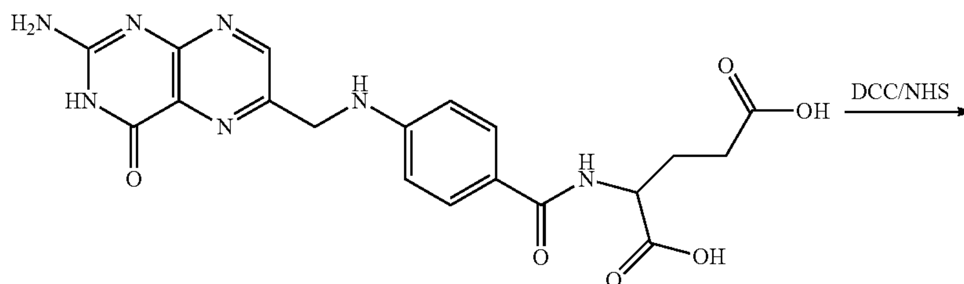
Scheme XXXXIX
