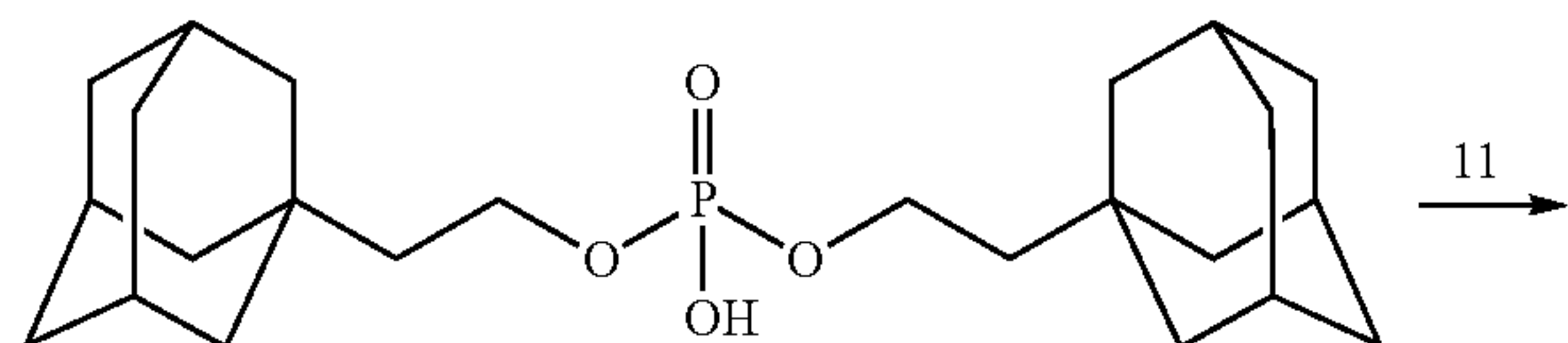
Scheme XXXXVIII
