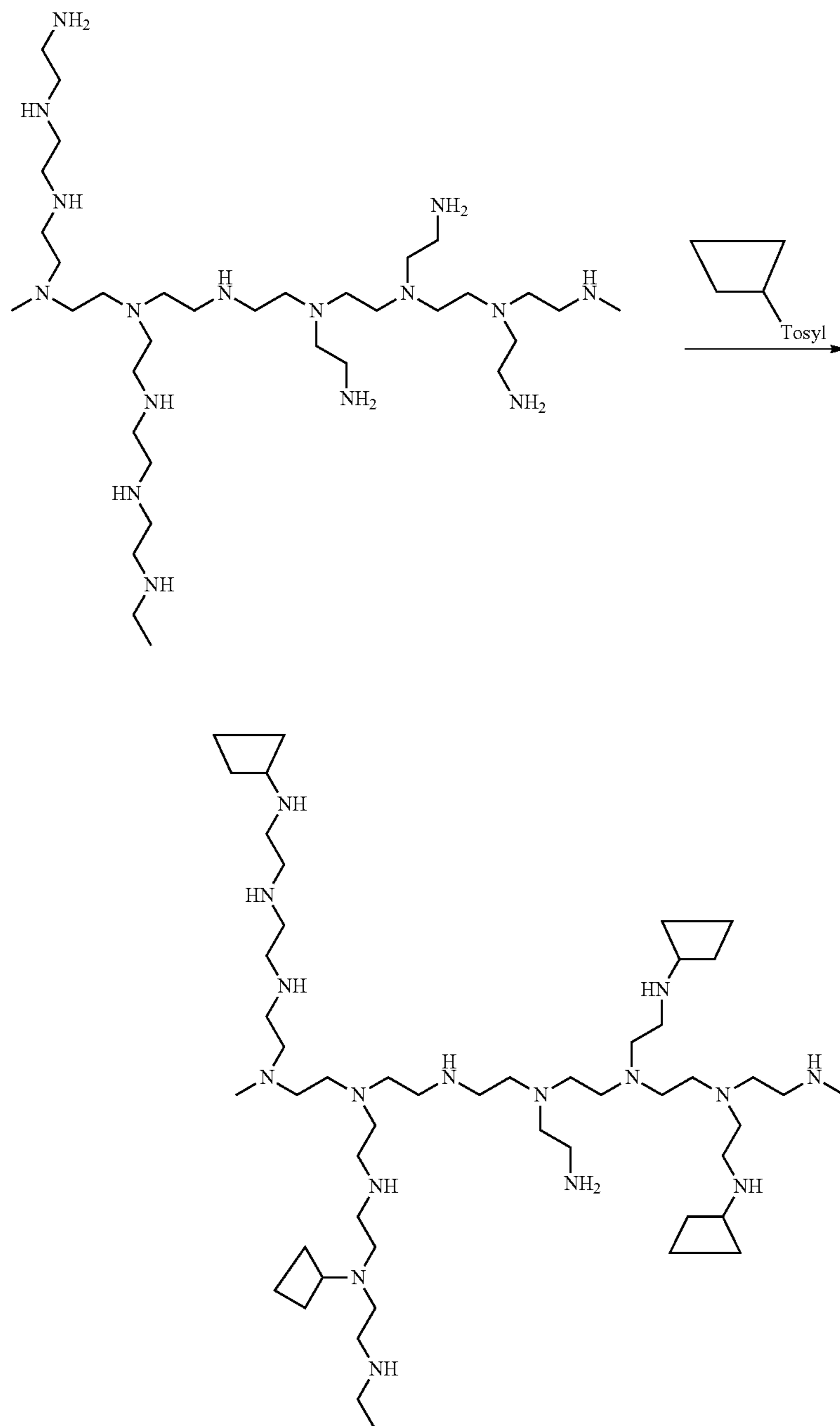
Scheme XXXXIV
