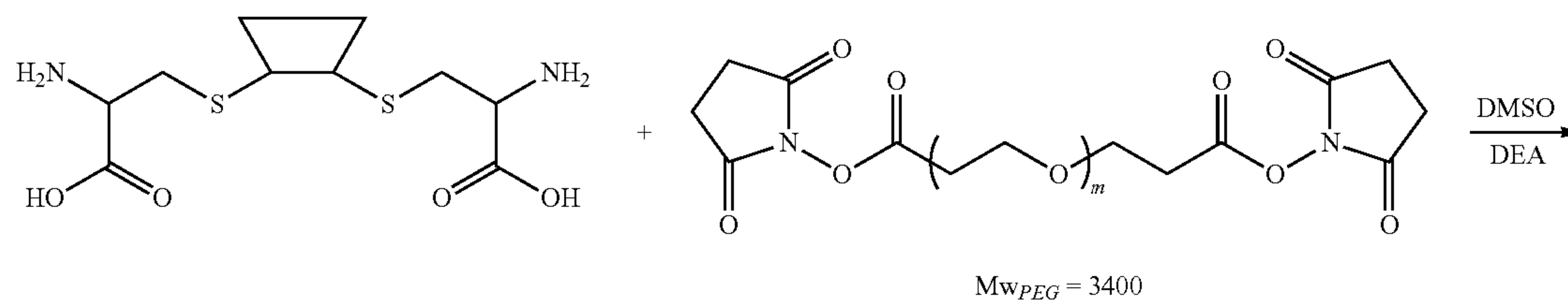
Scheme XIII
