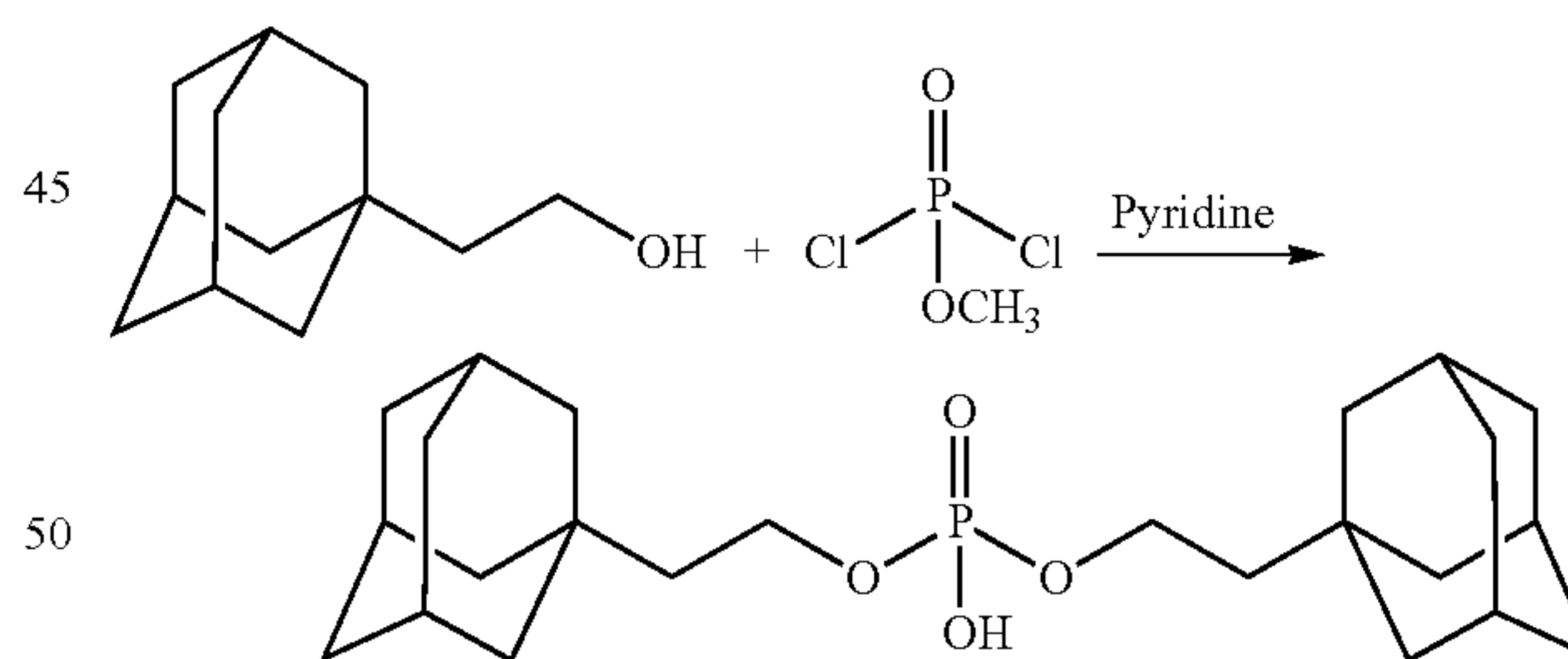
Scheme XXXXVII
