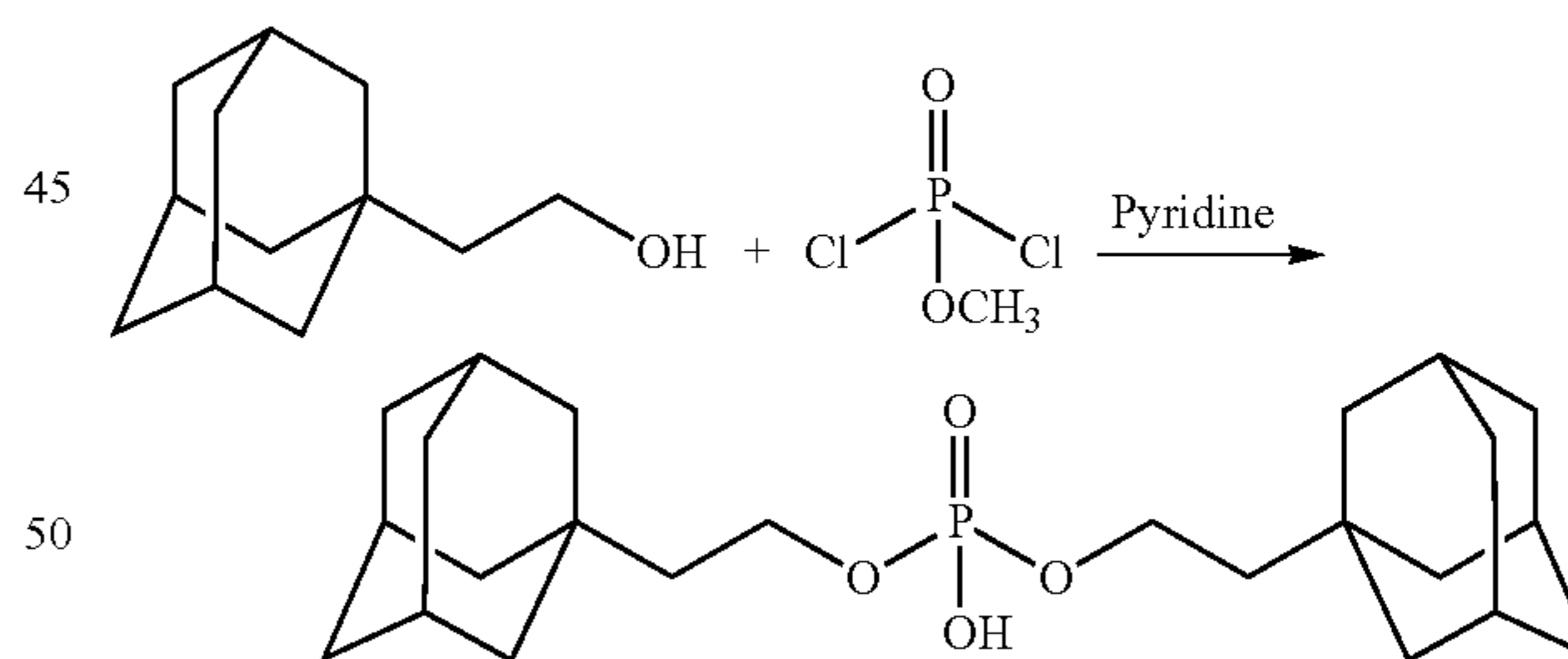
Scheme XXXXVII
