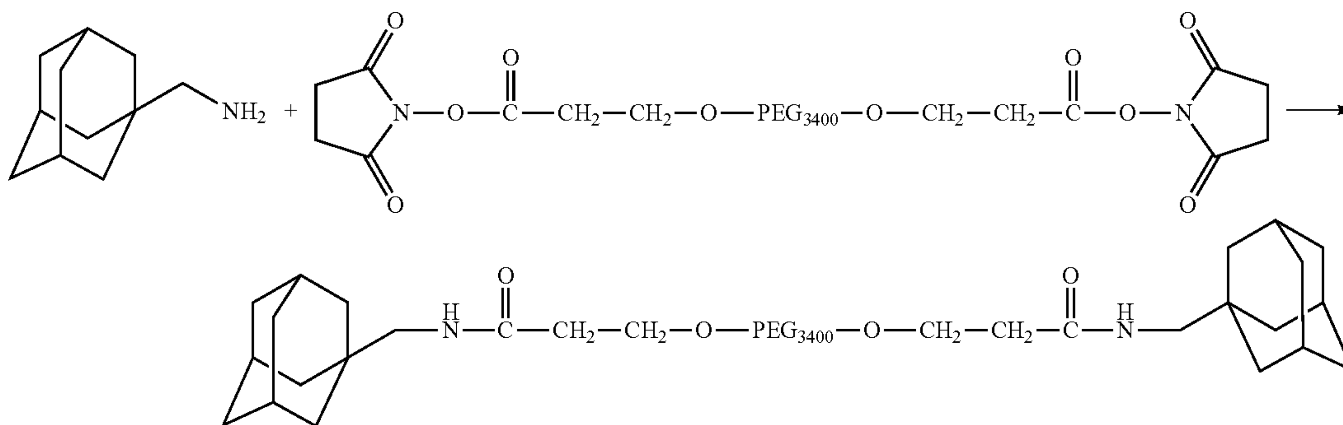
Scheme XXXXVI
