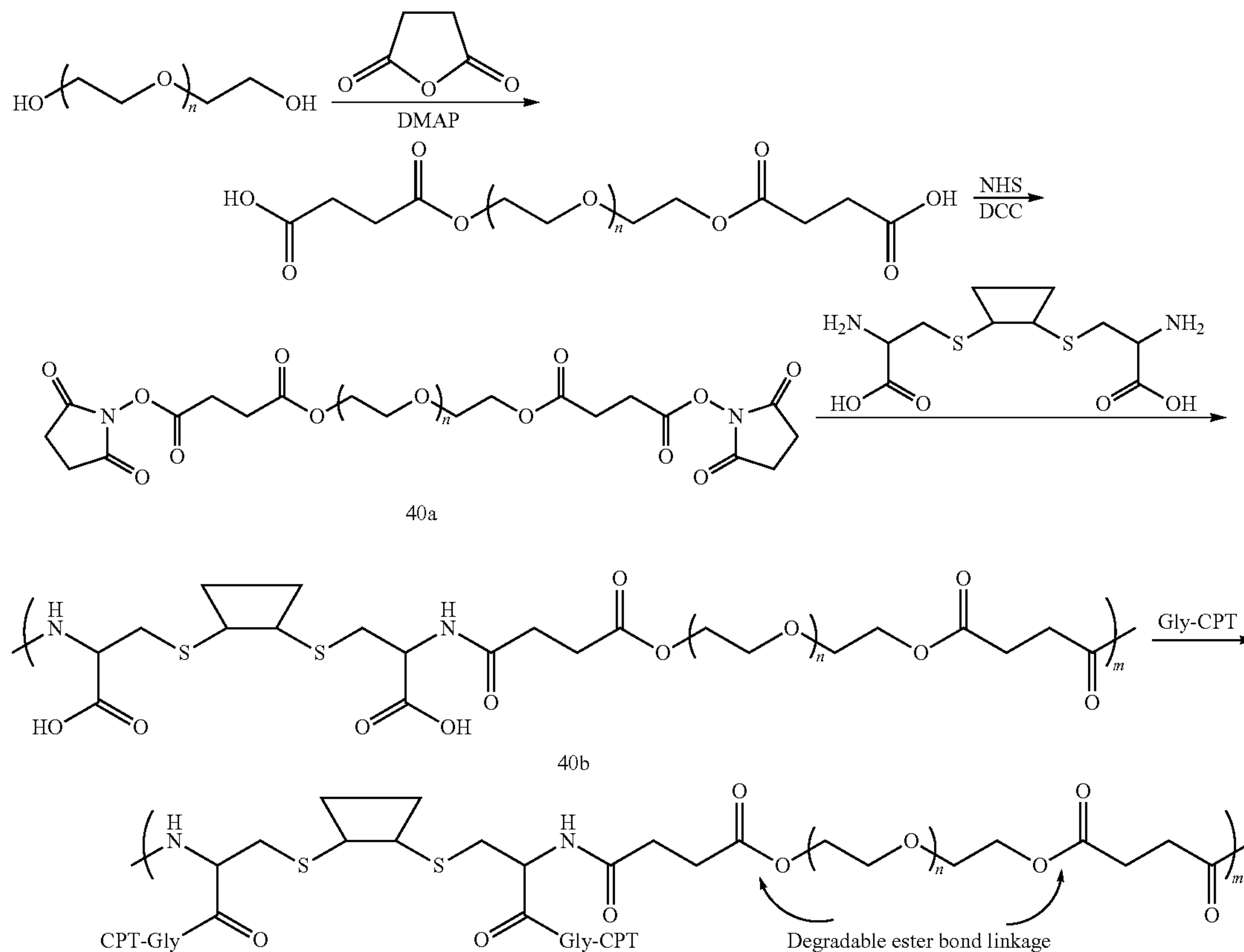
Scheme XXXXI
