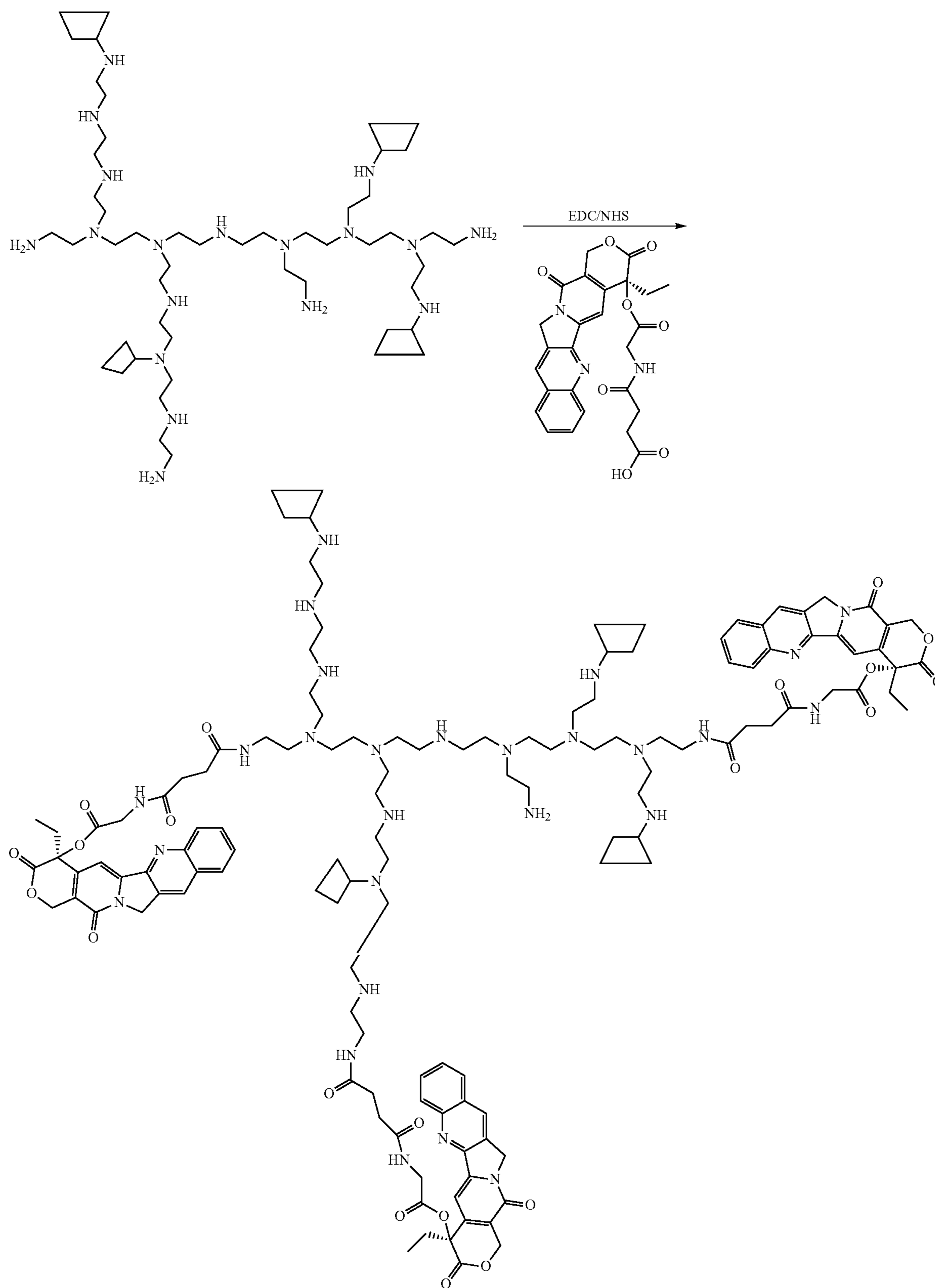
Scheme XXXXV
