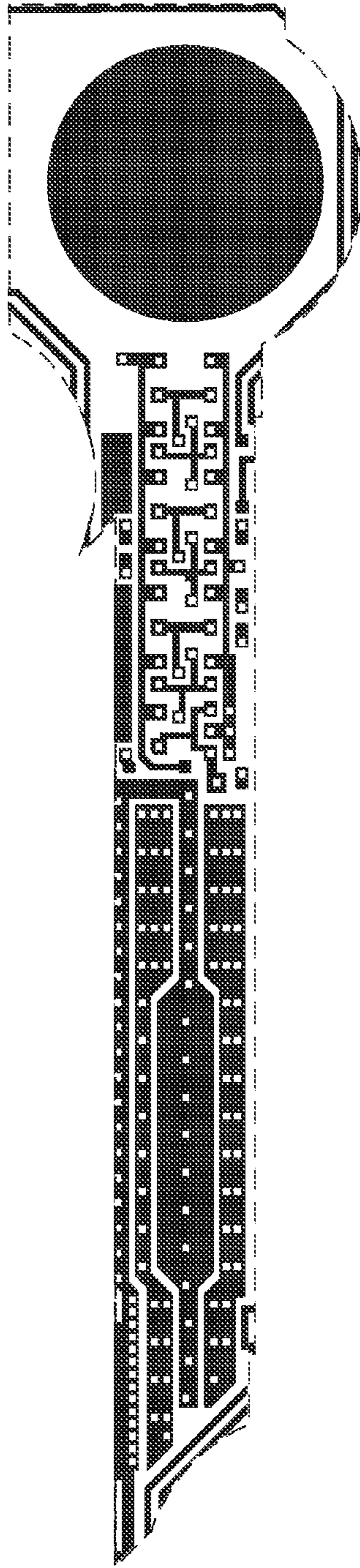
Metal 1 mask
