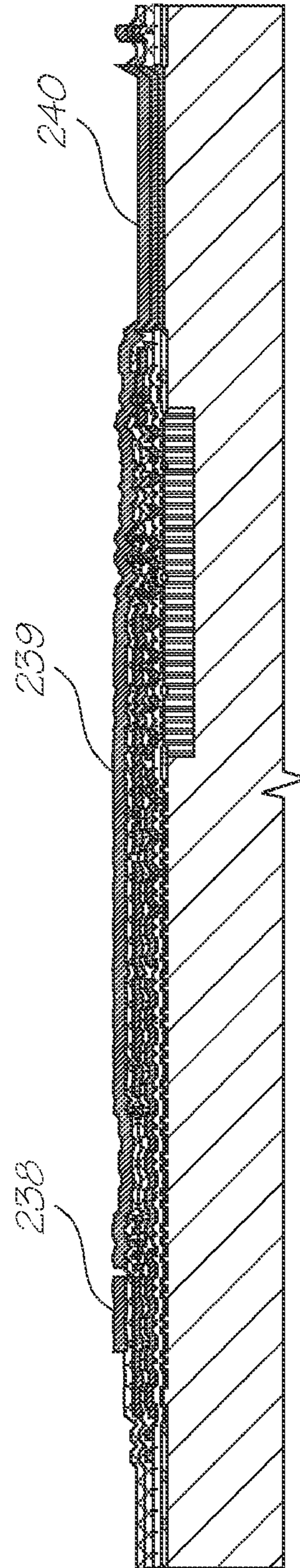
Deposit metal 3
