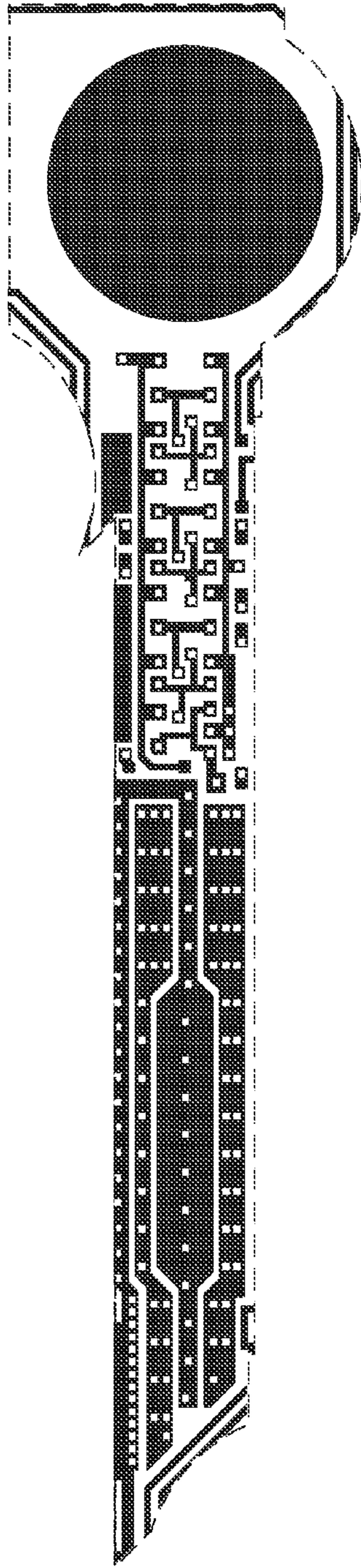
Metal 1 mask
