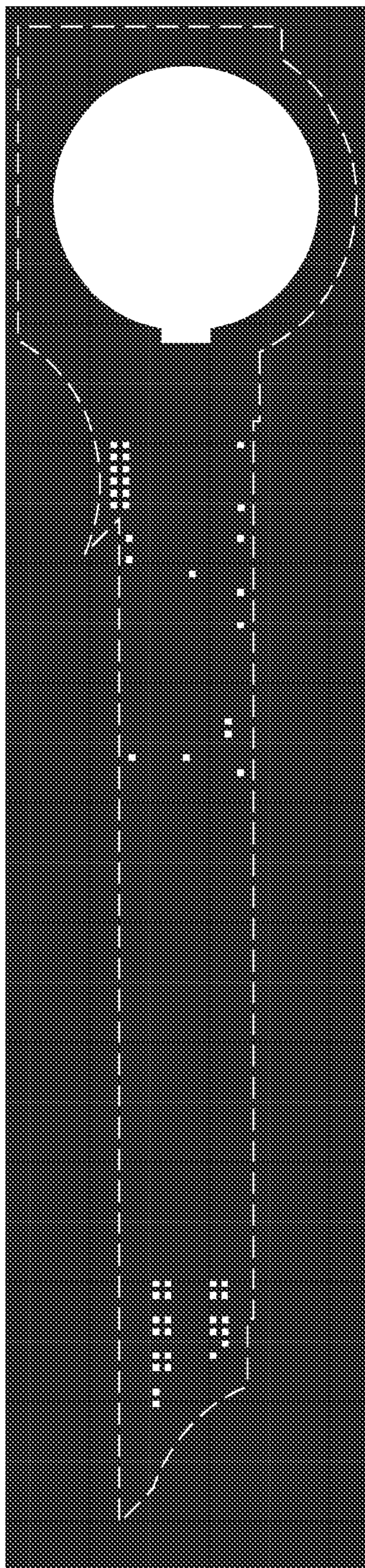
Via 1 mask
