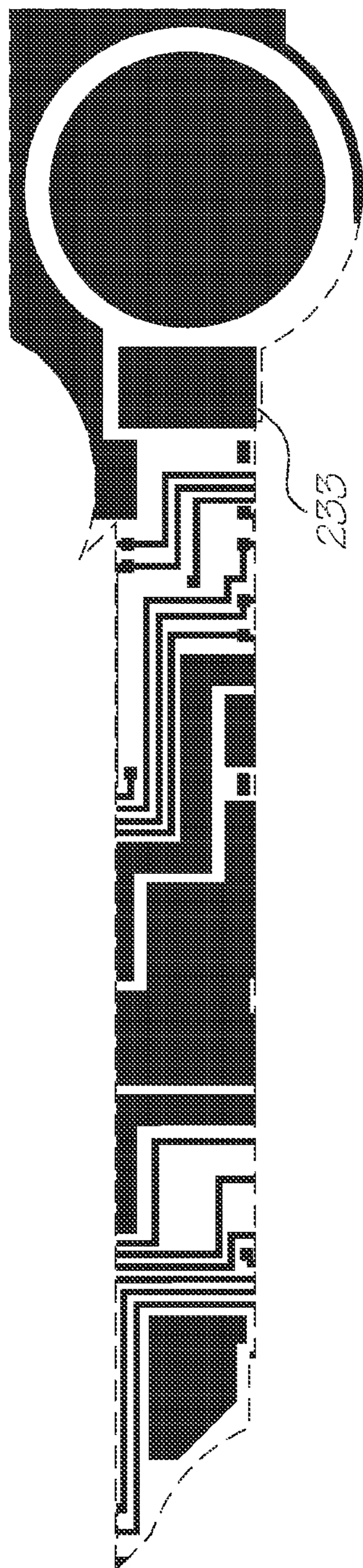
Metal 2 mask
