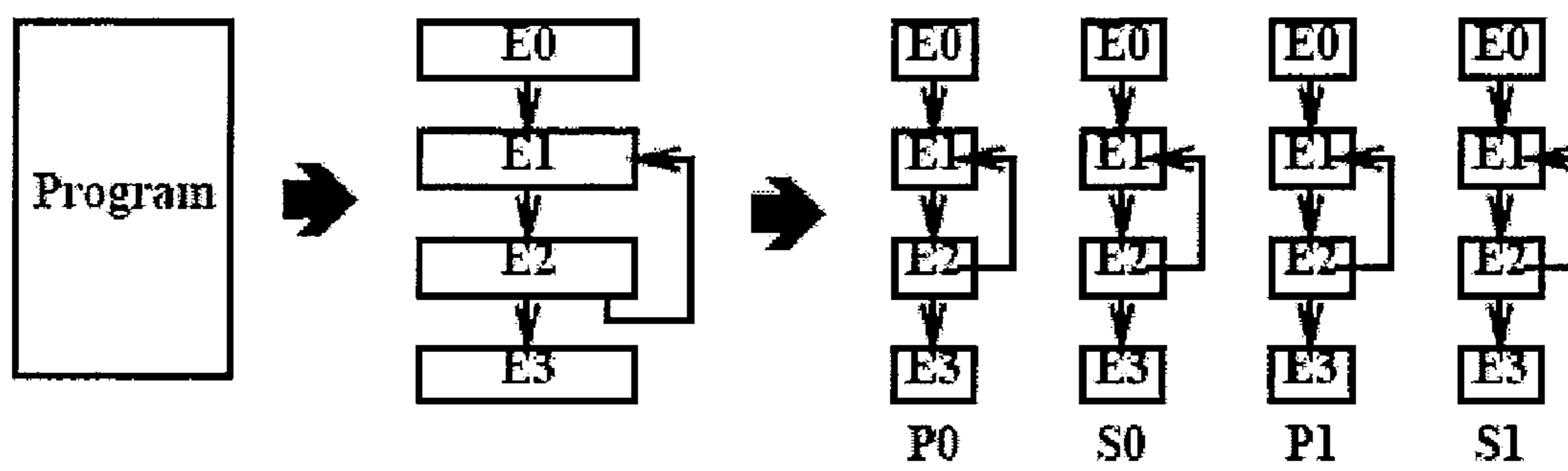
FIG. 3 (a) Compile time
