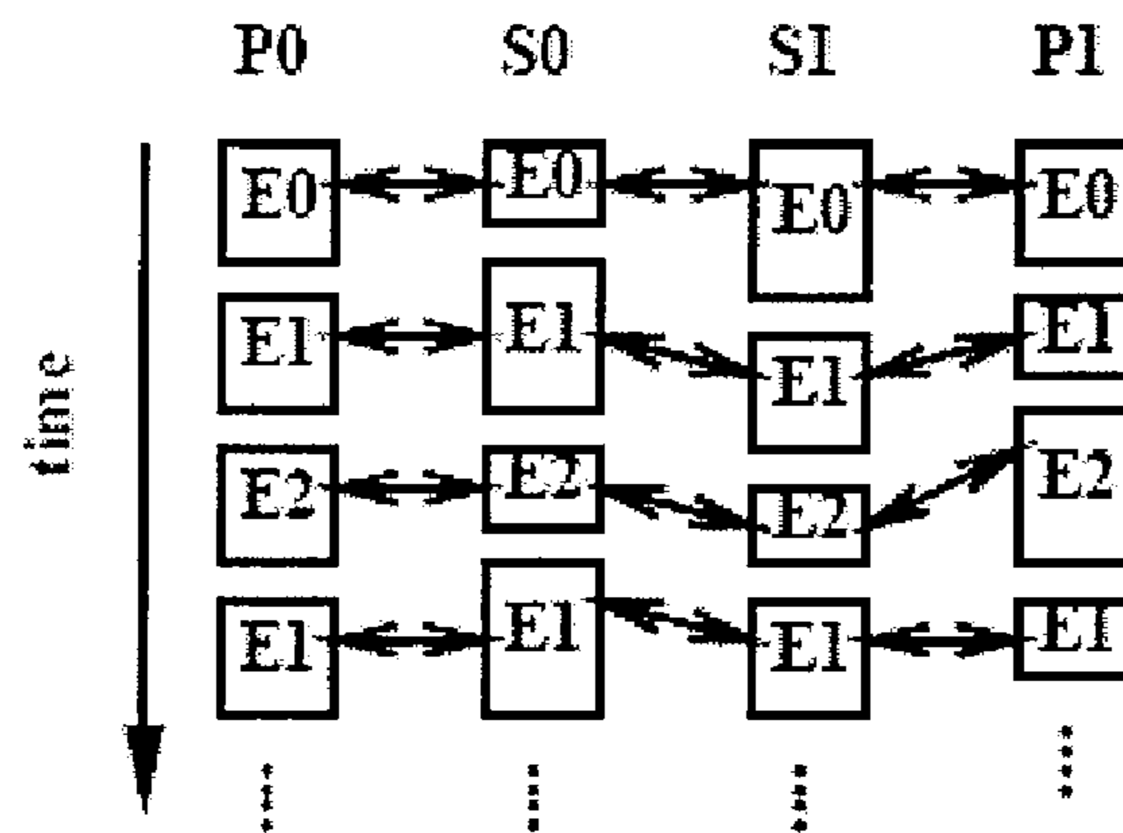
FIG. 3 (b) Run time
