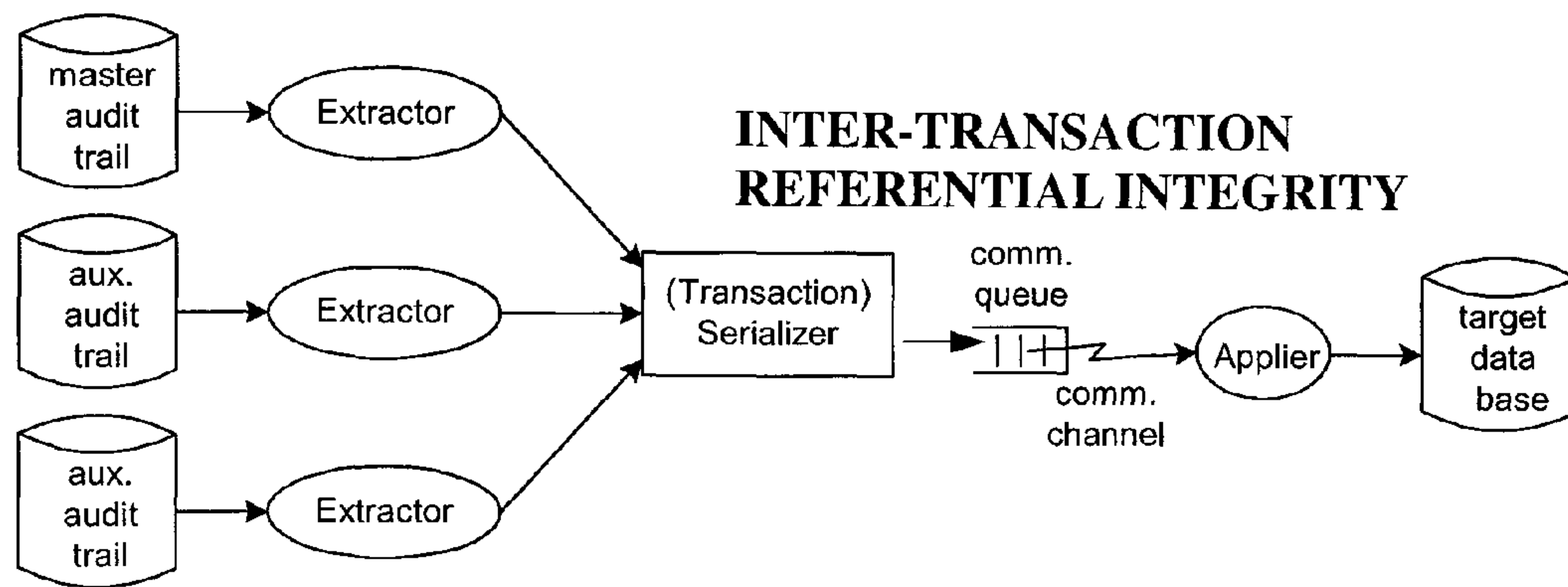
Use of a Transaction Serializer
