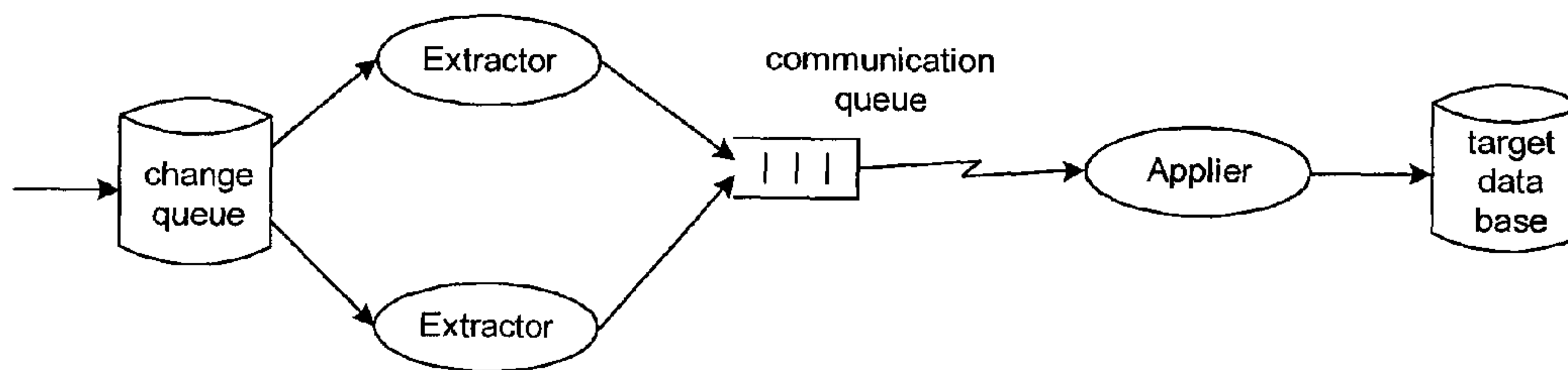
Rules- Based Extractor - Common Comm/Applier Thread
