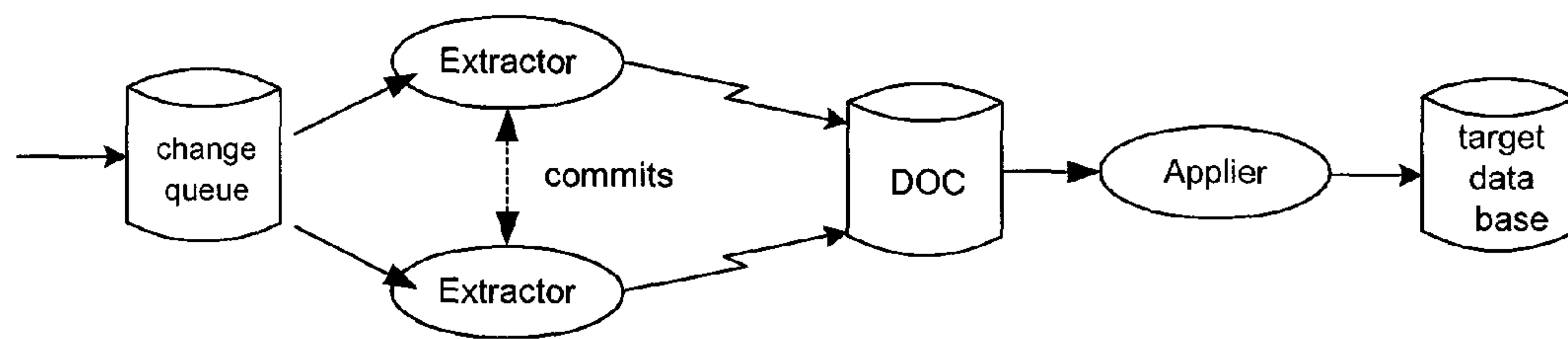
Transaction Serializing with Extractor Coordination
