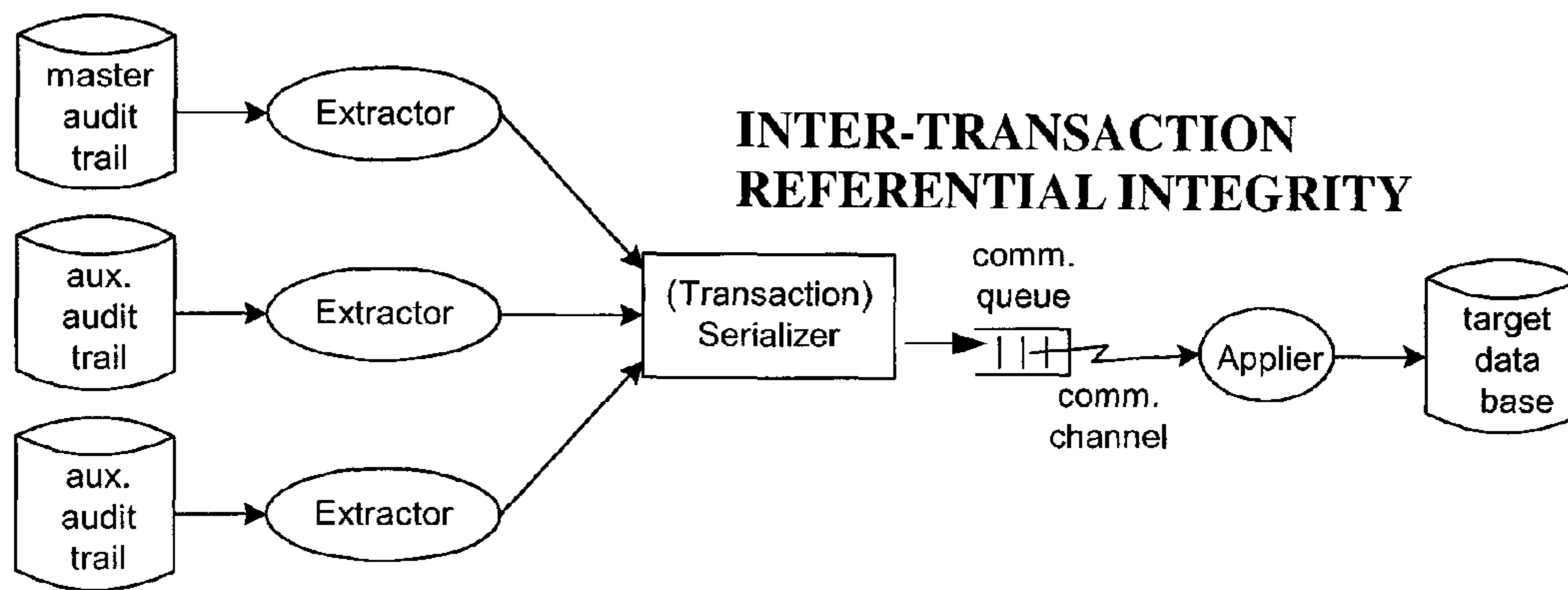
Use of a Transaction Serializer
