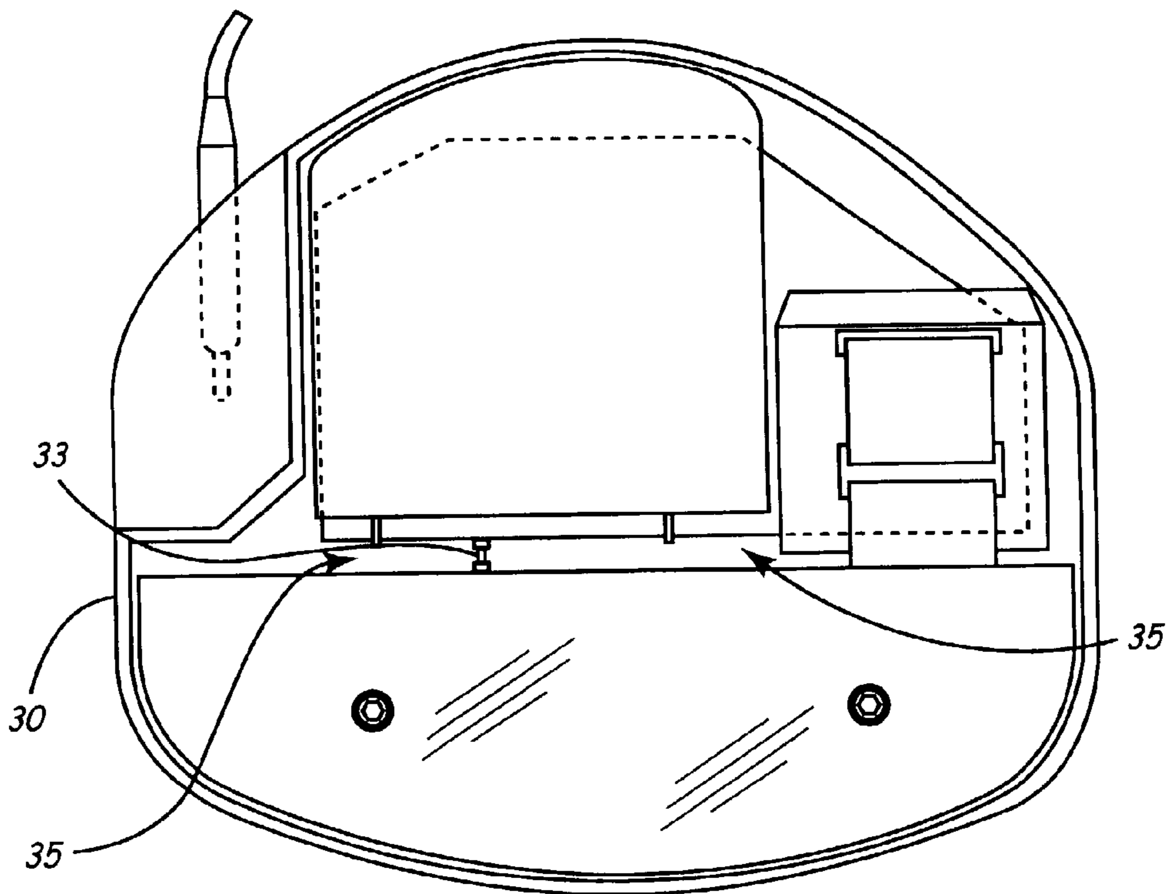
FIG. 2 (PRIOR ART)
