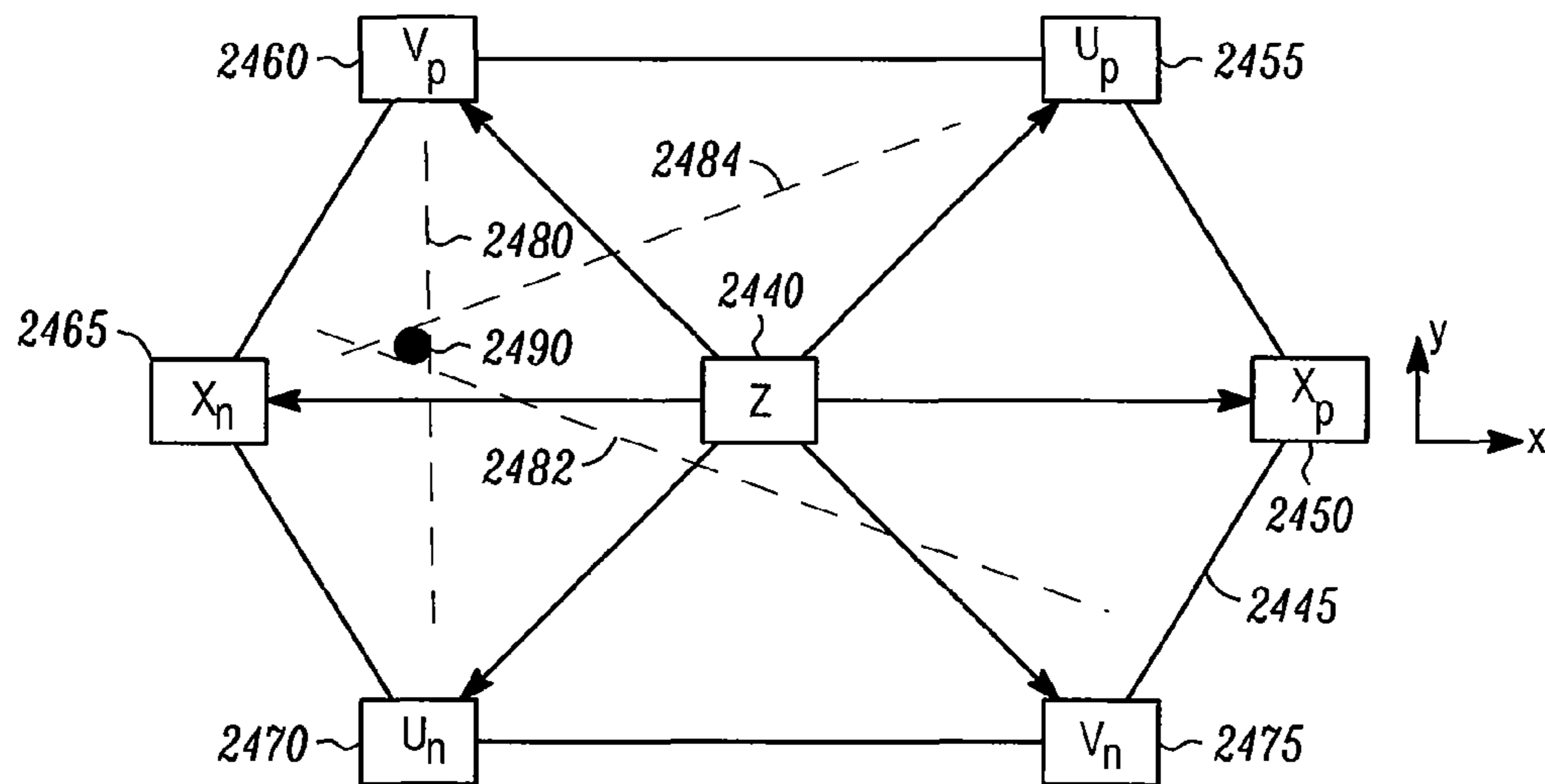
HEXAGONAL INTERPOLATION
