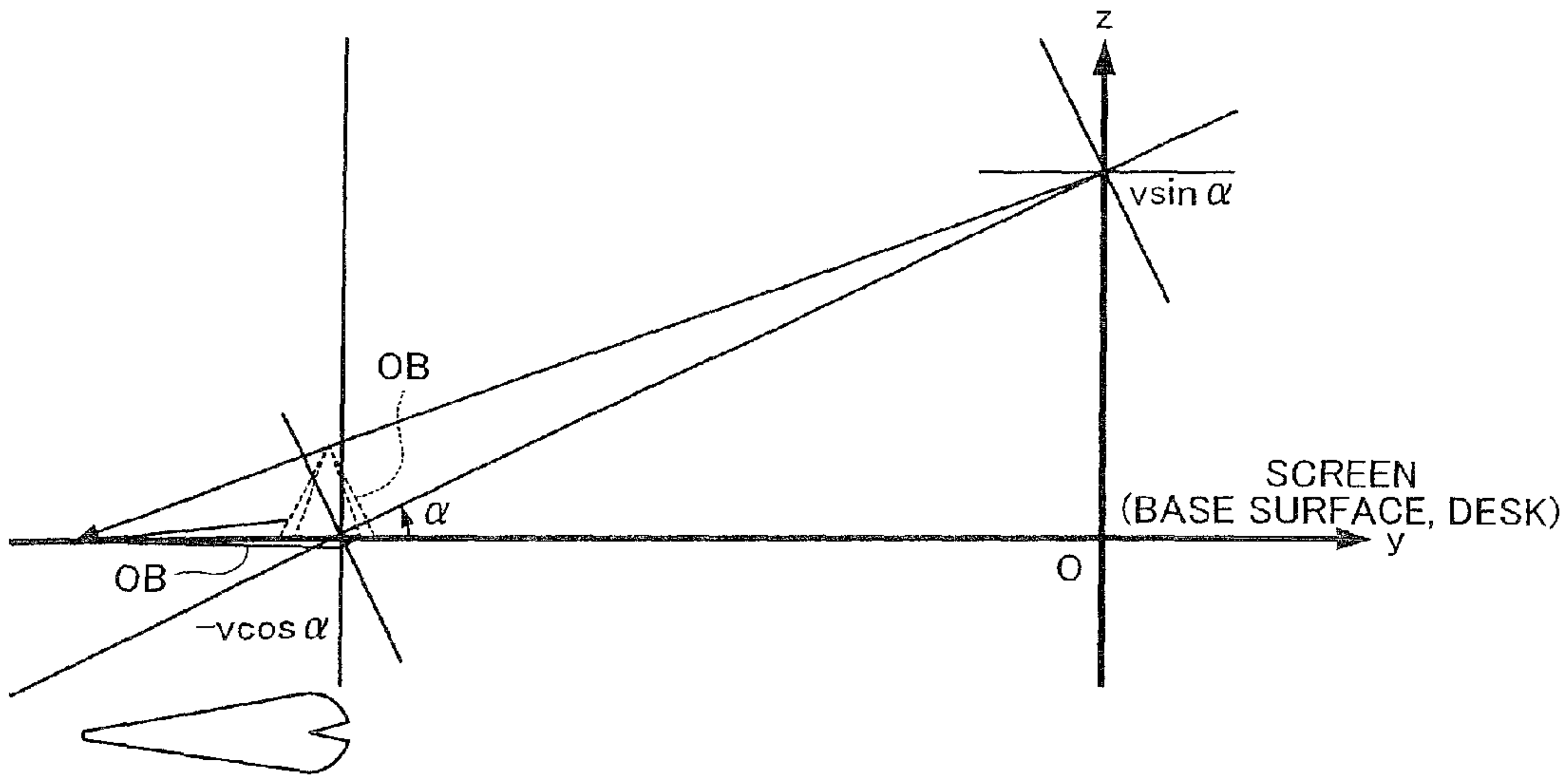
FIG. 25B PROJECTION P_z
