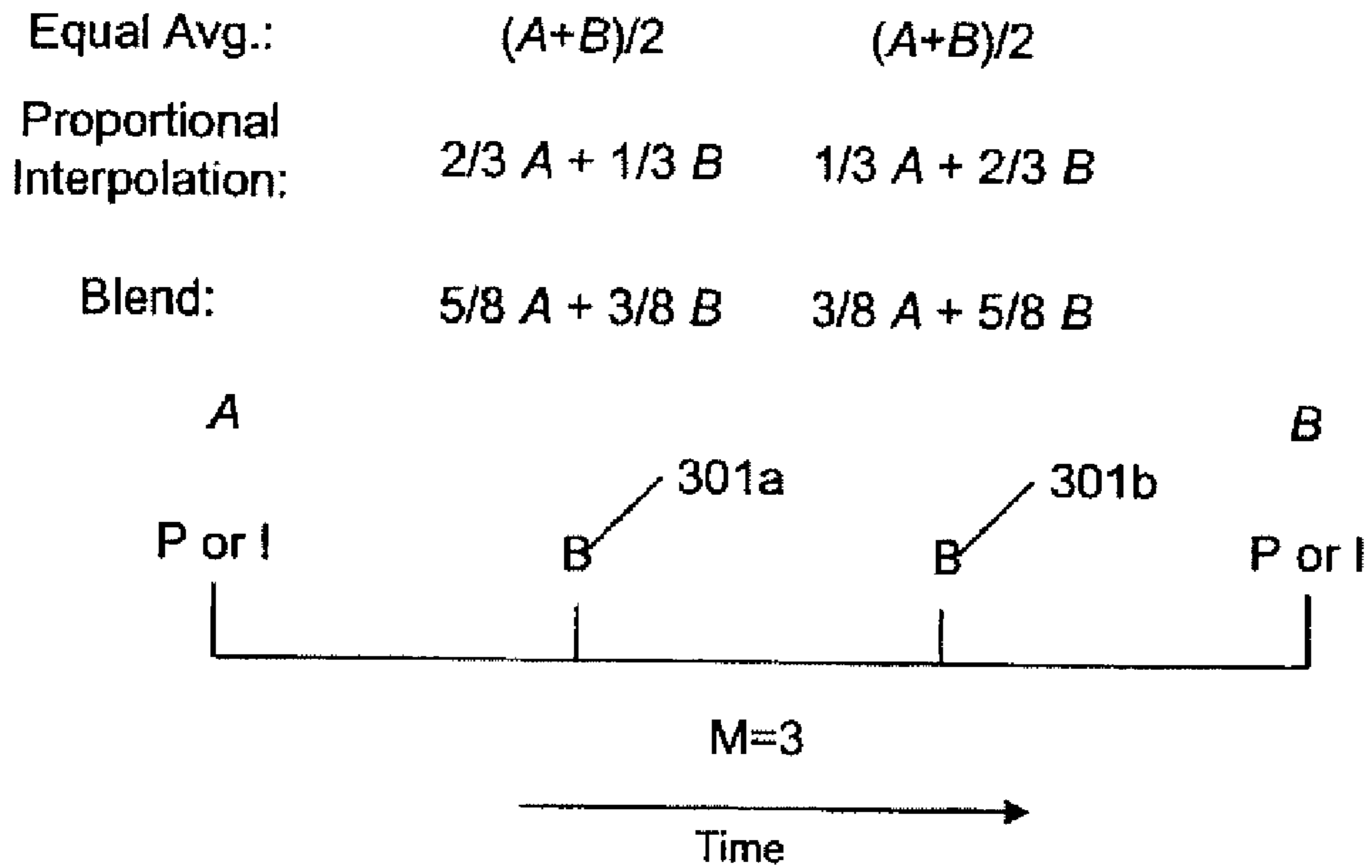
FIG. 3 Blended Pixel Value Weighting
