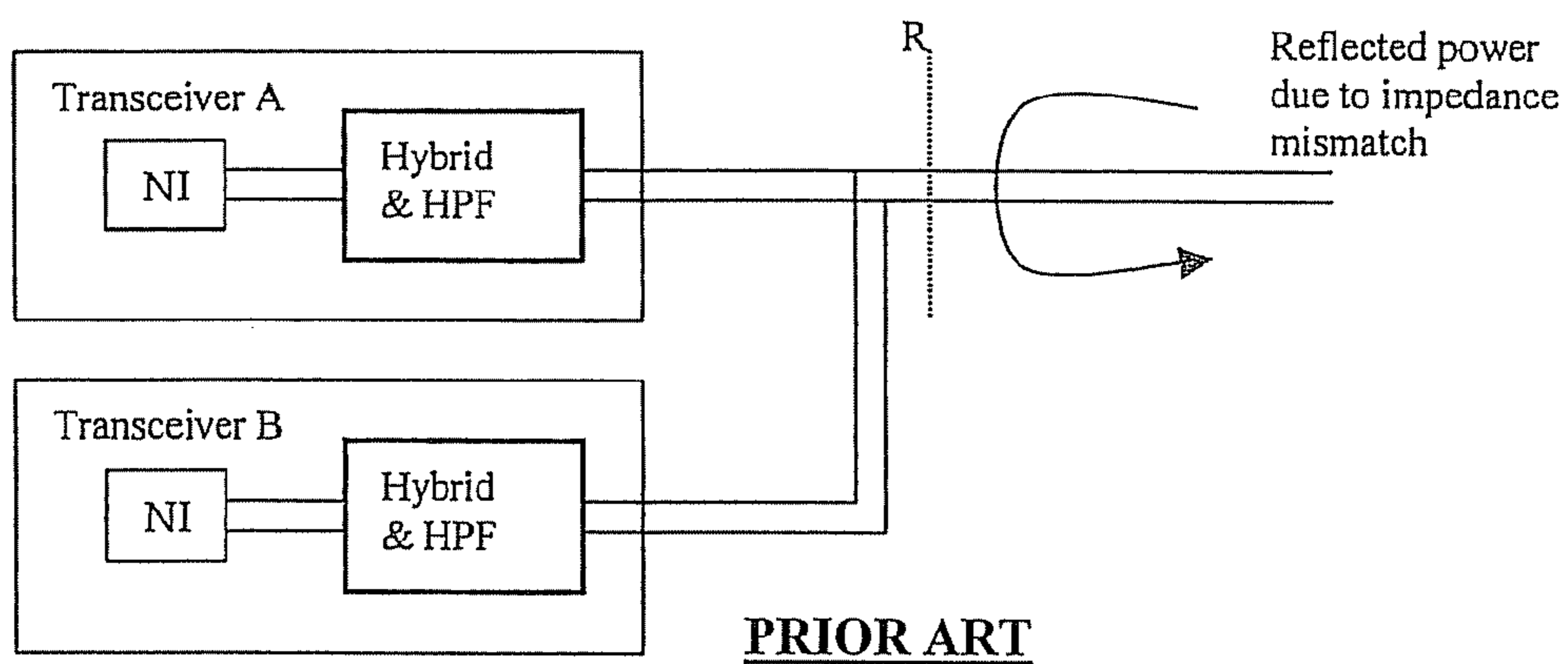
Figure 5: Echo of the Received Signal
