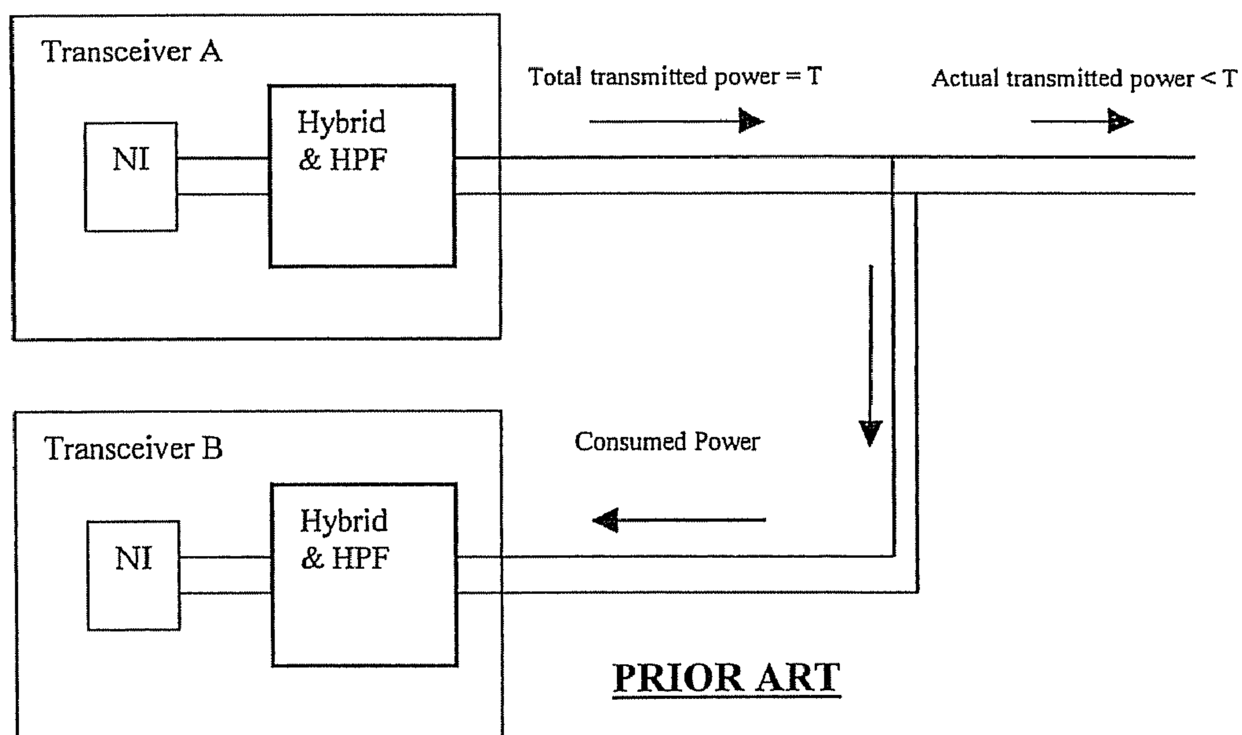
Figure 3: Attenuation of Transmitted Signal
