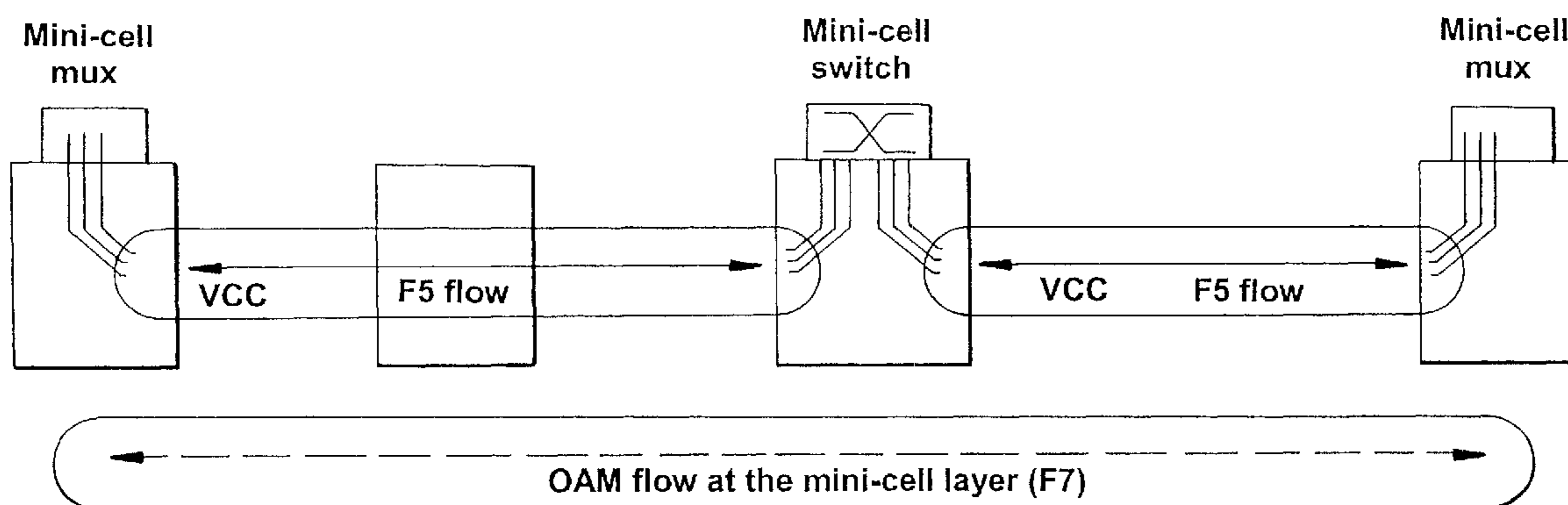
Switching of AAL-CU Packets
