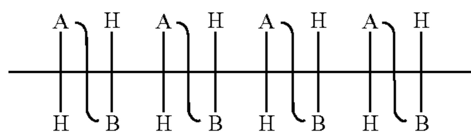
threodiisotactic homopolymer
