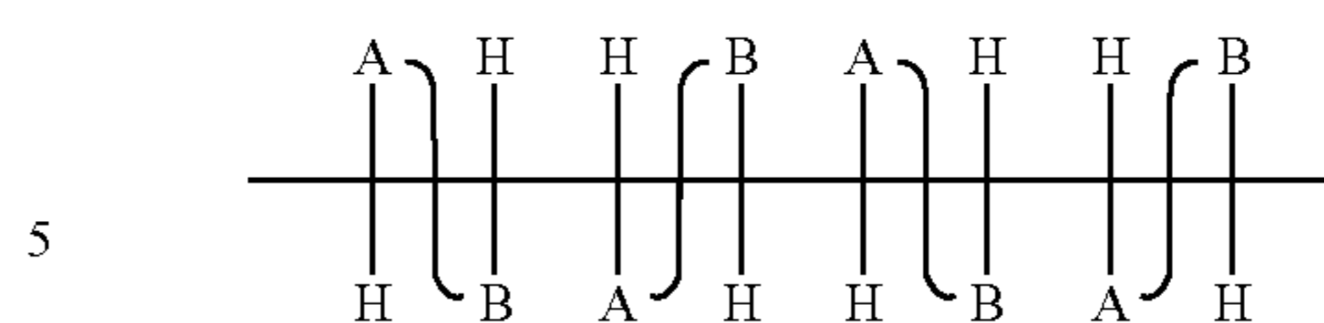
threodisyndiotactic homopolymer
