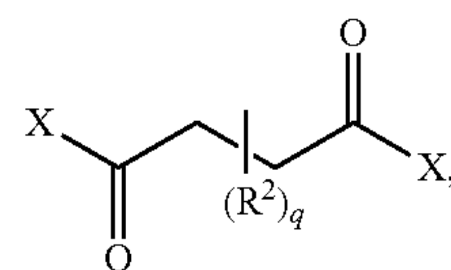
succinyl dihaloanhydride
