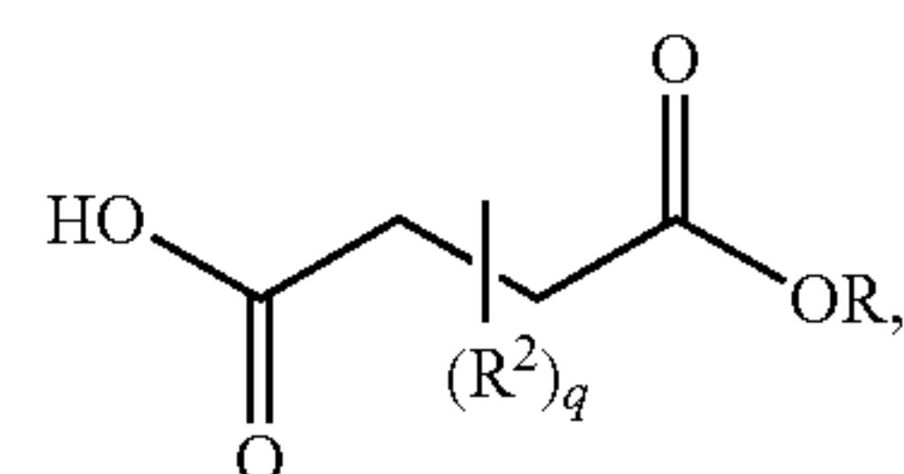
succinic ester
