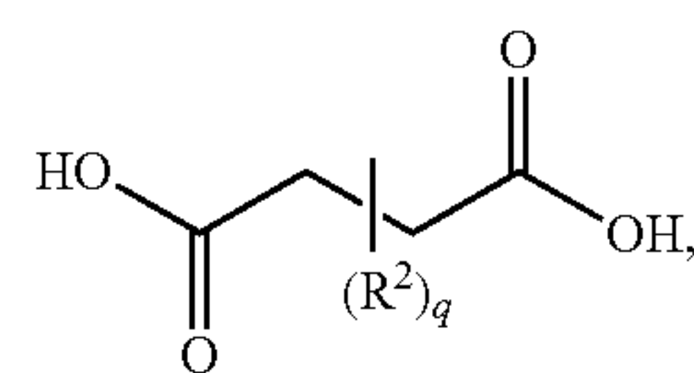
succinyl dihaloanhydride
