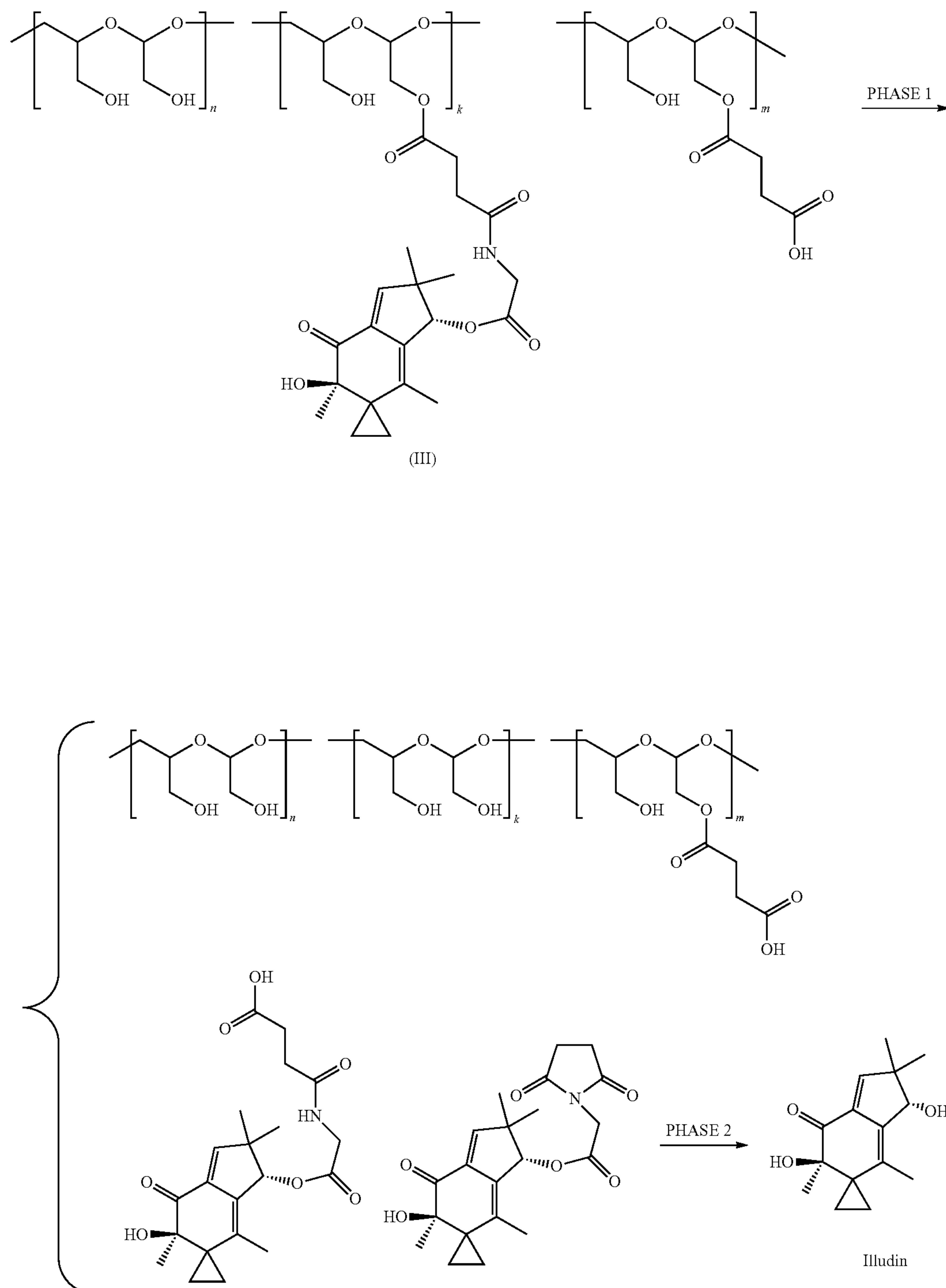
Scheme 5
