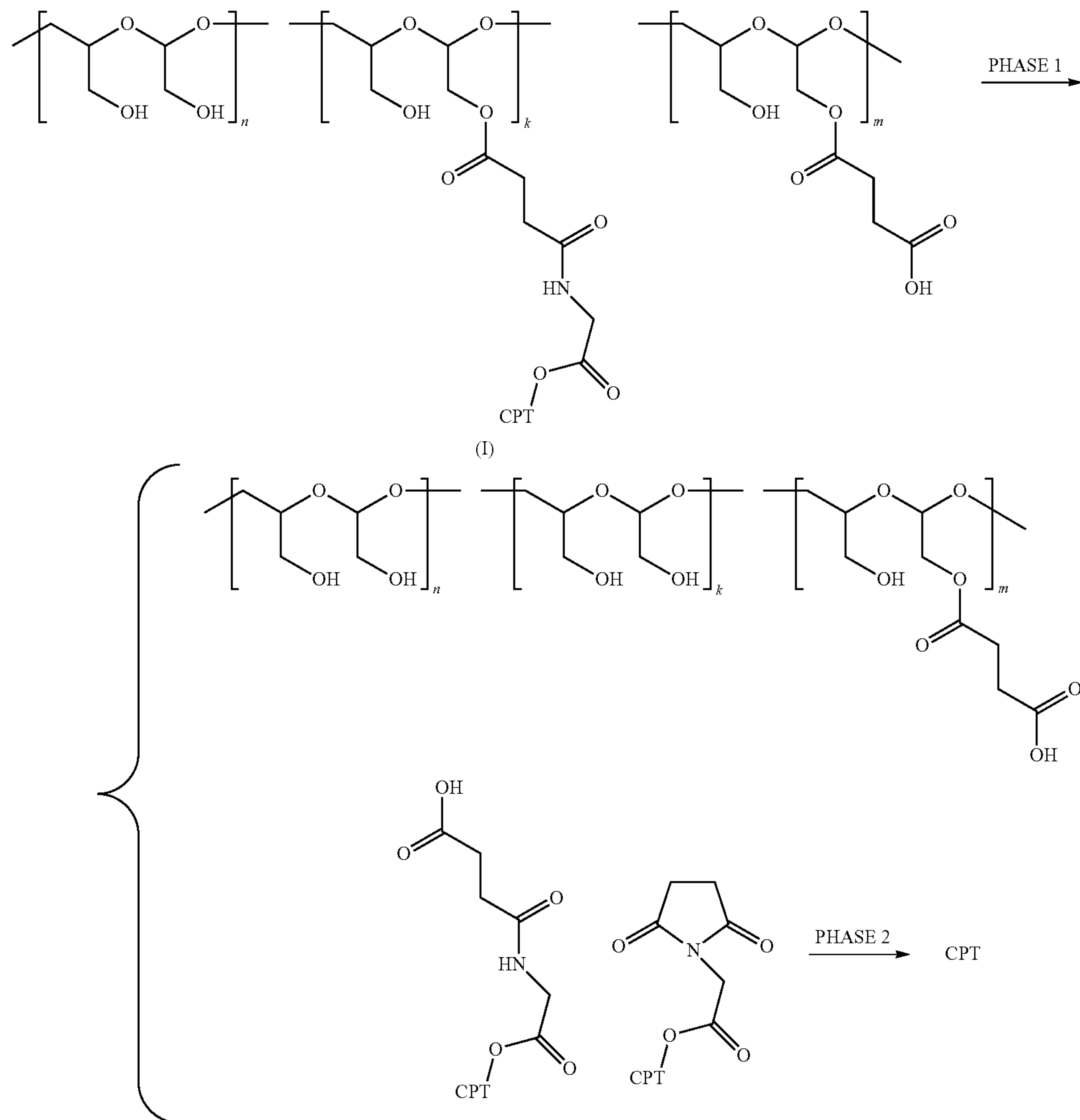
Scheme 3
