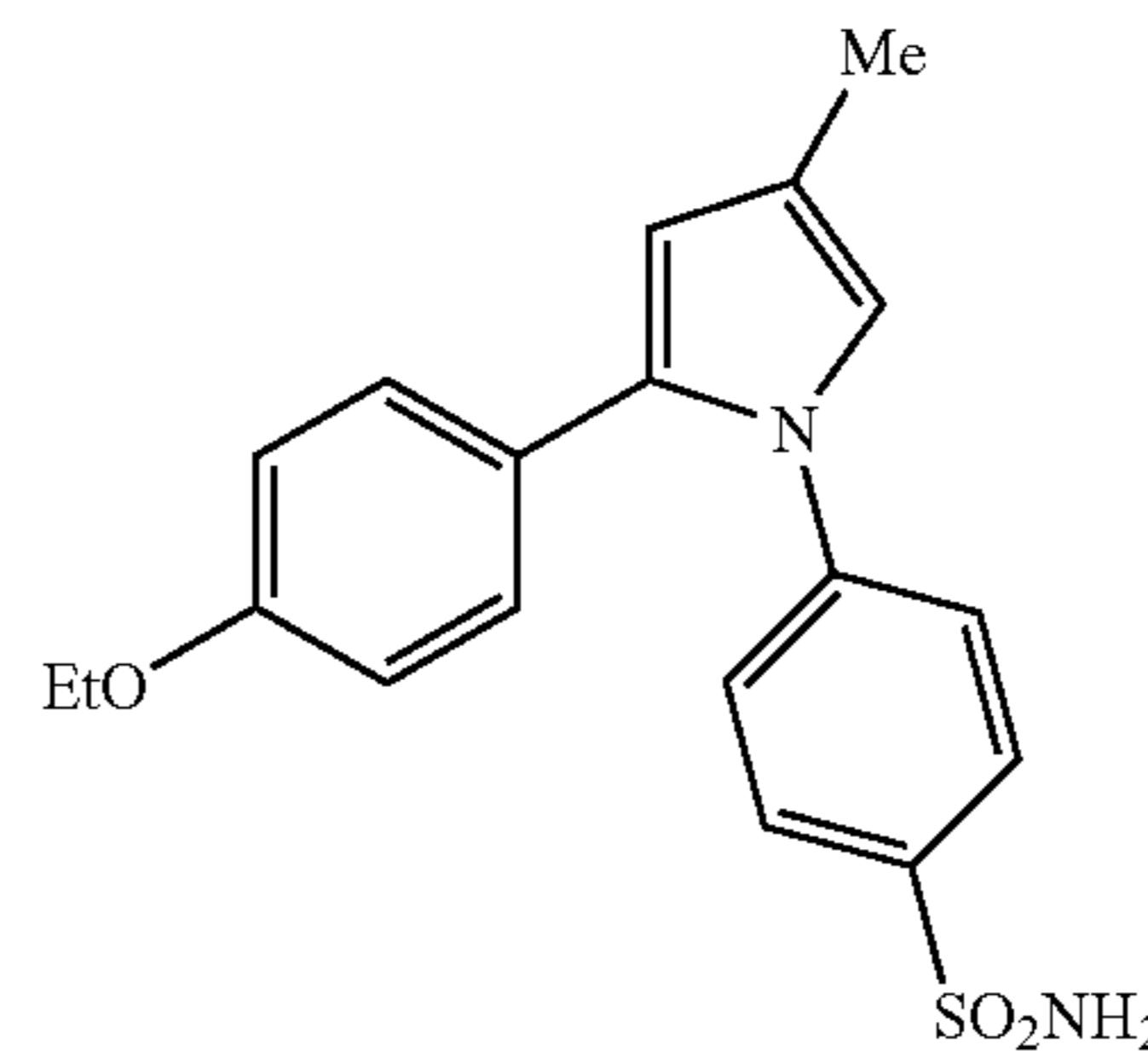
2-(4-ethoxyphenyl)-4-methyl-1-(4-sulfamoylphenyl)-pyrrole
