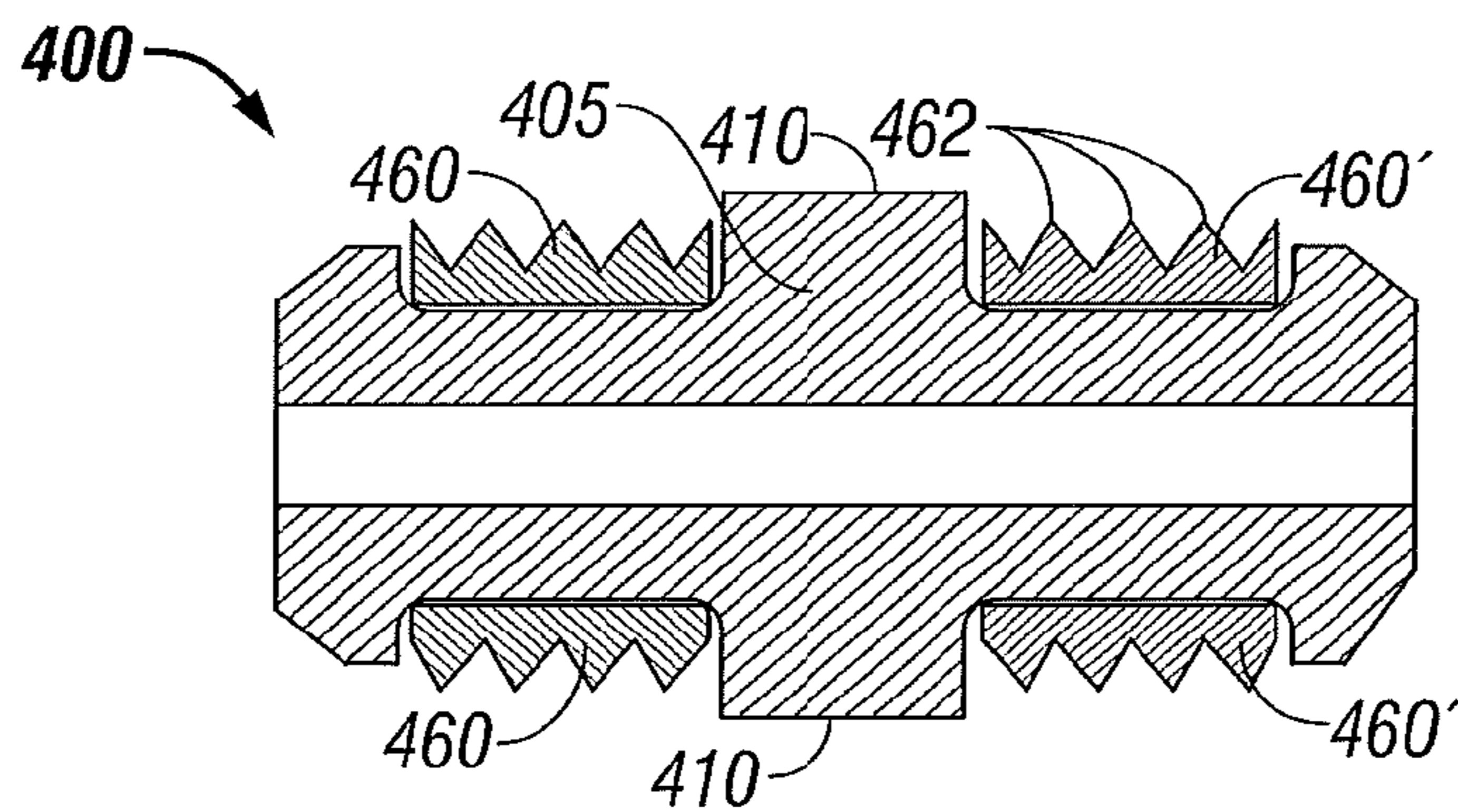
Section B-B
