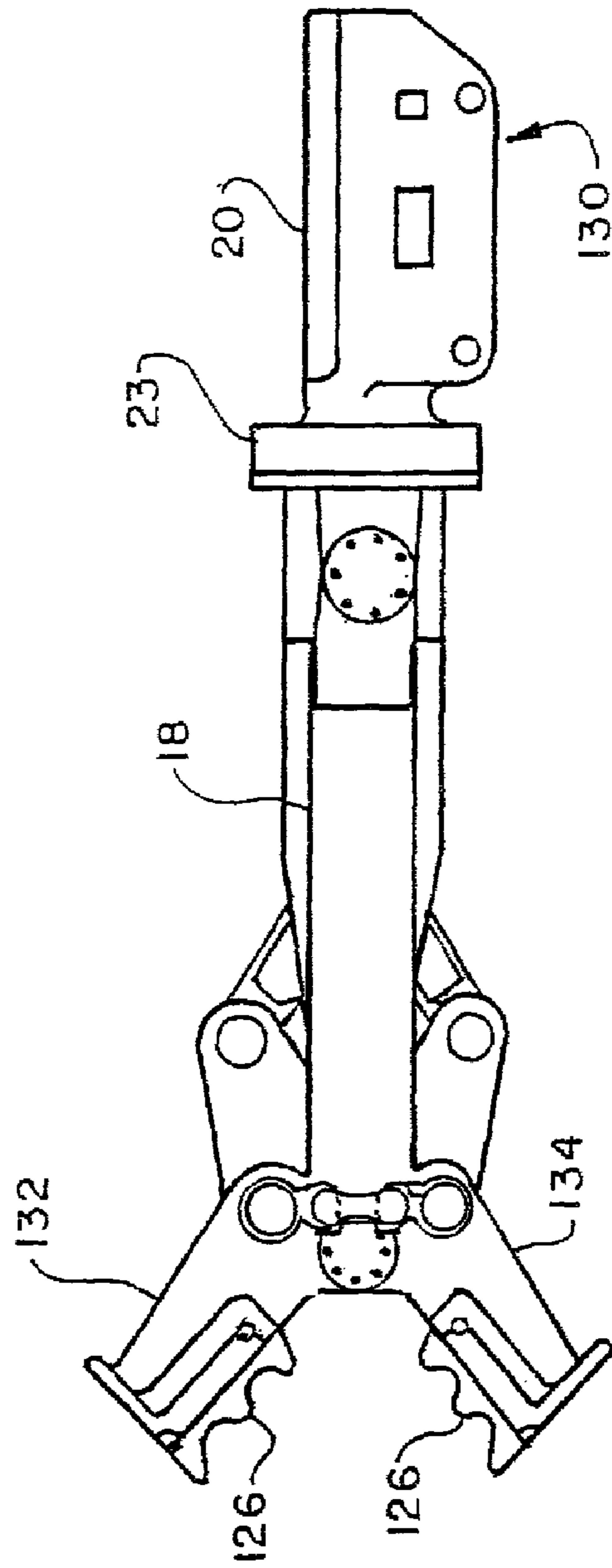
CONCRETE PULVERIZER
