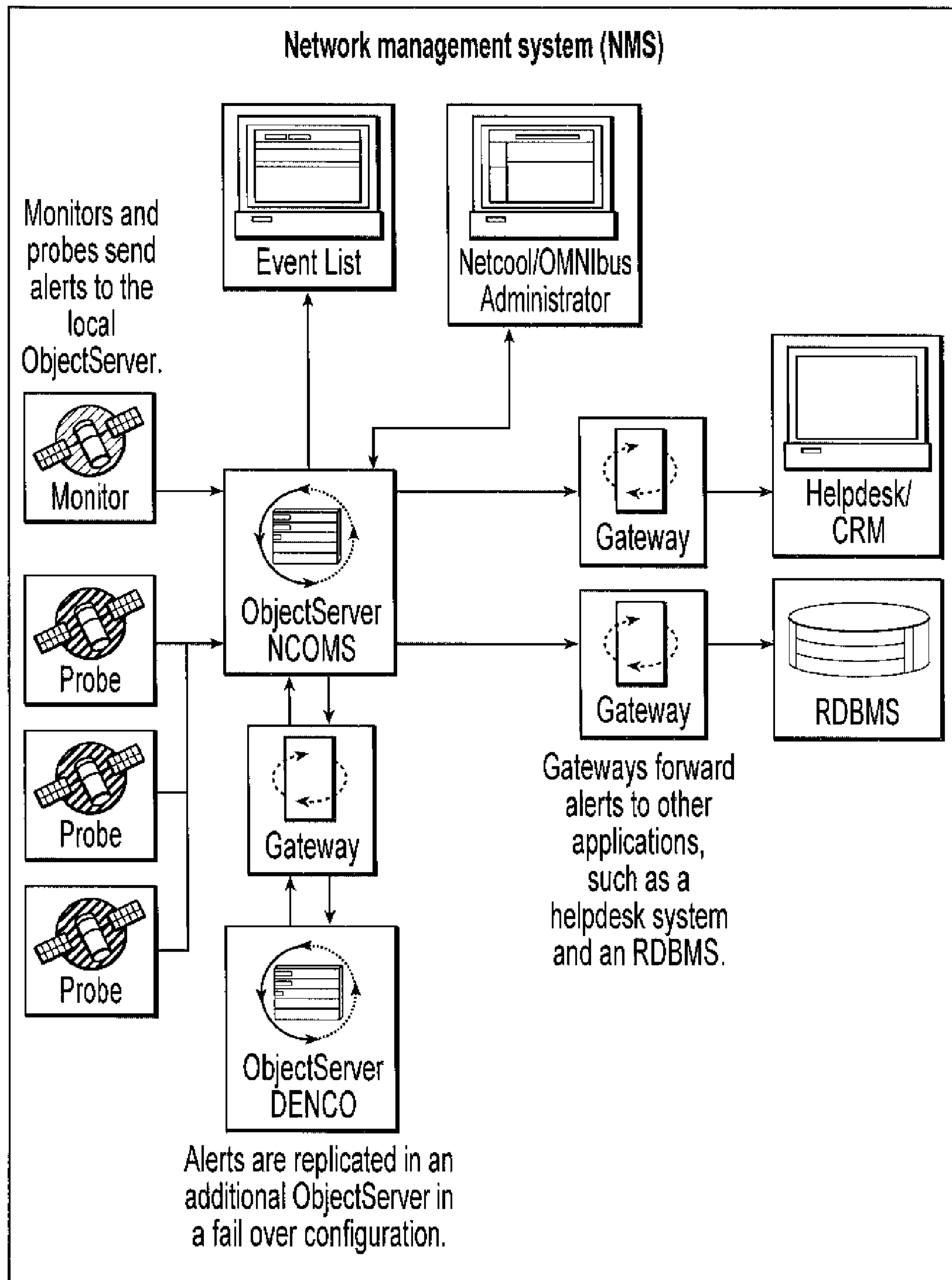
FIG. 1 PRIOR ART
