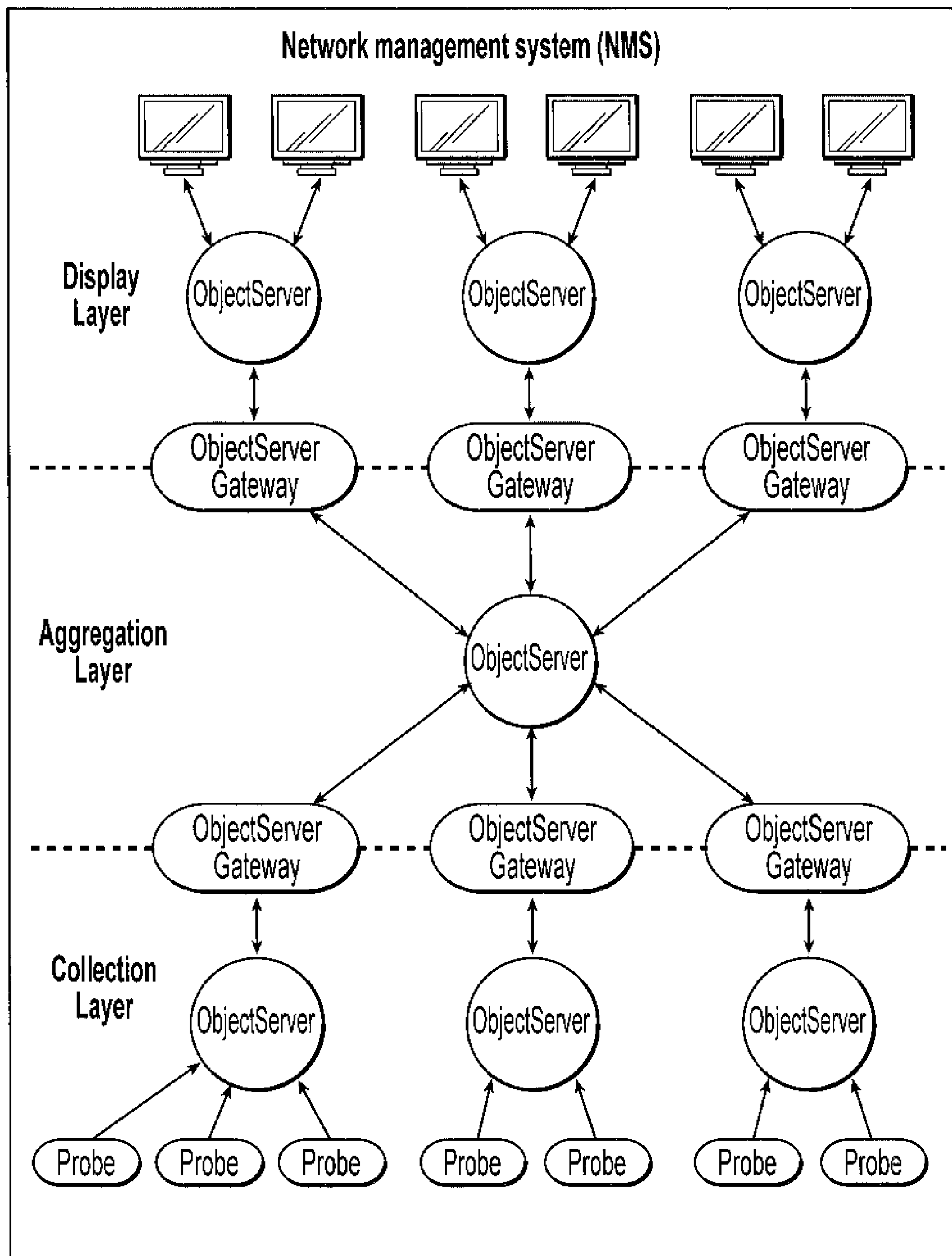
FIG. 2 PRIOR ART
