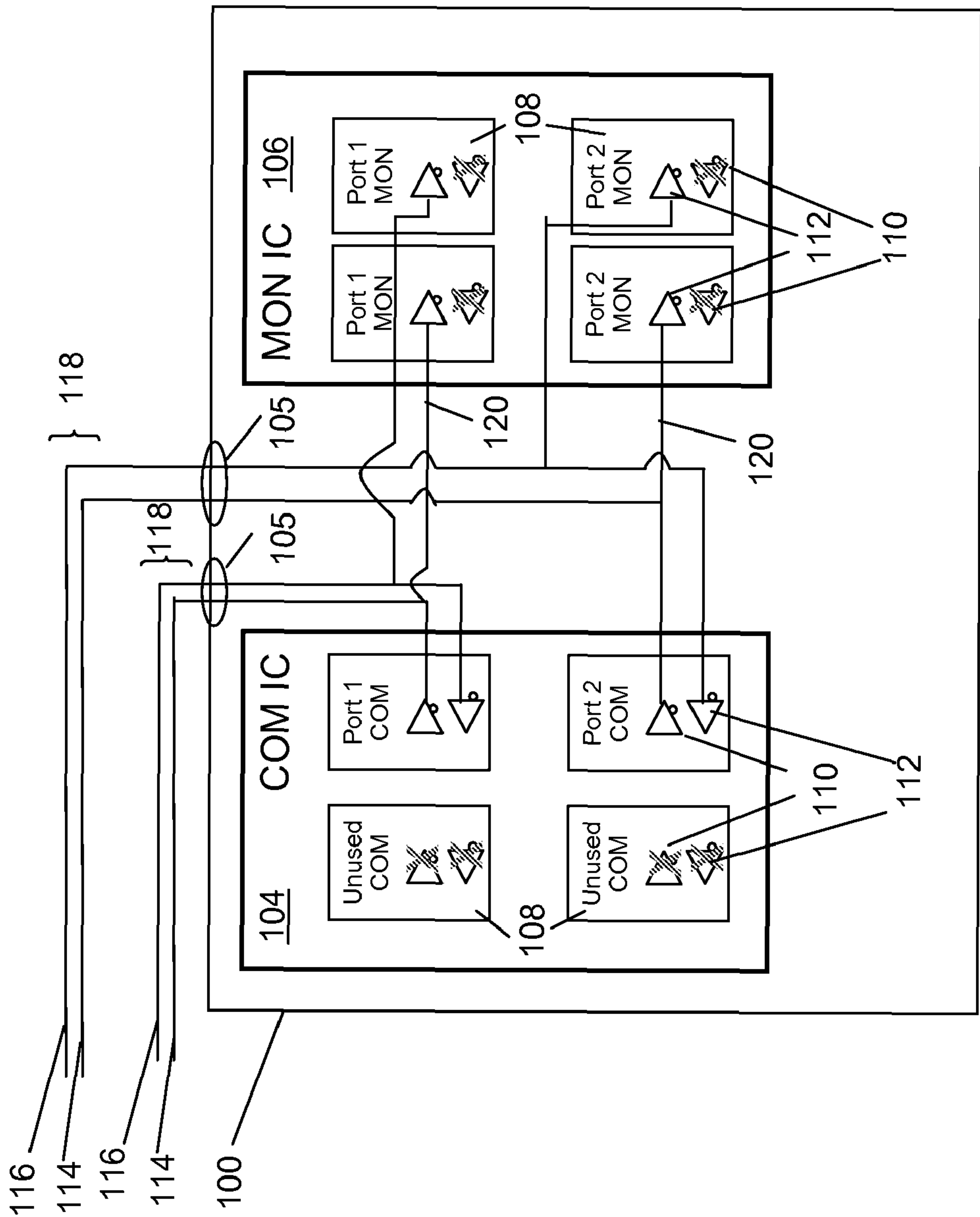
Fig. 1 (Prior Art)
