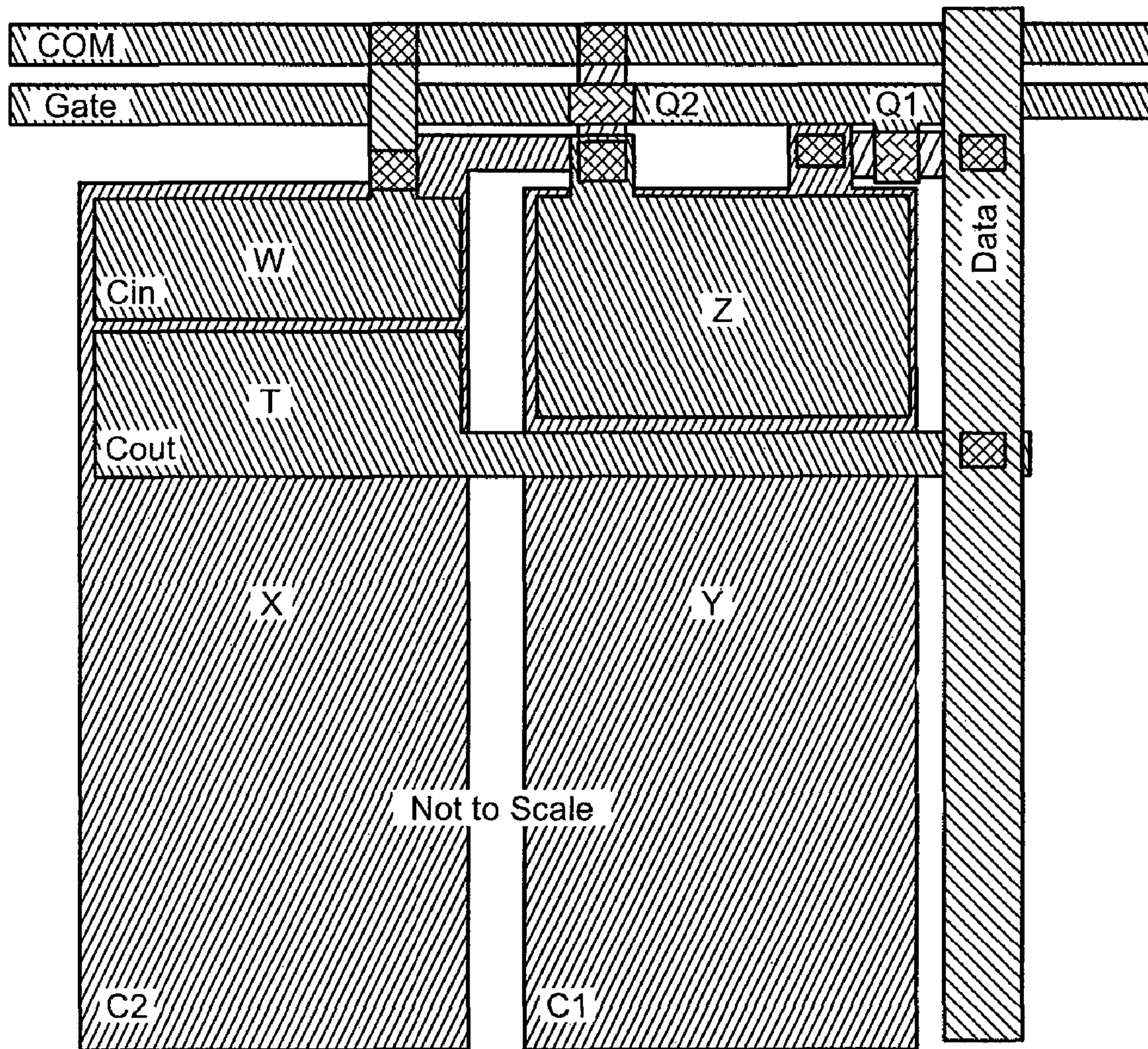
Subpixel Layout
