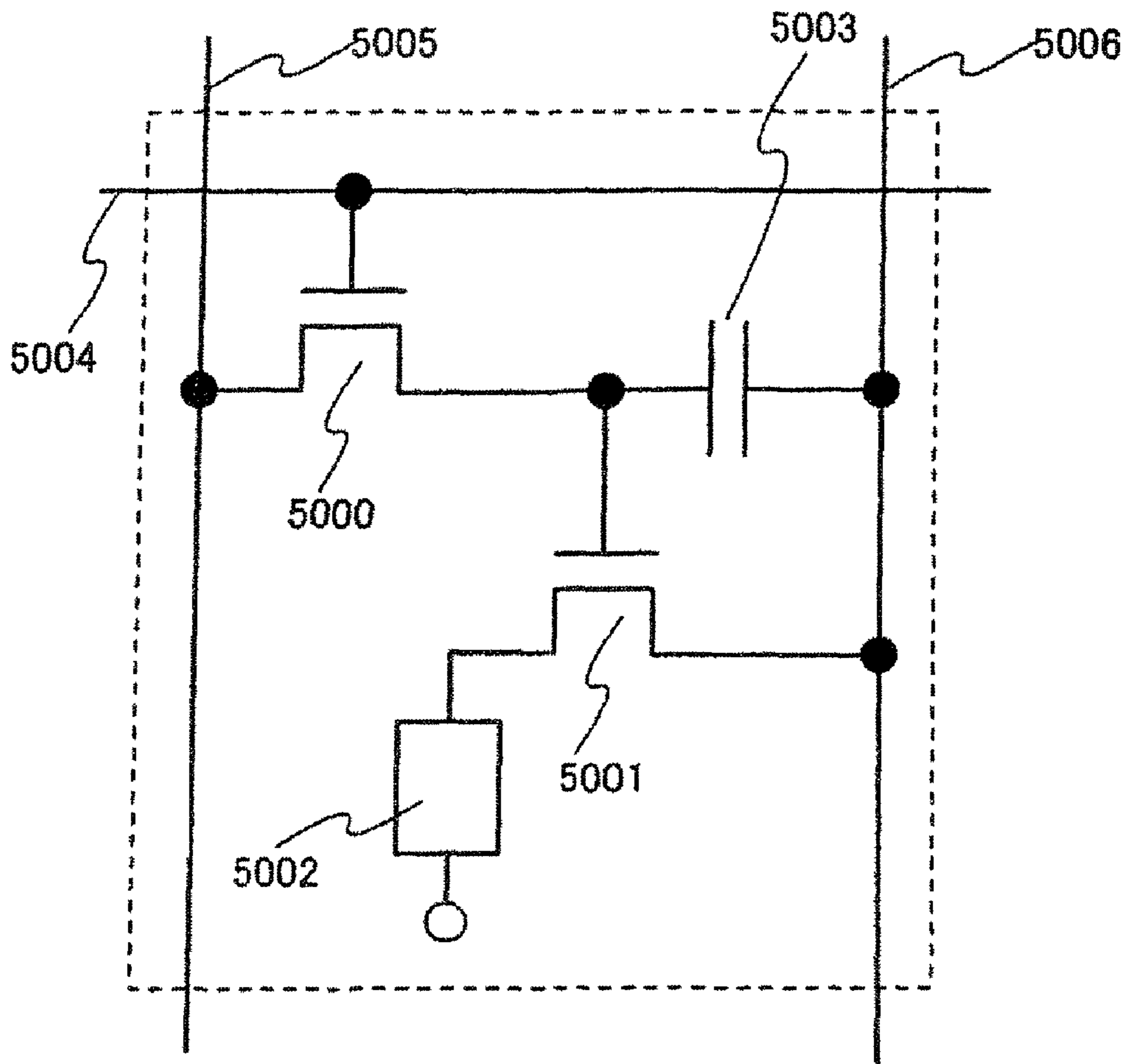
Fig. 18 PRIOR ART
