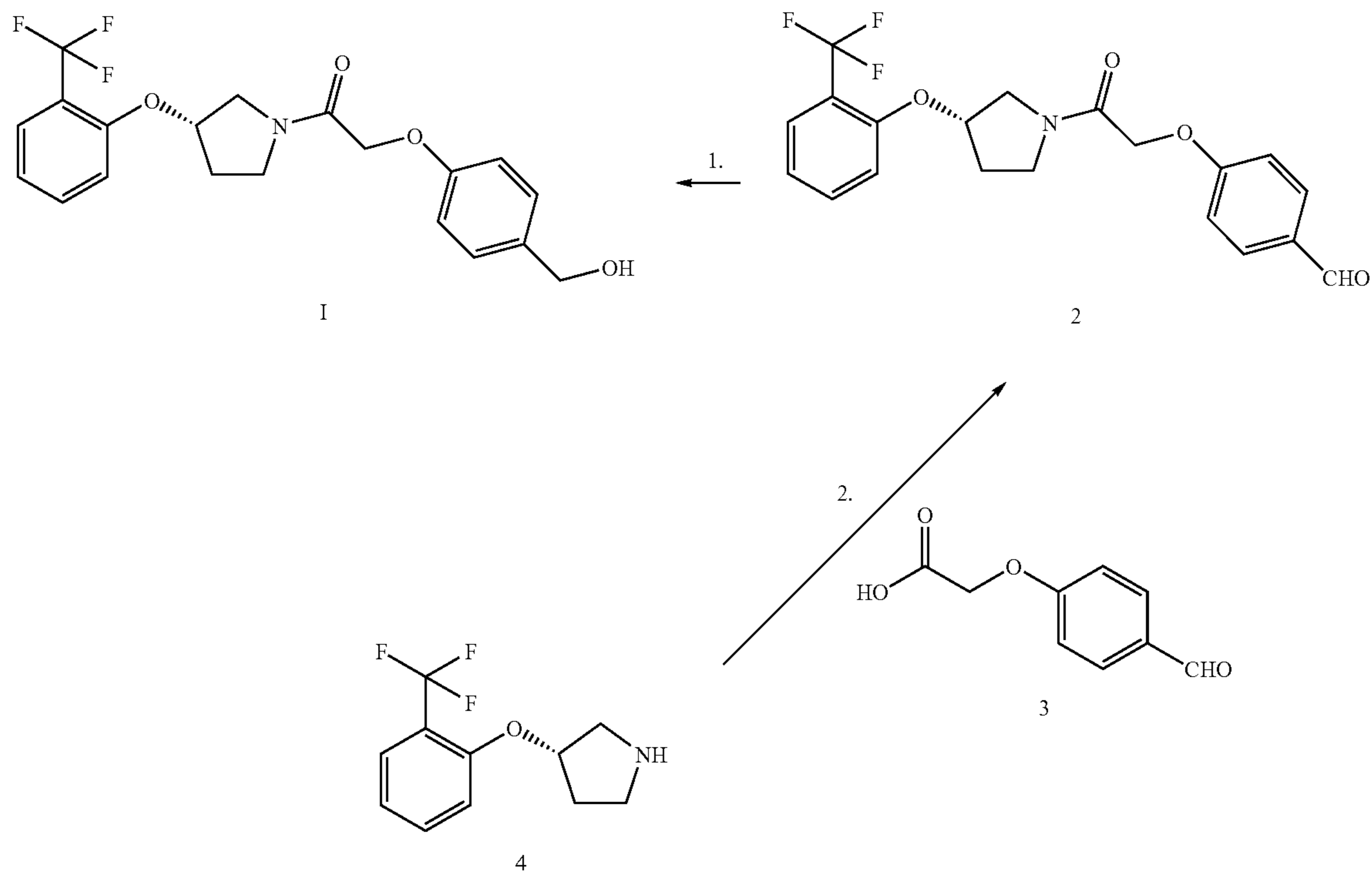
SCHEME 1
