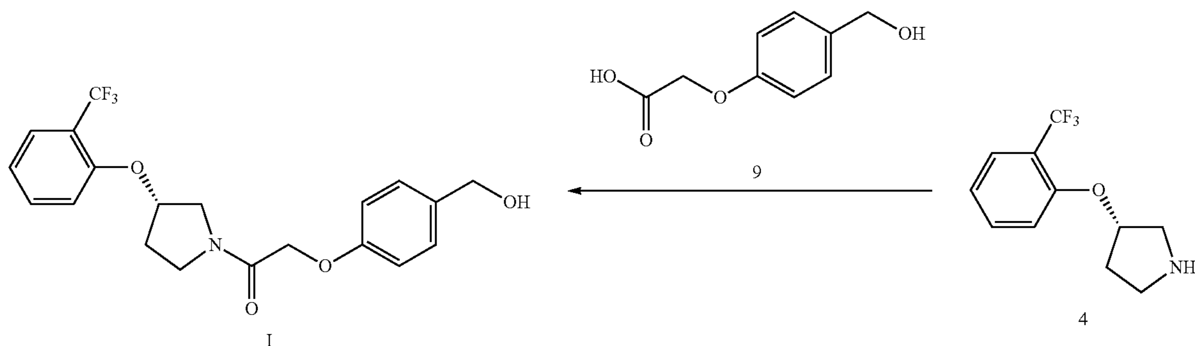
Scheme II
