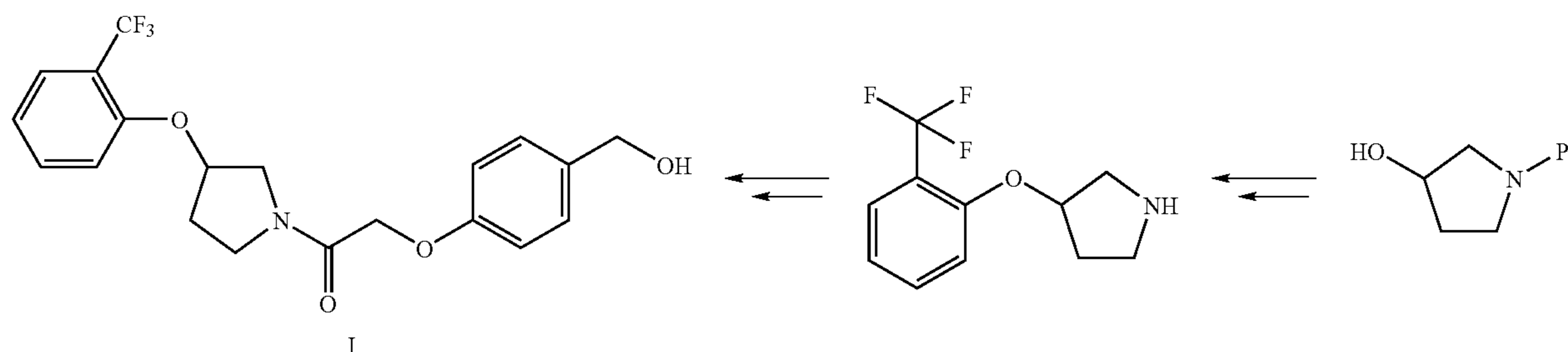
Scheme IV
