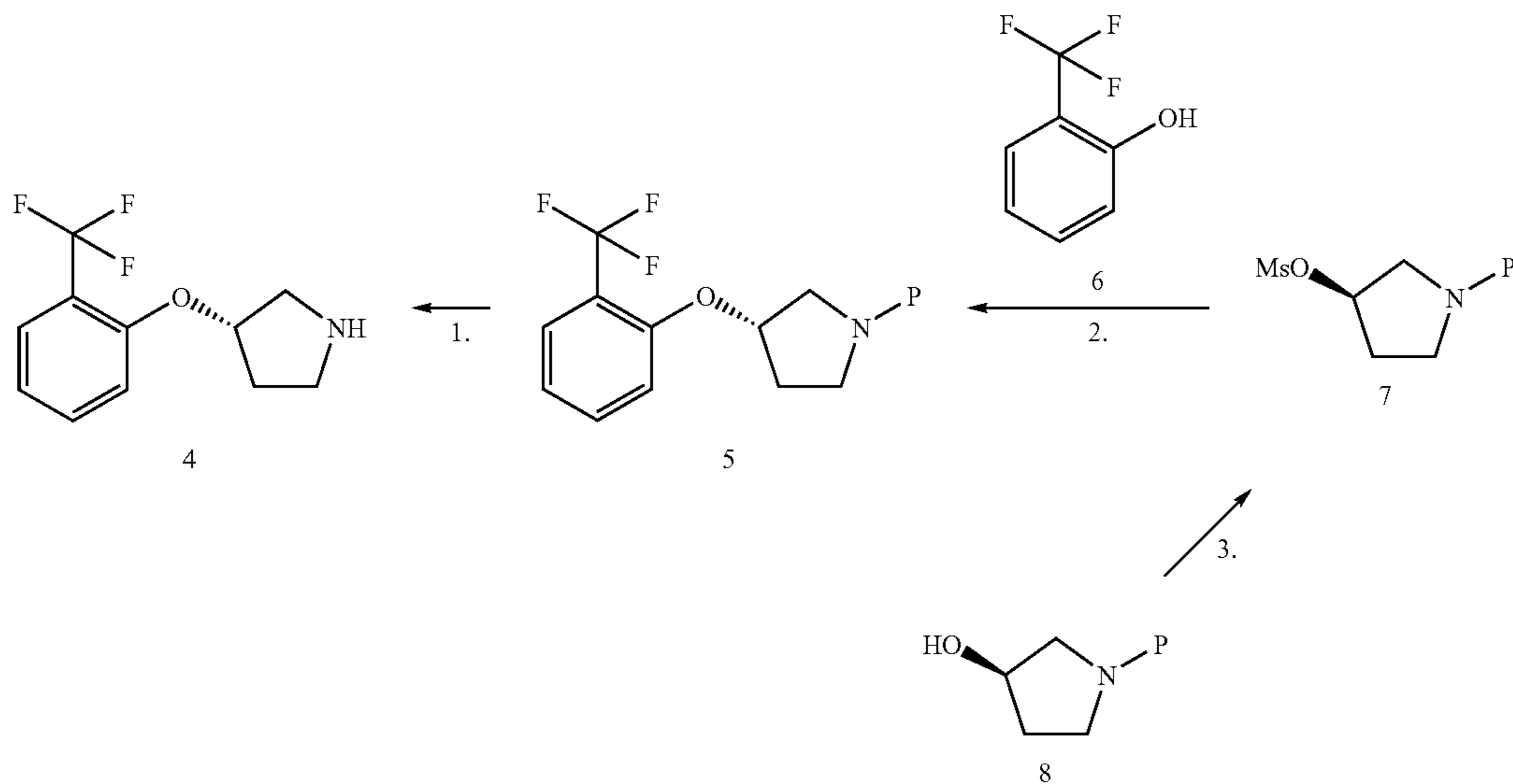
SCHEME III
