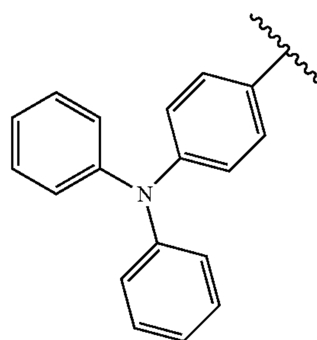
triphenyl amine
