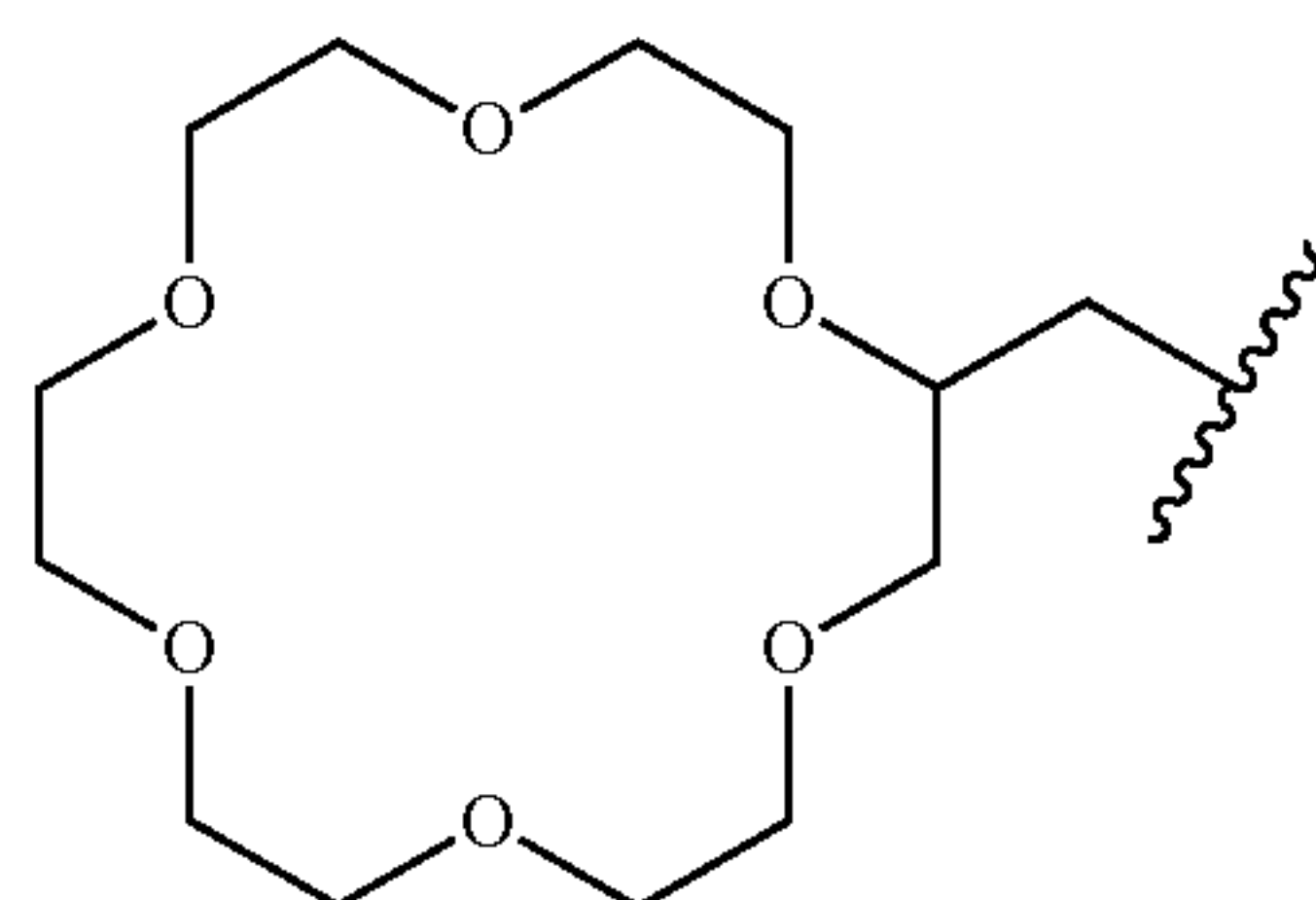
methyl 18-crown-6
