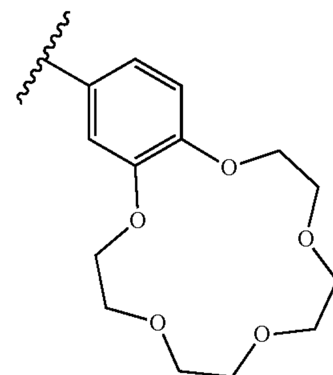
benzo 15-crown-5
