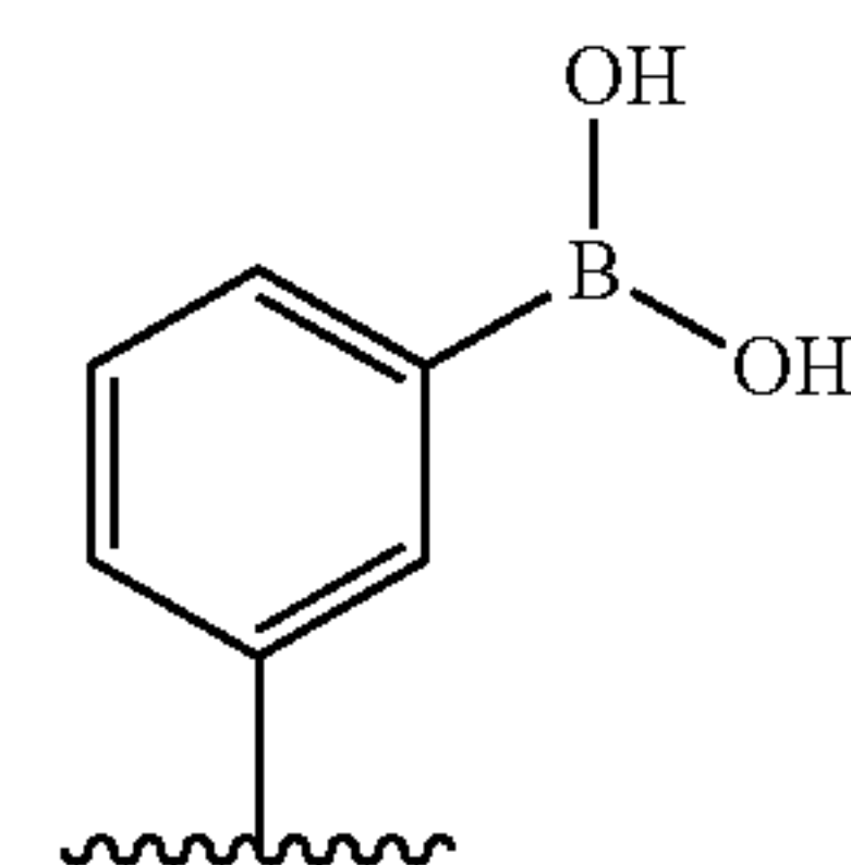
phenyl boronic acid
