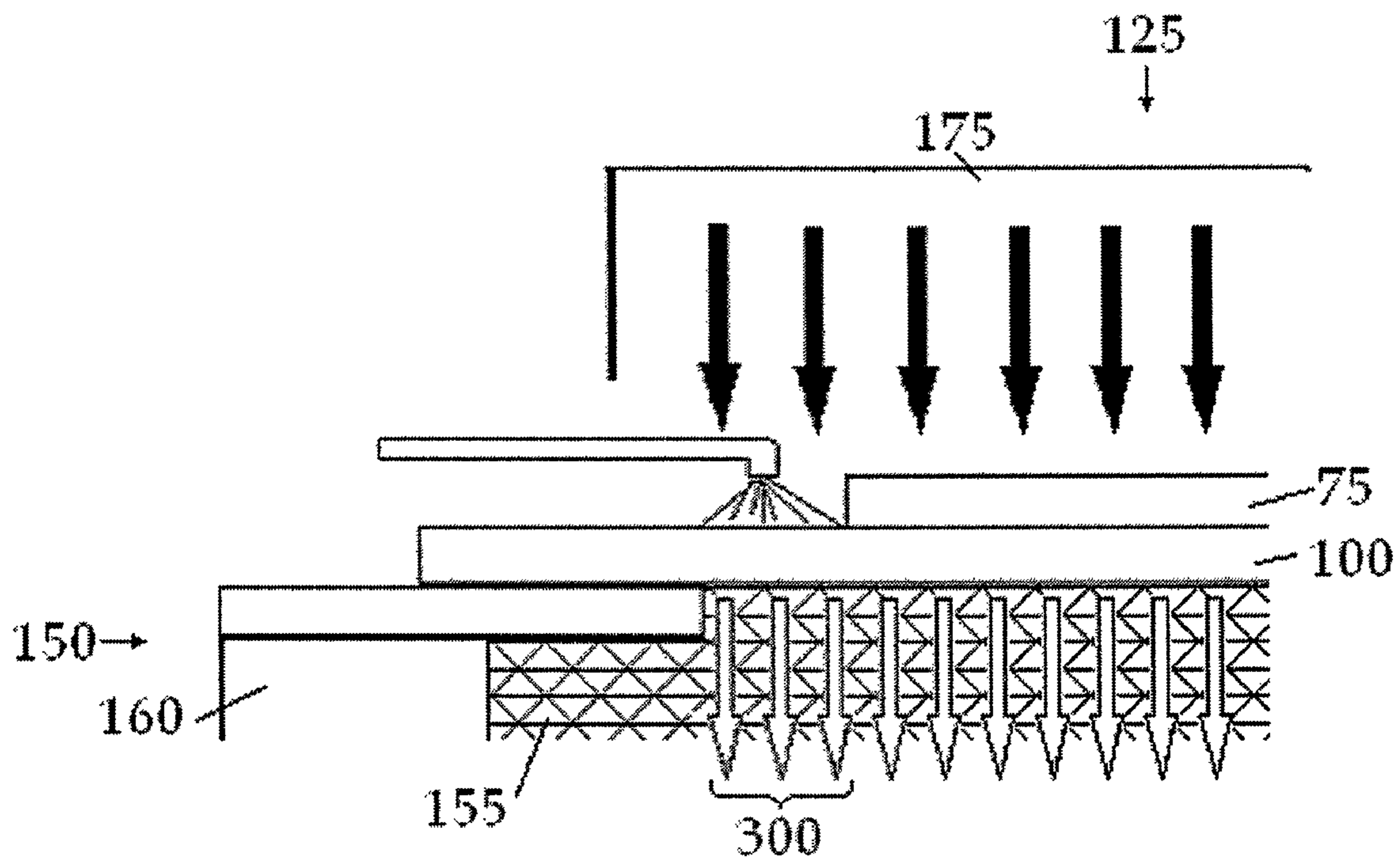
FIG. 5 – PRIOR ART
