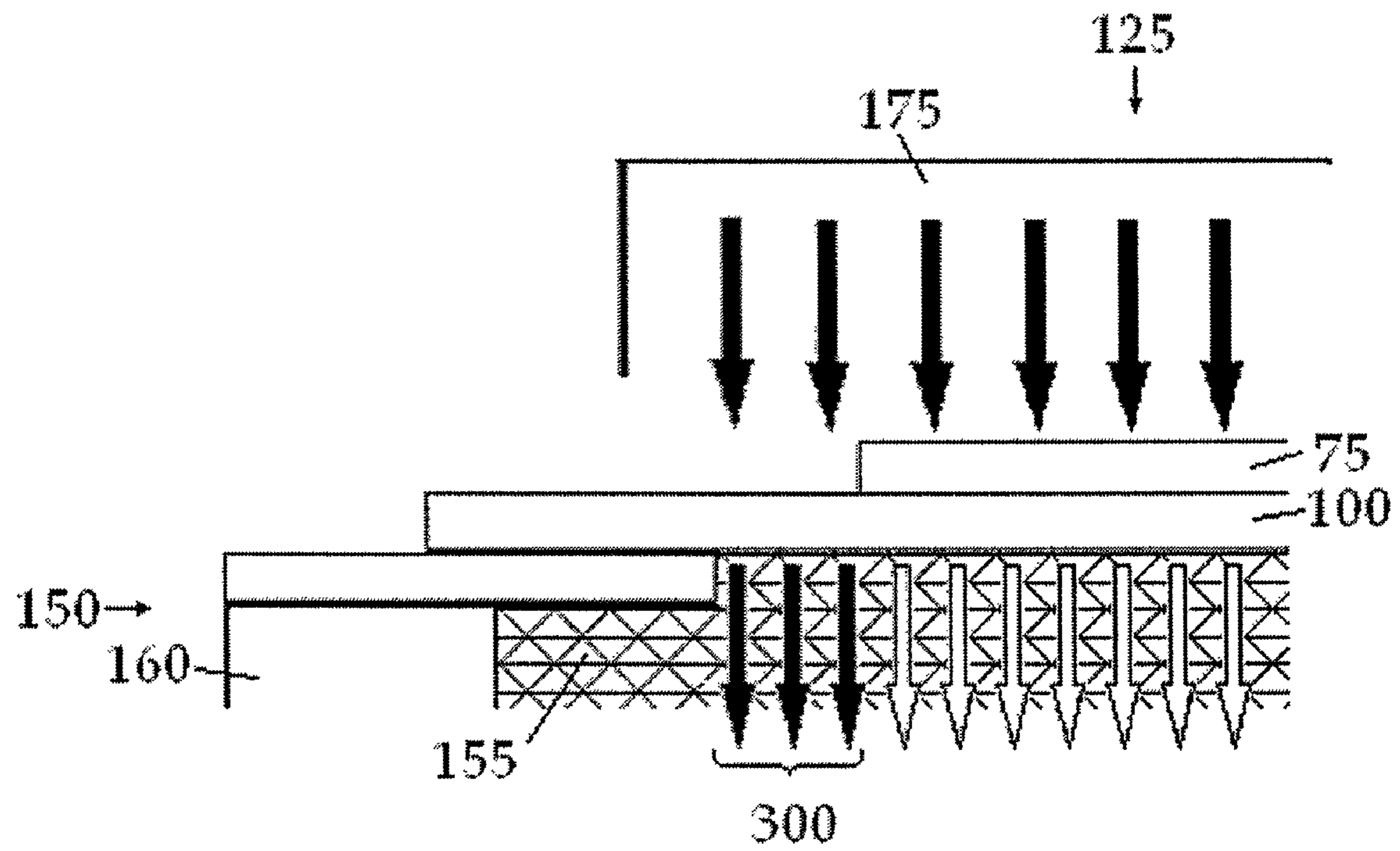
FIG. 3 – PRIOR ART
