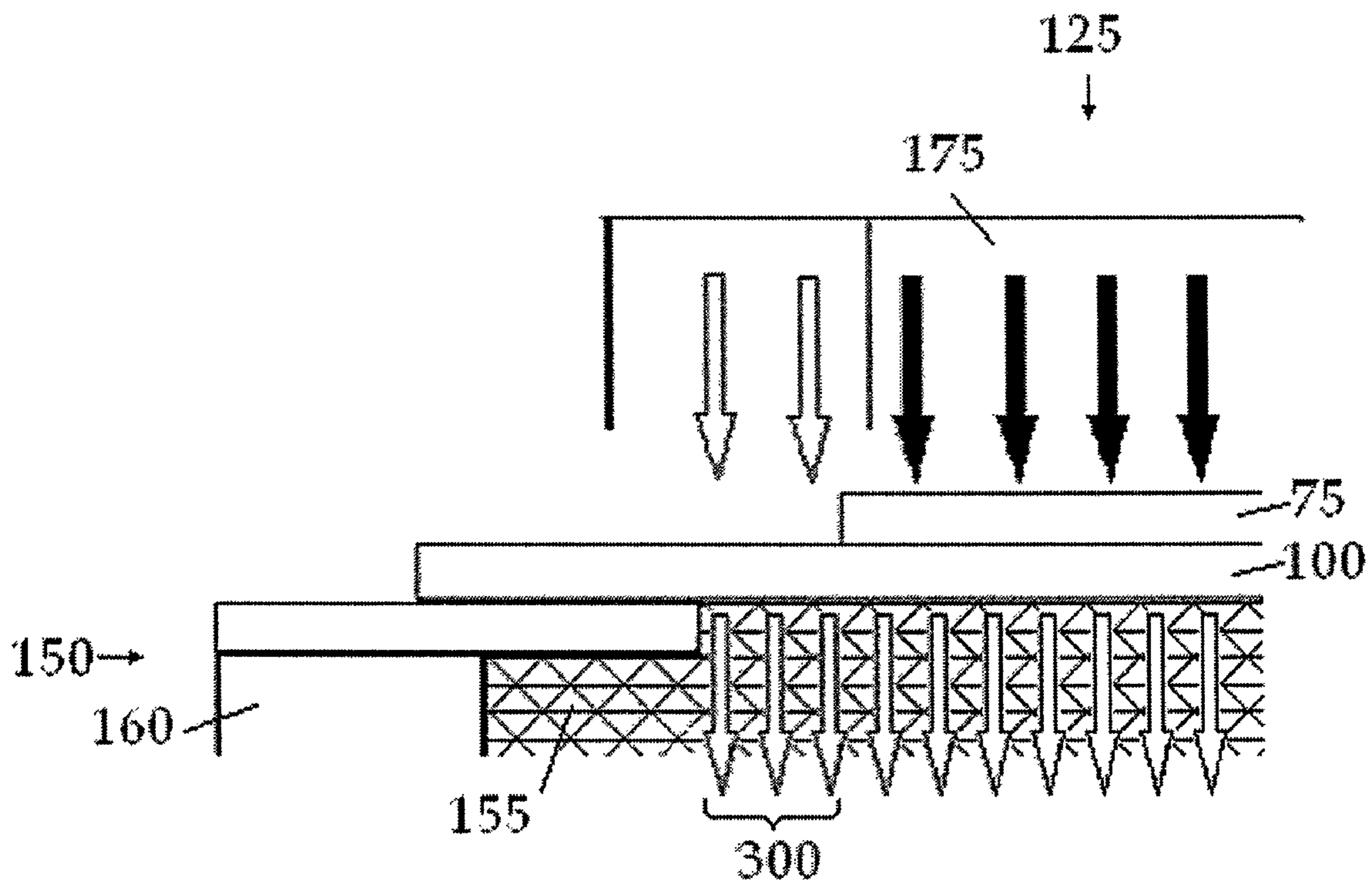
FIG. 4 – PRIOR ART
