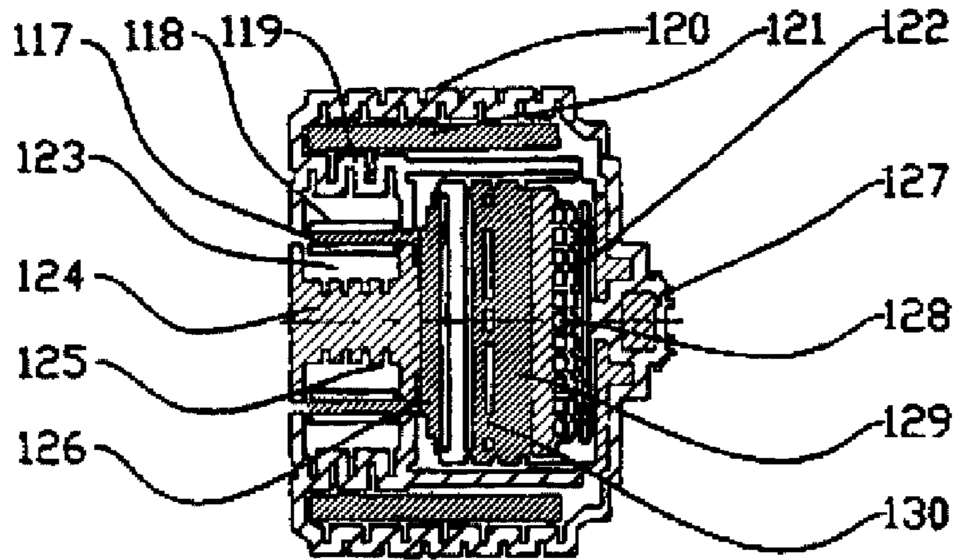
DETAIL 1 Fig.5
