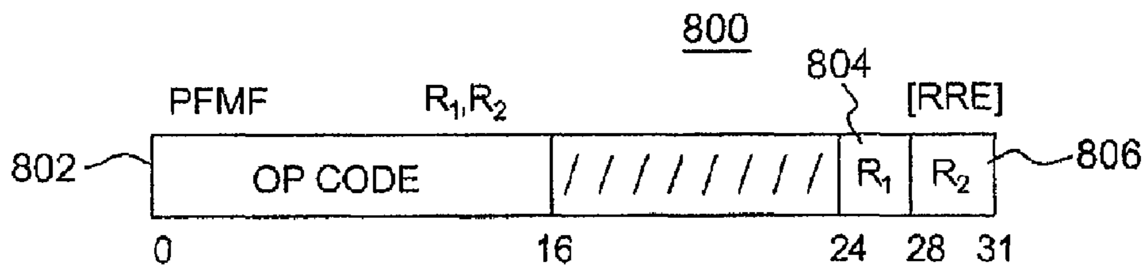
FORMAT OF PFMF INSTRUCTION
