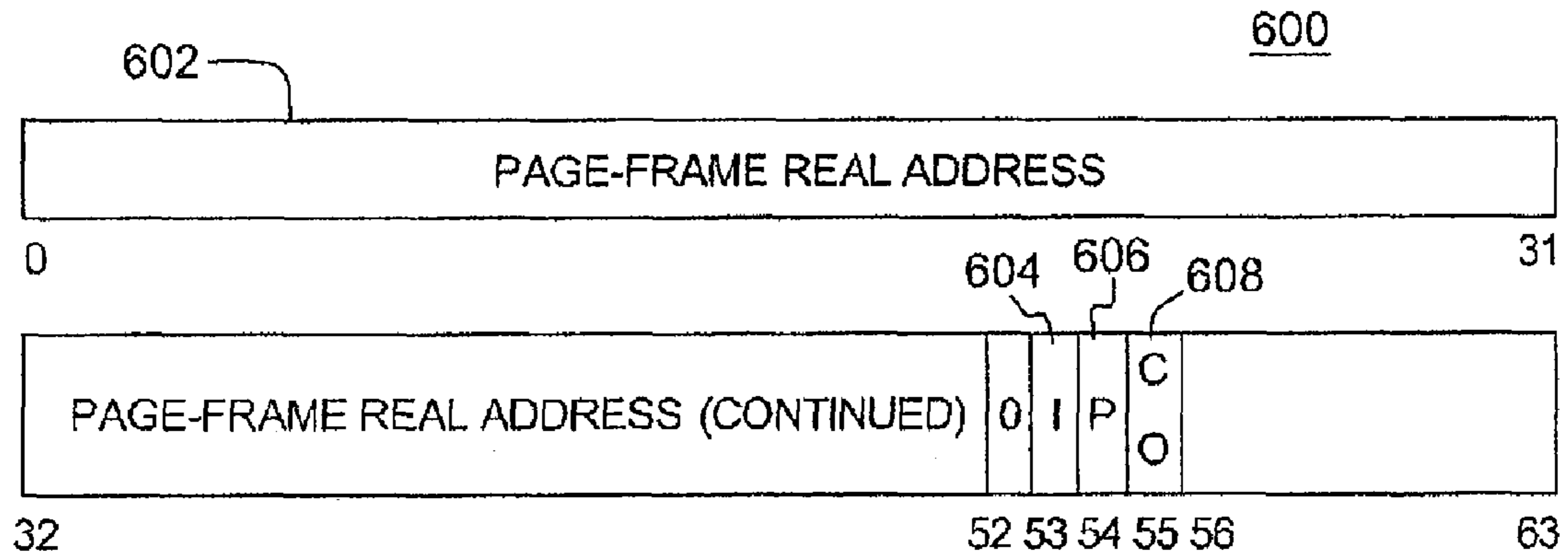
FORMAT OF A PAGE TABLE ENTRY
