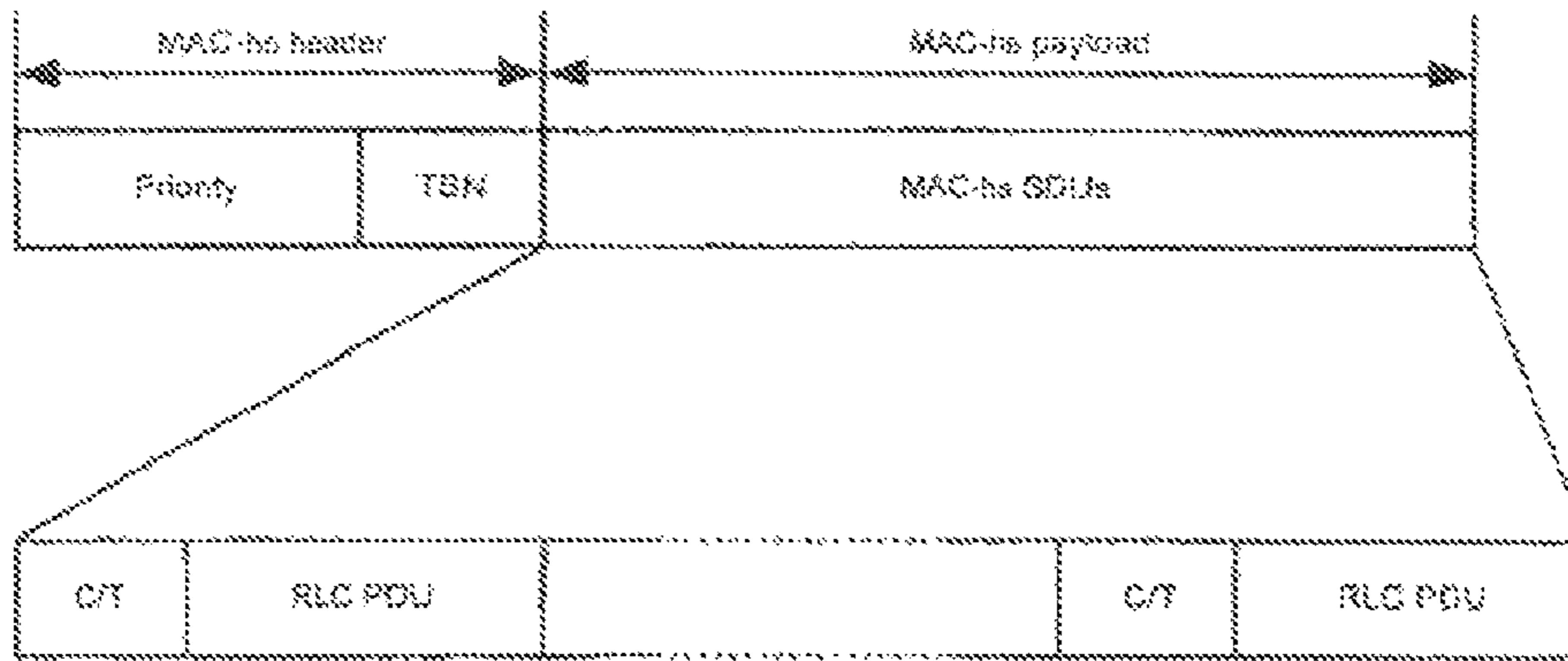
FIG. 7 PRIOR ART
