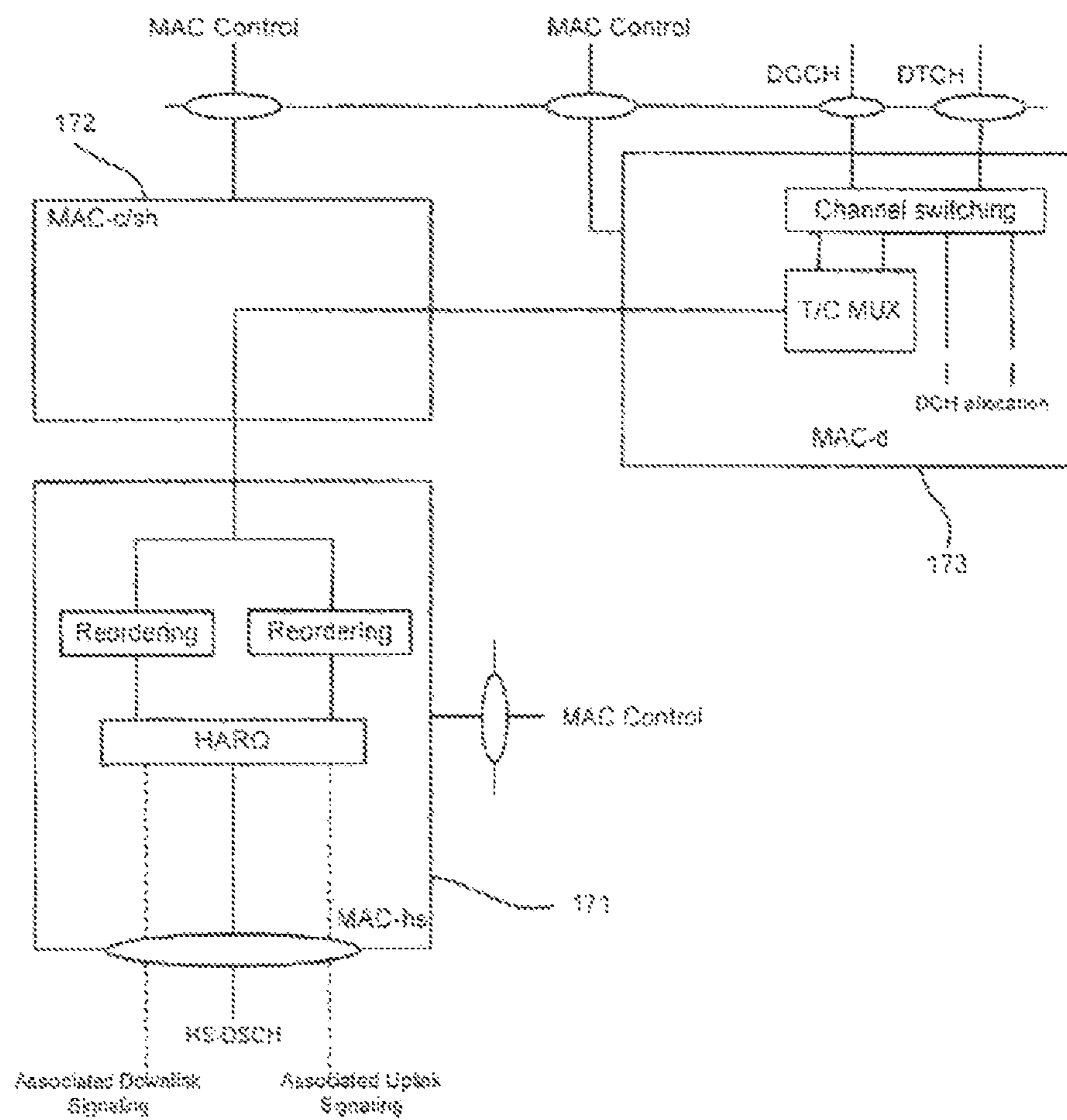
FIG. 5 PRIOR ART
