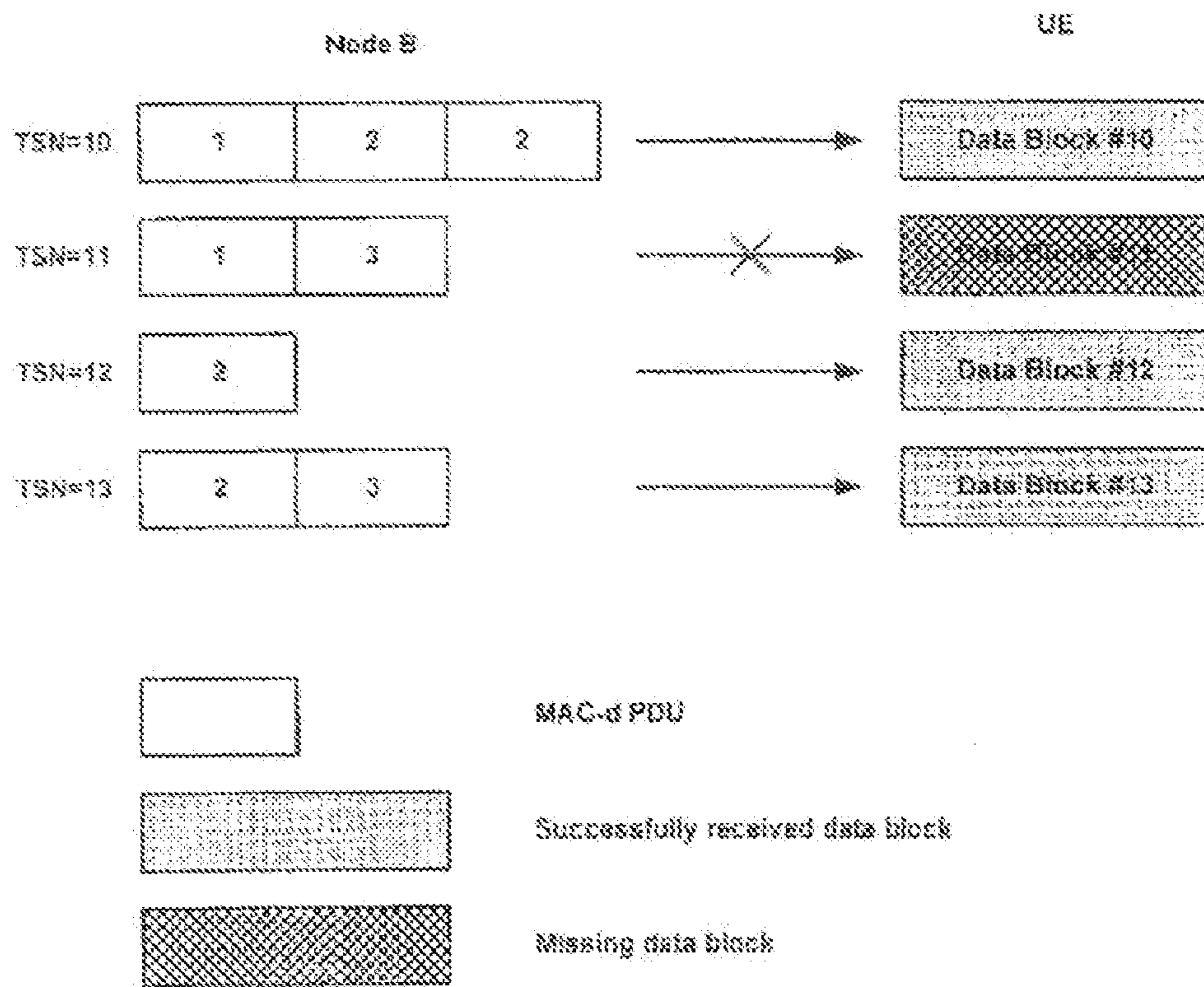
FIG. 9 PRIOR ART
